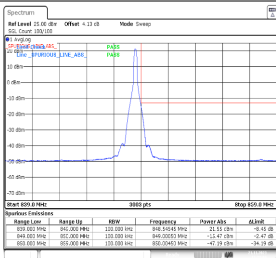
1-N5-PC3-15-10-H-2-DFT-PI2BPSK-Edge_1RB_Right-1@51-Ant41-1--PASS-see graph
