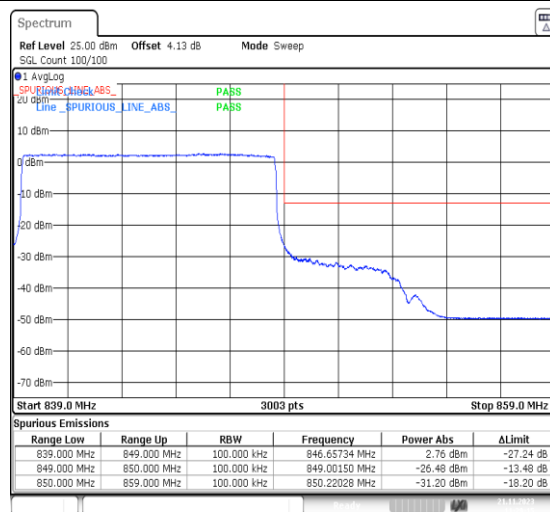
1-N5-PC3-15-10-H-6-CP-QPSK-Outer_Full-52@0-Ant41-1--PASS-see graph
