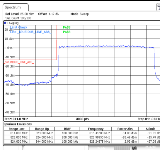
1-N5-PC3-15-20-L-3-DFT-PI2BPSK-Outer_Full-100@0-Ant41-1--PASS-see graph
