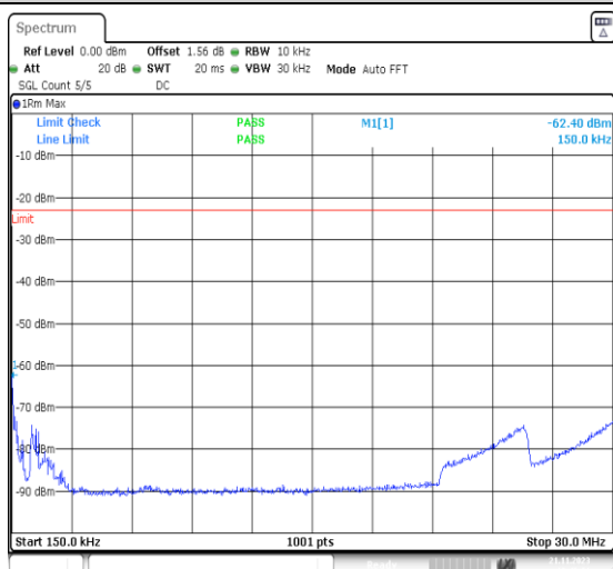
1-N5-PC3-15-20-M-1-DFT-PI2BPSK-Inner_1RB_Left t-1@1-0.15-30-Ant41-0.15--62.40--23-PASS
