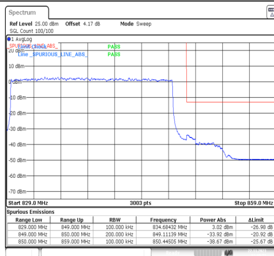
1-N5-PC3-15-20-H-3-DFT-PI2BPSK-Outer_Full-100@0-Ant41-1--PASS-see graph
