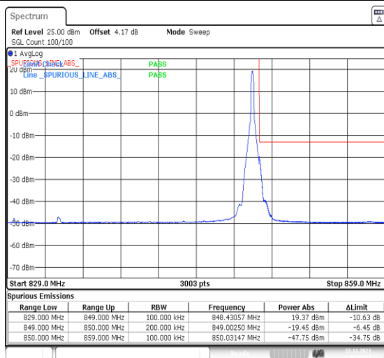
1-N5-PC3-15-20-H-5-CP-QPSK-Edge_1RB_Right-1@105-Ant41-1--PASS-see graph
