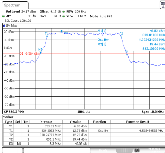
1-N5-PC3-15-5-M-1-DFT-QPSK-Outet_Full-25@0-A Ant41-4.565-5.300-≤5-PASS
