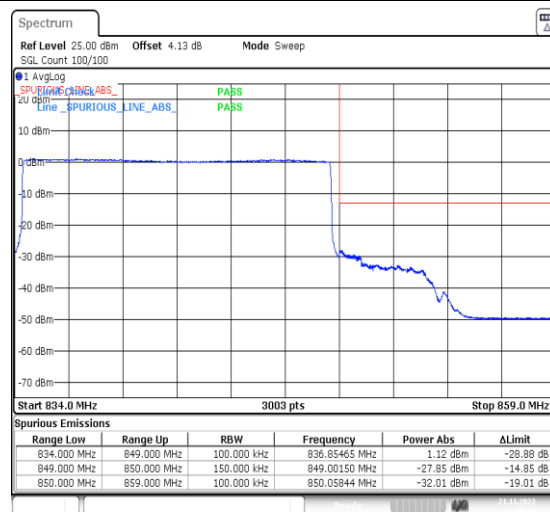
1-N5-PC3-15-15-H-6-CP-QPSK-Outer_Full-79@0-Ant41-1--PASS-see graph
