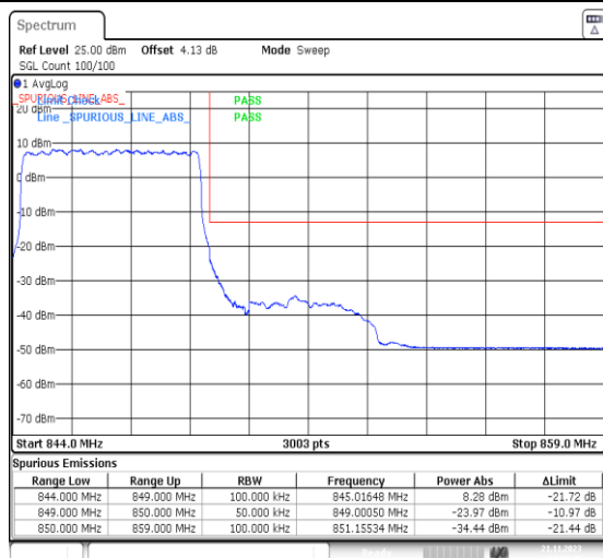
1-N5-PC3-15-5-H-3-DFT-PI2BPSK-Outer_Full-25 @0-Ant41-1--PASS-see graph
