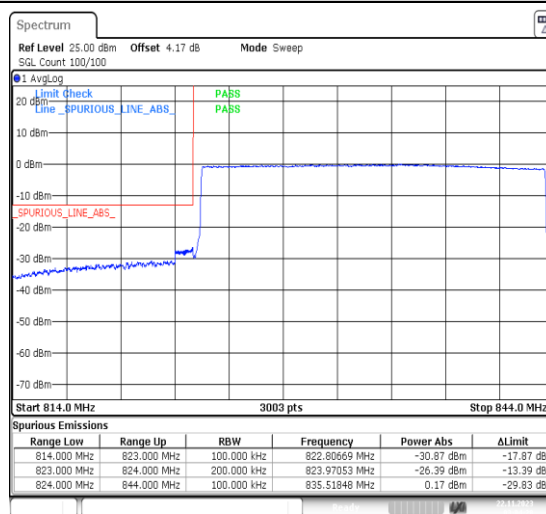
1-N5-PC3-15-20-L-6-CP-QPSK-Outer_Full-106@0-Ant41-1--PASS-see graph
