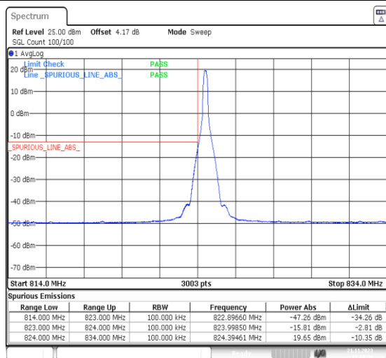
1-N5-PC3-15-10-L-4-CP-QPSK-Edge_1RB_Left-1@0- Ant41-1--PASS-see graph
