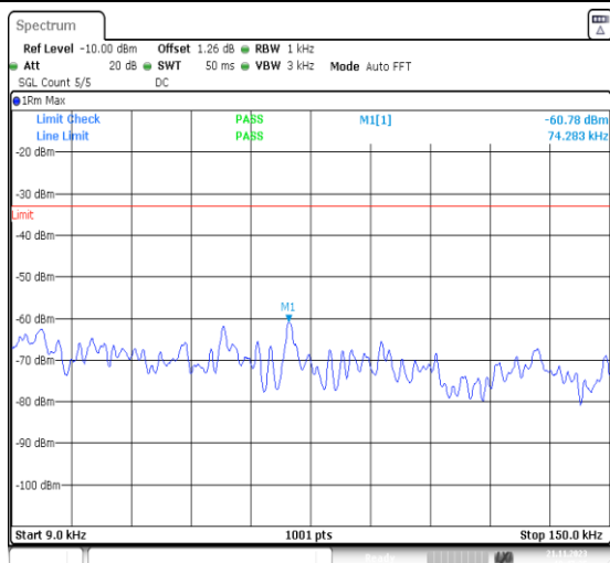
1-N5-PC3-15-20-M-1-DFT-PI2BPSK-Inner_1RB_Lef t-1@1-1000-3000-Ant41-2481.50--28.65--13-PASS
