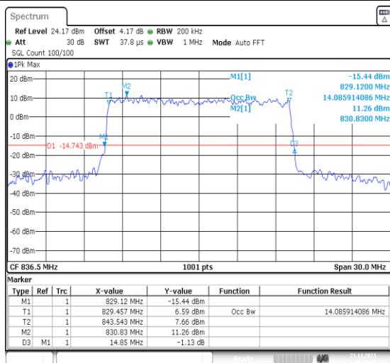
1-N5-PC3-15-15-M-9-CP-256QAM-Outer_Full-79@0- -Ant41-14.086-14.850-≤15-PASS
