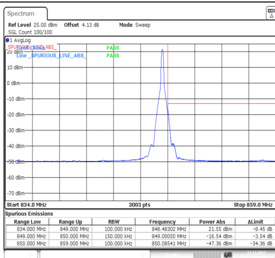
1-N5-PC3-15-15-H-2-DFT-PI2BPSK-Edge_1RB_Right-1@78-Ant41-1--PASS-see graph
