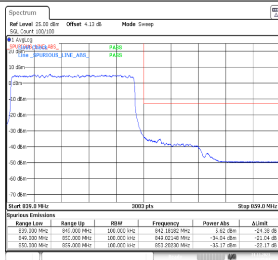
1-N5-PC3-15-10-H-3-DFT-PI2BPSK-Outer_Full-50@0-Ant41-1--PASS-see graph
