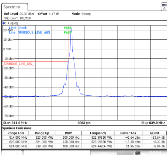
1-N5-PC3-15-15-L-1-DFT-PI2BPSK-Edge_1RB_Left-1 @0-Ant41-1--PASS-see graph
