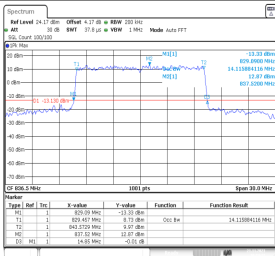
1-N5-PC3-15-15-M-7-CP-16QAM-Outer_Full-79@0- Ant41-14.116-14.850-≤15-PASS
