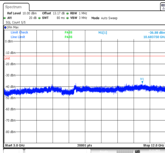
1-N5-PC3-15-20-M-1-DFT-PI2BPSK-Inner_1RB_Left -1@1-3000-12000-Ant41-10694.10--36.88--13-PASS
