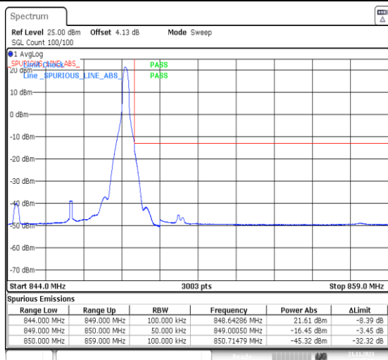
1-N5-PC3-15-5-H-2-DFT-PI2BPSK-Edge_1RB_Right-1 @24-Ant41-1--PASS-see graph
