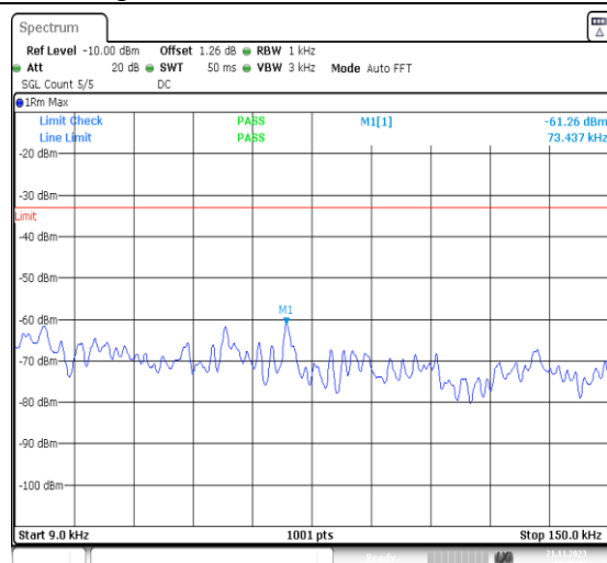
1-N5-PC3-15-20-M-1-DFT-PI2BPSK-Inner_1RB_Left -1@1-0.009-0.15-Ant41-0.02--61.26--33-PASS
