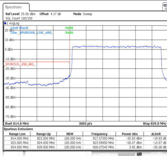
1-N5-PC3-15-15-L-3-DFT-PI2BPSK-Outer_Full-75 @0-Ant41-1--PASS-see graph
