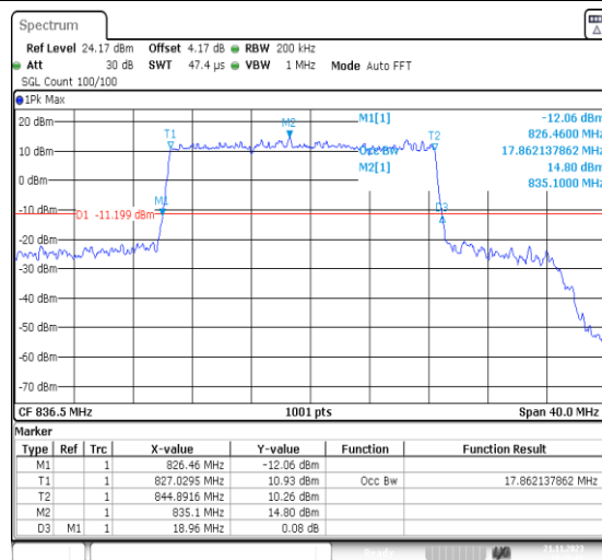
1-N5-PC3-15-20-M-1-DFT-QPSK-Outer_Full-100@0- -Ant41-17.862-18.960-≤20-PASS
