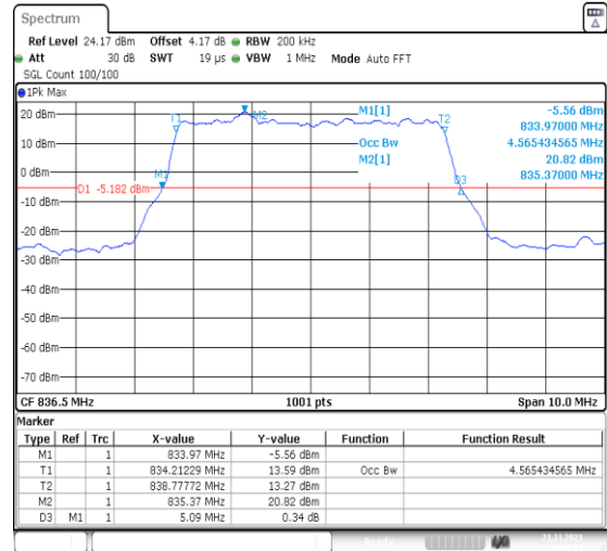
1-N5-PC3-15-5-M-2-DFT-PI2BPSK-Outet_Full-25@0 -Ant41-4.565-5.090-≤5-PASS
