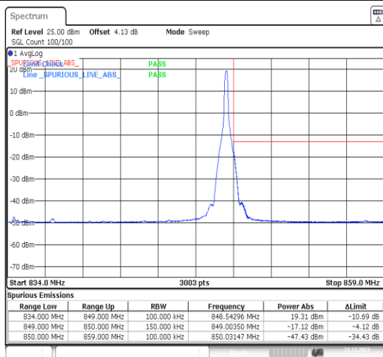
1-N5-PC3-15-15-H-5-CP-QPSK-Edge_1RB_Right-1@78-Ant41-1--PASS-see graph
