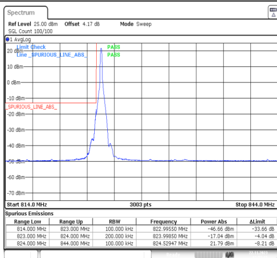
1-N5-PC3-15-20-L-1-DFT-PI2BPSK-Edge_1RB_Left-1@0-Ant41-1--PASS-see graph
