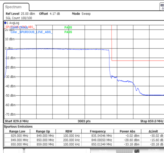
1-N5-PC3-15-20-H-6-CP-QPSK-Outer_Full-106@0-Ant41-1--PASS-see graph
