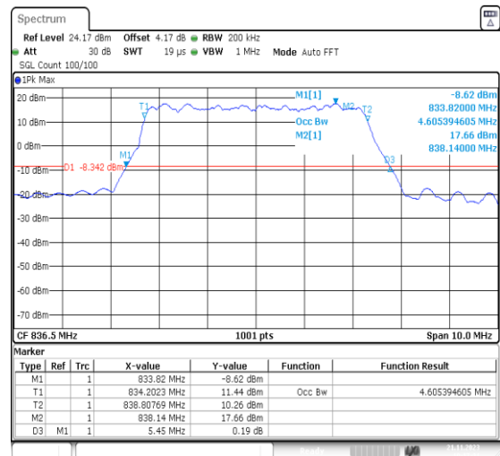
1-N5-PC3-15-5-M-4-DFT-64QAM-Outet_Full-25@0 Ant41-4.605-5.450-≤5-PASS
