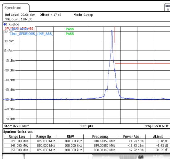
1-N5-PC3-15-20-H-2-DFT-PI2BPSK-Edge_1RB_Right-1@105-Ant41-1--PASS-see graph
