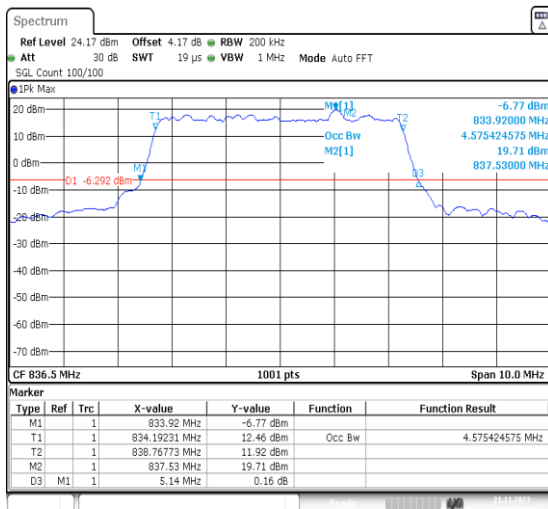
1-N5-PC3-15-5-M-3-DFT-16QAM-Outet_Full-25@0 Ant41-4.575-5.140-≤5-PASS
