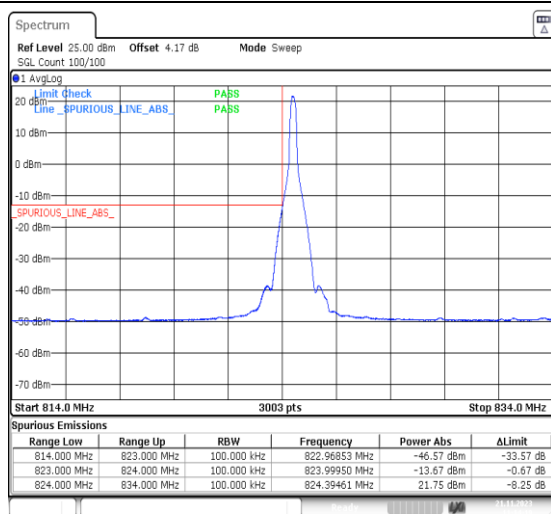
1-N5-PC3-15-10-L-1-DFT-PI2BPSK-Edge_1RB_Left-1 @0-Ant41-1--PASS-see graph
