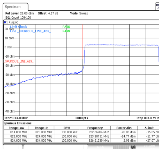
1-N5-PC3-15-10-L-6-CP-QPSK-Outer_Full-52@0- Ant41-1--PASS-see graph
