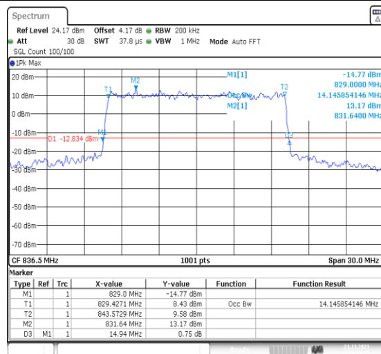
1-N5-PC3-15-15-M-8-CP-64QAM-Outer_Full-79@0- Ant41-14.146-14.940-≤15-PASS
