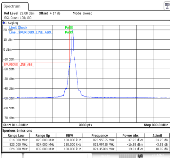
1-N5-PC3-15-15-L-4-CP-QPSK-Edge_1RB_Left-1@0-Ant41-1--PASS-see graph
