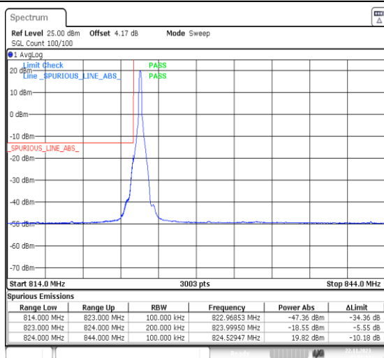
1-N5-PC3-15-20-L-4-CP-QPSK-Edge_1RB_Left-1@0-Ant41-1--PASS-see graph
