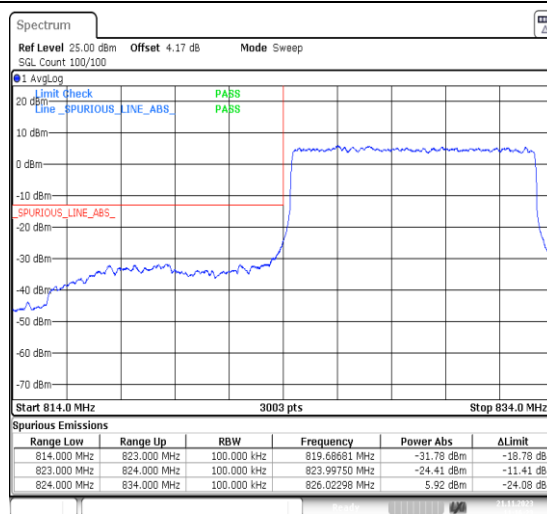
1-N5-PC3-15-10-L-3-DFT-PI2BPSK-Outer_Full-50 @0-Ant41-1--PASS-see graph
