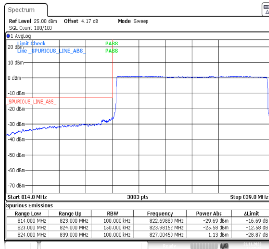
1-N5-PC3-15-15-L-6-CP-QPSK-Outer_Full-79@0-Ant41-1--PASS-see graph
