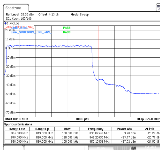
1-N5-PC3-15-15-H-3-DFT-PI2BPSK-Outer_Full-75@0-Ant41-1--PASS-see graph
