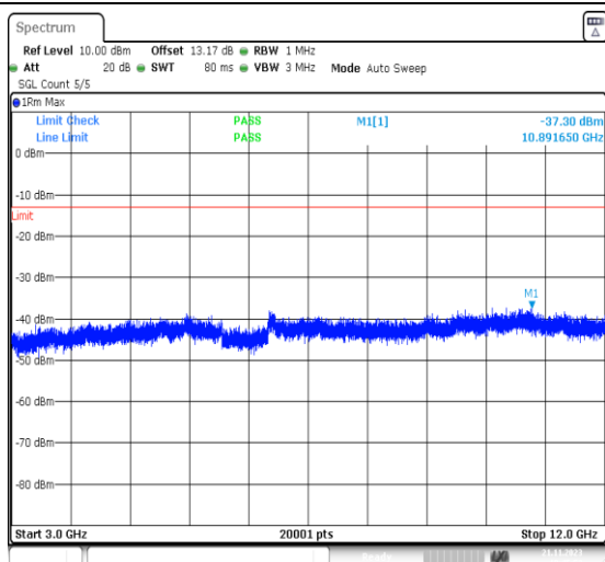
1-N5-PC3-15-20-L-1-DFT-PI2BPSK-Inner_1RB_Left -1@1-3000-12000-Ant41-6994.20--37.30--13-PASS
