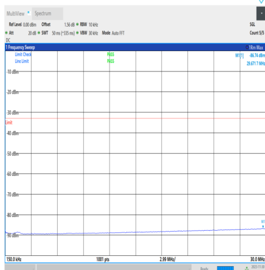
NTNV_N66_PC3_15_40_M_TID1_0.15_30_#1
