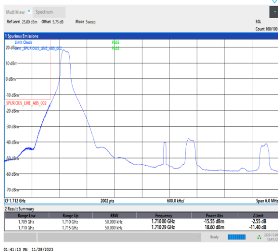
1-N66-PC3-15-5-L-1-DFT-PI2BPSK-Edge_1RB_Left-1 @0-Ant14-1-seegraph-PASS-see graph
