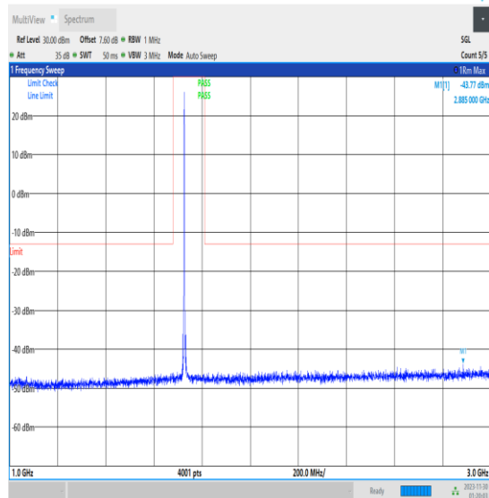
NTNV_N66_PC3_15_40_M_TID1_1000_3000_#1
