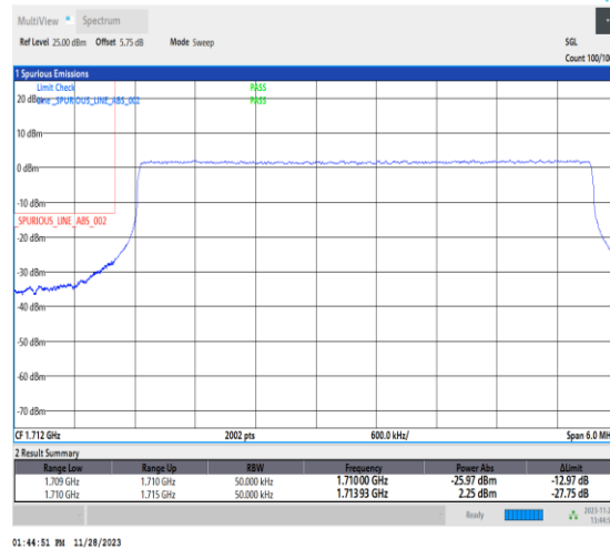
1-N66-PC3-15-5-L-6-CP-QPSK-Outer_Full-25@0-Ant14-1-seegraph-PASS-see graph
