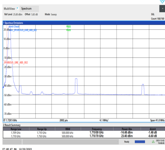
1-N66-PC3-15-35-L-4-CP-QPSK-Edge_1RB_Left-1@ 0-Ant14-1-seegraph-PASS-see graph
