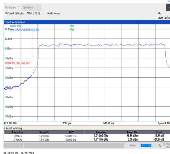
1-N66-PC3-15-5-L-3-DFT-PI2BPSK-Outer_Full-25 @0-Ant14-1-seegraph-PASS-see graph
