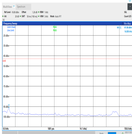
NTNV_N66_PC3_15_40_M_TID1_0.009_0.15_#1
