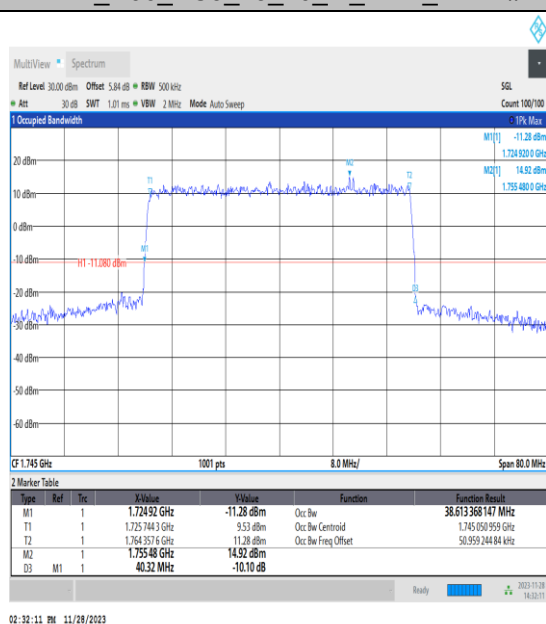
NTNV_N66_PC3_15_40_M_TID4_Ant14#1
