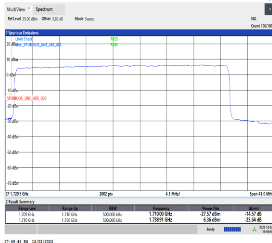
1-N66-PC3-15-35-L-3-DFT-PI2BPSK-Outer_Full-18 0@0-Ant14-1-seegraph-PASS-see graph
