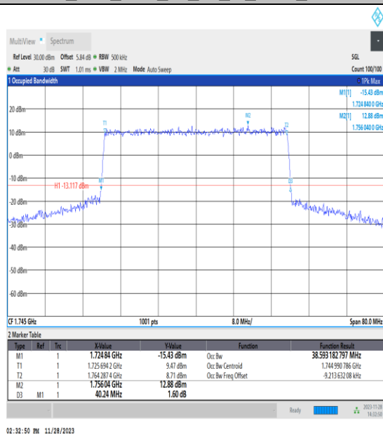
NTNV_N66_PC3_15_40_M_TID8_Ant14#1
