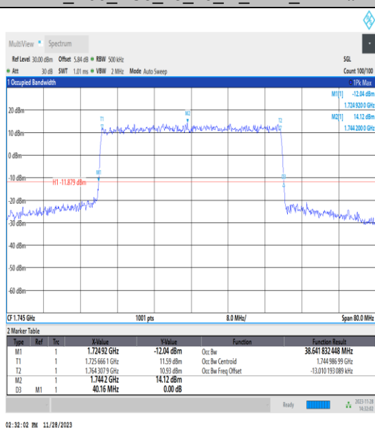
NTNV_N66_PC3_15_40_M_TID3_Ant14#1
