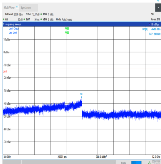
NTNV_N66_PC3_15_40_M_TID1_3000_12000_#1
