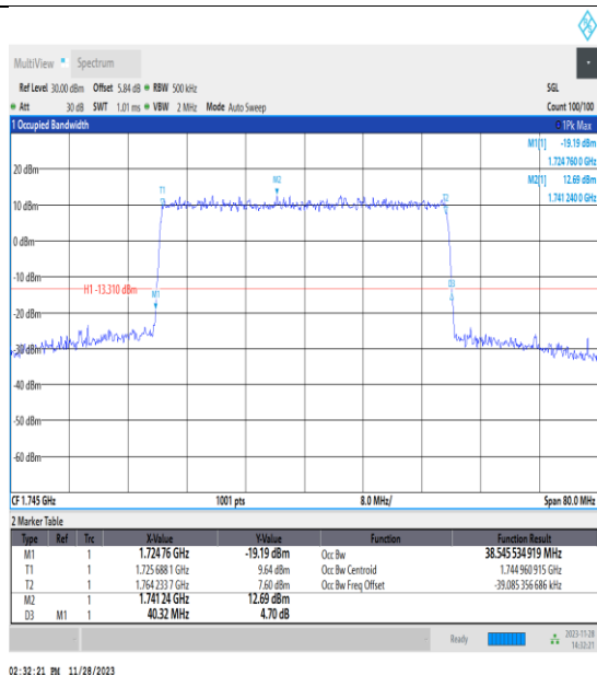
NTNV_N66_PC3_15_40_M_TID5_Ant14#1
