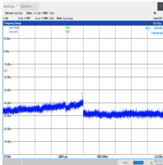
NTNV_N66_PC3_15_40_L_TID1_3000_12000_#1
