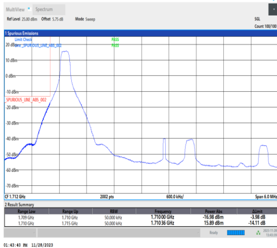
1-N66-PC3-15-5-L-4-CP-QPSK-Edge_1RB_Left-1@0-Ant14-1-seegraph-PASS-see graph
