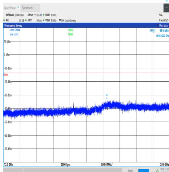
NTNV_N66_PC3_15_40_M_TID1_12000_20000_#1
