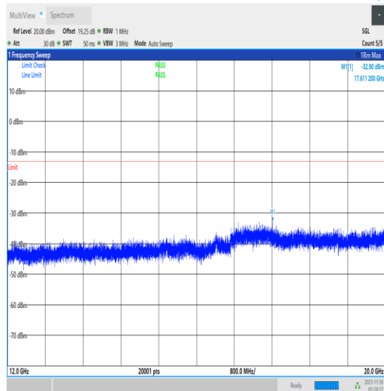
NTNV_N66_PC3_15_40_L_TID1_12000_20000_#1
