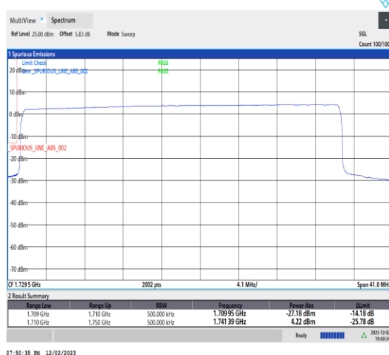
1-N66-PC3-15-35-L-6-CP-QPSK-Outer_Full-188@0 -Ant14-1-seegraph-PASS-see graph
