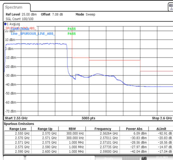
1-N7-PC3-15-20-H-3-DFT-PI2BPSK-Outer_Full-100@0-Ant31-1--PASS-see graph
