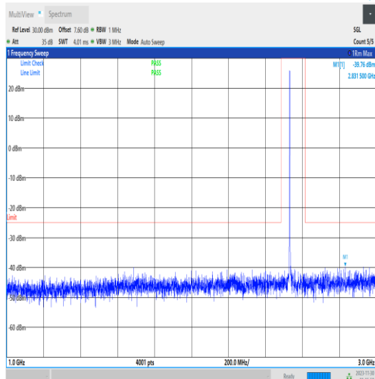
NTNV_N7_PC3_15_40_H_TID1_1000_3000_#1
