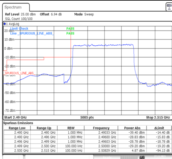
1-N7-PC3-15-10-L-3-DFT-PI2BPSK-Outer_Full-50 @0-Ant31-1--PASS-see graph
