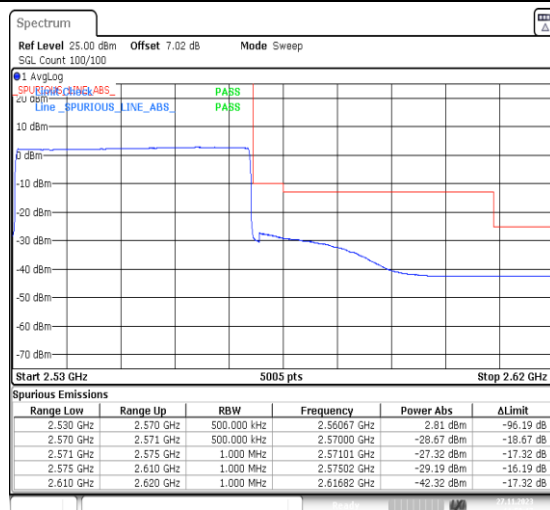
1-N7-PC3-15-40-H-3-DFT-PI2BPSK-Outer_Full-216@0-Ant31-1--PASS-see graph
