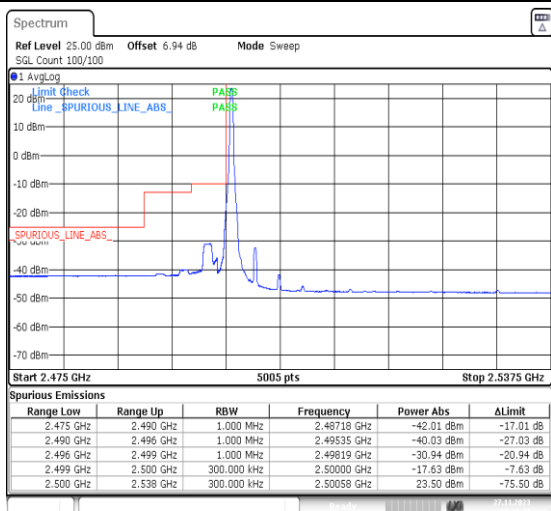
1-N7-PC3-15-25-L-1-DFT-PI2BPSK-Edge_1RB_Left-1 @0-Ant31-1--PASS-see graph
