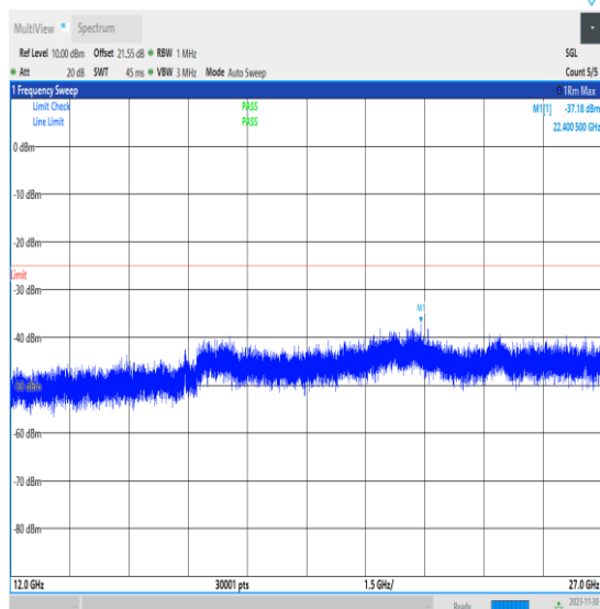
NTVN_N7_PC3_15_40_M_TID1_12000_27000_#1
