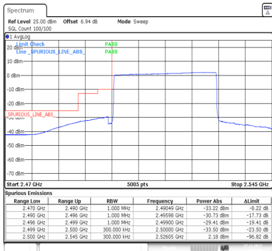
1-N7-PC3-15-30-L-6-CP-QPSK-Outer_Full-160@0- -Ant31-1--PASS-see graph
