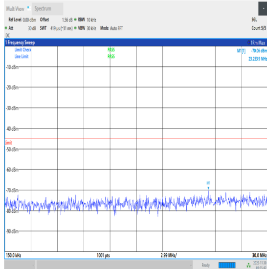
NTNV_N7_PC3_15_40_H_TID1_0.15_30_#1
