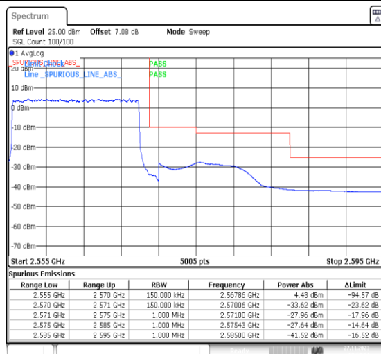
1-N7-PC3-15-15-H-3-DFT-PI2BPSK-Outer_Full-75@0-Ant31-1--PASS-see graph
