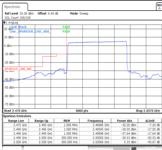
1-N7-PC3-15-25-L-3-DFT-PI2BPSK-Outer_Full-12 8@0-Ant31-1--PASS-see graph
