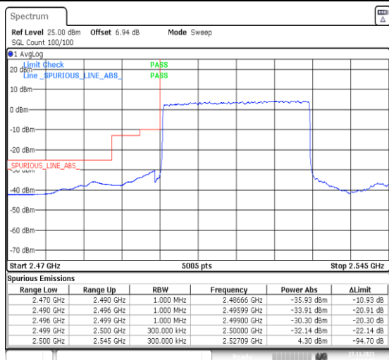
1-N7-PC3-15-30-L-3-DFT-PI2BPSK-Outer_Full-16 0@0-Ant31-1--PASS-see graph
