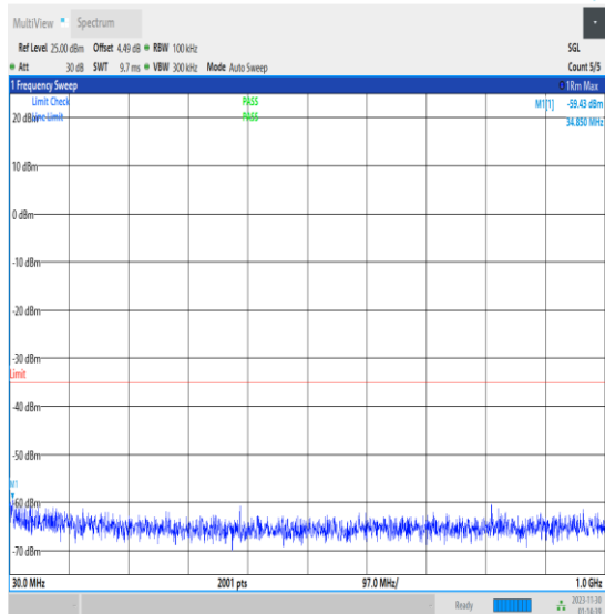
NTVN_N7_PC3_15_40_M_TID1_30_1000_#1
