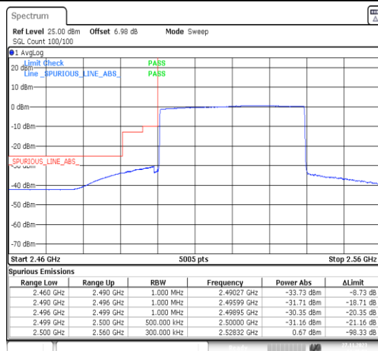
1-N7-PC3-15-40-L-3-DFT-PI2BPSK-Outer_Full-21 6@0-Ant31-1--PASS-see graph
