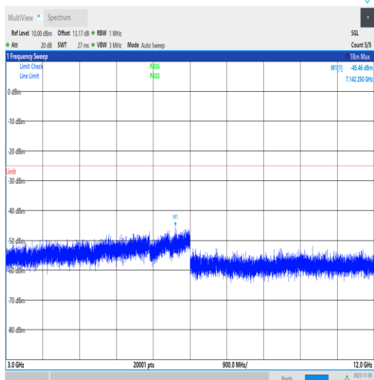
NTVN_N7_PC3_15_40_M_TID1_3000_12000_#1
