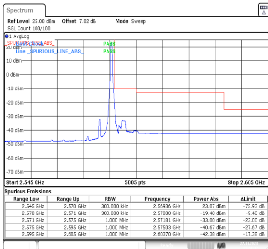
1-N7-PC3-15-25-H-2-DFT-PI2BPSK-Edge_1RB_Right-1@132-Ant31-1--PASS-see graph
