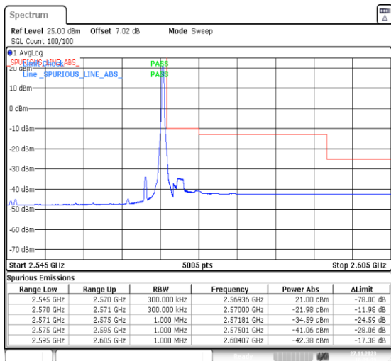
1-N7-PC3-15-25-H-5-CP-QPSK-Edge_1RB_Right-1@132-Ant31-1--PASS-see graph
