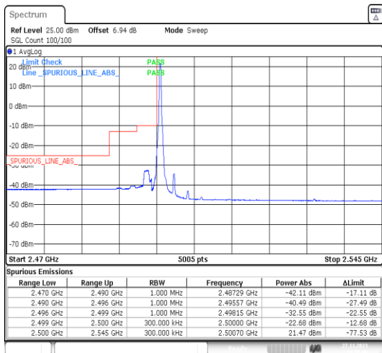
1-N7-PC3-15-30-L-4-CP-QPSK-Edge_1RB_Left-1@0- Ant31-1--PASS-see graph
