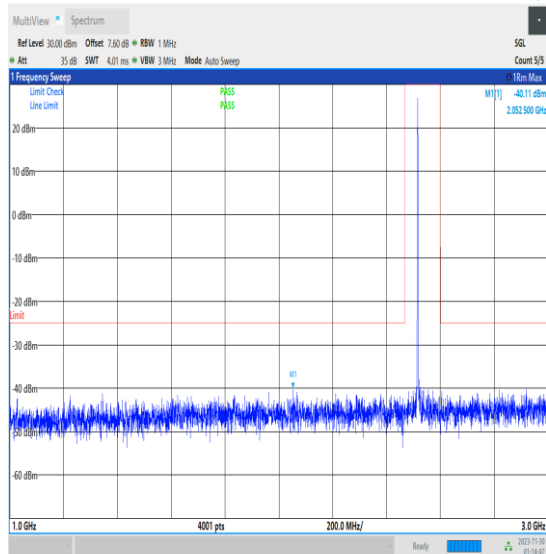
NTVN_N7_PC3_15_40_M_TID1_1000_3000_#1
