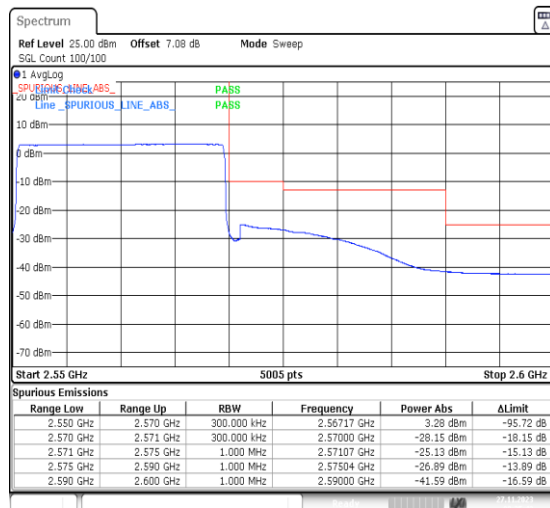
1-N7-PC3-15-20-H-6-CP-QPSK-Outer_Full-106@0-Ant31-1--PASS-see graph
