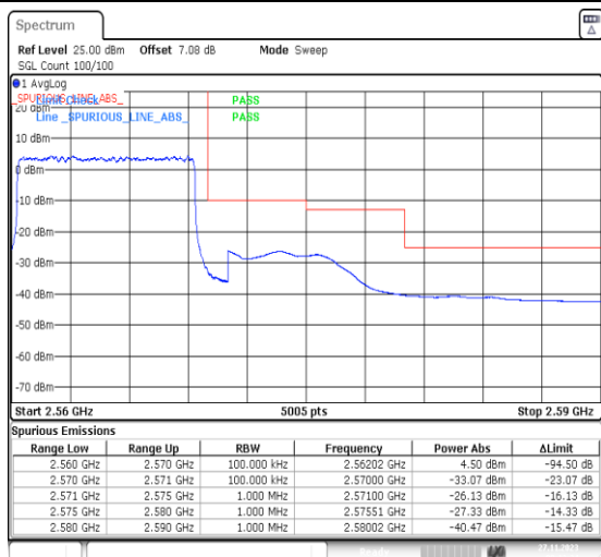
1-N7-PC3-15-10-H-3-DFT-PI2BPSK-Outer_Full-50@0-Ant31-1--PASS-see graph
