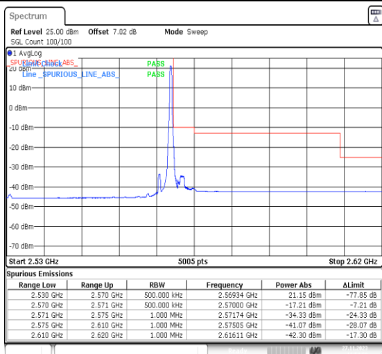
1-N7-PC3-15-40-H-2-DFT-PI2BPSK-Edge_1RB_Right-1@215-Ant31-1--PASS-see graph
