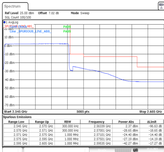
1-N7-PC3-15-25-H-6-CP-QPSK-Outer_Full-133@0-Ant31-1--PASS-see graph
