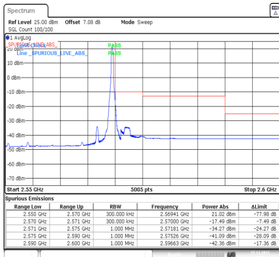
1-N7-PC3-15-20-H-5-CP-QPSK-Edge_1RB_Right-1@105-Ant31-1--PASS-see graph
