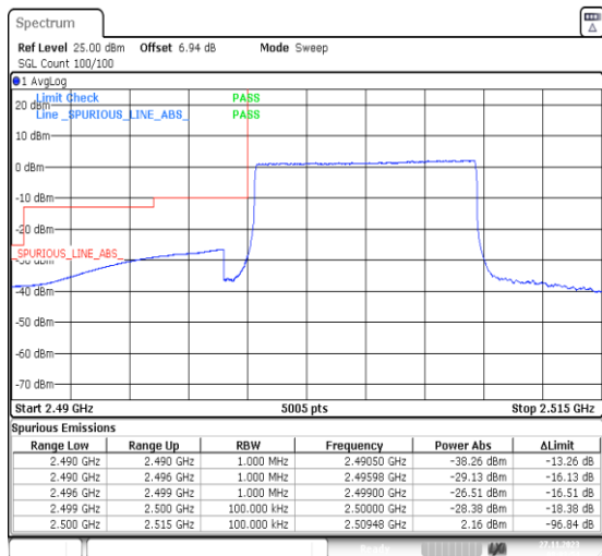
1-N7-PC3-15-10-L-6-CP-QPSK-Outer_Full-52@0-Ant31-1--PASS-see graph
