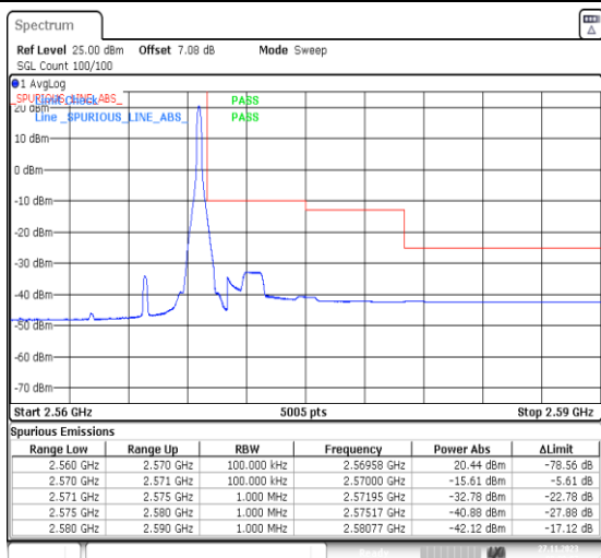
1-N7-PC3-15-10-H-2-DFT-PI2BPSK-Edge_1RB_Right-1@51-Ant31-1--PASS-see graph
