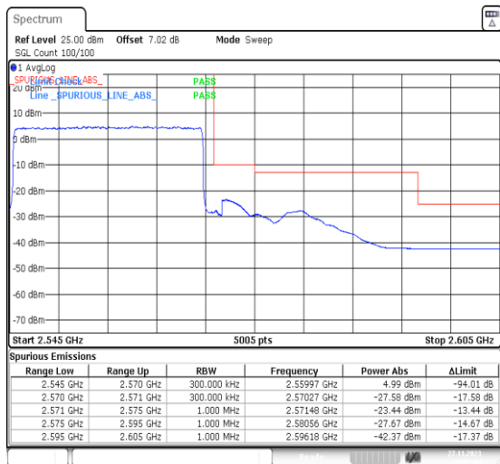
1-N7-PC3-15-25-H-3-DFT-PI2BPSK-Outer_Full-128@0-Ant31-1--PASS-see graph
