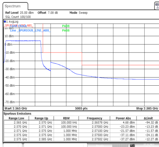
1-N7-PC3-15-5-H-6-CP-QPSK-Outer_Full-25@0- Ant31-1--PASS-see graph
