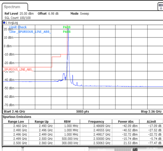
1-N7-PC3-15-40-L-1-DFT-PI2BPSK-Edge_1RB_Left-1 @0-Ant31-1--PASS-see graph
