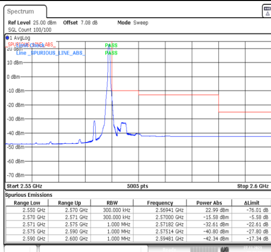
1-N7-PC3-15-20-H-2-DFT-PI2BPSK-Edge_1RB_Right-1@105-Ant31-1--PASS-see graph
