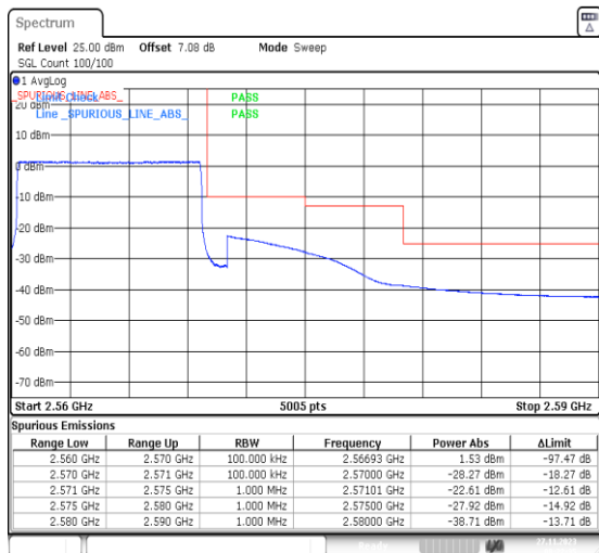
1-N7-PC3-15-10-H-6-CP-QPSK-Outer_Full-52@0-Ant31-1--PASS-see graph
