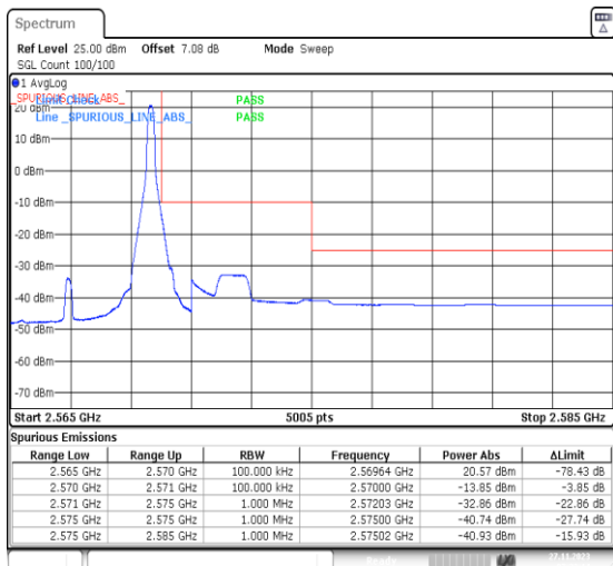
1-N7-PC3-15-5-H-2-DFT-PI2BPSK-Edge_1RB_Right-1 @24-Ant31-1--PASS-see graph
