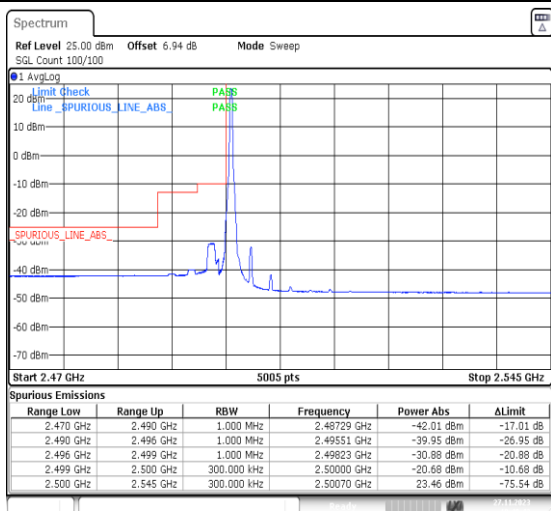
1-N7-PC3-15-30-L-1-DFT-PI2BPSK-Edge_1RB_Left-1 @0-Ant31-1--PASS-see graph
