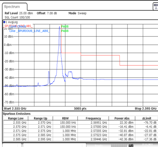
1-N7-PC3-15-15-H-2-DFT-PI2BPSK-Edge_1RB_Right-1@78-Ant31-1--PASS-see graph
