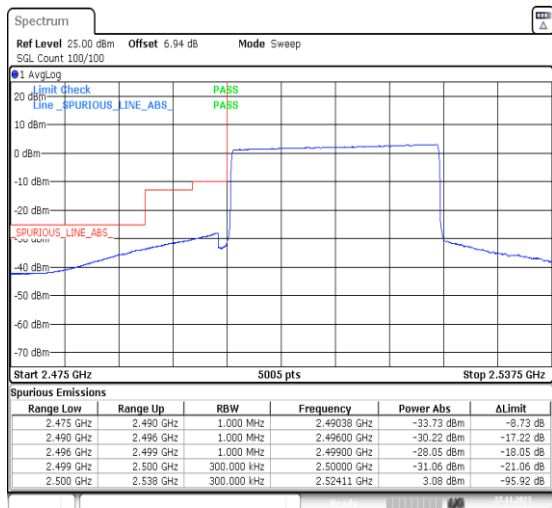
1-N7-PC3-15-25-L-6-CP-QPSK-Outer_Full-133@0-Ant31-1--PASS-see graph
