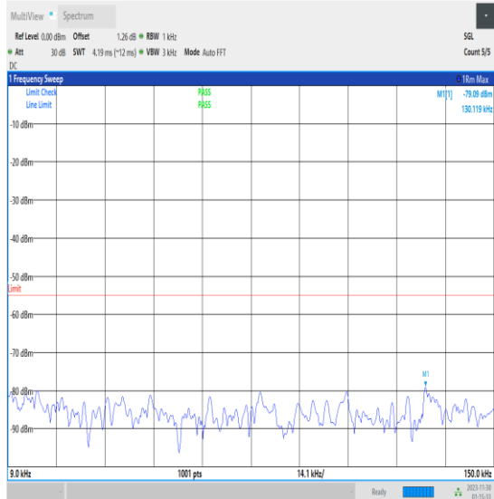
NTNV_N7_PC3_15_40_H_TID1_0.009_0.15_#1
