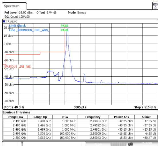
1-N7-PC3-15-10-L-4-CP-QPSK-Edge_1RB_Left-1@0-Ant31-1--PASS-see graph
