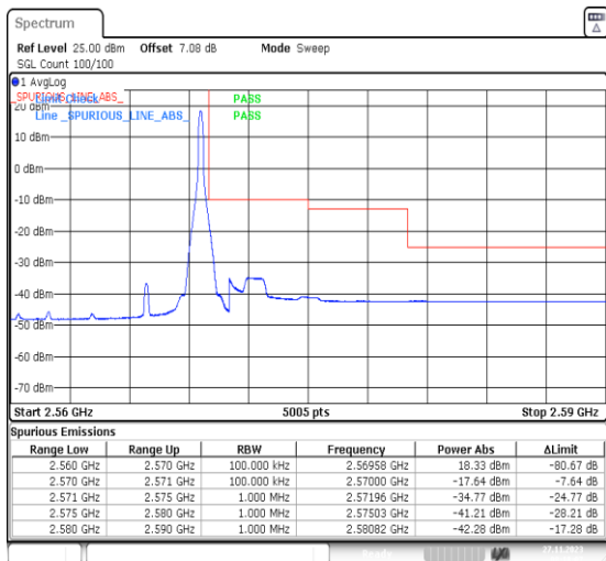
1-N7-PC3-15-10-H-5-CP-QPSK-Edge_1RB_Right-1@51-Ant31-1--PASS-see graph
