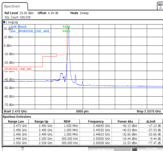
1-N7-PC3-15-25-L-4-CP-QPSK-Edge_1RB_Left-1@0-Ant31-1--PASS-see graph
