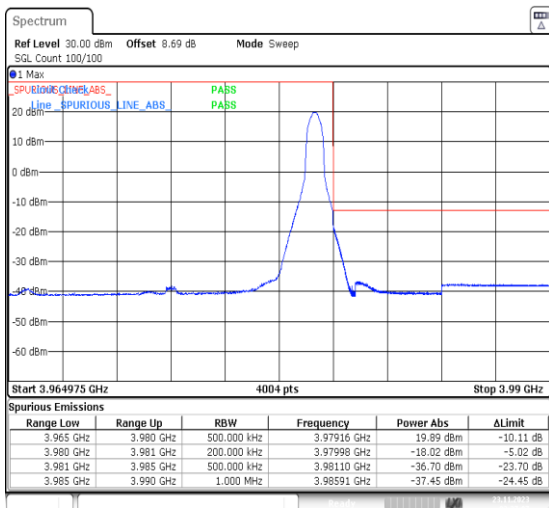
1-N77-3700-3980-PC3-30-15-H-5-CP-QPSK-Edge_1RB_Right-1@37-Ant13-1--PASS-see graph
