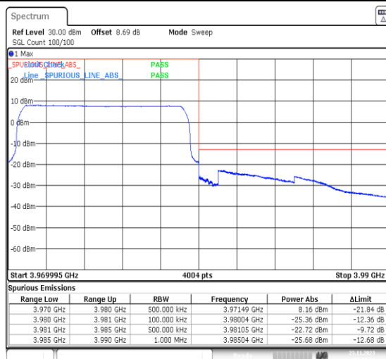
1-N77-3700-3980-PC3-30-10-H-6-CP-QPSK-Outer_Full-24@0-Ant13-1--PASS-see graph
