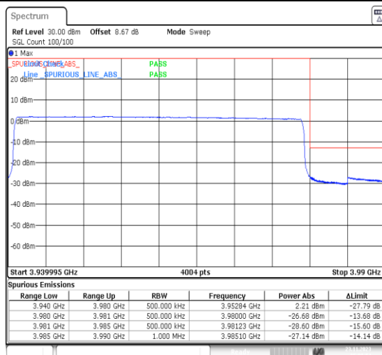
1-N77-3700-3980-PC3-30-40-H-6-CP-QPSK-Outer_Full-106@0-Ant13-1--PASS-see graph
