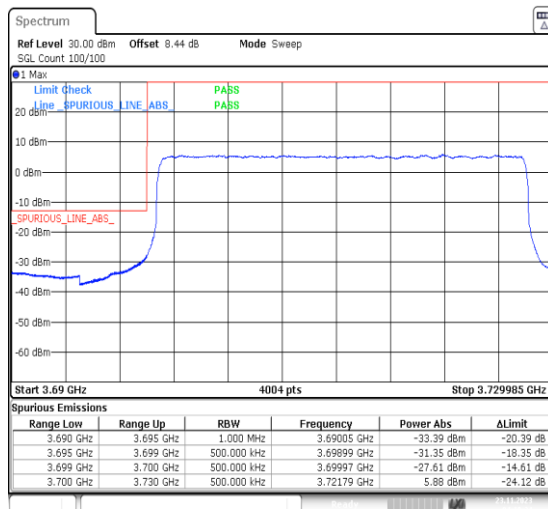
1-N77-3700-3980-PC3-30-30-L-3-DFT-PI2BPSK-Outer_Full-75@0-Ant13-1--PASS-see graph
