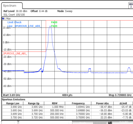
1-N77-3700-3980-PC3-30-20-L-1-DFT-PI2BPSK-Edge_1RB_Left-1@0-Ant13-1--PASS-see graph
