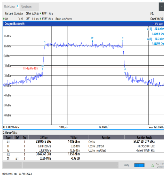
NTNV_N77-3700-3980_PC3_30_60_M_TID8_Ant13#1
