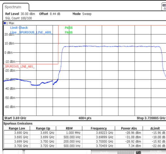
1-N77-3700-3980-PC3-30-20-L-3-DFT-PI2BPSK-Outer_Full-50@0-Ant13-1--PASS-see graph
