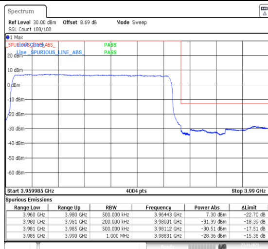
1-N77-3700-3980-PC3-30-20-H-3-DFT-PI2BPSK-Outer_Full-50@0-Ant13-1--PASS-see graph
