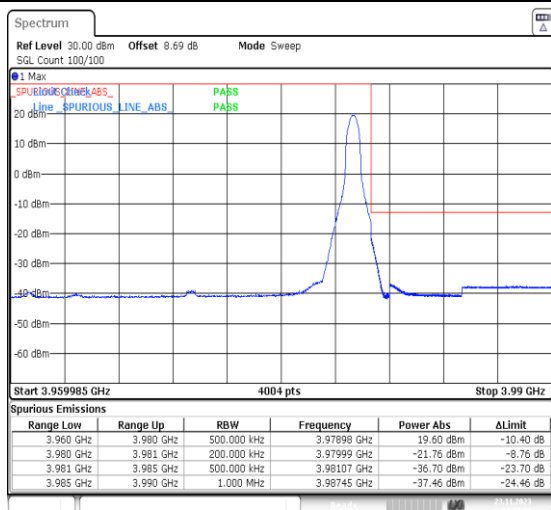
1-N77-3700-3980-PC3-30-20-H-5-CP-QPSK-Edge_1RB_Right-1@50-Ant13-1--PASS-see graph
