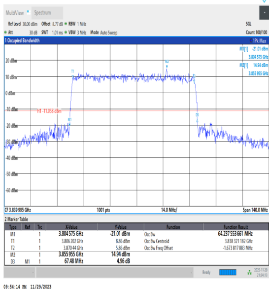
NTNV_N77-3700-3980_PC3_30_70_M_TID4_Ant13#1
