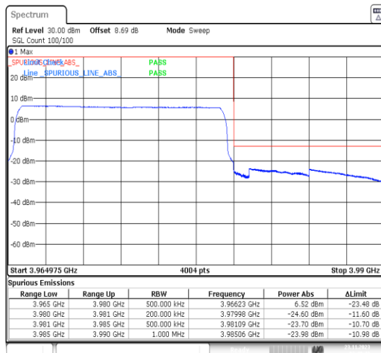
1-N77-3700-3980-PC3-30-15-H-6-CP-QPSK-Outer_Full-38@0-Ant13-1--PASS-see graph
