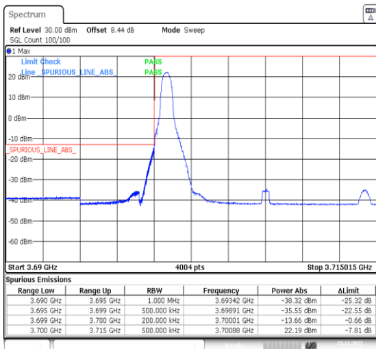
1-N77-3700-3980-PC3-30-15-L-1-DFT-PI2BPSK-Edge_1RB_Left-1@0-Ant13-1--PASS-see graph
