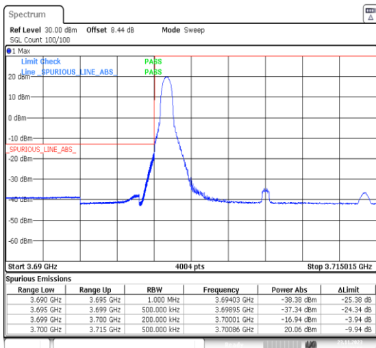
1-N77-3700-3980-PC3-30-15-L-4-CP-QPSK-Edge_1RB_Left-1@0-Ant13-1--PASS-see graph
