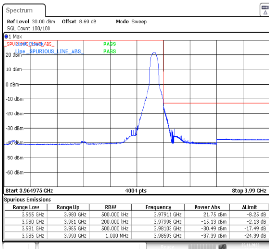
1-N77-3700-3980-PC3-30-15-H-2-DFT-PI2BPSK-Edge_1RB_Right-1@37-Ant13-1--PASS-see graph
