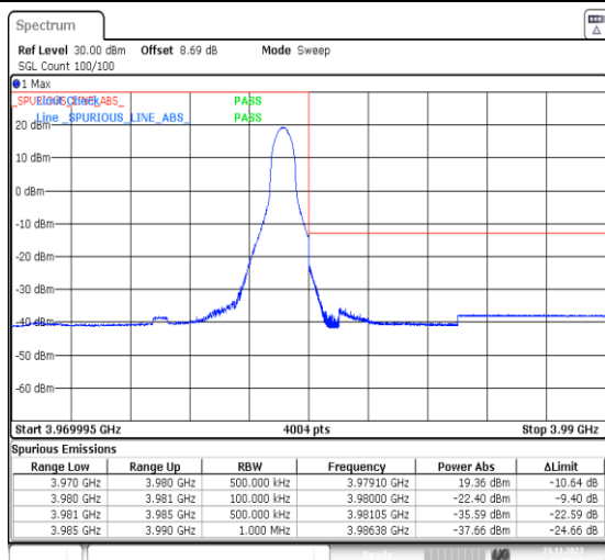
1-N77-3700-3980-PC3-30-10-H-5-CP-QPSK-Edge_1RB_Right-1@23-Ant13-1--PASS-see graph
