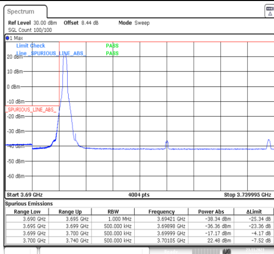
1-N77-3700-3980-PC3-30-40-L-1-DFT-PI2BPSK-Edge_1RB_Left-1@0-Ant13-1--PASS-see graph
