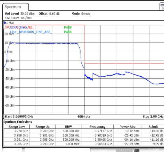
1-N77-3700-3980-PC3-30-10-H-3-DFT-PI2BPSK-Outer_Full-24@0-Ant13-1--PASS-see graph
