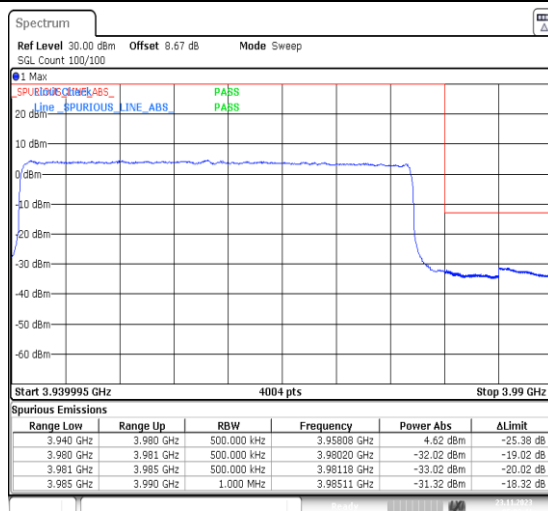
1-N77-3700-3980-PC3-30-40-H-3-DFT-PI2BPSK-Outer_Full-100@0-Ant13-1--PASS-see graph
