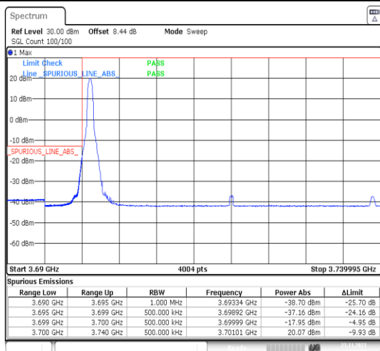
1-N77-3700-3980-PC3-30-40-L-4-CP-QPSK-Edge_1RB_Left-1@0-Ant13-1--PASS-see graph
