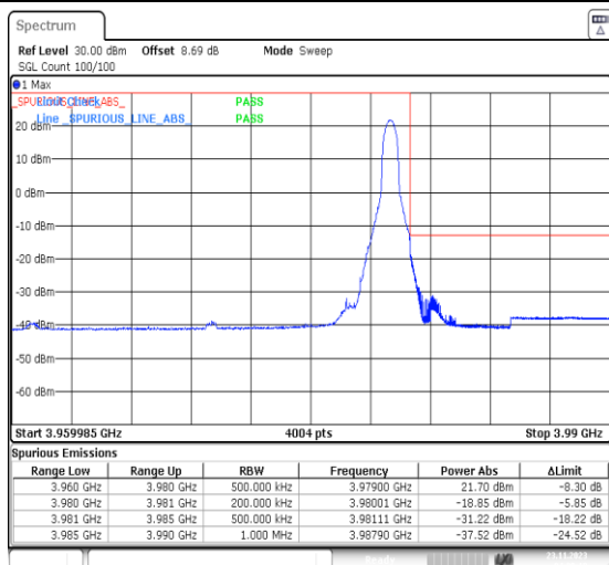
1-N77-3700-3980-PC3-30-20-H-2-DFT-PI2BPSK-Edge_1RB_Right-1@50-Ant13-1--PASS-see graph
