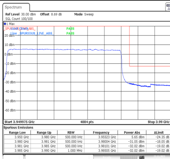
1-N77-3700-3980-PC3-30-30-H-3-DFT-PI2BPSK-Outer_Full-75@0-Ant13-1--PASS-see graph
