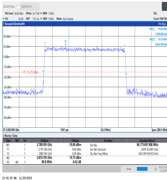
NTVN_N77-3700-3980_PC3_30_100_M_TID5_Ant13#1
