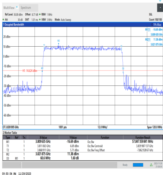
NTNV_N77-3700-3980_PC3_30_60_M_TID9_Ant13#1
