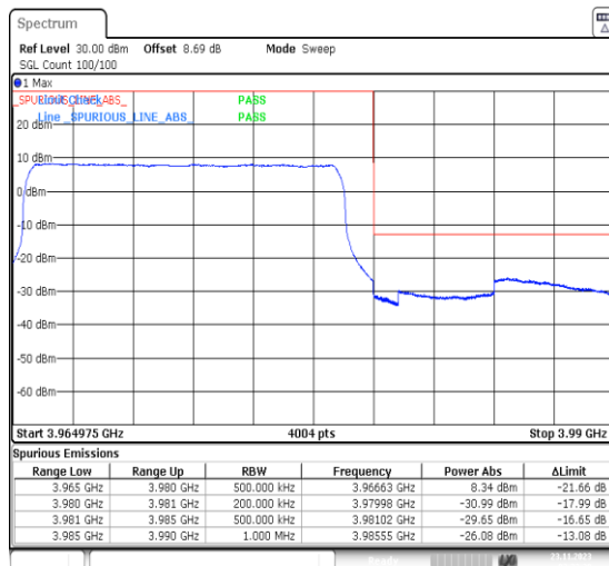
1-N77-3700-3980-PC3-30-15-H-3-DFT-PI2BPSK-Outer_Full-36@0-Ant13-1--PASS-see graph
