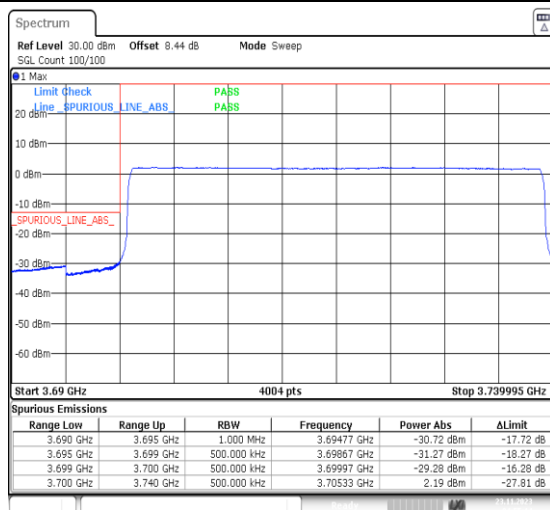
1-N77-3700-3980-PC3-30-40-L-6-CP-QPSK-Outer_Full-106@0-Ant13-1--PASS-see graph
