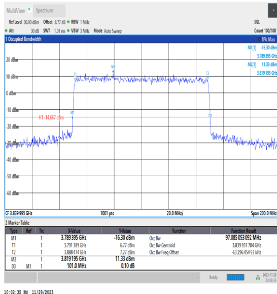
NTVN_N77-3700-3980_PC3_30_100_M_TID8_Ant13#1
