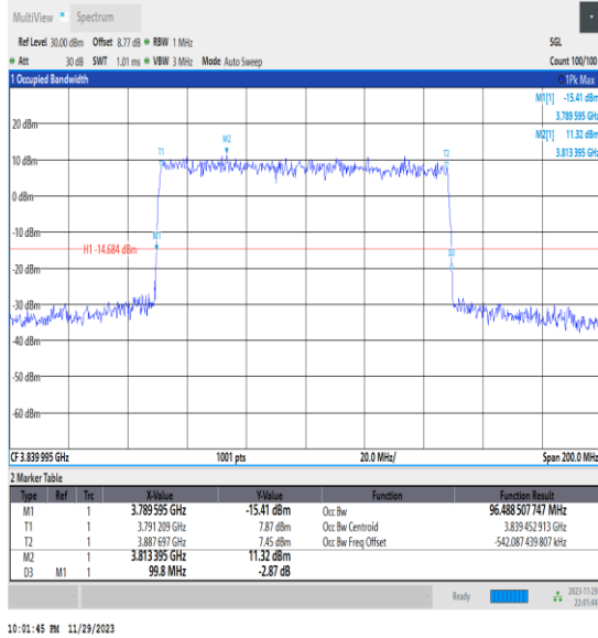
NTVN_N77-3700-3980_PC3_30_100_M_TID3_Ant13#1
