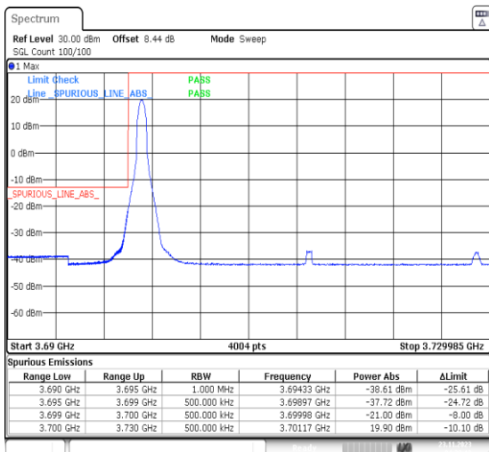
1-N77-3700-3980-PC3-30-30-L-4-CP-QPSK-Edge_1RB_Left-1@0-Ant13-1--PASS-see graph
