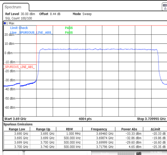
1-N77-3700-3980-PC3-30-40-L-3-DFT-PI2BPSK-Outer_Full-100@0-Ant13-1--PASS-see graph
