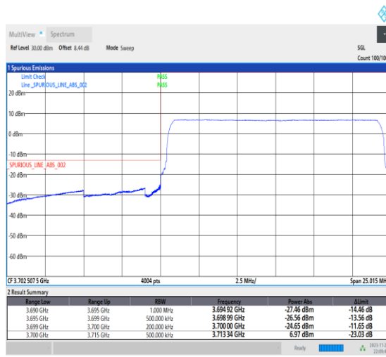
1-N77-3700-3980-PC3-30-15-L-6-CP-QPSK-Outer_Full-38@0-Ant13-1--PASS-see graph
