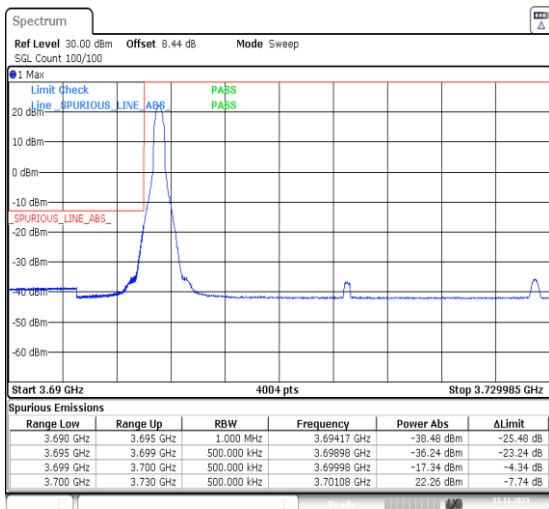
1-N77-3700-3980-PC3-30-30-L-1-DFT-PI2BPSK-Edge_1RB_Left-1@0-Ant13-1--PASS-see graph
