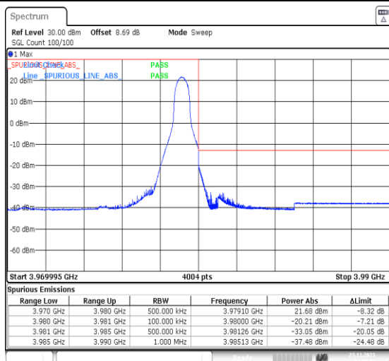
1-N77-3700-3980-PC3-30-10-H-2-DFT-PI2BPSK-Edge_1RB_Right-1@23-Ant13-1--PASS-see graph
