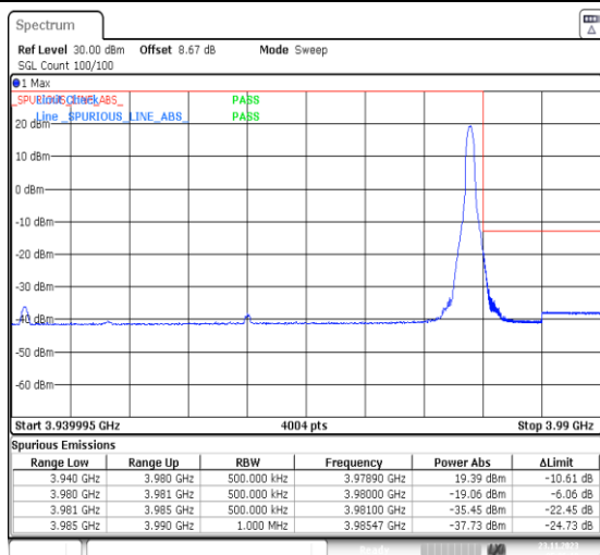
1-N77-3700-3980-PC3-30-40-H-5-CP-QPSK-Edge_1RB_Right-1@105-Ant13-1--PASS-see graph
