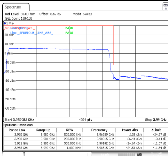
1-N77-3700-3980-PC3-30-20-H-6-CP-QPSK-Outer_Full-51@0-Ant13-1--PASS-see graph
