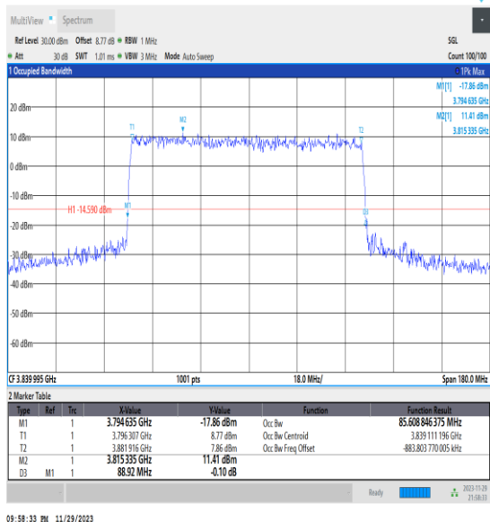
NTNV_N77-3700-3980_PC3_30_90_M_TID4_Ant13#1
