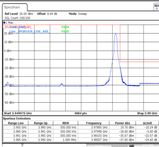
1-N77-3700-3980-PC3-30-30-H-2-DFT-PI2BPSK-Edge_1RB_Right-1@77-Ant13-1--PASS-see graph
