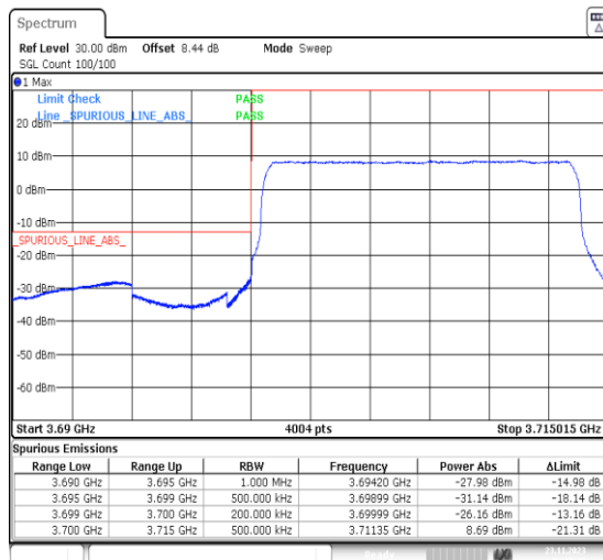
1-N77-3700-3980-PC3-30-15-L-3-DFT-PI2BPSK-Outer_Full-36@0-Ant13-1--PASS-see graph
