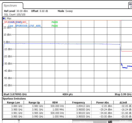
1-N77-3700-3980-PC3-30-100-H-6-CP-QPSK-Outer_Full-273@0-Ant13-1--PASS-see graph
