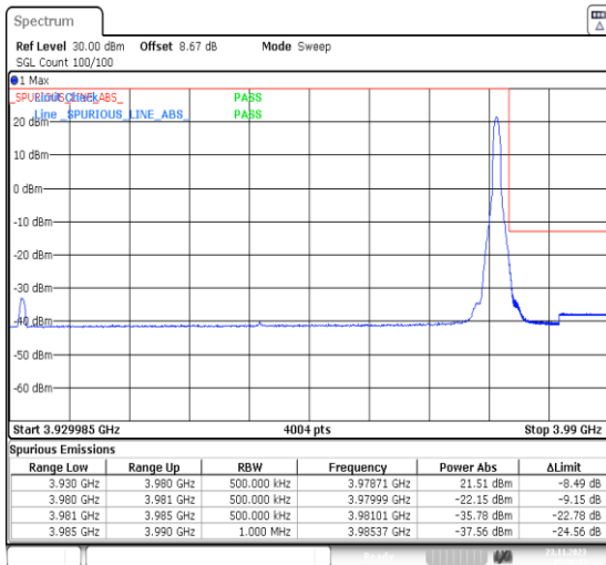
1-N77-3700-3980-PC3-30-50-H-2-DFT-PI2BPSK-Edge_1RB_Right-1@132-Ant13-1--PASS-see graph
