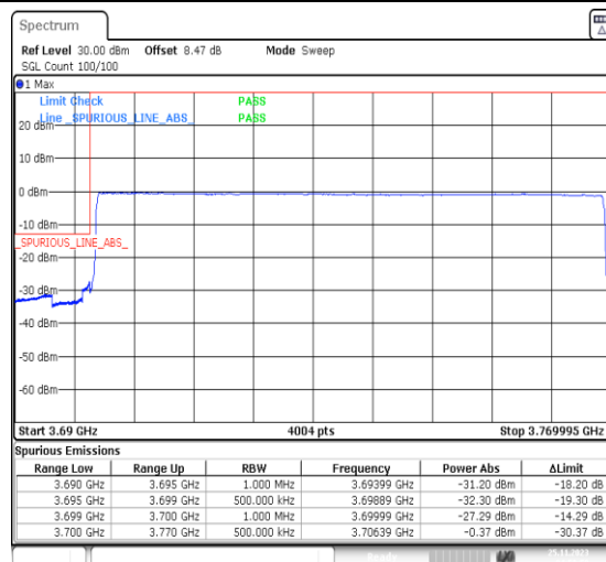
1-N77-3700-3980-PC3-30-70-L-6-CP-QPSK-Outer_Full-189@0-Ant13-1--PASS-see graph
