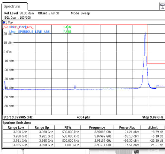
1-N77-3700-3980-PC3-30-80-H-2-DFT-PI2BPSK-Edge_1RB_Right-1@216-Ant13-1--PASS-see graph
