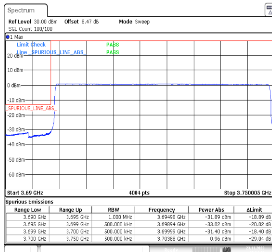
1-N77-3700-3980-PC3-30-50-L-6-CP-QPSK-Outer_Full-133@0-Ant13-1--PASS-see graph
