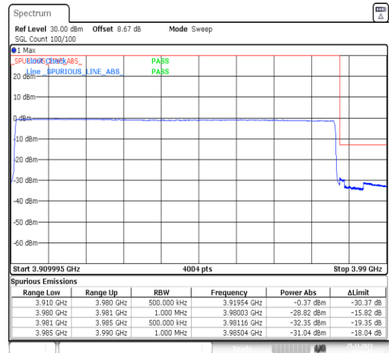
1-N77-3700-3980-PC3-30-70-H-3-DFT-PI2BPSK-Outer_Full-180@0-Ant13-1--PASS-see graph
