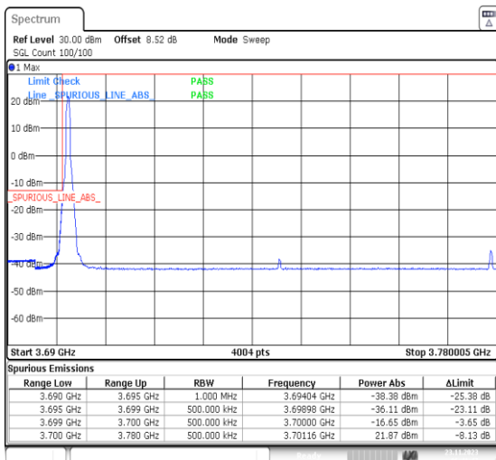
1-N77-3700-3980-PC3-30-80-L-1-DFT-PI2BPSK-Edge_1RB_Left-1@0-Ant13-1--PASS-see graph
