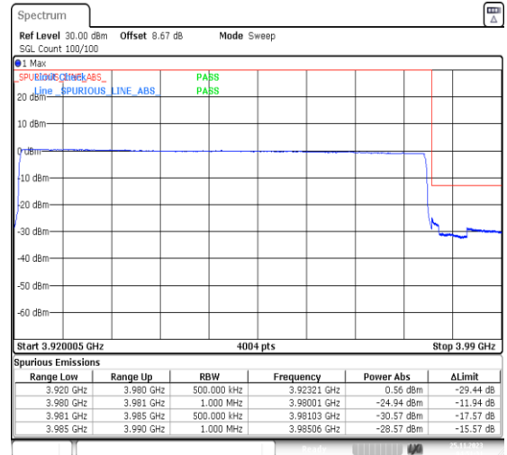
1-N77-3700-3980-PC3-30-60-H-6-CP-QPSK-Outer_Full-162@0-Ant13-1--PASS-see graph
