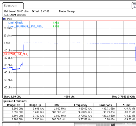
1-N77-3700-3980-PC3-30-60-L-6-CP-QPSK-Outer_Full-162@0-Ant13-1--PASS-see graph
