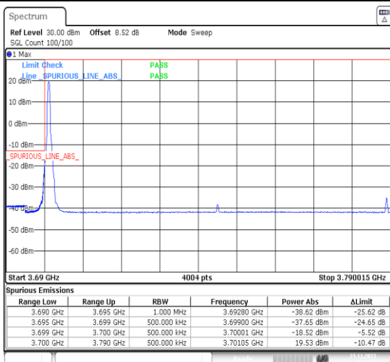
1-N77-3700-3980-PC3-30-90-L-1-DFT-PI2BPSK-Edge_1RB_Left-1@0-Ant13-1--PASS-see graph
