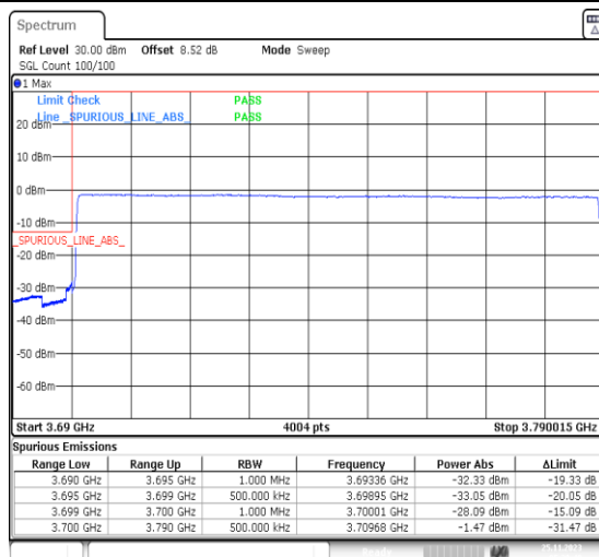
1-N77-3700-3980-PC3-30-90-L-3-DFT-PI2BPSK-Outer_Full-240@0-Ant13-1--PASS-see graph
