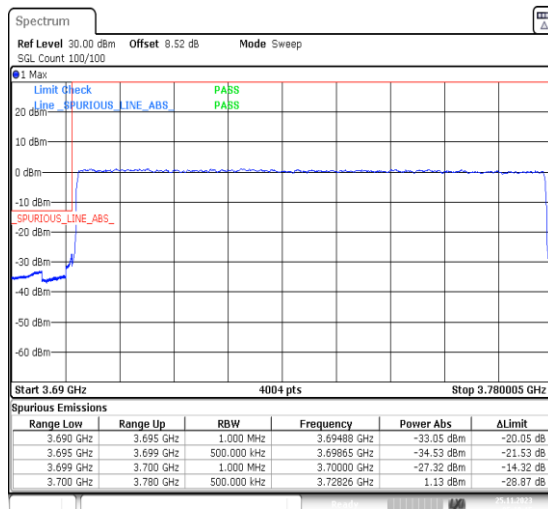
1-N77-3700-3980-PC3-30-80-L-3-DFT-PI2BPSK-Outer_Full-216@0-Ant13-1--PASS-see graph
