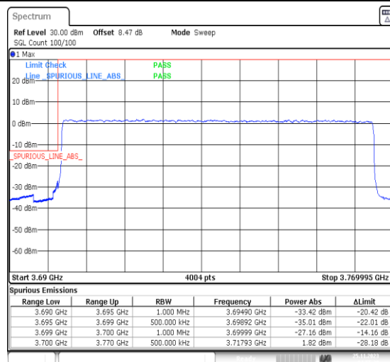
1-N77-3700-3980-PC3-30-70-L-3-DFT-PI2BPSK-Outer_Full-180@0-Ant13-1--PASS-see graph
