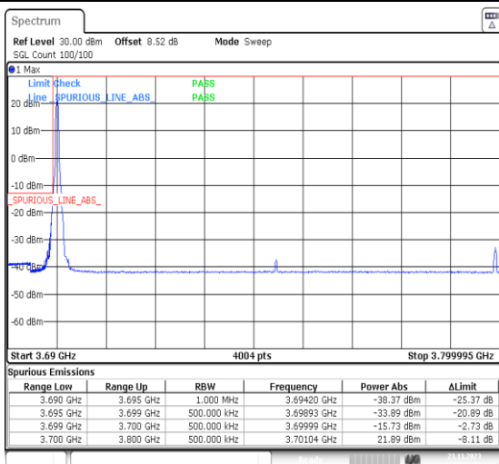
1-N77-3700-3980-PC3-30-100-L-1-DFT-P12BPSK-Edge_1RB_Left-1@0-Ant13-1--PASS-see graph
