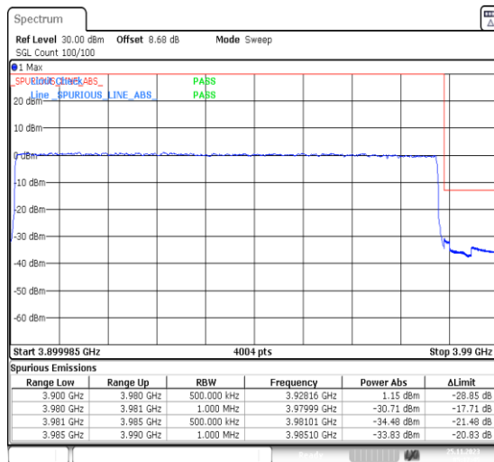
1-N77-3700-3980-PC3-30-80-H-3-DFT-PI2BPSK-Outer_Full-216@0-Ant13-1--PASS-see graph
