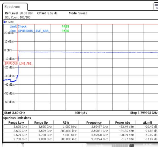
1-N77-3700-3980-PC3-30-100-L-6-CP-QPSK-Outer_Full-273@0-Ant13-1--PASS-see graph
