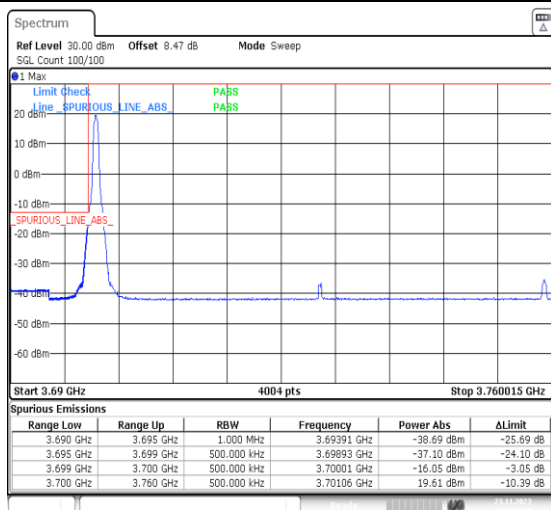
1-N77-3700-3980-PC3-30-60-L-4-CP-QPSK-Edge_1RB_Left-1@0-Ant13-1--PASS-see graph
