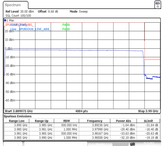
1-N77-3700-3980-PC3-30-90-H-6-CP-QPSK-Outer_Full-245@0-Ant13-1--PASS-see graph
