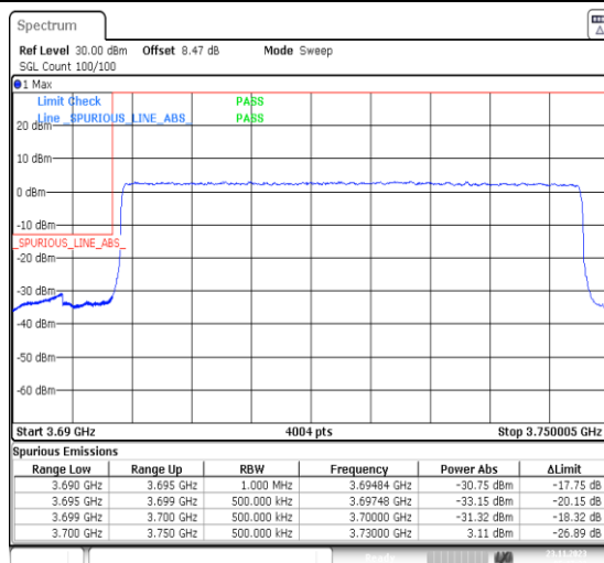
1-N77-3700-3980-PC3-30-50-L-3-DFT-PI2BPSK-Outer_Full-128@0-Ant13-1--PASS-see graph
