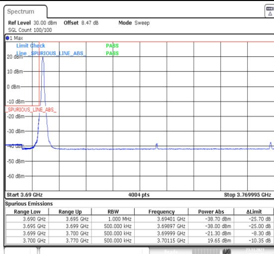
1-N77-3700-3980-PC3-30-70-L-4-CP-QPSK-Edge_1RB_Left-1@0-Ant13-1--PASS-see graph
