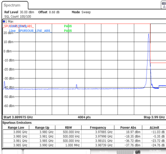
1-N77-3700-3980-PC3-30-90-H-5-CP-QPSK-Edge_1RB_Right-1@244-Ant13-1--PASS-see graph
