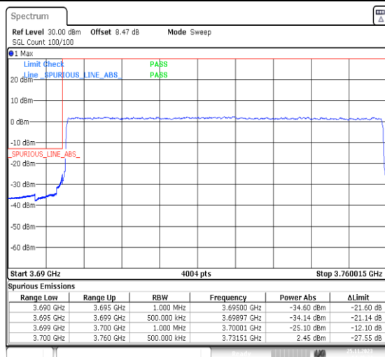
1-N77-3700-3980-PC3-30-60-L-3-DFT-PI2BPSK-Outer_Full-162@0-Ant13-1--PASS-see graph
