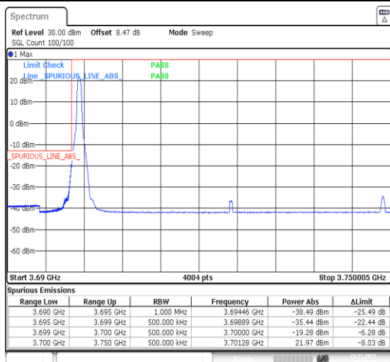
1-N77-3700-3980-PC3-30-50-L-1-DFT-PI2BPSK-Edge_1RB_Left-1@0-Ant13-1--PASS-see graph
