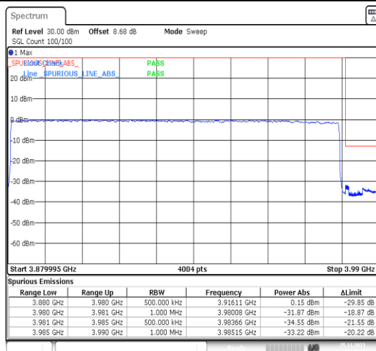
1-N77-3700-3980-PC3-30-100-H-3-DFT-PI2BPSK-Outer_Full-270@0-Ant13-1--PASS-see graph
