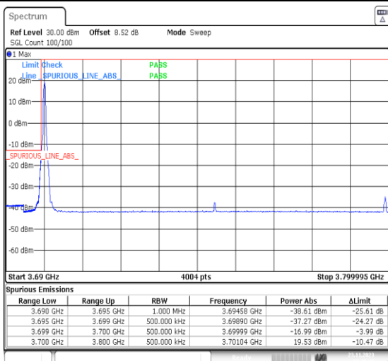
1-N77-3700-3980-PC3-30-100-L-4-CP-QPSK-Edge_1RB_Left-1@0-Ant13-1--PASS-see graph
