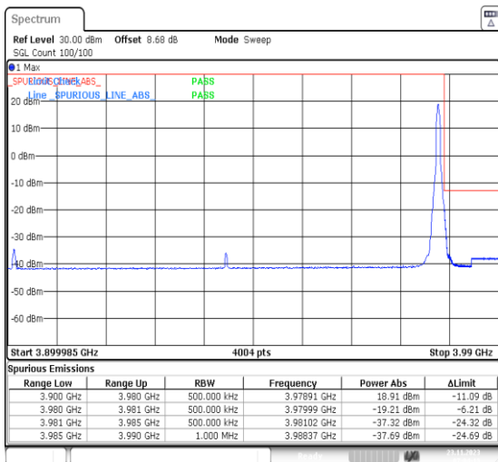
1-N77-3700-3980-PC3-30-80-H-5-CP-QPSK-Edge_1RB_Right-1@216-Ant13-1--PASS-see graph
