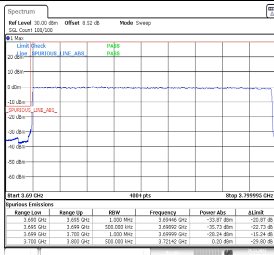
1-N77-3700-3980-PC3-30-100-L-3-DFT-P12BPSK-Outer_Full-270@0-Ant13-1--PASS-see graph
