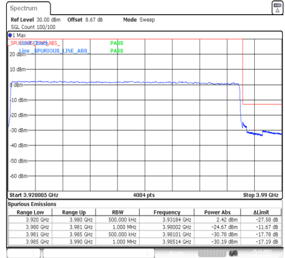
1-N77-3700-3980-PC3-30-60-H-3-DFT-PI2BPSK-Outer_Full-162@0-Ant13-1--PASS-see graph
