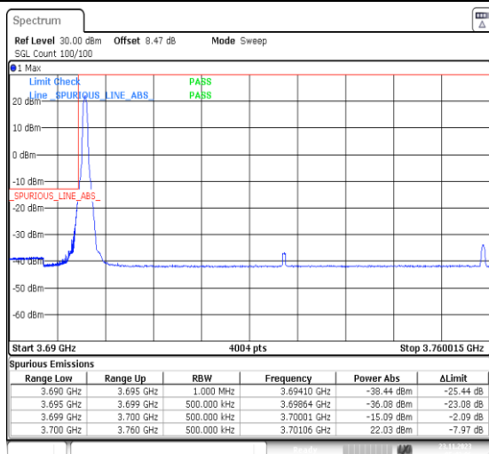
1-N77-3700-3980-PC3-30-60-L-1-DFT-PI2BPSK-Edge_1RB_Left-1@0-Ant13-1--PASS-see graph
