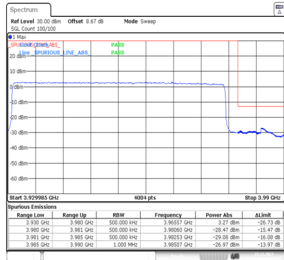
1-N77-3700-3980-PC3-30-50-H-3-DFT-PI2BPSK-Outer_Full-128@0-Ant13-1--PASS-see graph
