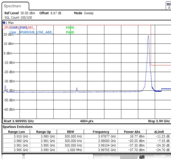
1-N77-3700-3980-PC3-30-70-H-2-DFT-PI2BPSK-Edge_1RB_Right-1@188-Ant13-1--PASS-see graph
