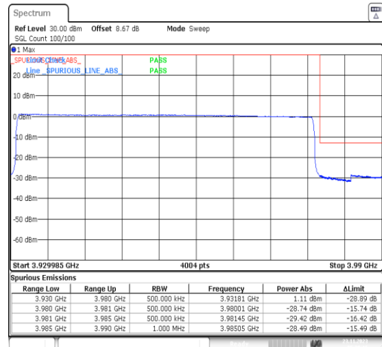
1-N77-3700-3980-PC3-30-50-H-6-CP-QPSK-Outer_Full-133@0-Ant13-1--PASS-see graph
