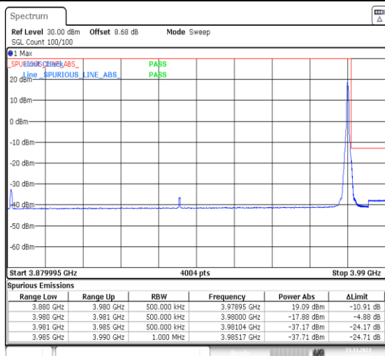
1-N77-3700-3980-PC3-30-100-H-5-CP-QPSK-Edge_1RB_Right-1@272-Ant13-1--PASS-see graph
