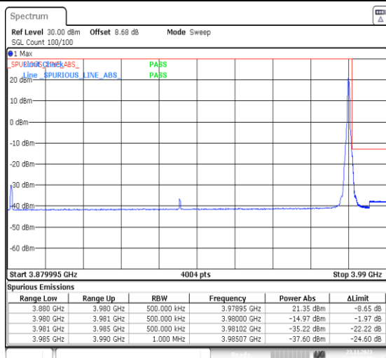
1-N77-3700-3980-PC3-30-100-H-2-DFT-PI2BPSK-Edge_1RB_Right-1@272-Ant13-1--PASS-see graph
