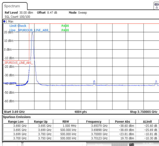
1-N77-3700-3980-PC3-30-50-L-4-CP-QPSK-Edge_1RB_Left-1@0-Ant13-1--PASS-see graph
