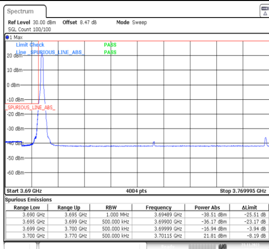
1-N77-3700-3980-PC3-30-70-L-1-DFT-PI2BPSK-Edge_1RB_Left-1@0-Ant13-1--PASS-see graph
