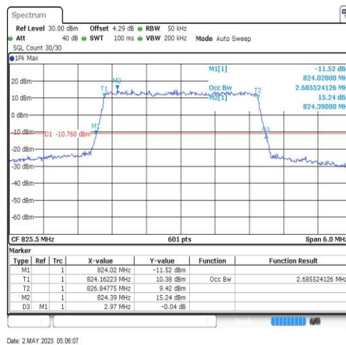
Band26-3MHz-64QAM-26805-15RB#0-2.686
