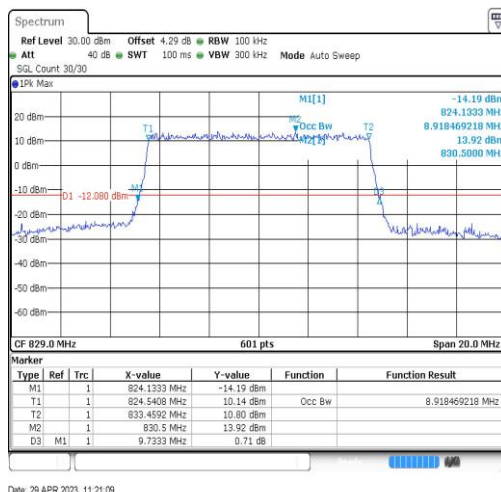
Band26-10MHz-16QAM-26840-50RB#0-8.918
