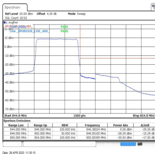
Band26-3MHz-QPSK-27025-15RB#0
