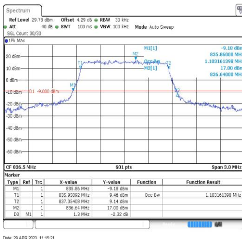
Band26-1.4MHz-16QAM-26915-6RB#0-1.103
