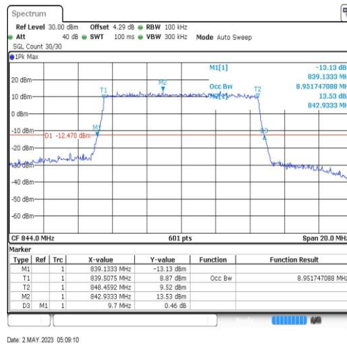
Band26-10MHz-64QAM-26990-50RB#0-8.952
