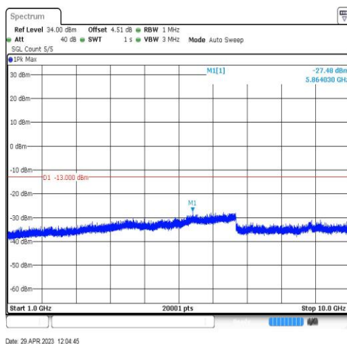
Band26-15MHz-QPSK-26965-1RB#0-Range4:1000~10000MHz
