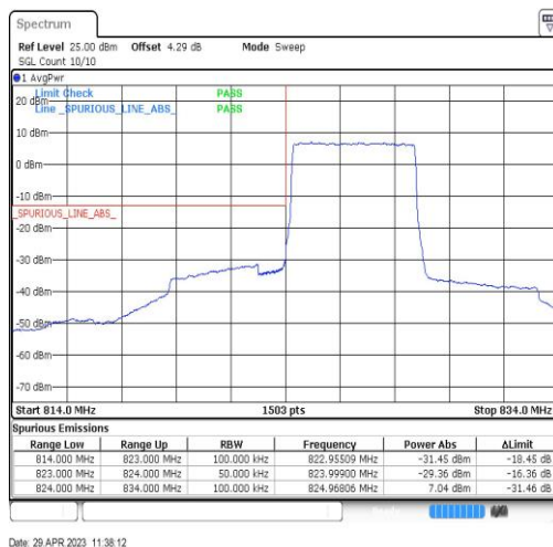
Band26-5MHz-QPSK-26815-25RB#0
