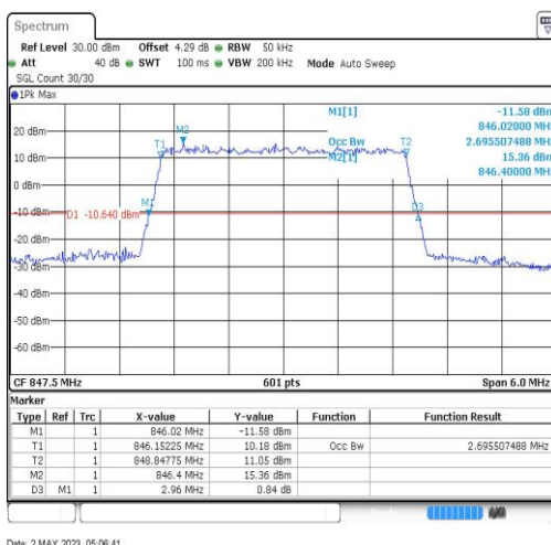
Band26-3MHz-64QAM-27025-15RB#0-2.696
