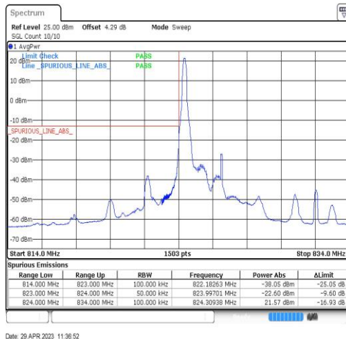
Band26-5MHz-QPSK-26815-1RB#0
