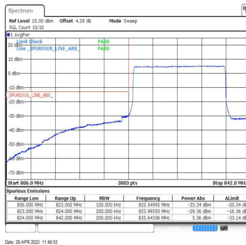
Band26-15MHz-QPSK-26865-75RB#0
