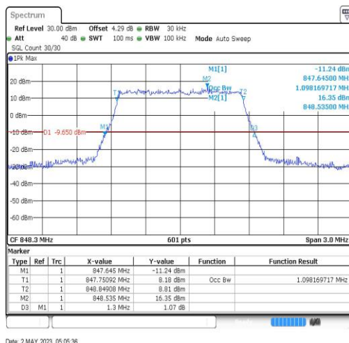
Band26-1.4MHz-64QAM-27033-6RB#0-1.098
