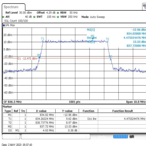
Band26-5MHz-64QAM-26915-25RB#0-4.476
