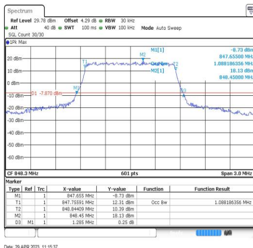
Band26-1.4MHz-QPSK-27033-6RB#0-1.088
