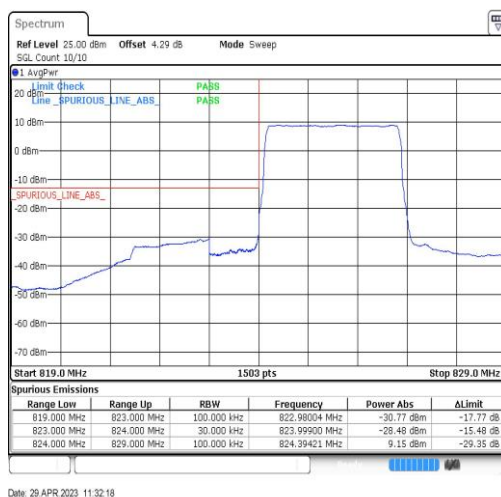
Band26-3MHz-QPSK-26805-15RB#0
