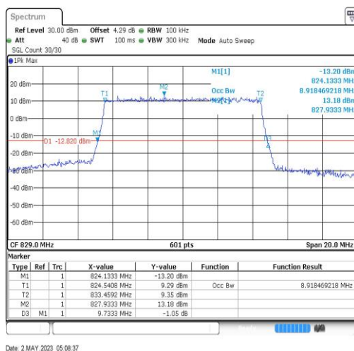
Band26-10MHz-64QAM-26840-50RB#0-8.918
