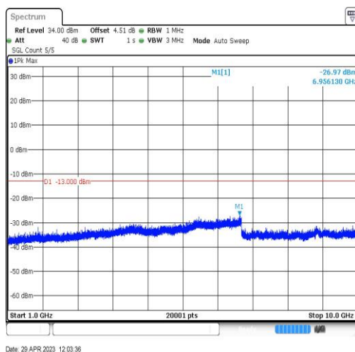
Band26-15MHz-QPSK-26865-1RB#0-Range4:1000~10000MHz
