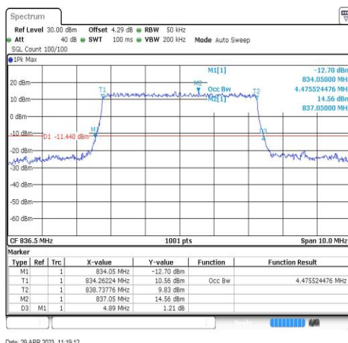
Band26-5MHz-QPSK-26915-25RB#0-4.476
