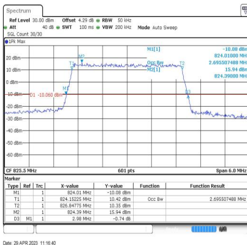
Band26-3MHz-16QAM-26805-15RB#0-2.696
