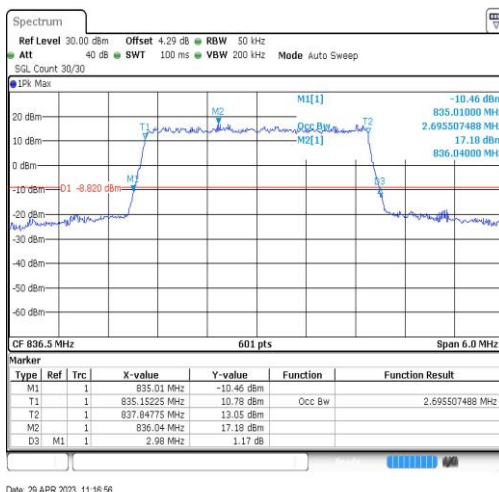
Band26-3MHz-QPSK-26915-15RB#0-2.696
