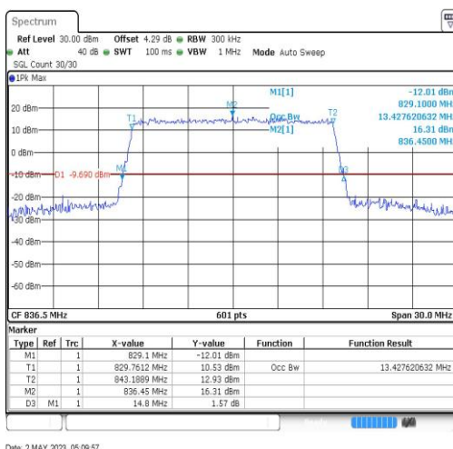
Band26-15MHz-64QAM-26915-75RB#0-13.428
