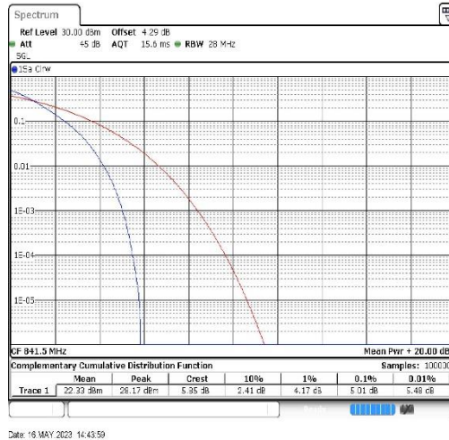
Band26-15MHz-QPSK-26965-75RB#0
