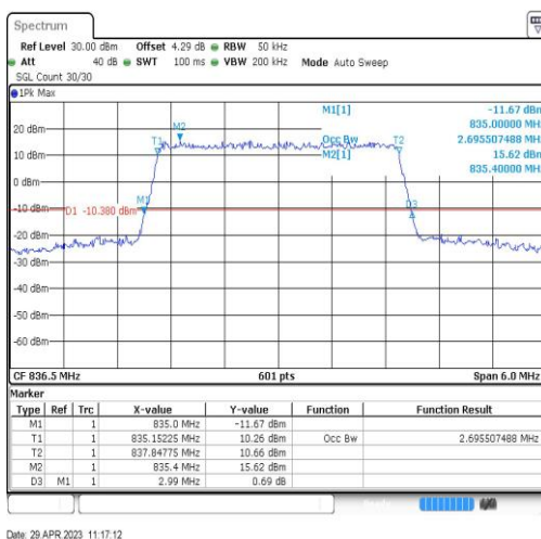
Band26-3MHz-16QAM-26915-15RB#0-2.696
