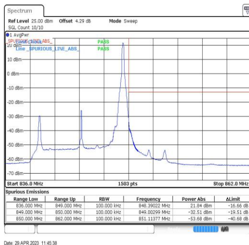
Band26-10MHz-QPSK-26990-1RB#49
