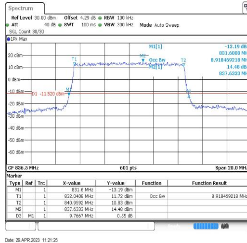
Band26-10MHz-QPSK-26915-50RB#0-8.918
