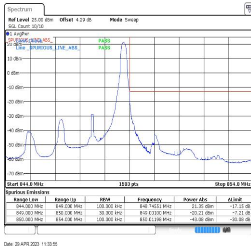
Band26-3MHz-QPSK-27025-1RB#14
