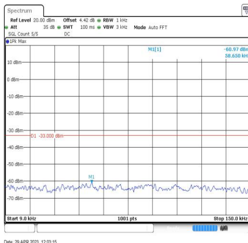
Band26-15MHz-QPSK-26865-1RB#0-Range1:0.009~0.15MHz
