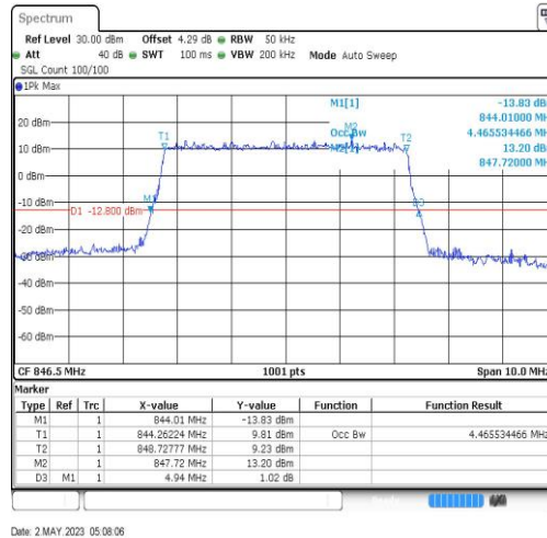
Band26-5MHz-64QAM-27015-25RB#0-4.466
