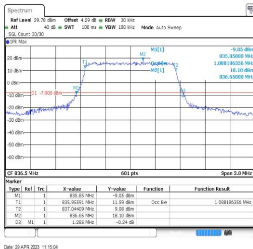
Band26-1.4MHz-QPSK-26915-6RB#0-1.088
