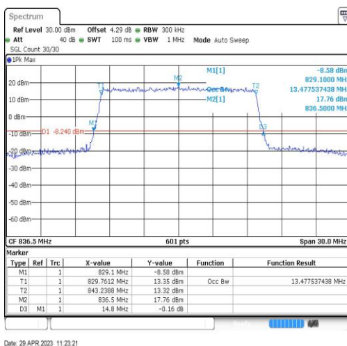
Band26-15MHz-QPSK-26915-75RB#0-13.478
