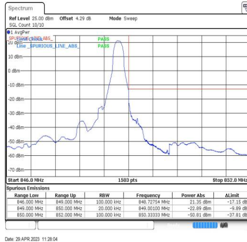
Band26-1.4MHz-QPSK-27033-1RB#5
