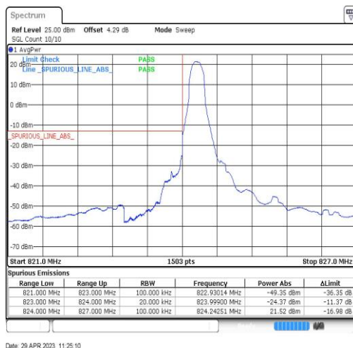
Band26-1.4MHz-QPSK-26797-1RB#0
