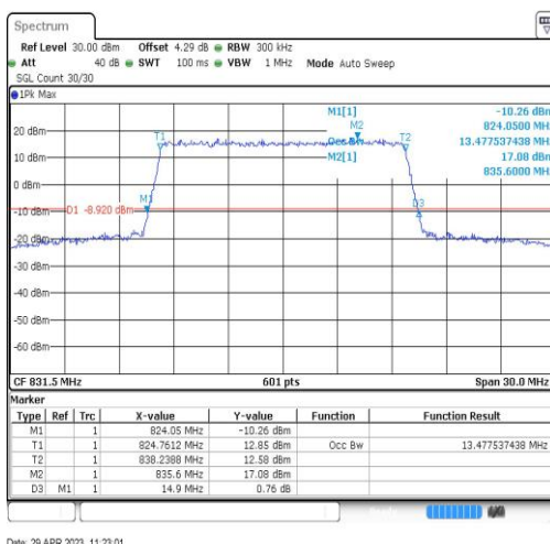
Band26-15MHz-16QAM-26865-75RB#0-13.478
