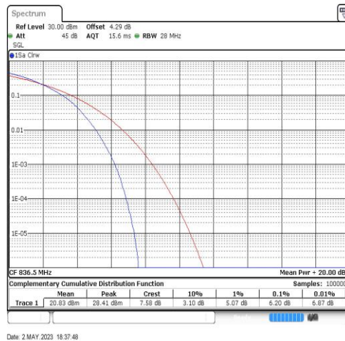
Band26-15MHz-64QAM-26915-75RB#0
