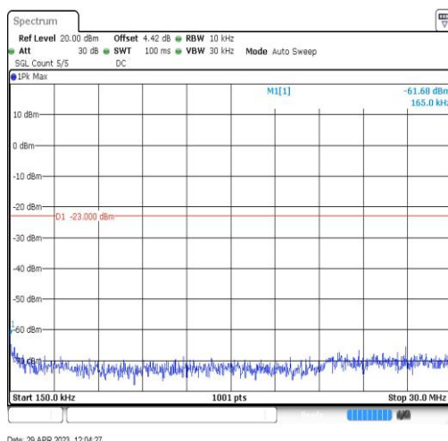
Band26-15MHz-QPSK-26965-1RB#0-Range2:0.15~30MHz
