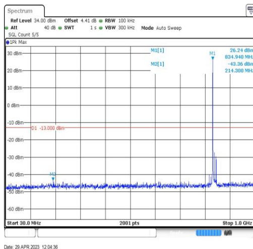
Band26-15MHz-QPSK-26965-1RB#0-Range3:30~1000MHz
