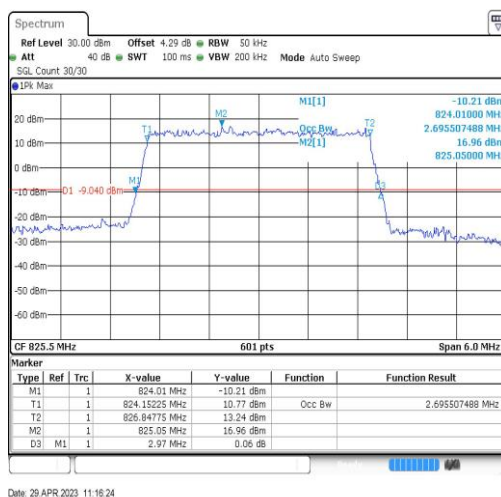
Band26-3MHz-QPSK-26805-15RB#0-2.696
