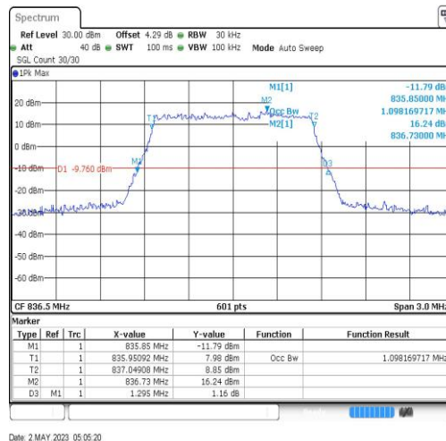
Band26-1.4MHz-64QAM-26915-6RB#0-1.098
