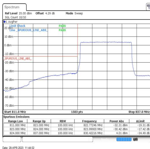
Band26-10MHz-QPSK-26840-50RB#0
