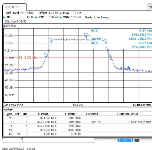
Band26-1.4MHz-16QAM-26797-6RB#0-1.093
