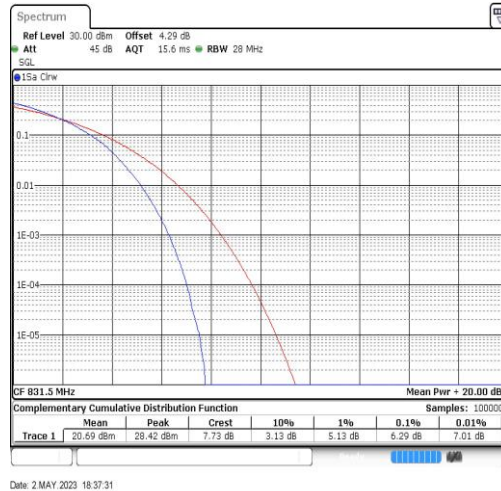
Band26-15MHz-64QAM-26865-75RB#0
