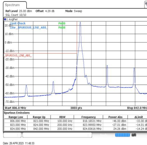
Band26-15MHz-QPSK-26865-1RB#0
