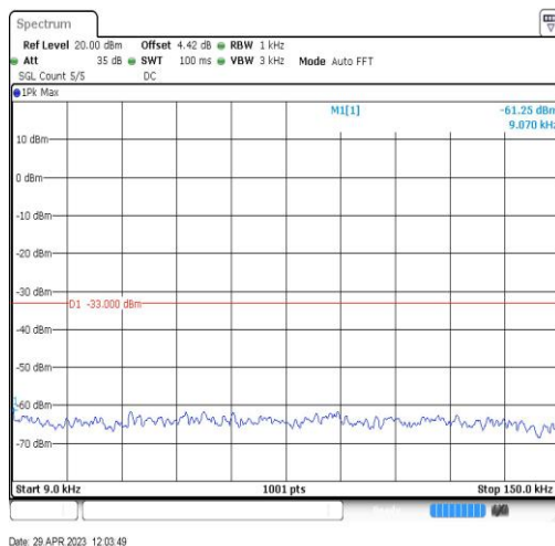
Band26-15MHz-QPSK-26915-1RB#0-Range1:0.009~0.15MHz
