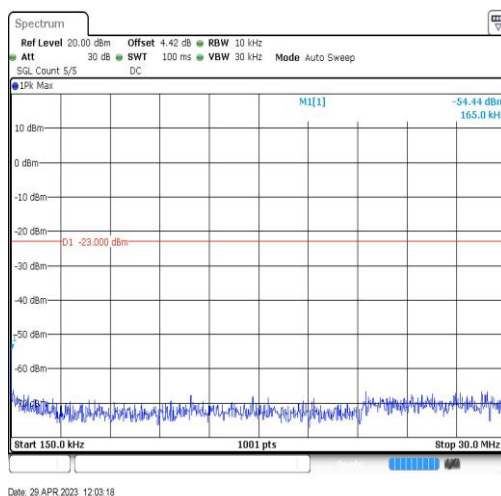
Band26-15MHz-QPSK-26865-1RB#0-Range2:0.15~30MHz
