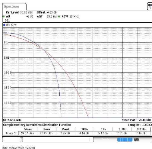
Band41-20MHz-QPSK-40620-100RB#0
