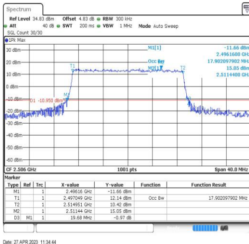
Band41-20MHz-16QAM-39750-100RB#0-17.902
