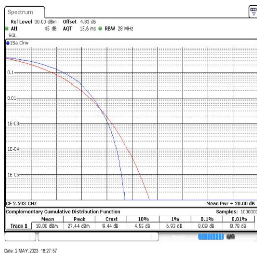
Band41-20MHz-64QAM-40620-100RB#0
