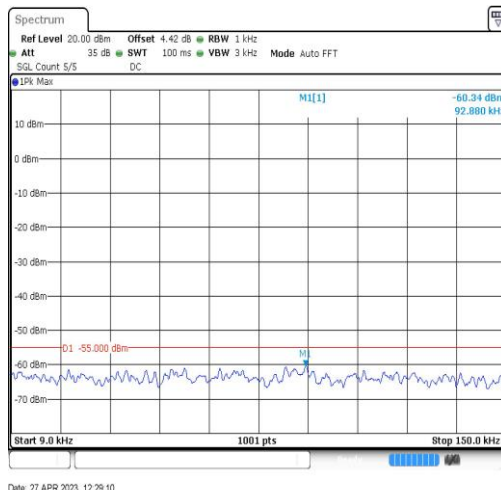
Band41-20MHz-QPSK-39750-1RB#0-Range1:0.009~0.15MHz
