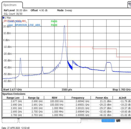
Band41-10MHz-QPSK-41540-1RB#49
