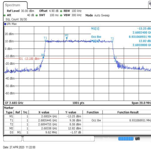
Band41-10MHz-16QAM-41540-50RB#0-8.931
