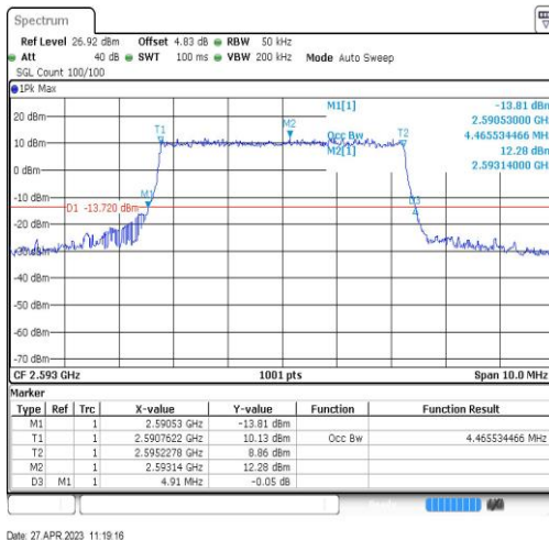
Band41-5MHz-16QAM-40620-25RB#0-4.466
