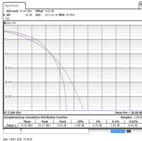
Band41-20MHz-16QAM-39750-100RB#0
