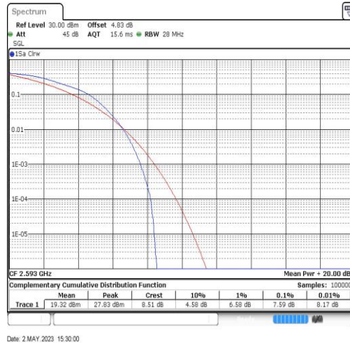
Band41-20MHz-16QAM-40620-100RB#0
