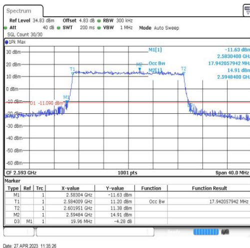
Band41-20MHz-16QAM-40620-100RB#0-17.942
