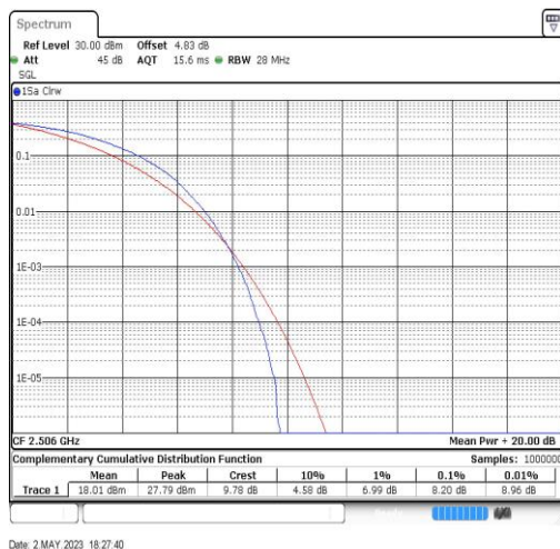
Band41-20MHz-64QAM-39750-100RB#0
