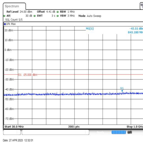
Band41-20MHz-QPSK-40620-1RB#0-Range3:30~1000MHz
