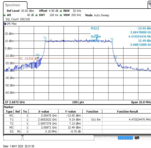
Band41-5MHz-64QAM-41565-25RB#0-4.476
