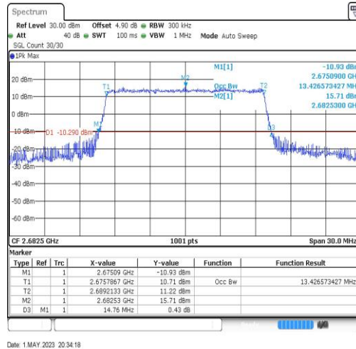
Band41-15MHz-64QAM-41515-75RB#0-13.427
