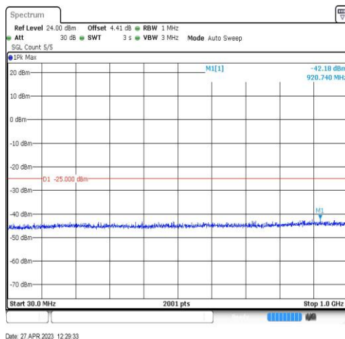
Band41-20MHz-QPSK-39750-1RB#0-Range3:30~1000MHz
