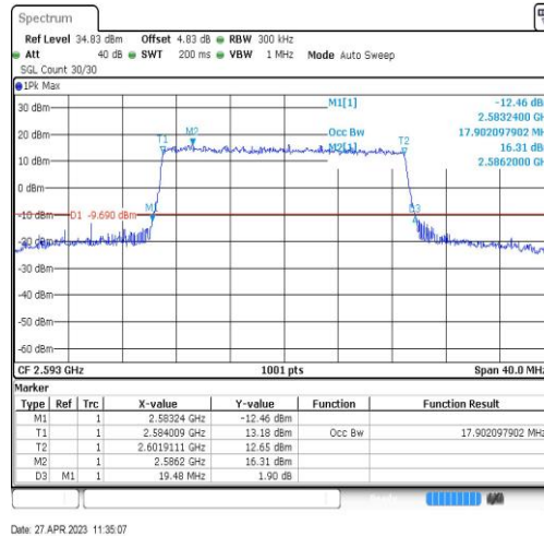
Band41-20MHz-QPSK-40620-100RB#0-17.902
