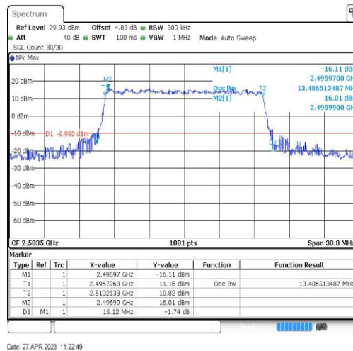
Band41-15MHz-16QAM-39725-75RB#0-13.487
