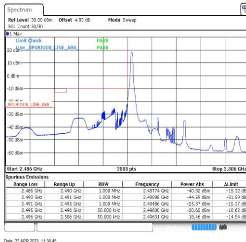
Band41-5MHz-QPSK-39675-1RB#0
