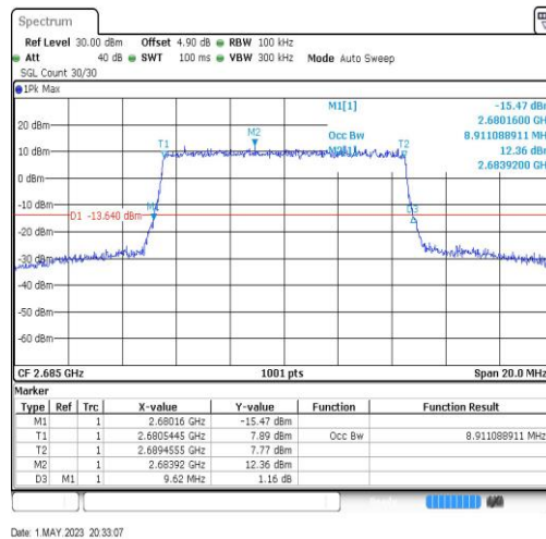
Band41-10MHz-64QAM-41540-50RB#0-8.911
