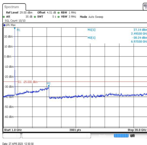
Band41-20MHz-QPSK-39750-1RB#0-Range4:1000~20000MHz
