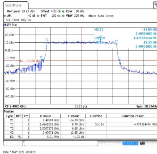
Band41-5MHz-64QAM-39675-25RB#0-4.476
