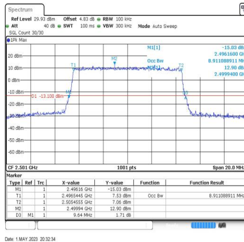
Band41-10MHz-64QAM-39700-50RB#0-8.911
