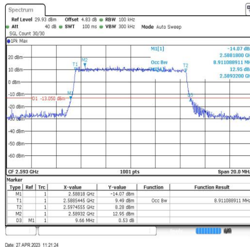
Band41-10MHz-16QAM-40620-50RB#0-8.911
