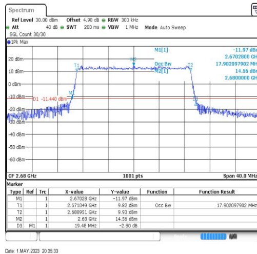
Band41-20MHz-64QAM-41490-100RB#0-17.902
