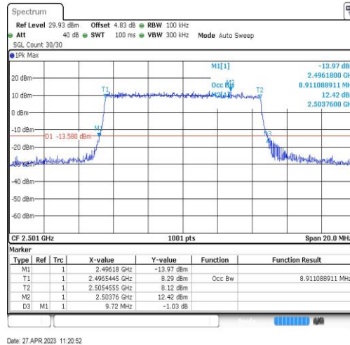
Band41-10MHz-16QAM-39700-50RB#0-8.911
