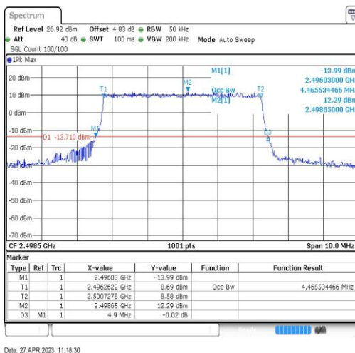
Band41-5MHz-16QAM-39675-25RB#0-4.466
