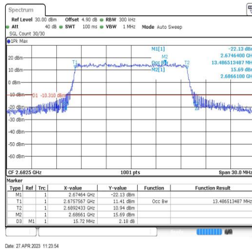
Band41-15MHz-16QAM-41515-75RB#0-13.487
