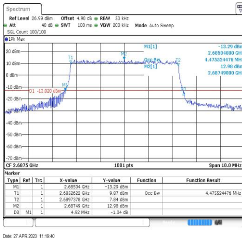
Band41-5MHz-QPSK-41565-25RB#0-4.476
