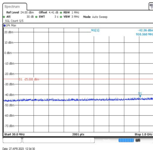
Band41-20MHz-QPSK-41490-1RB#0-Range3:30~1000MHz
