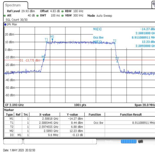
Band41-10MHz-64QAM-40620-50RB#0-8.911
