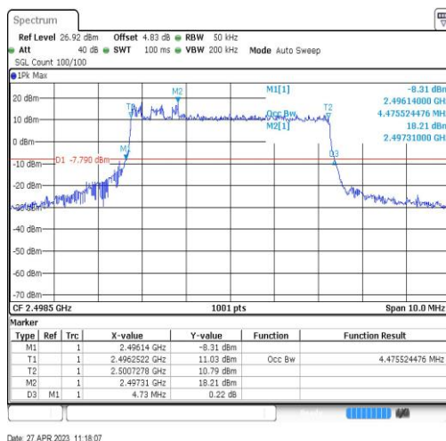
Band41-5MHz-QPSK-39675-25RB#0-4.476
