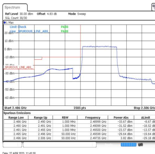
Band41-5MHz-QPSK-39675-25RB#0
