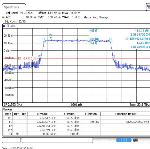
Band41-15MHz-64QAM-40620-75RB#0-13.457
