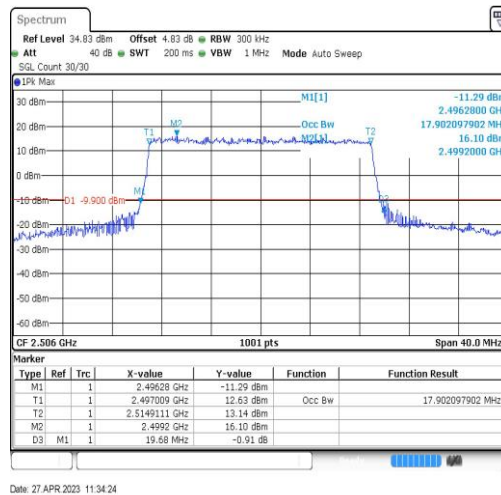
Band41-20MHz-QPSK-39750-100RB#0-17.902
