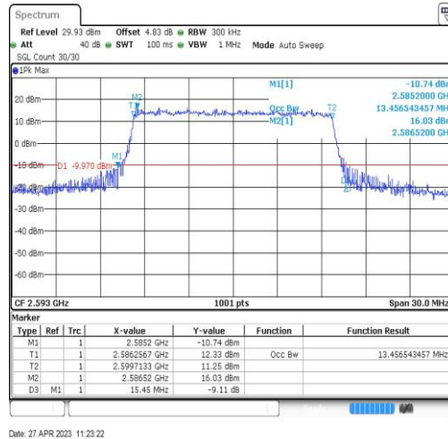
Band41-15MHz-16QAM-40620-75RB#0-13.457
