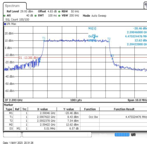
Band41-5MHz-64QAM-40620-25RB#0-4.476
