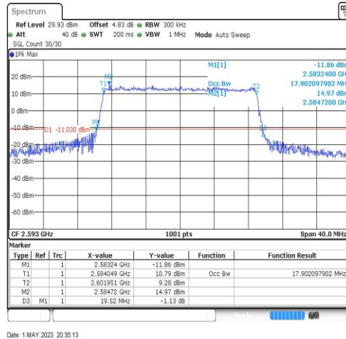
Band41-20MHz-64QAM-40620-100RB#0-17.902
