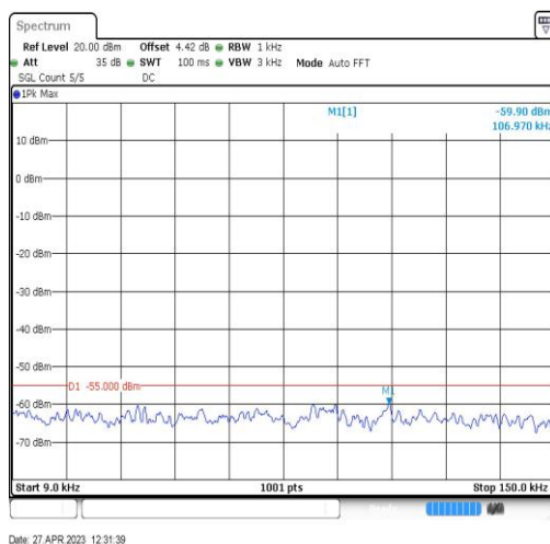
Band41-20MHz-QPSK-40620-1RB#0-Range1:0.009~0.15MHz
