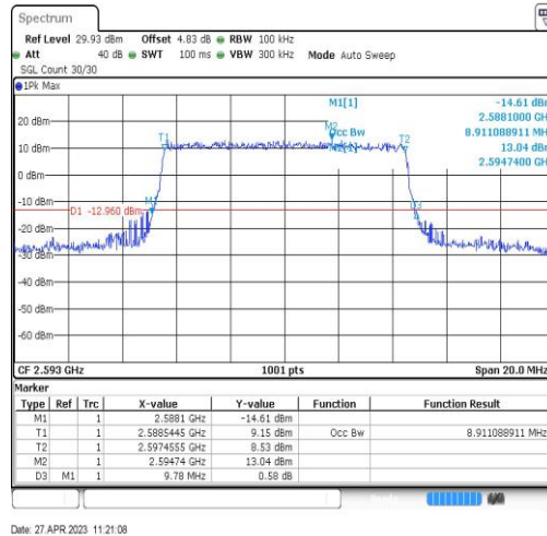
Band41-10MHz-QPSK-40620-50RB#0-8.911
