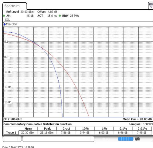
Band41-20MHz-QPSK-39750-100RB#0
