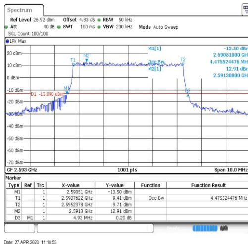
Band41-5MHz-QPSK-40620-25RB#0-4.476
