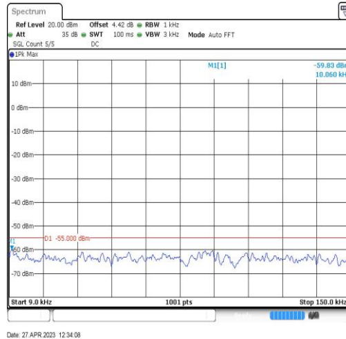
Band41-20MHz-QPSK-41490-1RB#0-Range1:0.009~0.15MHz
