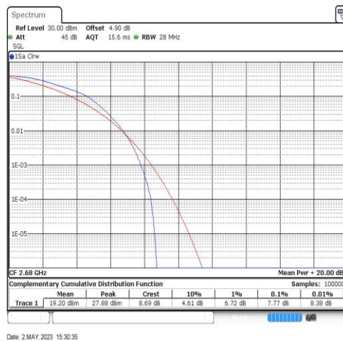
Band41-20MHz-16QAM-41490-100RB#0
