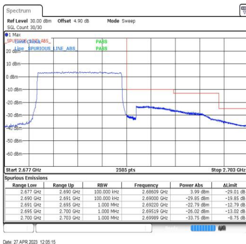
Band41-10MHz-QPSK-41540-50RB#0
