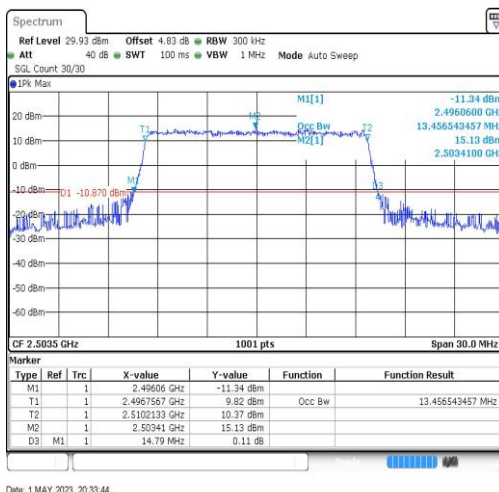
Band41-15MHz-64QAM-39725-75RB#0-13.457
