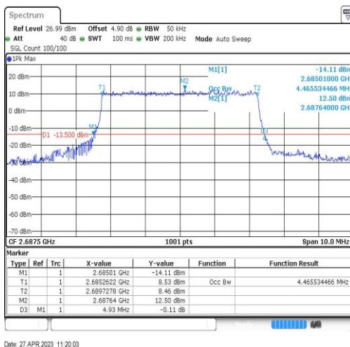
Band41-5MHz-16QAM-41565-25RB#0-4.466
