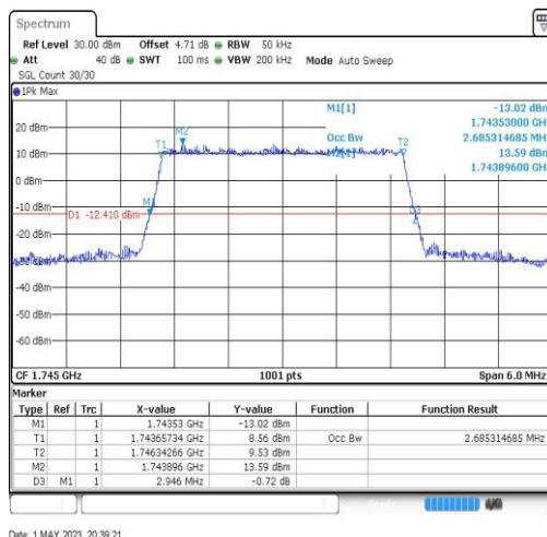
Band66-3MHz-64QAM-132322-15RB#0-2.685
