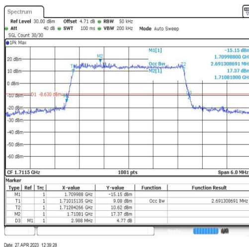
Band66-3MHz-QPSK-131987-15RB#0-2.691
