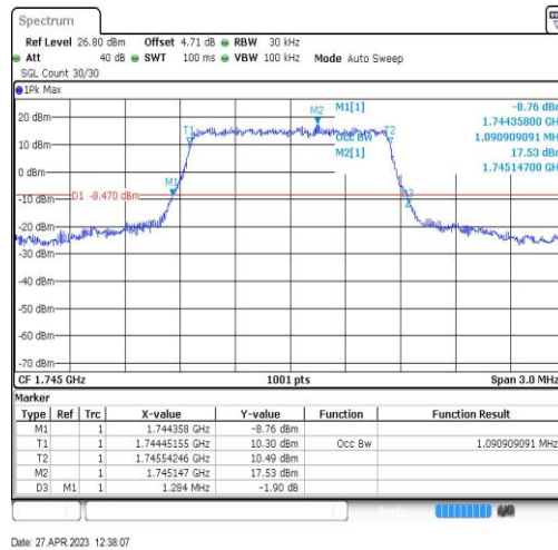
Band66-1.4MHz-QPSK-132322-6RB#0-1.091
