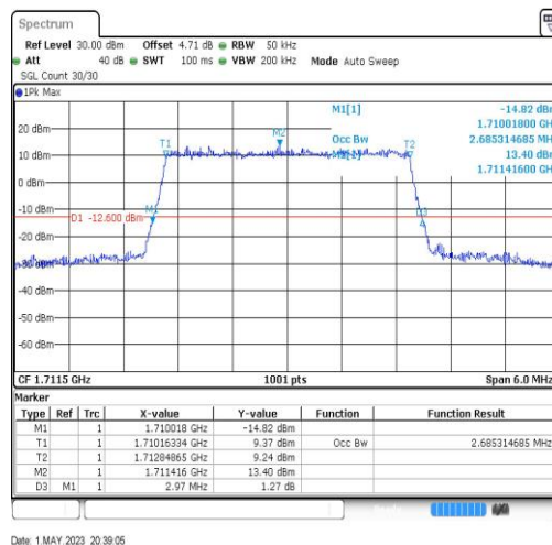
Band66-3MHz-64QAM-131987-15RB#0-2.685
