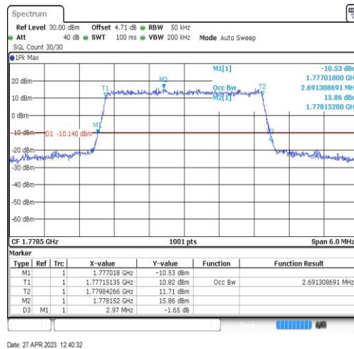
Band66-3MHz-QPSK-132657-15RB#0-2.691
