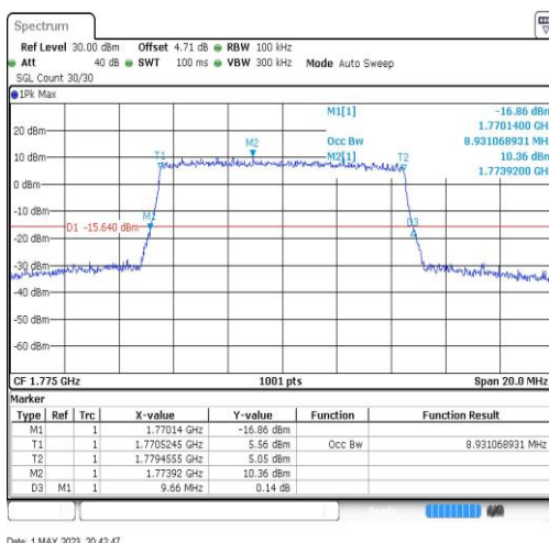
Band66-10MHz-64QAM-132622-50RB#0-8.931
