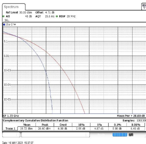
Band66-20MHz-16QAM-132072-100RB#0
