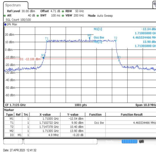
Band66-5MHz-QPSK-131997-25RB#0-4.466
