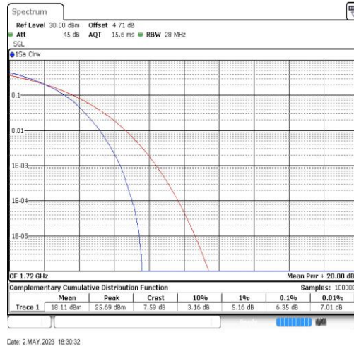
Band66-20MHz-64QAM-132072-100RB#0
