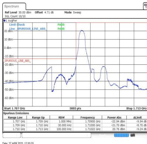
Band66-1.4MHz-QPSK-131979-1RB#0
