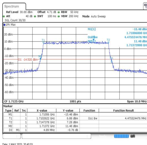
Band66-5MHz-64QAM-131997-25RB#0-4.476
