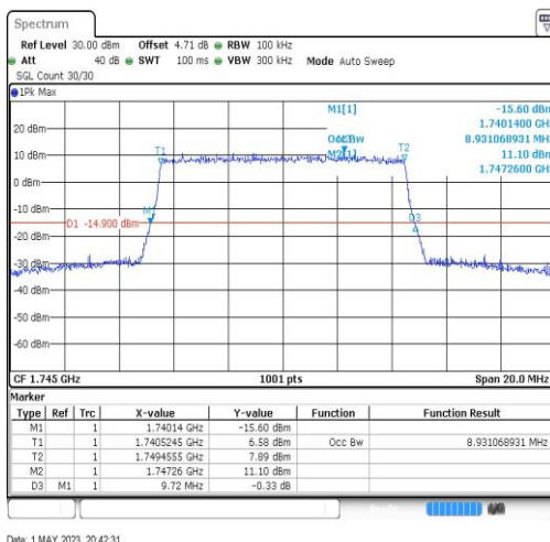
Band66-10MHz-64QAM-132322-50RB#0-8.931
