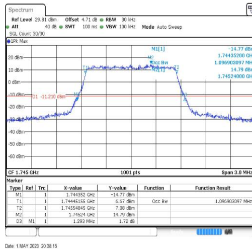
Band66-1.4MHz-64QAM-132322-6RB#0-1.097
