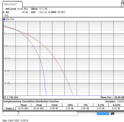
Band66-20MHz-16QAM-132322-100RB#0
