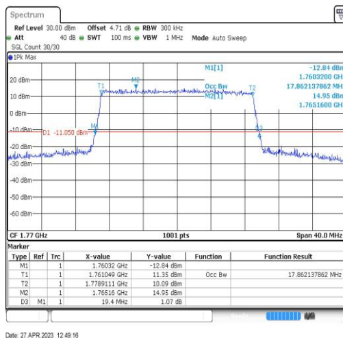
Band66-20MHz-16QAM-132572-100RB#0-17.862
