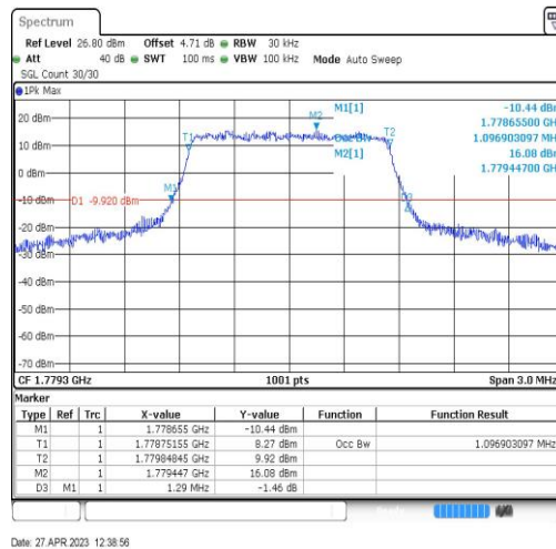
Band66-1.4MHz-16QAM-132665-6RB#0-1.097
