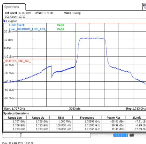
Band66-1.4MHz-QPSK-131979-6RB#0
