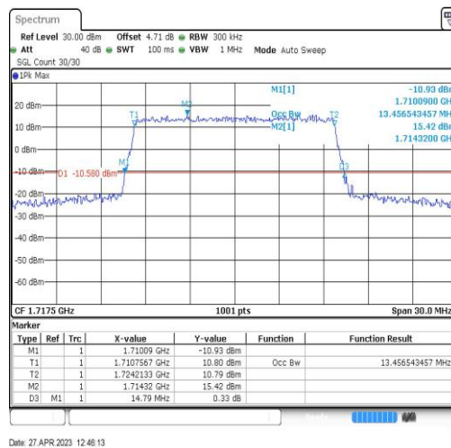
Band66-15MHz-16QAM-132047-75RB#0-13.457
