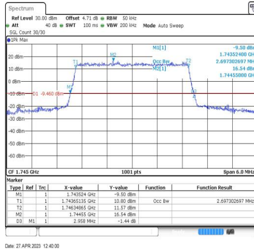
Band66-3MHz-QPSK-132322-15RB#0-2.697
