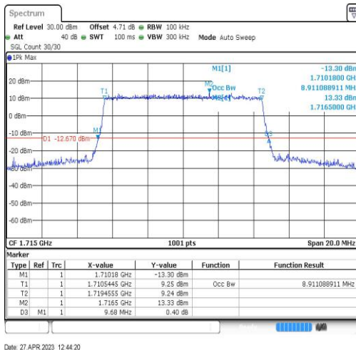
Band66-10MHz-16QAM-132022-50RB#0-8.911
