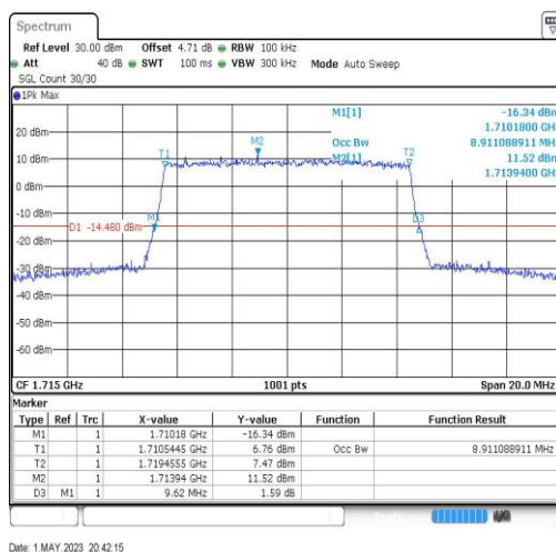
Band66-10MHz-64QAM-132022-50RB#0-8.911
