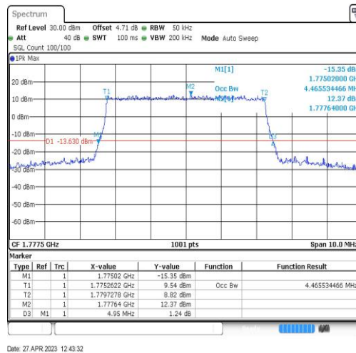
Band66-5MHz-16QAM-132647-25RB#0-4.466
