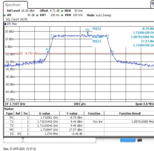
Band66-1.4MHz-QPSK-131979-6RB#0-1.088
