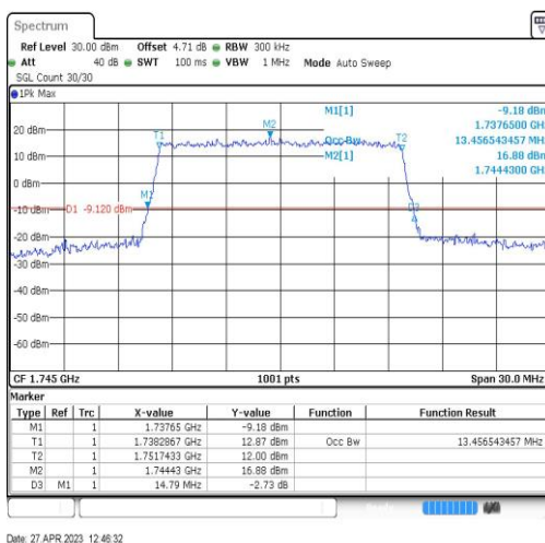
Band66-15MHz-QPSK-132322-75RB#0-13.457
