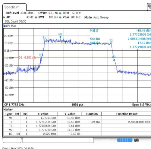
Band66-3MHz-64QAM-132657-15RB#0-2.685
