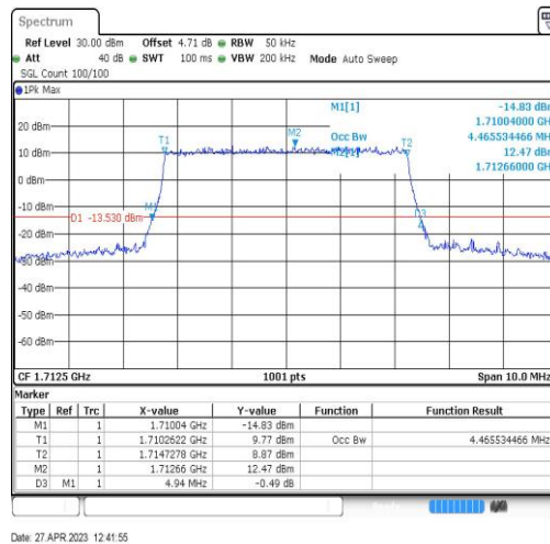
Band66-5MHz-16QAM-131997-25RB#0-4.466
