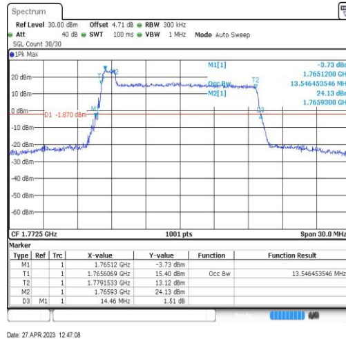
Band66-15MHz-QPSK-132597-75RB#0-13.546
