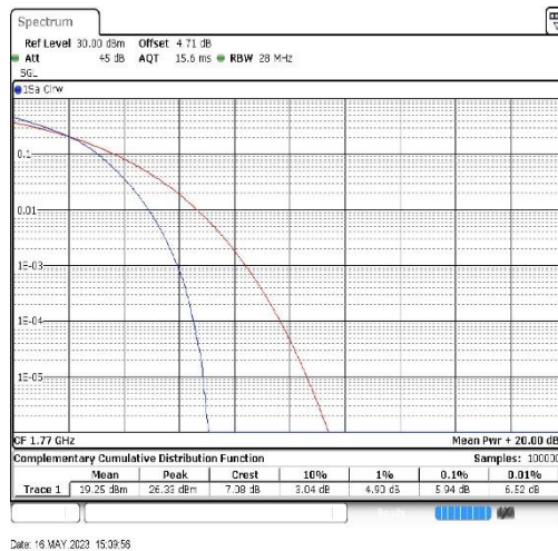
Band66-20MHz-16QAM-132572-100RB#0
