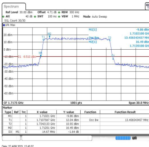
Band66-15MHz-QPSK-132047-75RB#0-13.457
