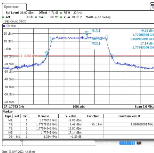
Band66-1.4MHz-QPSK-132665-6RB#0-1.091
