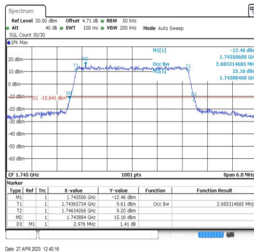
Band66-3MHz-16QAM-132322-15RB#0-2.685
