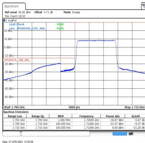
Band66-3MHz-QPSK-131987-15RB#0
