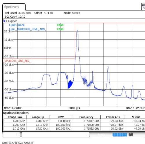
Band66-5MHz-QPSK-131997-1RB#0
