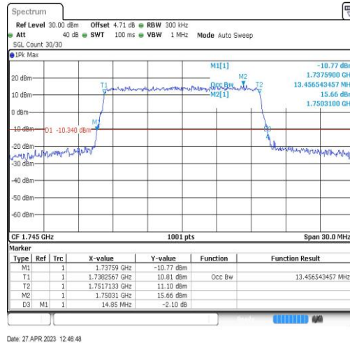
Band66-15MHz-16QAM-132322-75RB#0-13.457
