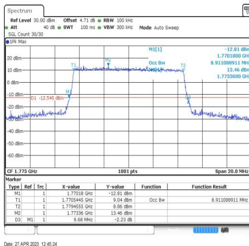
Band66-10MHz-16QAM-132622-50RB#0-8.911
