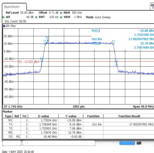
Band66-20MHz-64QAM-132322-100RB#0-17.902
