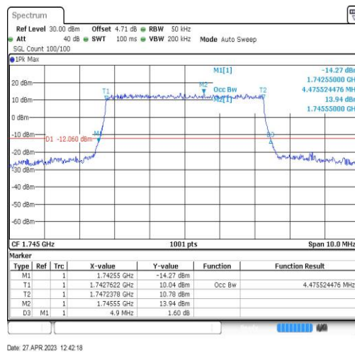
Band66-5MHz-QPSK-132322-25RB#0-4.476
