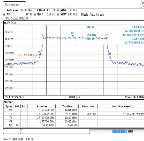
Band66-5MHz-QPSK-132647-25RB#0-4.476
