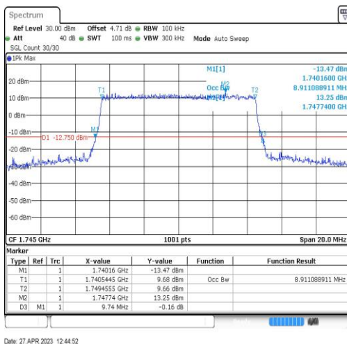
Band66-10MHz-16QAM-132322-50RB#0-8.911
