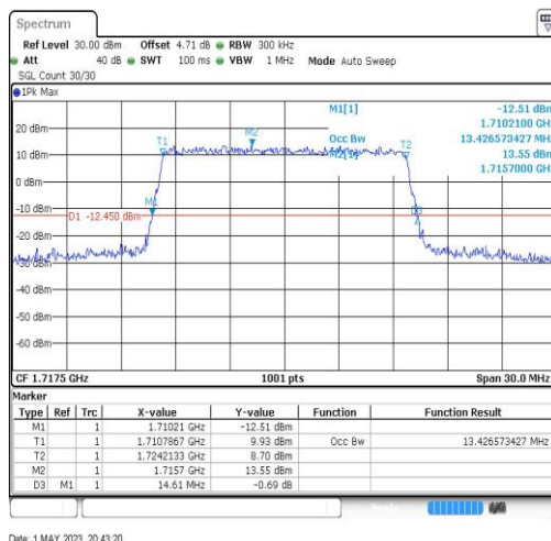
Band66-15MHz-64QAM-132047-75RB#0-13.427
