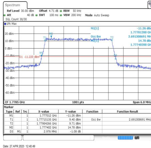
Band66-3MHz-16QAM-132657-15RB#0-2.691
