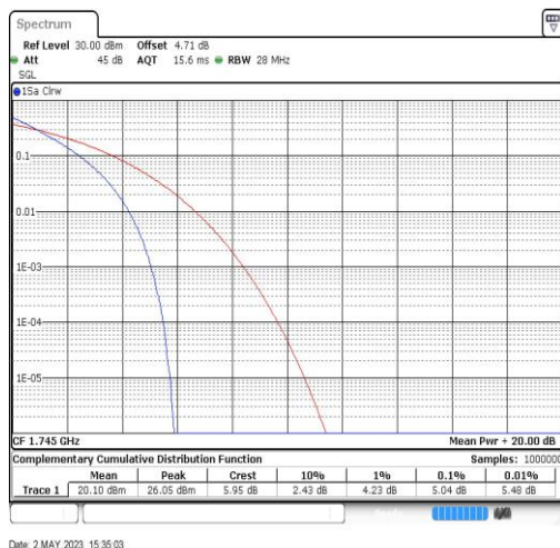
Band66-20MHz-QPSK-132322-100RB#0
