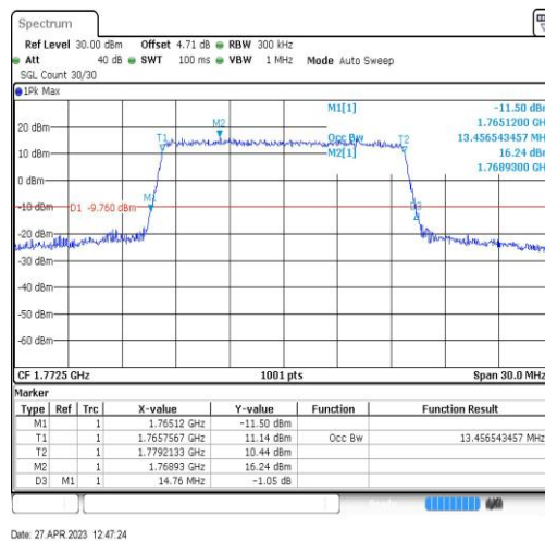
Band66-15MHz-16QAM-132597-75RB#0-13.457
