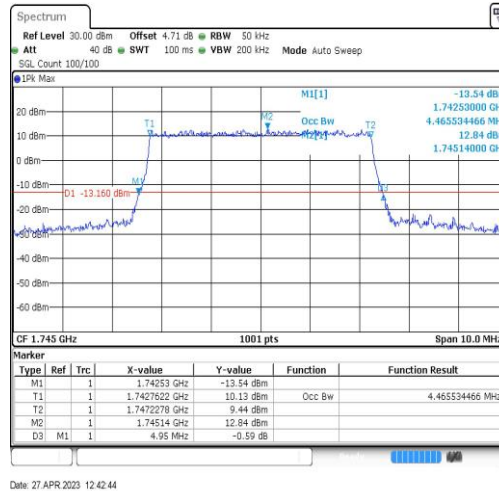
Band66-5MHz-16QAM-132322-25RB#0-4.466
