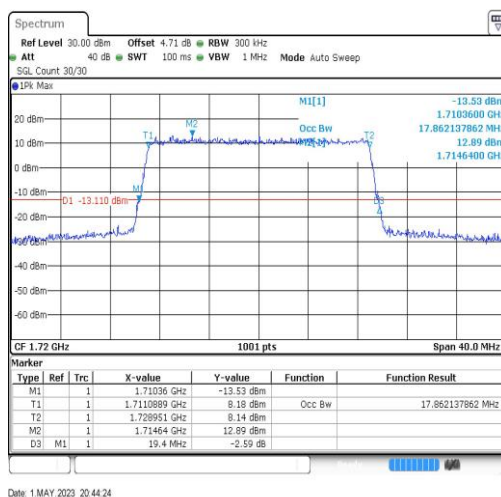
Band66-20MHz-64QAM-132072-100RB#0-17.862
