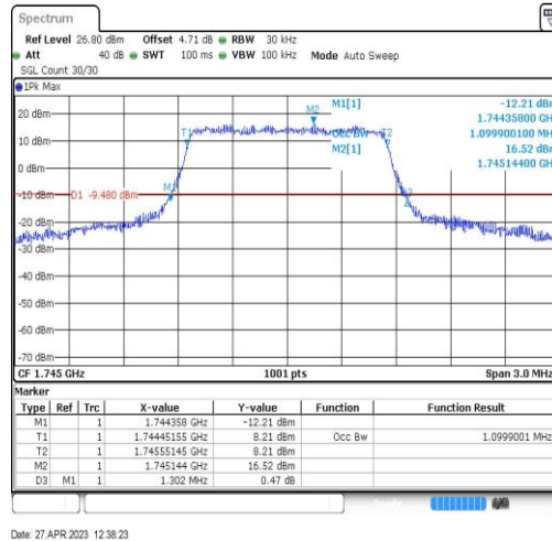
Band66-1.4MHz-16QAM-132322-6RB#0-1.1
