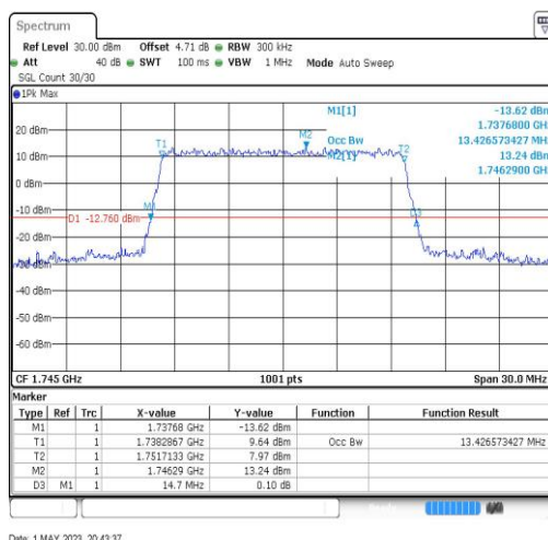
Band66-15MHz-64QAM-132322-75RB#0-13.427
