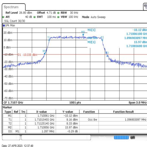
Band66-1.4MHz-16QAM-131979-6RB#0-1.097
