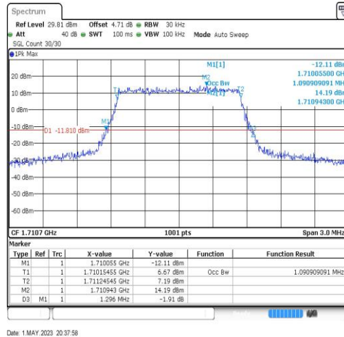
Band66-1.4MHz-64QAM-131979-6RB#0-1.091
