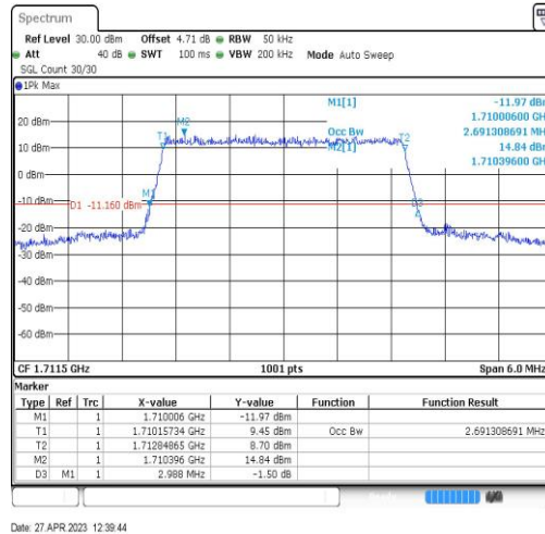
Band66-3MHz-16QAM-131987-15RB#0-2.691
