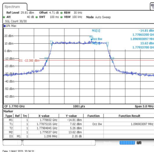
Band66-1.4MHz-64QAM-132665-6RB#0-1.097
