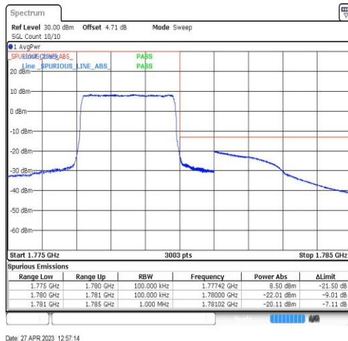
Band66-3MHz-QPSK-132657-15RB#0
