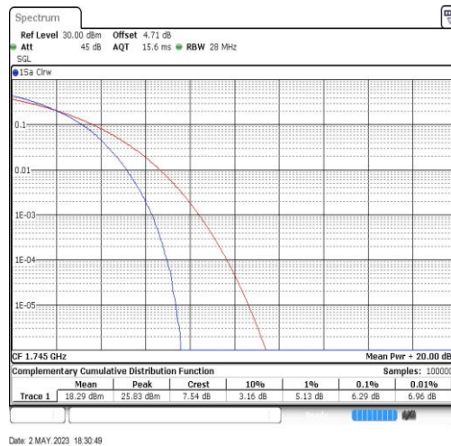
Band66-20MHz-64QAM-132322-100RB#0
