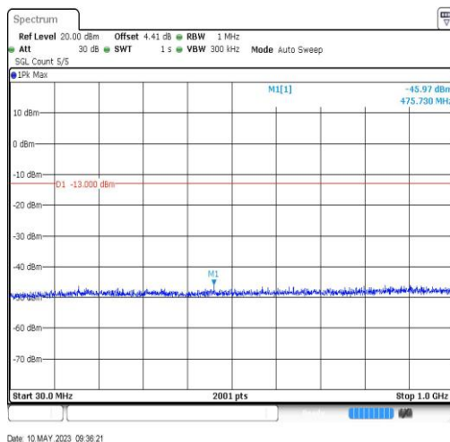
BandIV-1312-30~1000MHz-475.73
