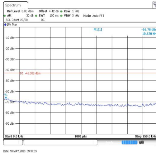
BandIV-1413-0.009~0.15MHz-0.01
