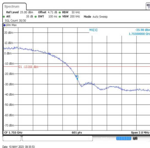
BandIV-1513-1755.00
