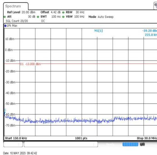
BandV-4233-0.15~30MHz-0.23
