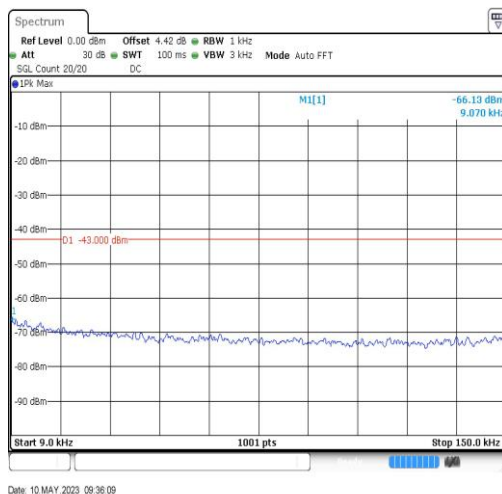
BandIV-1312-0.009~0.15MHz-0.01
