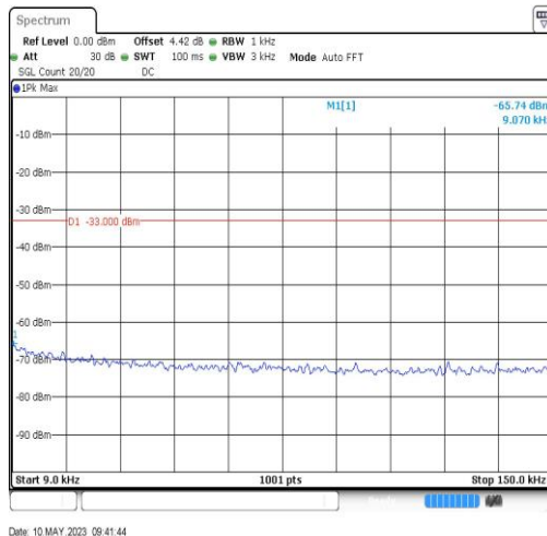
BandV-4182-0.009~0.15MHz-0.01
