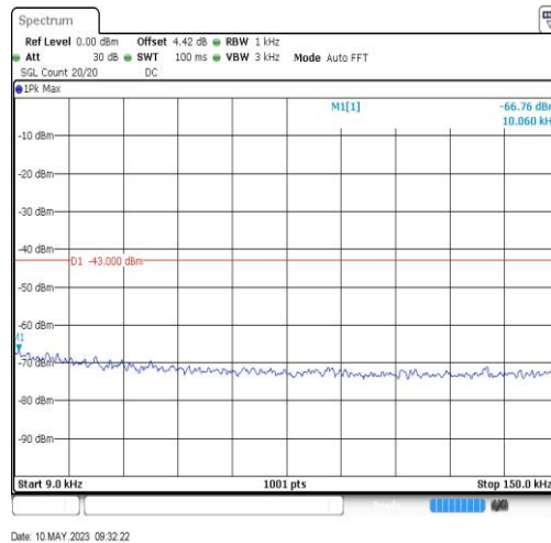
BandII-9400-0.009~0.15MHz-0.01
