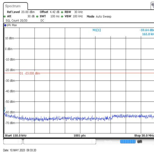
BandII-9538-0.15~30MHz-0.17
