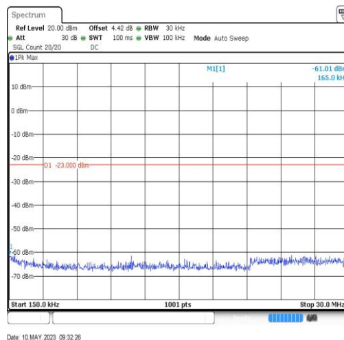
BandII-9400-0.15~30MHz-0.17
