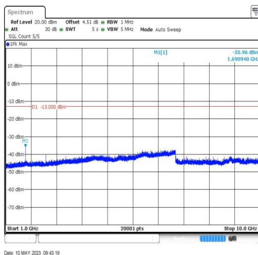
BandV-4233-1000~10000MHz-1690.94
