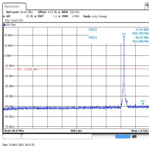
BandV-4132-30~1000MHz-951.5
