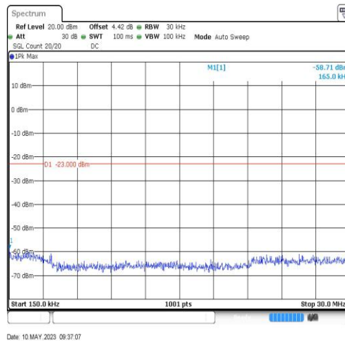
BandIV-1413-0.15~30MHz-0.17
