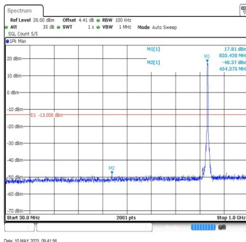
BandV-4182-30~1000MHz-454.38
