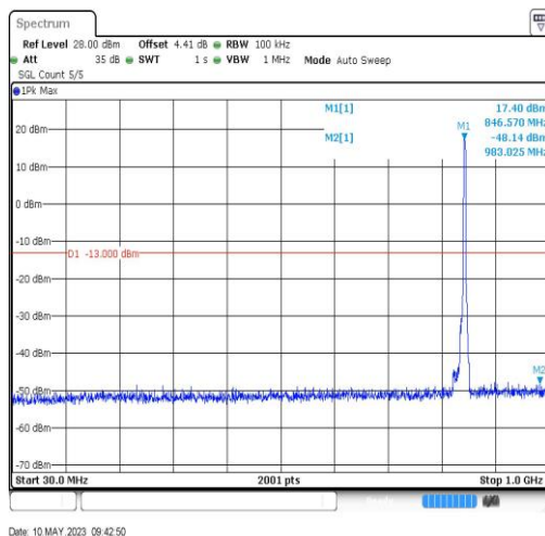
BandV-4233-30~1000MHz-983.03
