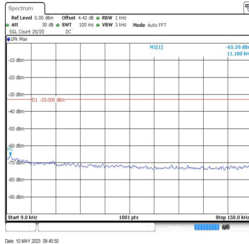
BandV-4132-0.009~0.15MHz-0.01
