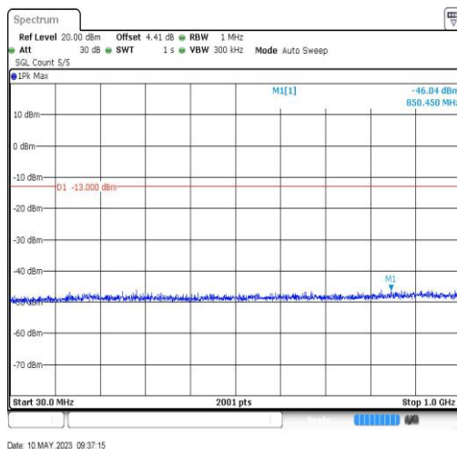
BandIV-1413-30~1000MHz-850.45
