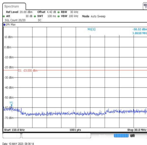
BandIV-1312-0.15~30MHz-1.87
