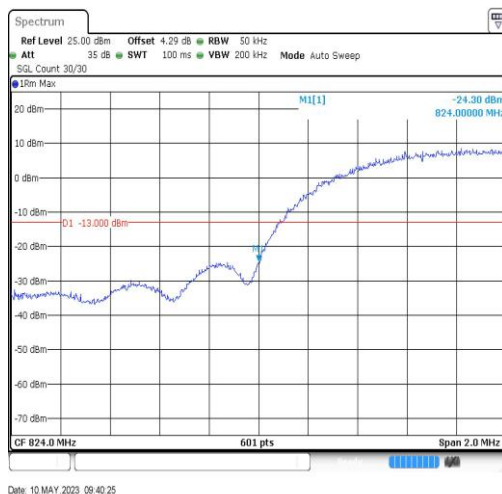
BandV-4132-824.00
