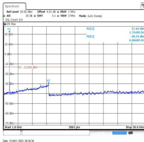
BandIV-1513-1000~20000MHz-6966
