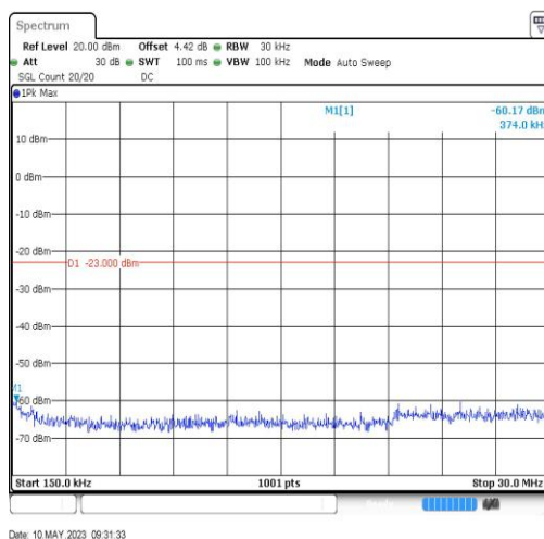
BandII-9262-0.15~30MHz-0.37
