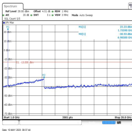
BandIV-1413-1000~20000MHz-6985
