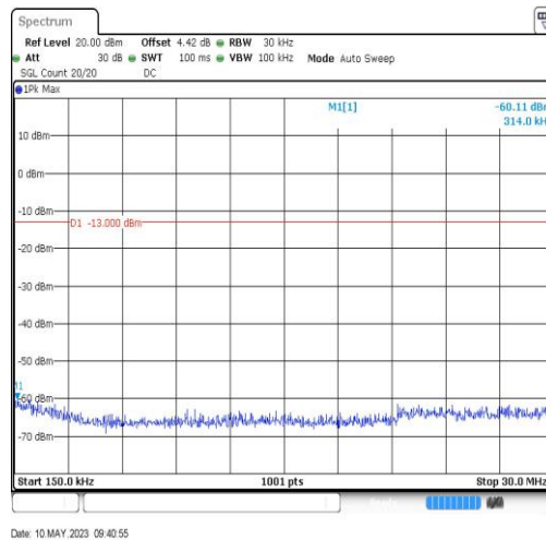
BandV-4132-0.15~30MHz-0.31
