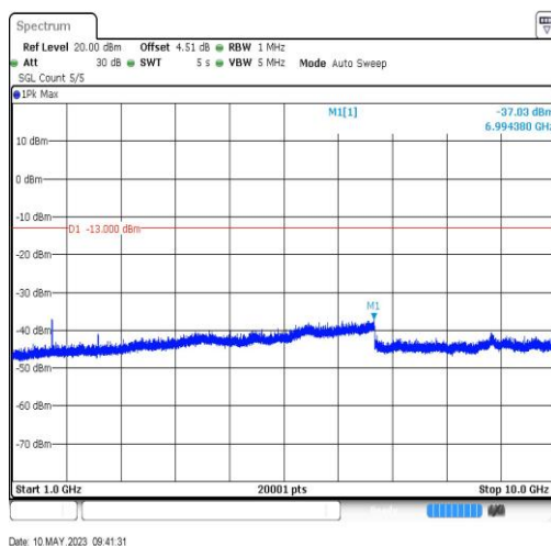
BandV-4132-1000~10000MHz-6994.38
