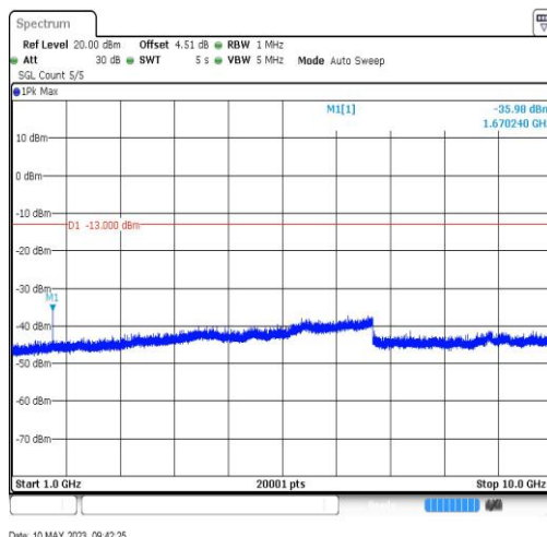
BandV-4182-1000~10000MHz-1670.24
