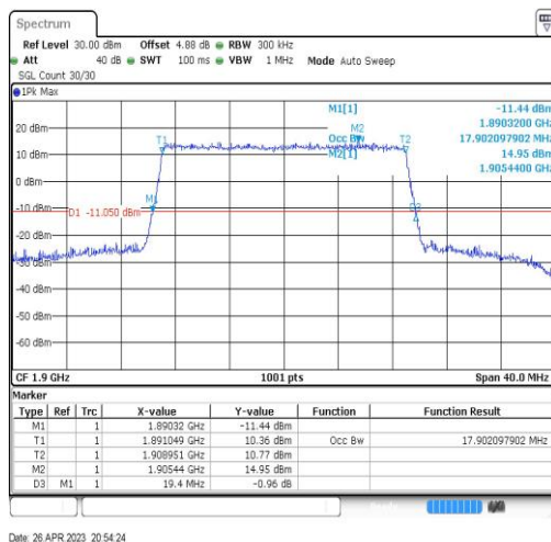
Band2-20MHz-16QAM-19100-100RB#0-17.902
