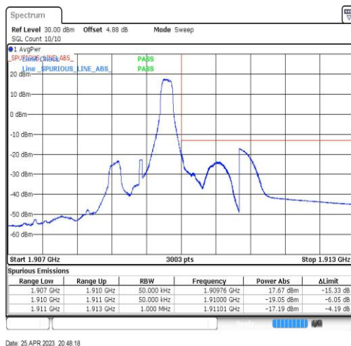
Band2-1.4MHz-QPSK-19193-1RB#5
