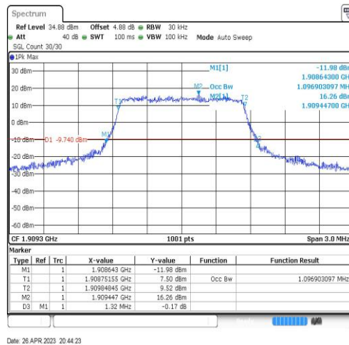
Band2-1.4MHz-16QAM-19193-6RB#0-1.097
