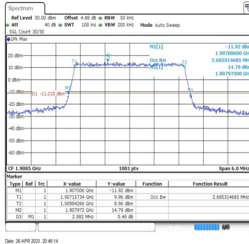
Band2-3MHz-16QAM-19185-15RB#0-2.685
