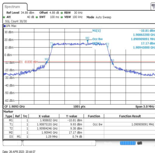
Band2-1.4MHz-QPSK-19193-6RB#0-1.091
