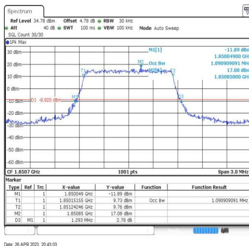
Band2-1.4MHz-QPSK-18607-6RB#0-1.091
