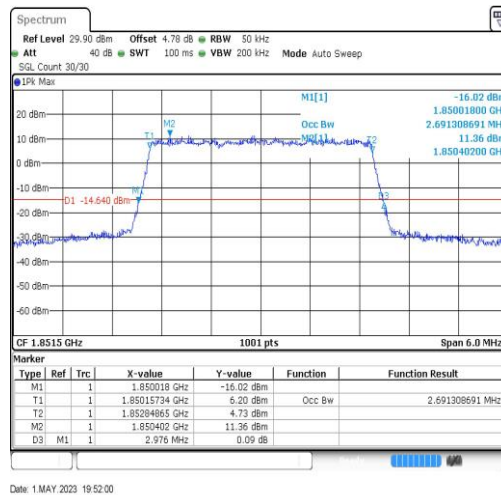
Band2-3MHz-64QAM-18615-15RB#0-2.691
