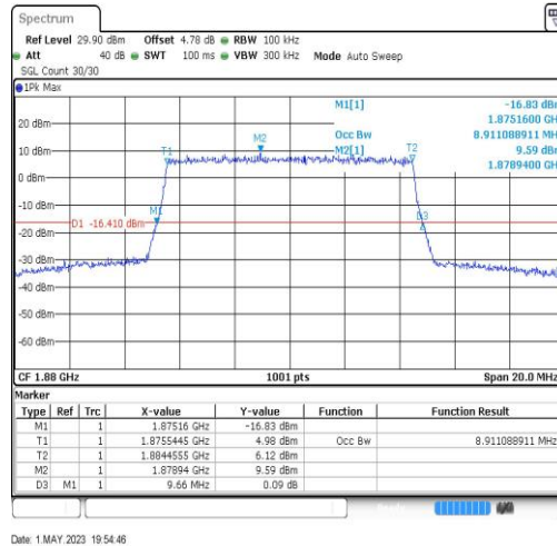
Band2-10MHz-64QAM-18900-50RB#0-8.911
