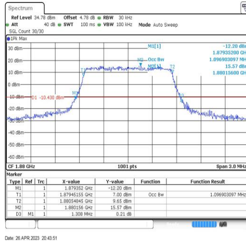
Band2-1.4MHz-16QAM-18900-6RB#0-1.097
