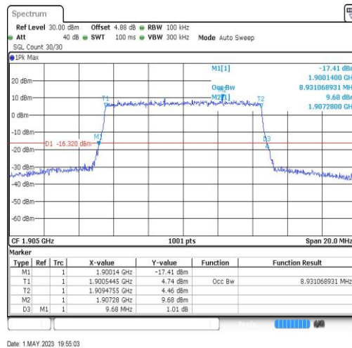
Band2-10MHz-64QAM-19150-50RB#0-8.931
