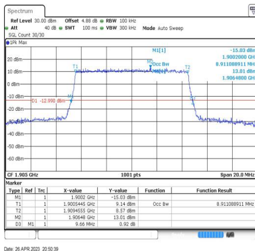
Band2-10MHz-16QAM-19150-50RB#0-8.911
