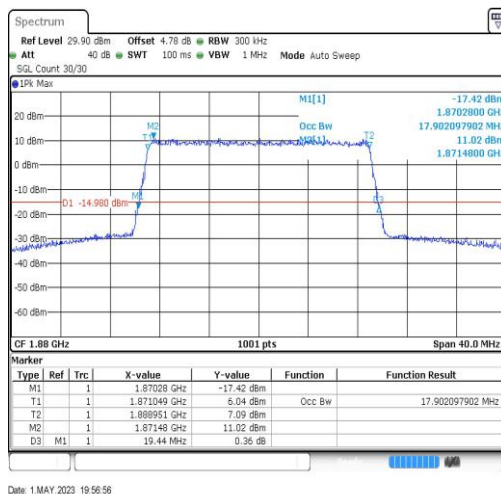
Band2-20MHz-64QAM-18900-100RB#0-17.902
