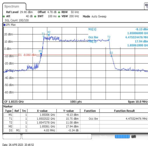
Band2-5MHz-QPSK-18625-25RB#0-4.476
