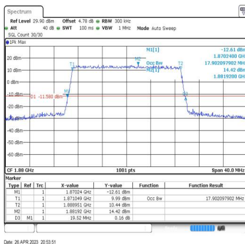
Band2-20MHz-16QAM-18900-100RB#0-17.902
