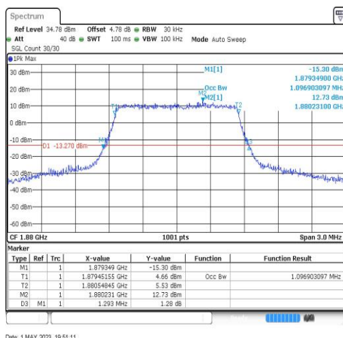
Band2-1.4MHz-64QAM-18900-6RB#0-1.097
