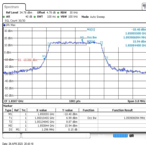
Band2-1.4MHz-16QAM-18607-6RB#0-1.094
