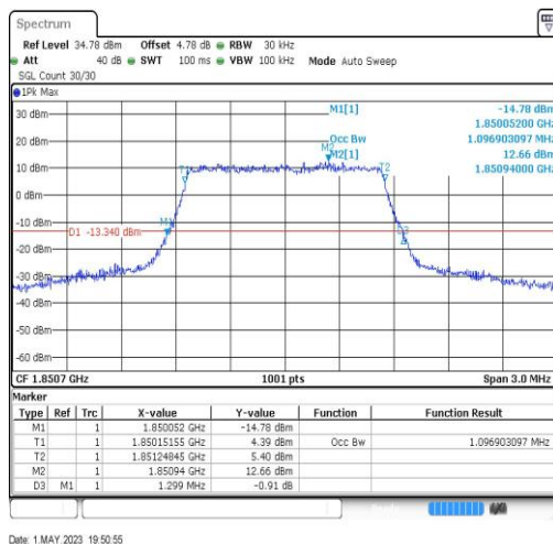
Band2-1.4MHz-64QAM-18607-6RB#0-1.097
