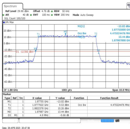
Band2-5MHz-QPSK-18900-25RB#0-4.476
