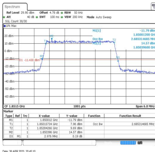
Band2-3MHz-16QAM-18615-15RB#0-2.685
