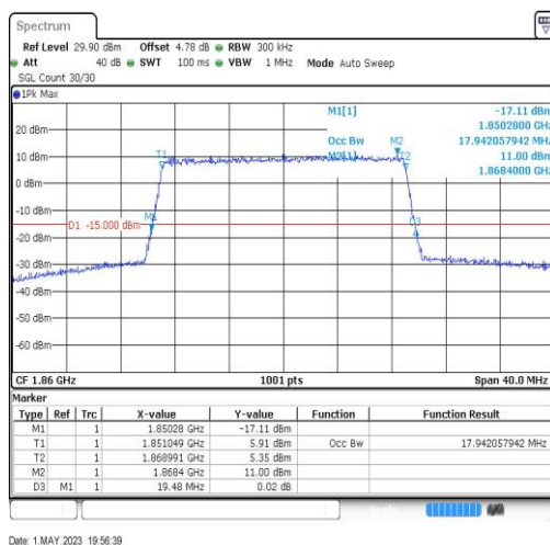
Band2-20MHz-64QAM-18700-100RB#0-17.942
