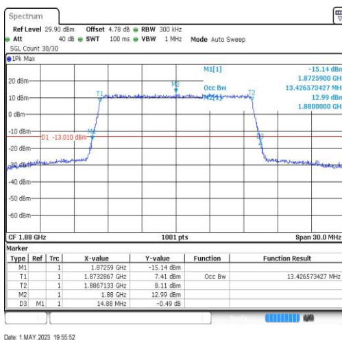
Band2-15MHz-64QAM-18900-75RB#0-13.427
