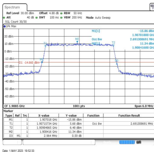
Band2-3MHz-64QAM-19185-15RB#0-2.691
