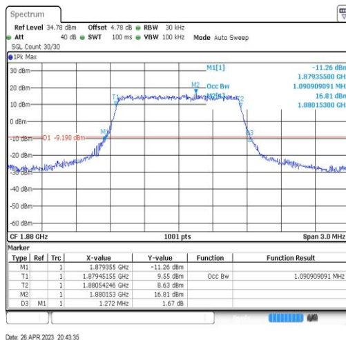
Band2-1.4MHz-QPSK-18900-6RB#0-1.091
