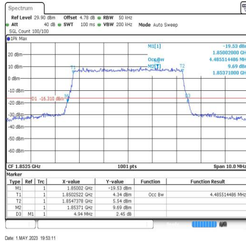
Band2-5MHz-64QAM-18625-25RB#0-4.486
