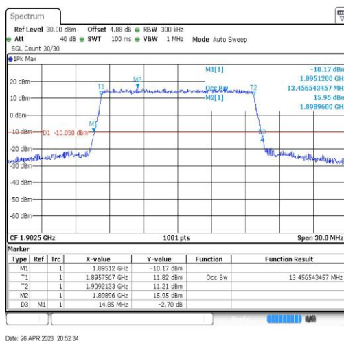
Band2-15MHz-16QAM-19125-75RB#0-13.457
