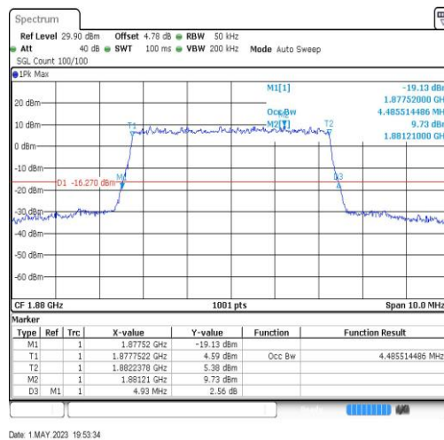
Band2-5MHz-64QAM-18900-25RB#0-4.486
