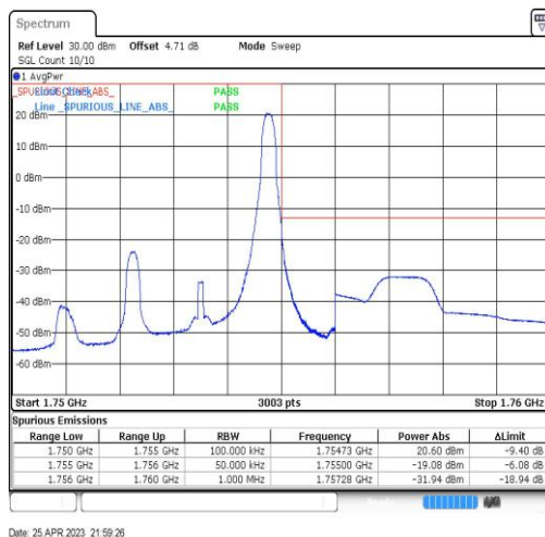
Band4-3MHz-QPSK-20385-1RB#14
