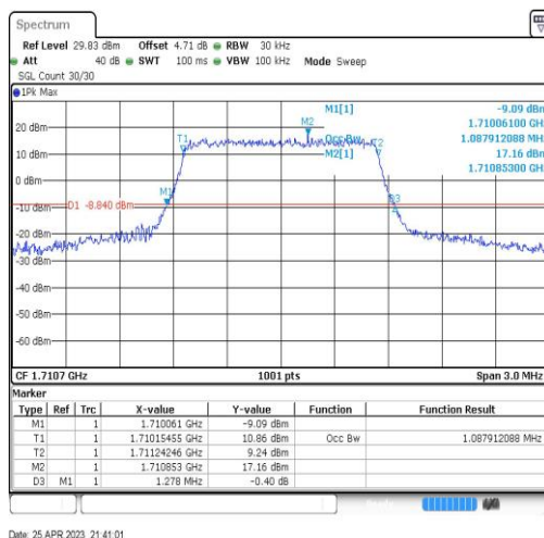
Band4-1.4MHz-QPSK-19957-6RB#0-1.088
