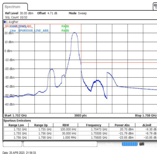
Band4-1.4MHz-QPSK-20393-1RB#5
