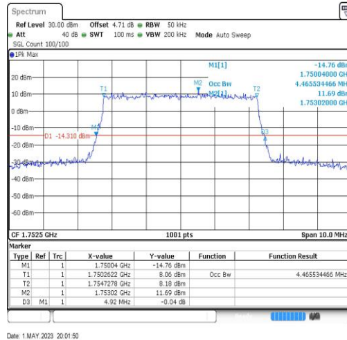
Band4-5MHz-64QAM-20375-25RB#0-4.466
