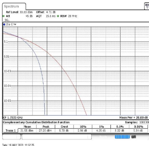
Band4-20MHz-QPSK-20175-100RB#0
