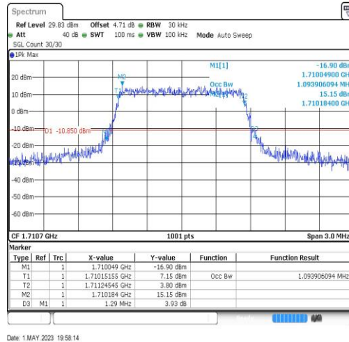
Band4-1.4MHz-64QAM-19957-6RB#0-1.094
