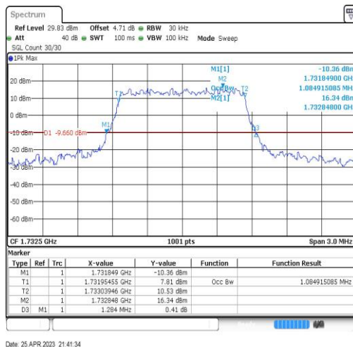
Band4-1.4MHz-QPSK-20175-6RB#0-1.085
