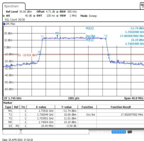
Band4-20MHz-16OAM-20300-100RB#0-17.902
