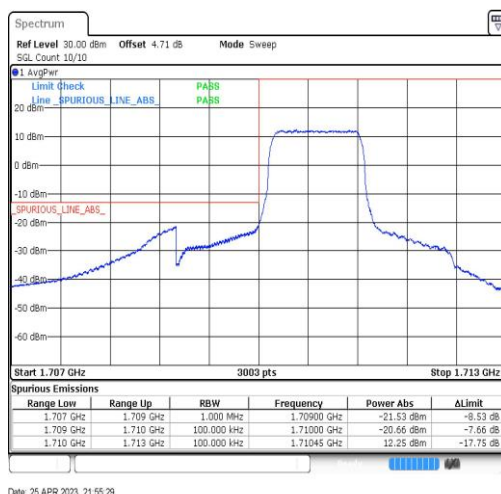
Band4-1.4MHz-QPSK-19957-6RB#0
