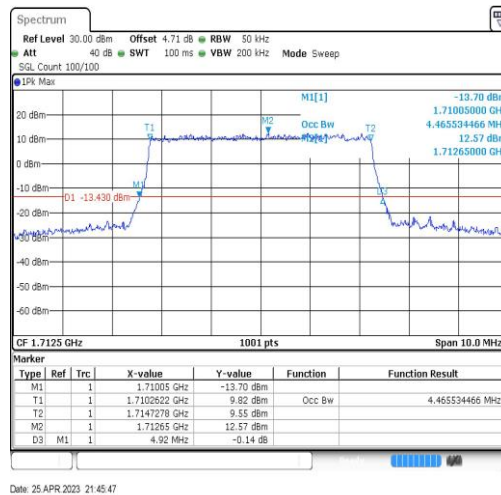
Band4-5MHz-16QAM-19975-25RB#0-4.466
