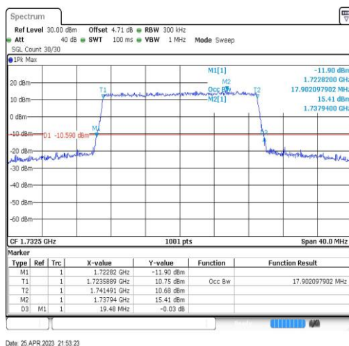
Band4-20MHz-16QAM-20175-100RB#0-17.902
