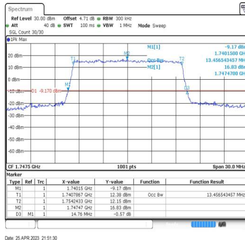
Band4-15MHz-QPSK-20325-75RB#0-13.457
