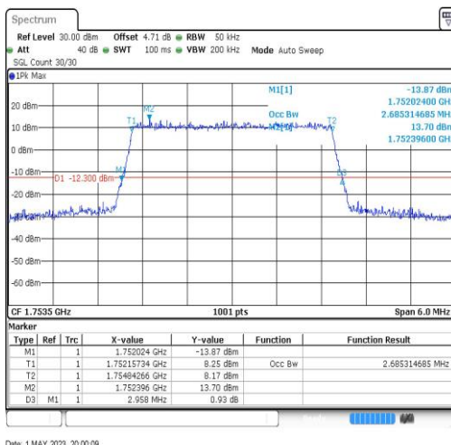
Band4-3MHz-64QAM-20385-15RB#0-2.685
