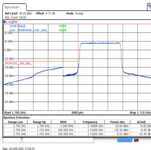
Band4-3MHz-QPSK-19965-15RB#0
