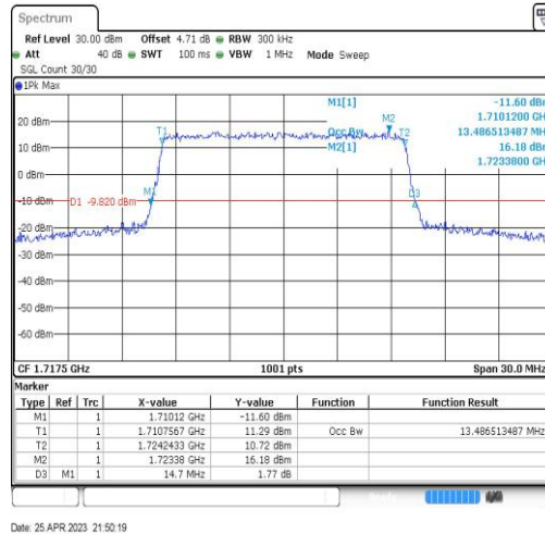
Band4-15MHz-QPSK-20025-75RB#0-13.487
