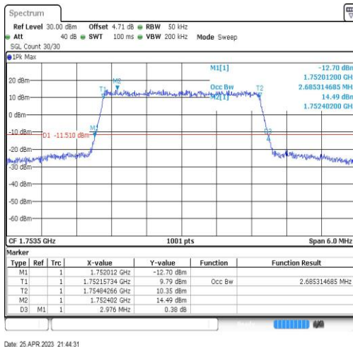
Band4-3MHz-16QAM-20385-15RB#0-2.685
