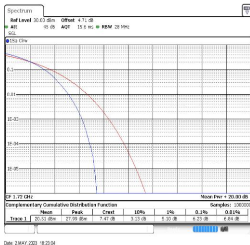
Band4-20MHz-64QAM-20050-100RB#0
