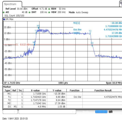
Band4-5MHz-64QAM-19975-25RB#0-4.476
