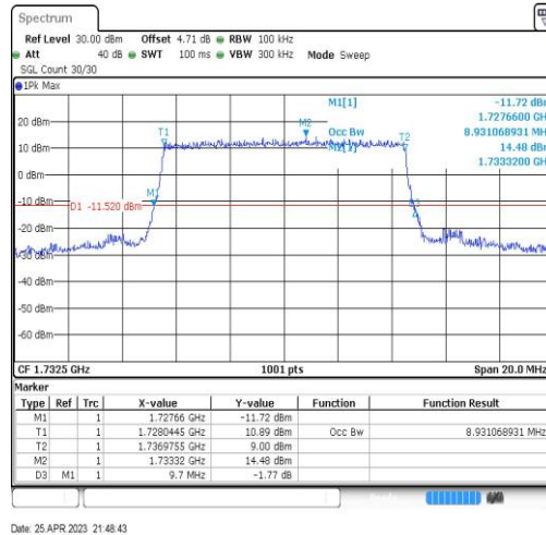
Band4-10MHz-QPSK-20175-50RB#0-8.931
