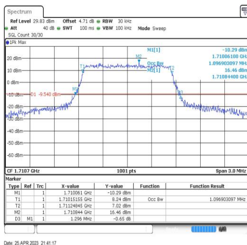
Band4-1.4MHz-16QAM-19957-6RB#0-1.097
