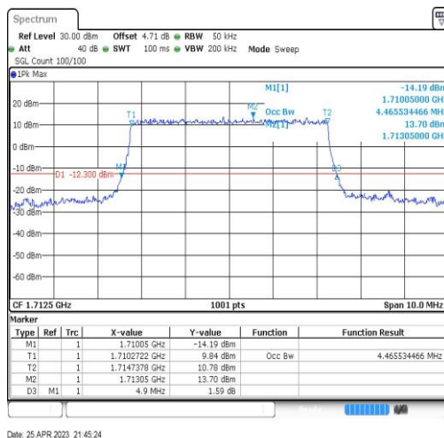
Band4-5MHz-QPSK-19975-25RB#0-4.466
