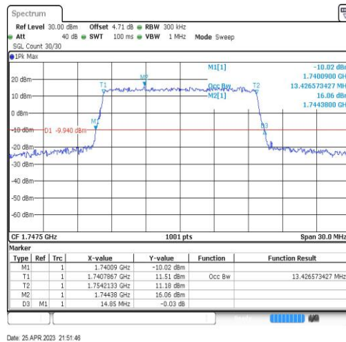
Band4-15MHz-16QAM-20325-75RB#0-13.427
