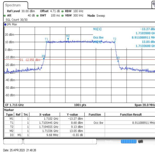
Band4-10MHz-16QAM-20000-50RB#0-8.911
