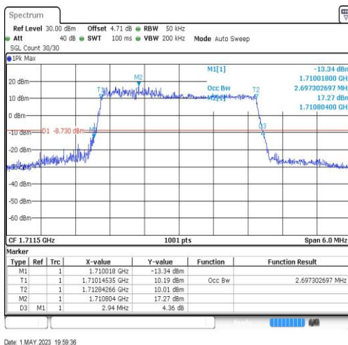
Band4-3MHz-64QAM-19965-15RB#0-2.697
