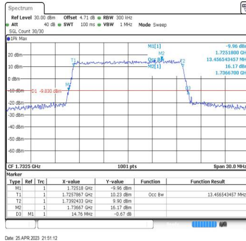
Band4-15MHz-16QAM-20175-75RB#0-13.457
