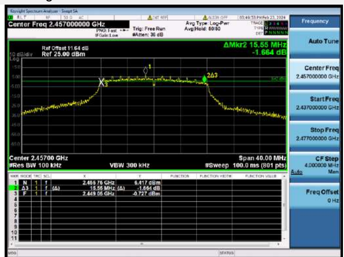
802.11g CHANNEL 10
