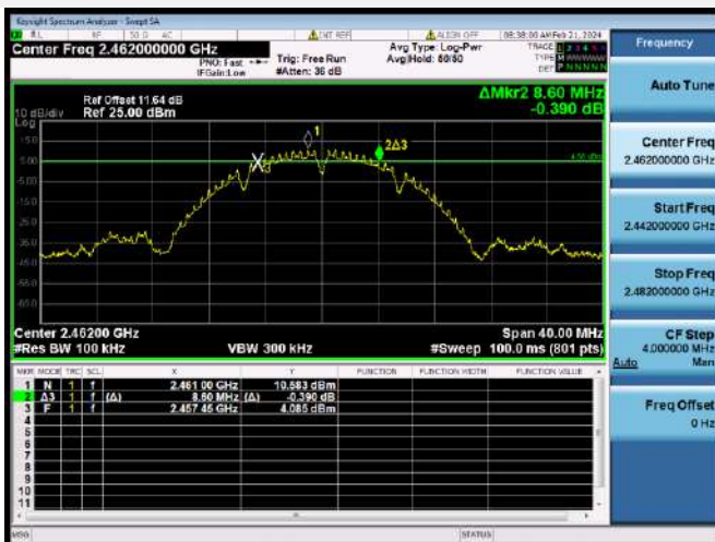
802.11b CHANNEL 11
