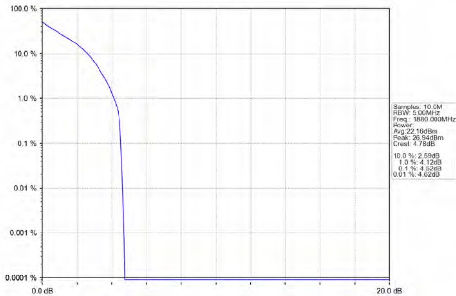
Band2_1.4MHz_QPSK_MCH_1880MHz_RB_6_0_NTNV
