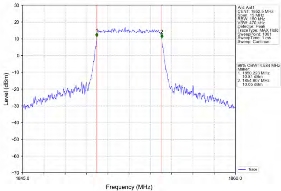
Band2_5MHz_64QAM_LCH_1852.5MHz_RB_25_0_NTNV
