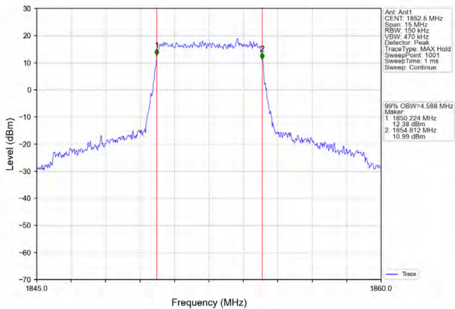
Band2_5MHz_QPSK_LCH_1852.5MHz_RB_25_0_NTNV
