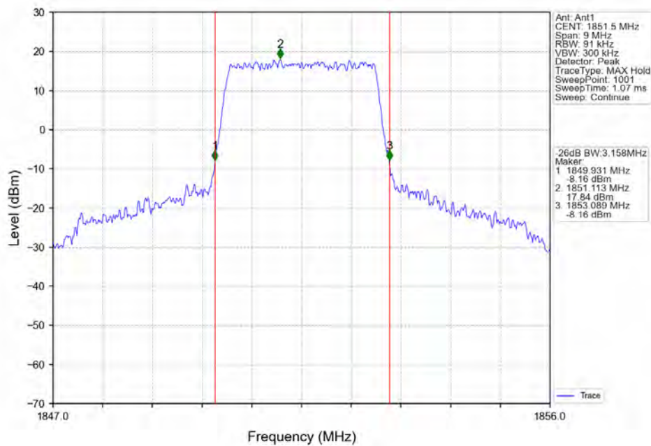
Band2_3MHz_QPSK_LCH_1851.5MHz_RB_15_0_NTNV
