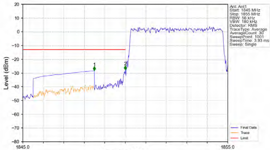
Band2_5MHz_64QAM_LCH_1852.5MHz_RB_25_0_NTNV
