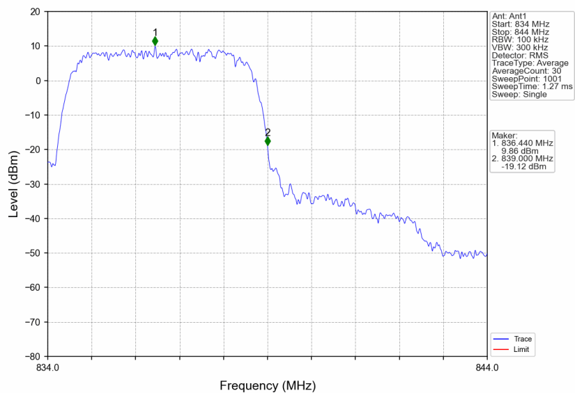
Band V_RMC_MCH_836.6MHz_12.2kbps RMC_NTNV
