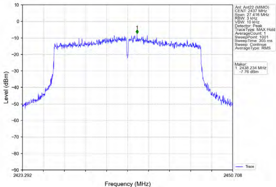
802.11ax(HEW20) MCH_2437MHz RU242 Left Ant22 (MIMO) NTN
