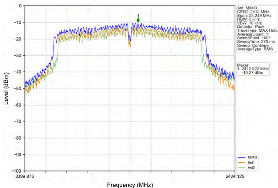
802.11g_LCH_2412MHz_MIMO NTN
