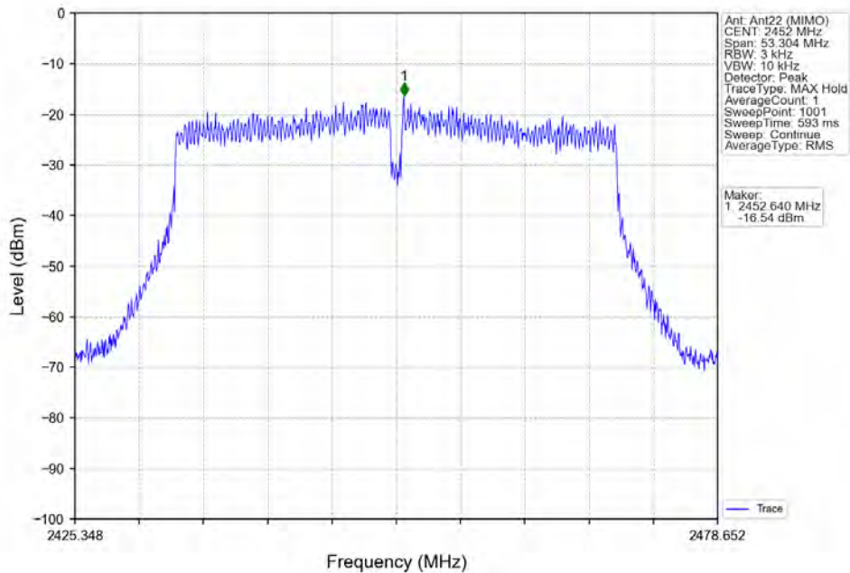
802.11ac(VHT40)_HCH_2452MHz_Ant22 (MIMO)_NTNV
