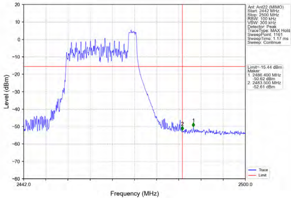
802.11ax(HEW20) HCH 2462MHz RU26 Right Ant22 (MIMO) NTN
