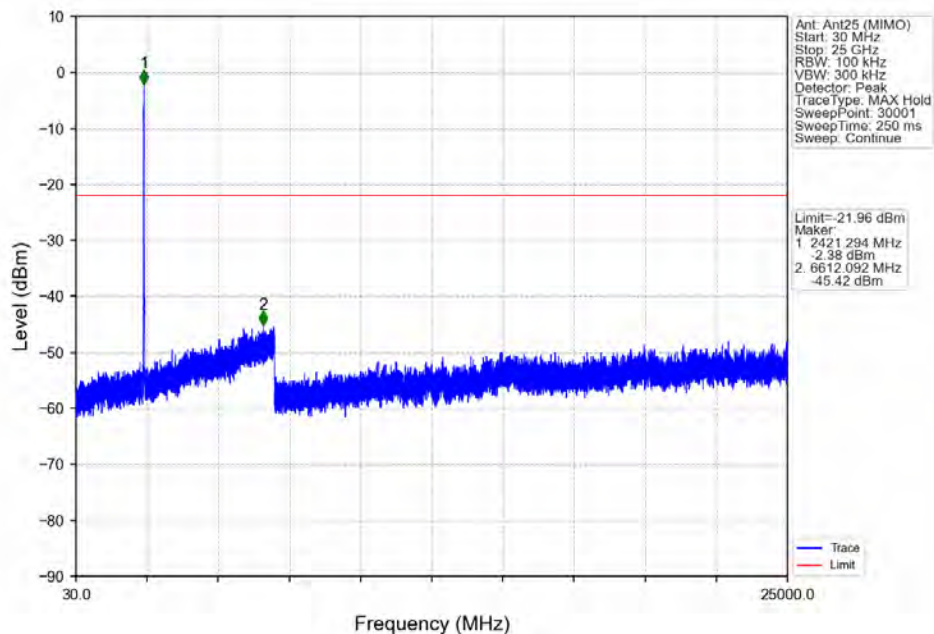
802.11ax(HEW40) LCH 2422MHz RU242 Left Ant25 (MIMO) NTN
