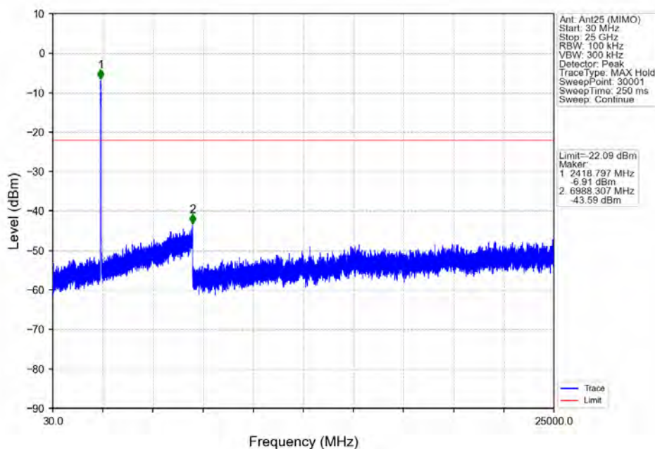
802.11ax(HEW40) LCH_2422MHz_RU484_Left_Ant25 (MIMO) NTN
