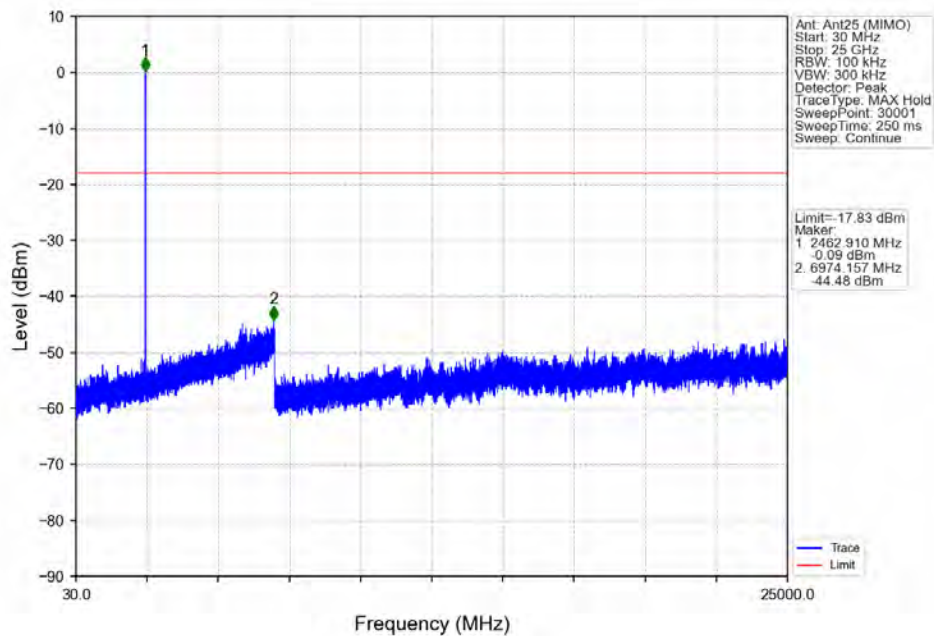
802.11ax(HEW20)_HCH_2462MHz_RU106_Right_Ant25 (MIMO)_NTNV
