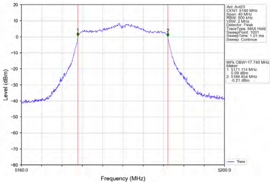
802.11n(HT20) LCH_5180MHz_Ant23_NTNV
