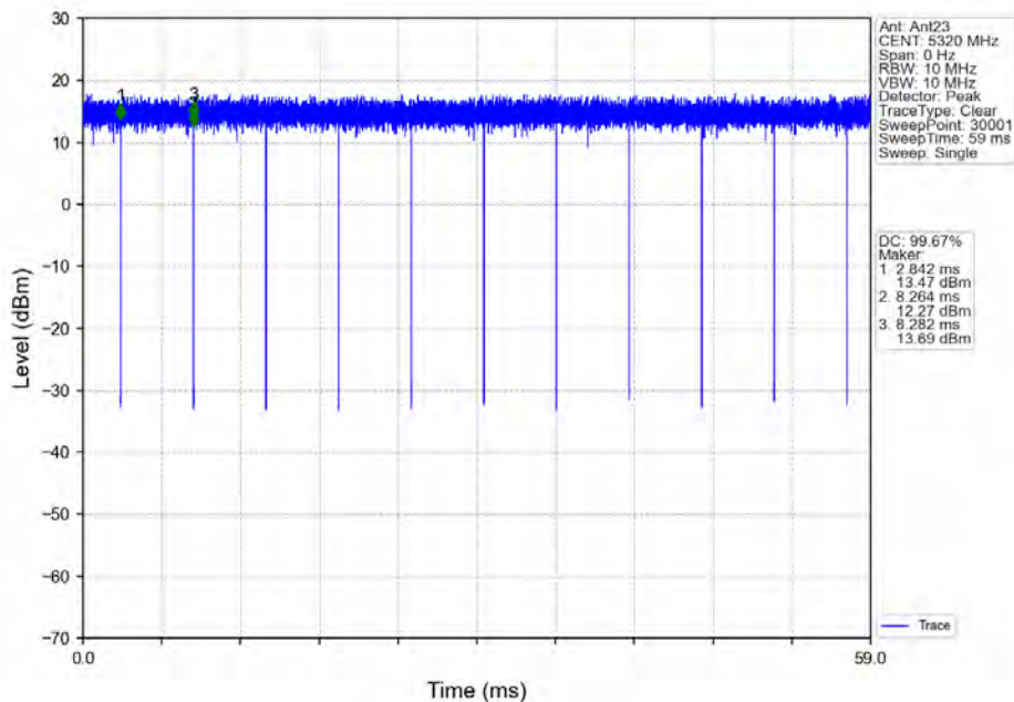
802.11ac(VHT20)_HCH_5320MHz_Ant23_NTNV
