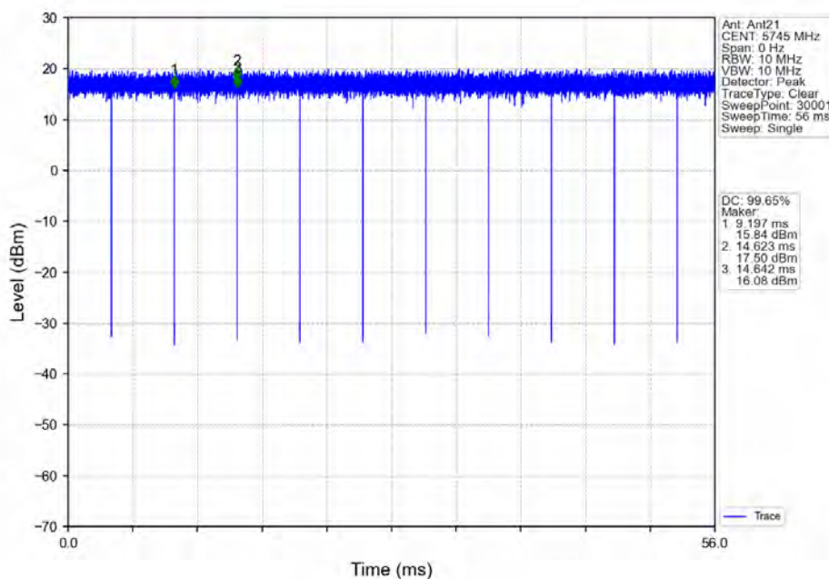
802.11ac(VHT20)_LCH_5745MHz_Ant21_NTNV
