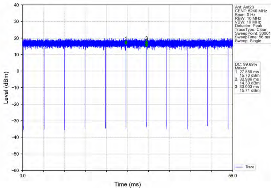
802.11n(HT20) HCH 5240MHz Ant23 NTN
