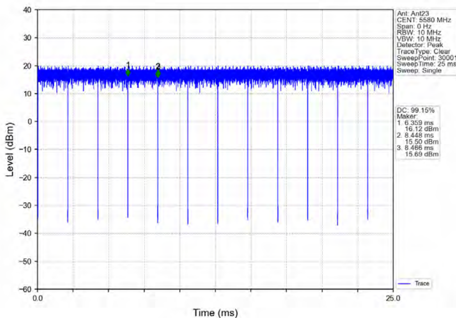
802.11a_MCH_5580MHz_Ant23_NTNV
