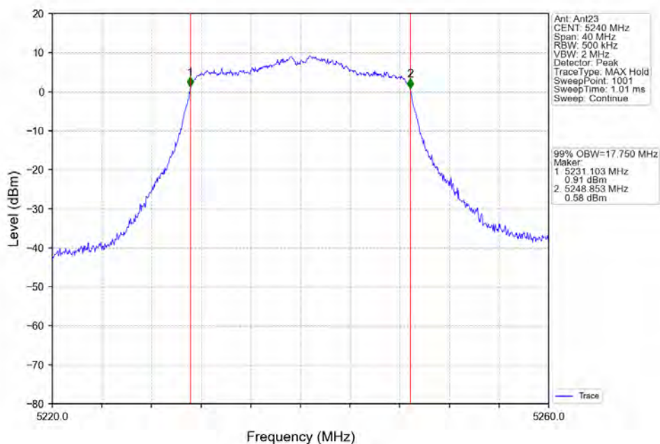
802.11n(HT20) HCH 5240MHz Ant23 NTN
