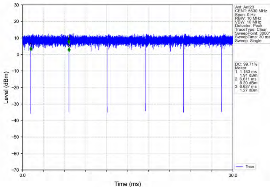
802.11ac(VHT80)_LCH_5530MHz_Ant23_NTNV
