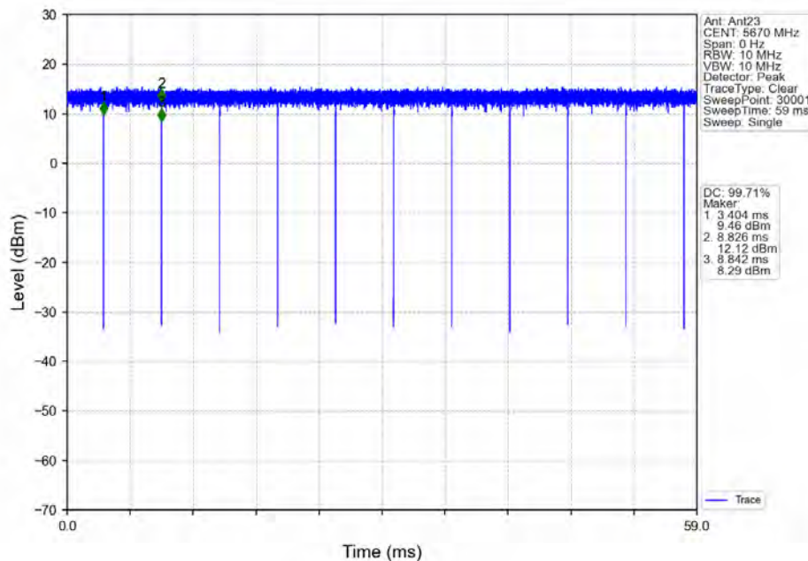
802.11ac(VHT40)_HCH_5670MHz_Ant23_NTNV
