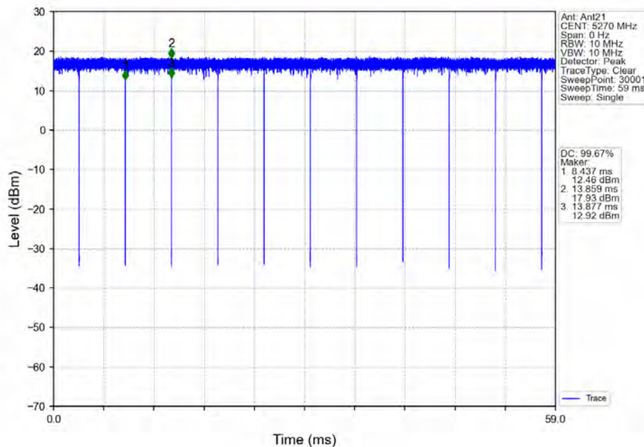
802.11ac(VHT40)_LCH_5270MHz_Ant21_NTNV
