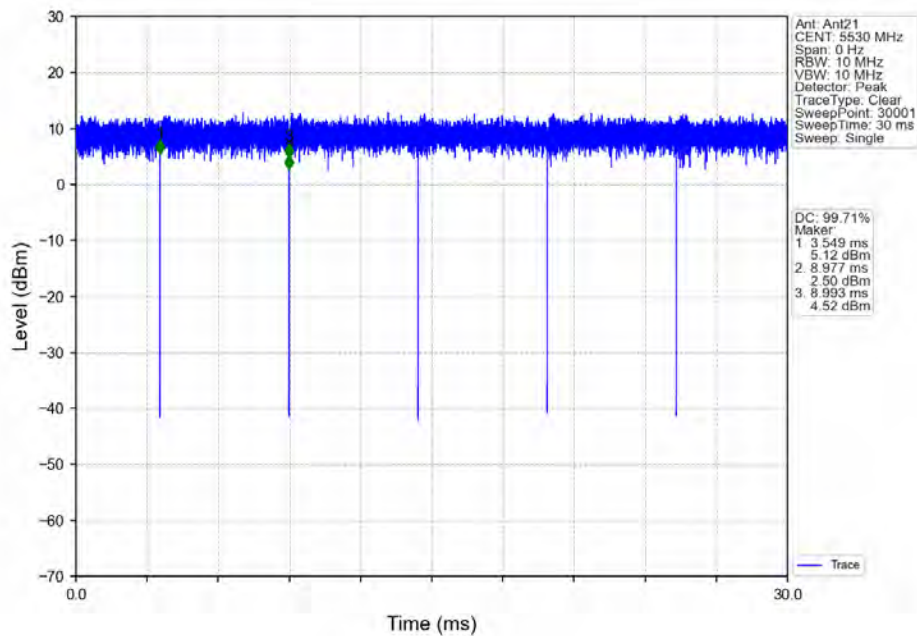
802.11ac(VHT80)_LCH_5530MHz_Ant21_NTNV
