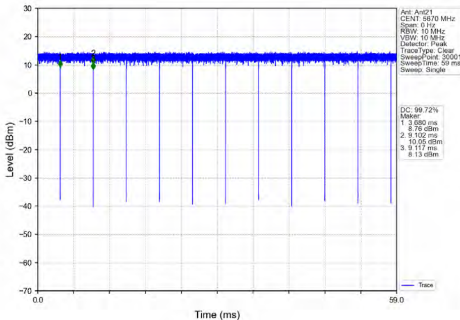
802.11ac(VHT40)_HCH_5670MHz_Ant21_NTNV
