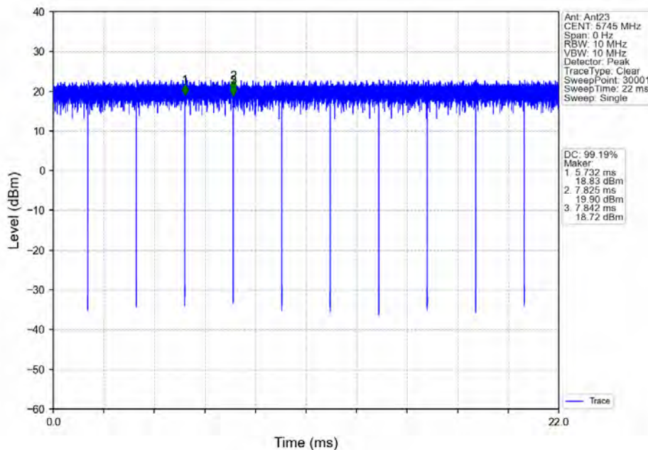
802.11a_LCH_5745MHz_Ant23_NTNV
