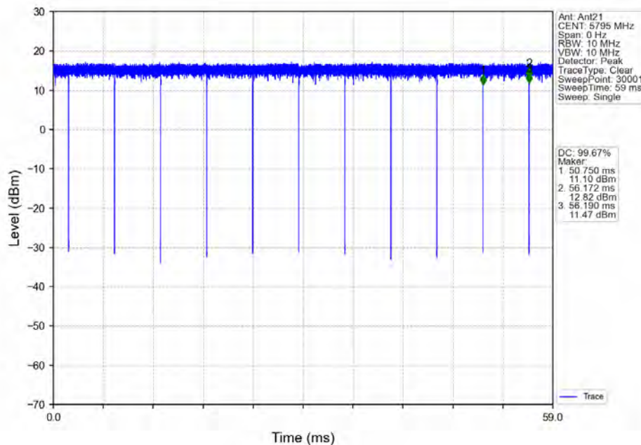
802.11ac(VHT40)_HCH_5795MHz_Ant21_NTNV
