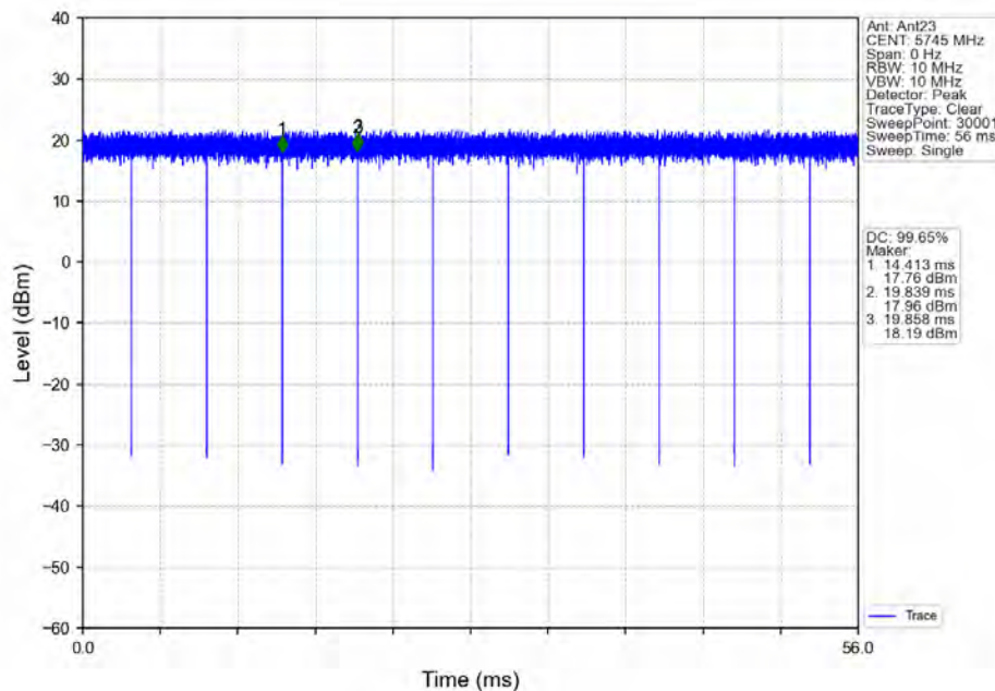
802.11ac(VHT20)_LCH_5745MHz_Ant23_NTNV
