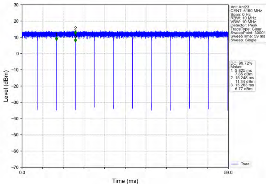
802.11ac(VHT40)_LCH_5190MHz_Ant23_NTNV
