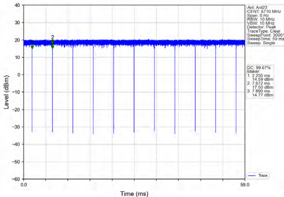
802.11n(HT40) HCH 5710MHz Ant23 NTNV
