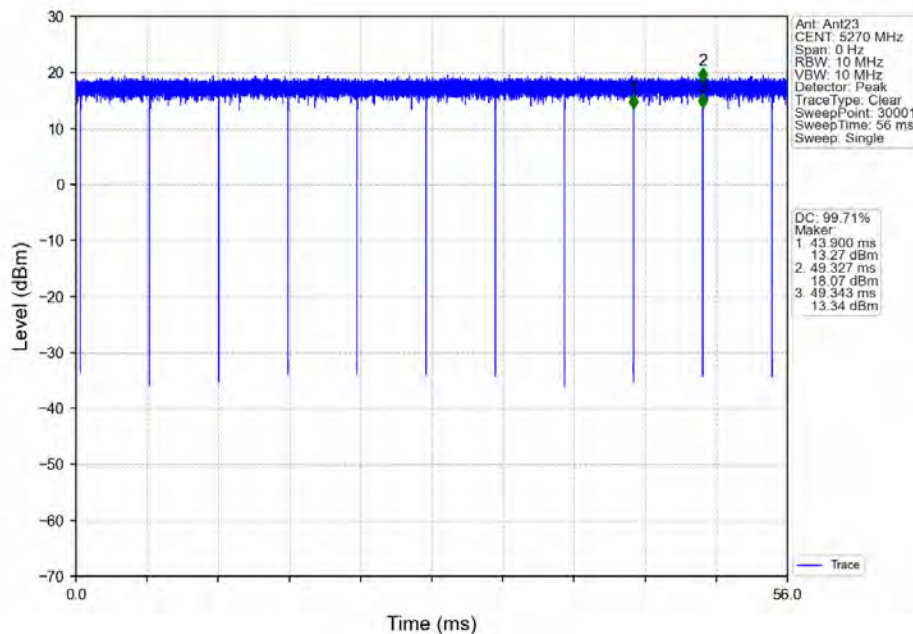
802.11ac(VHT40)_LCH_5270MHz_Ant23_NTNV
