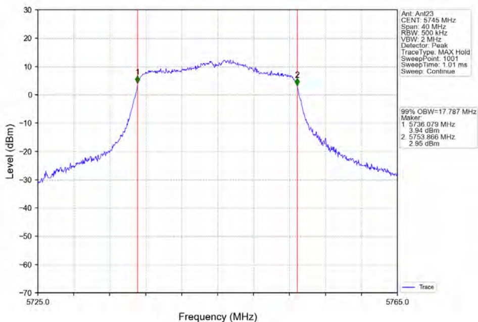
802.11n(HT20) LCH_5745MHz_Ant23_NTNV
