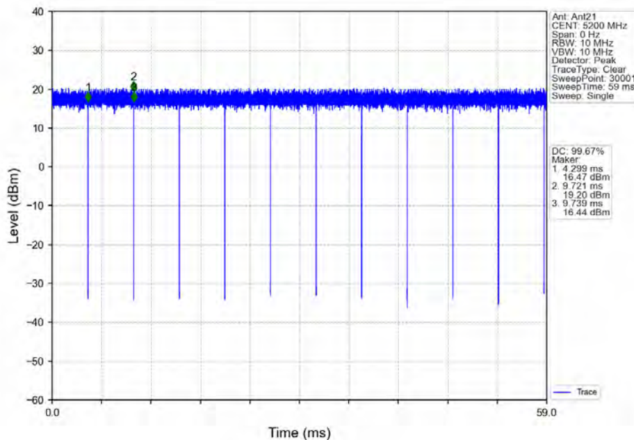
802.11ac(VHT20)_MCH_5200MHz_Ant21_NTNV
