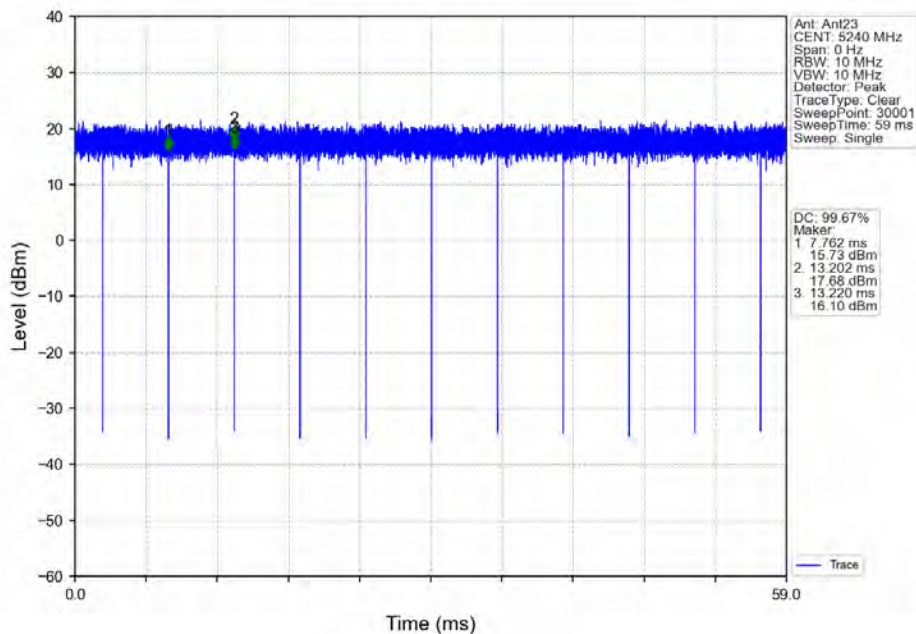
802.11ax(HE20) HCH 5240MHz RU242 Left Ant23 NTNV
