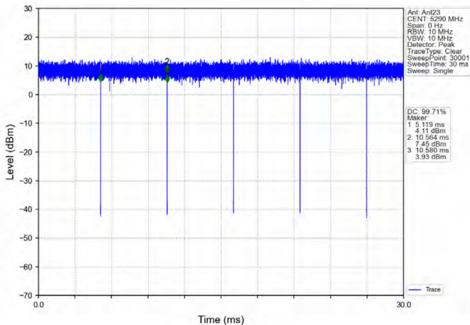
802.11ax(HE80) MCH 5290MHz RU996 Left Ant23 NTNV
