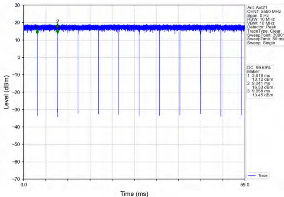
802.11n(HT40)_MCH_5550MHz_Ant21_NTNV
