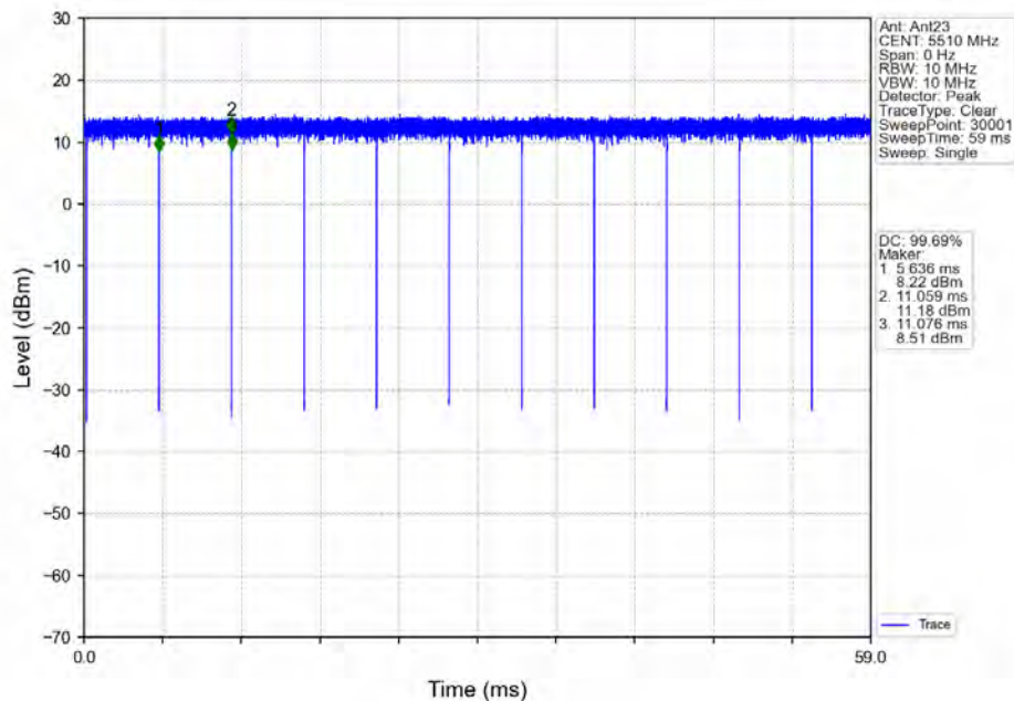
802.11ac(VHT40)_LCH_5510MHz_Ant23_NTNV
