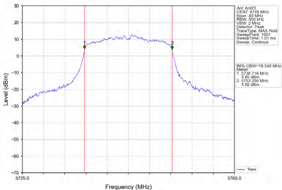
802.11a_LCH_5745MHz_Ant23_NTNV
