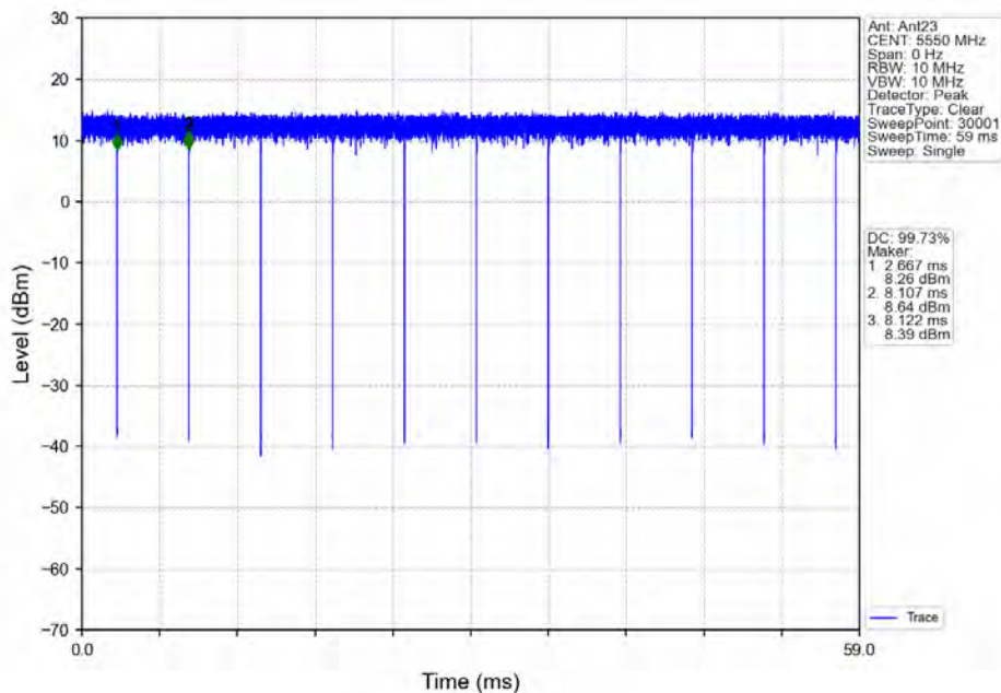
802.11ax(HE40) MCH 5550MHz RU484 Left Ant23 NTNV
