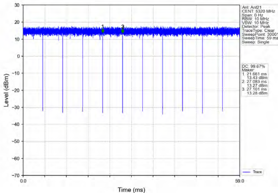
802.11ac(VHT20)_HCH_5320MHz_Ant21_NTNV
