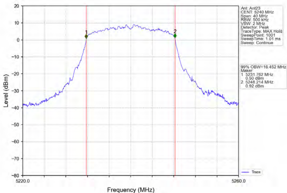
802.11a_HCH_5240MHz_Ant23_NTNV
