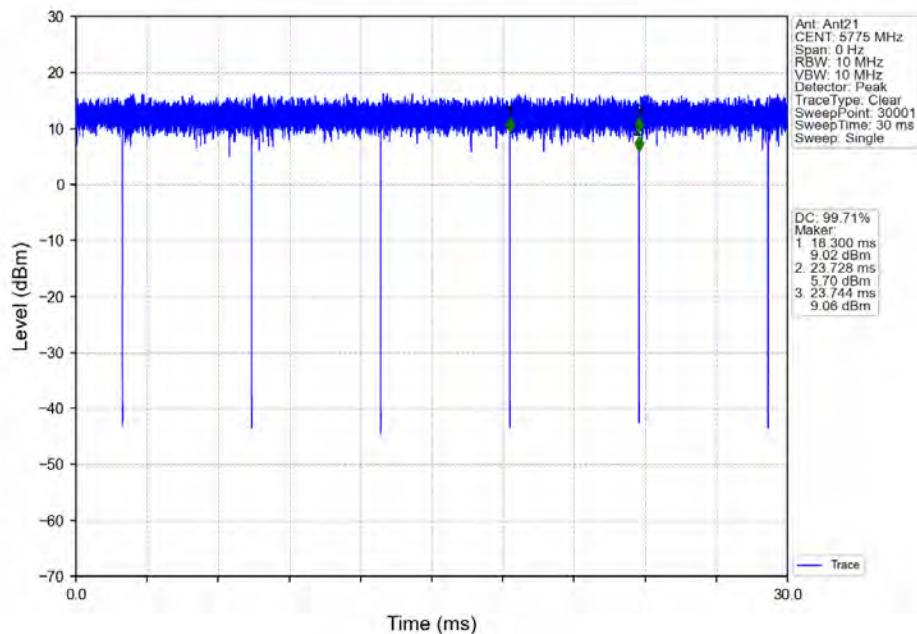
802.11ac(VHT80)_MCH_5775MHz_Ant21_NTNV
