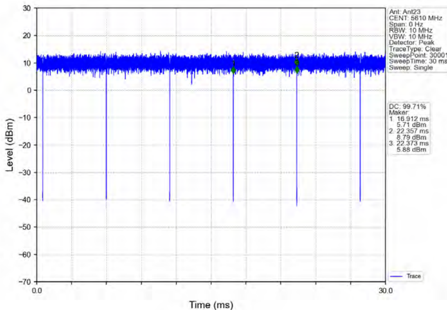
802.11ax(HE80) HCH 5610MHz RU996 Left Ant23 NTN
