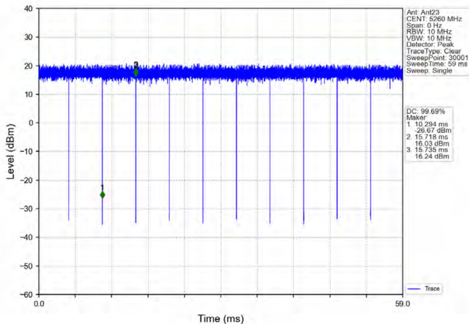
802.11ac(VHT20)_LCH_5260MHz_Ant23_NTNV
