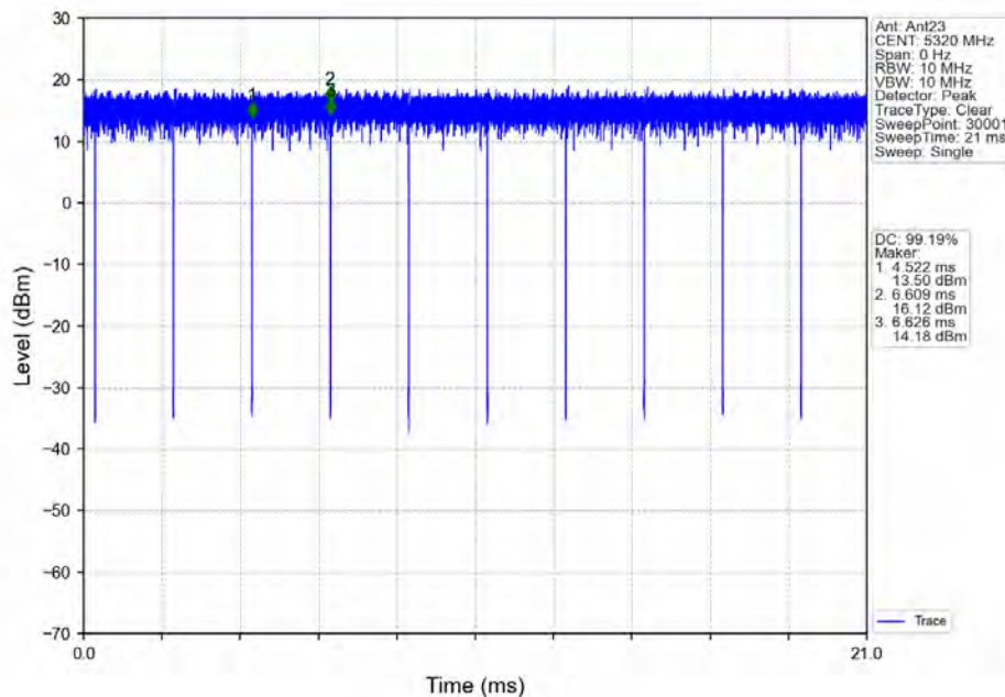
802.11a_HCH_5320MHz_Ant23_NTNV
