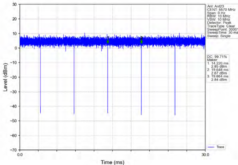
802.11ac(VHT160)_MCH_5570MHz_Ant23_NTNV
