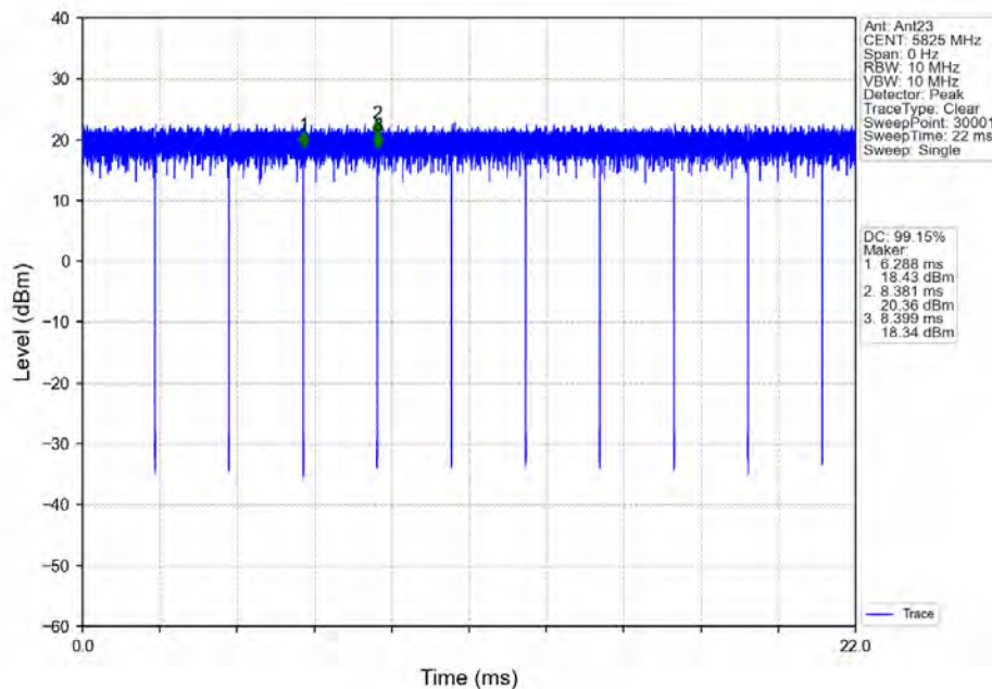
802.11a_HCH_5825MHz_Ant23_NTNV
