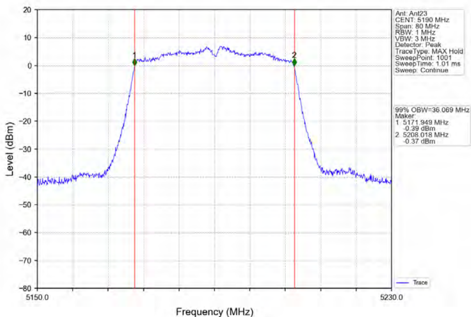
802.11n(HT40) LCH_5190MHz_Ant23_NTNV
