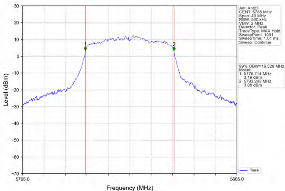
802.11a_MCH_5785MHz_Ant23_NTNV
