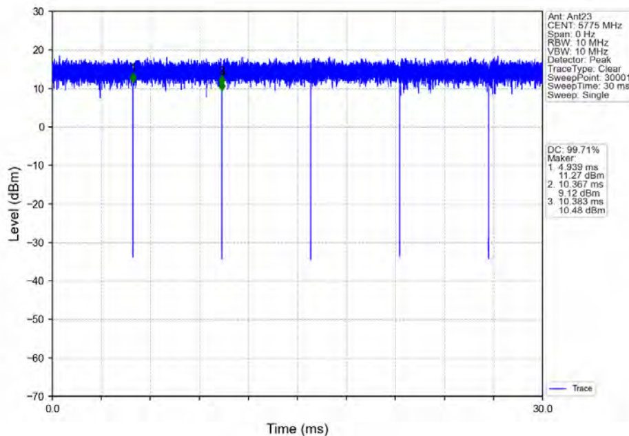
802.11ac(VHT80)_MCH_5775MHz_Ant23_NTNV
