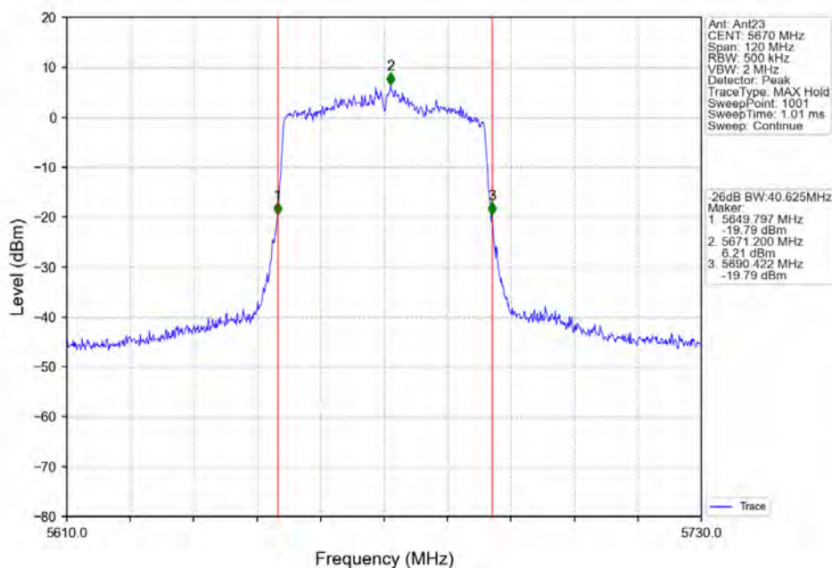
802.11ax(HE40) HCH 5670MHz RU484 Left Ant23 NTN
