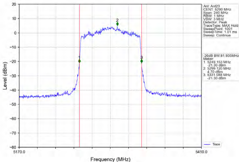
802.11ax(HE80) MCH 5290MHz RU996 Left Ant23 NTVN
