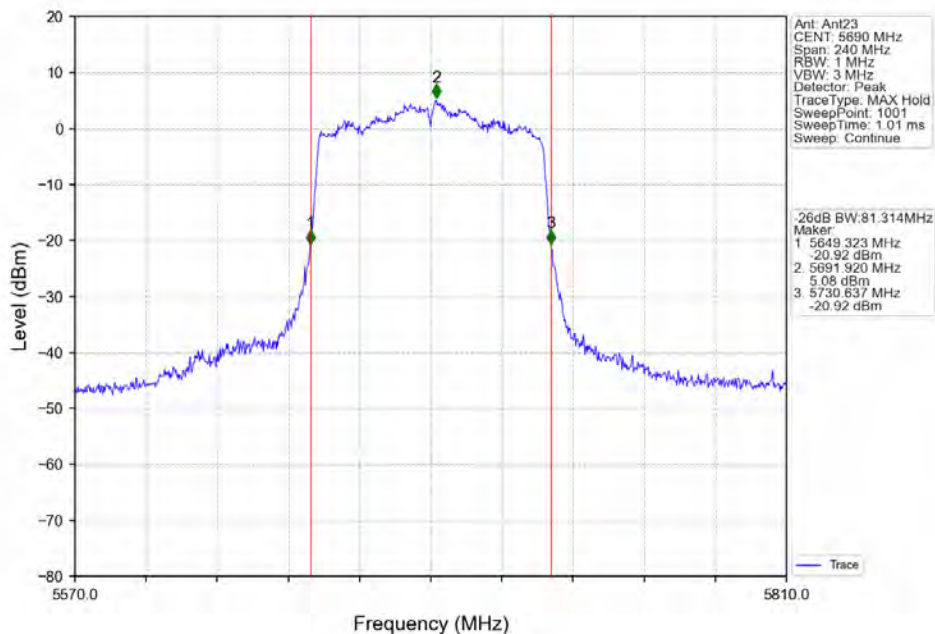
802.11ac(VHT80)_HCH_5690MHz_Ant23_NTNV
