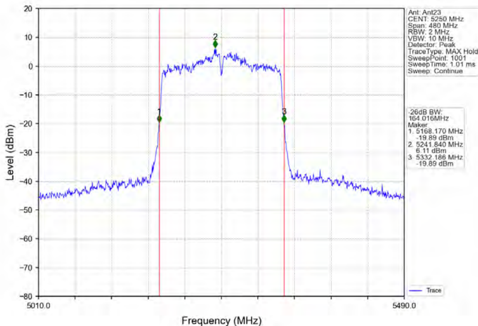
802.11ac(VHT160)_MCH_5250MHz_Ant23_NTNV
