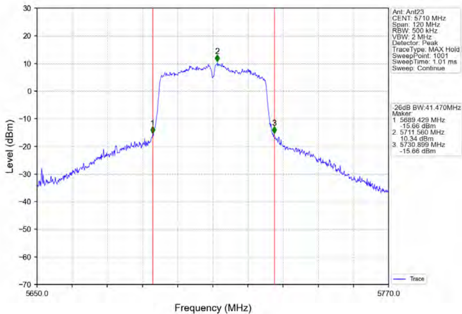
802.11n(HT40) HCH 5710MHz Ant23 NTN
