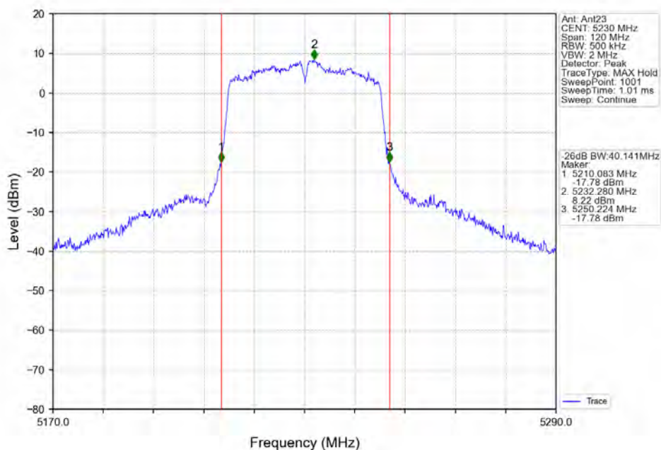
802.11ac(VHT40)_HCH_5230MHz_Ant23_NTNV
