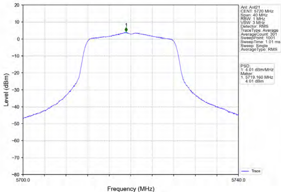
802.11a_HCH_5720MHz_Ant21_NTNV
