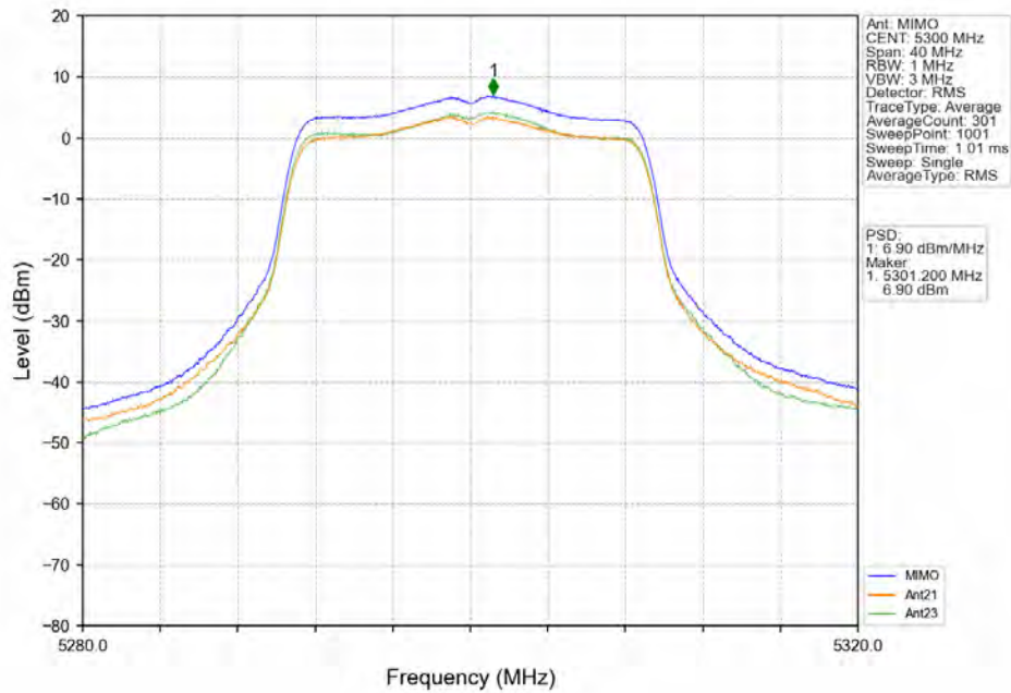
802.11ac(VHT20)_HCH_5320MHz_Ant21_NTNV
