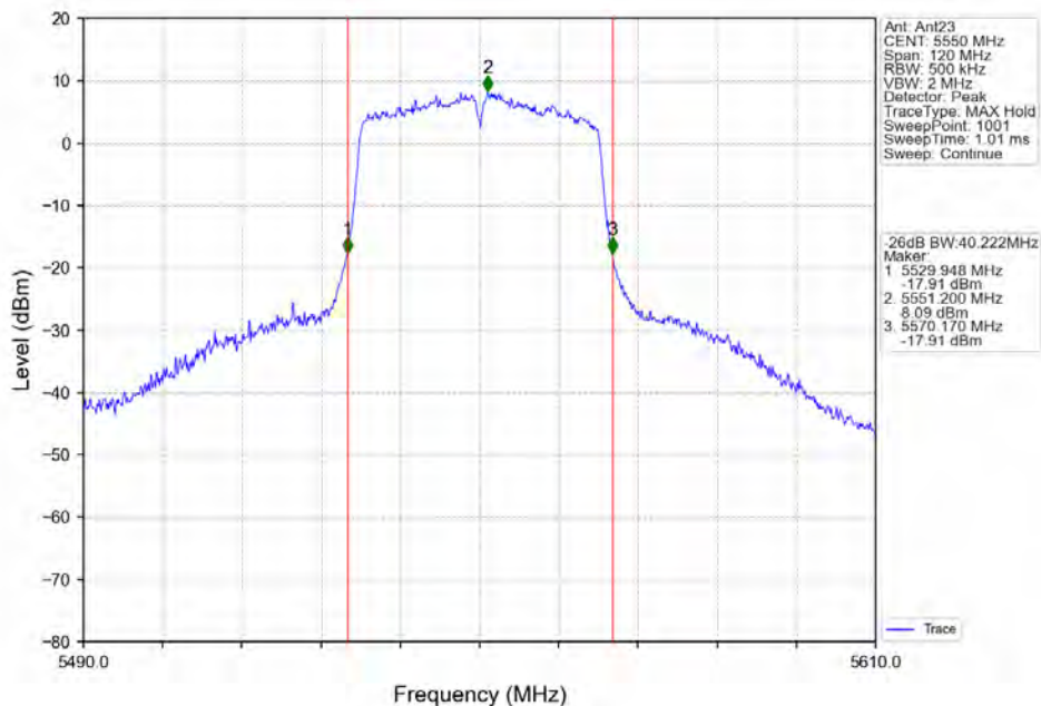
802.11ac(VHT40)_MCH_5550MHz_Ant23_NTNV
