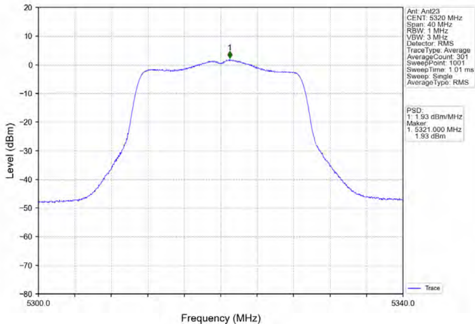
802.11ac(VHT20)_HCH_5320MHz_MIMO_NTNV
