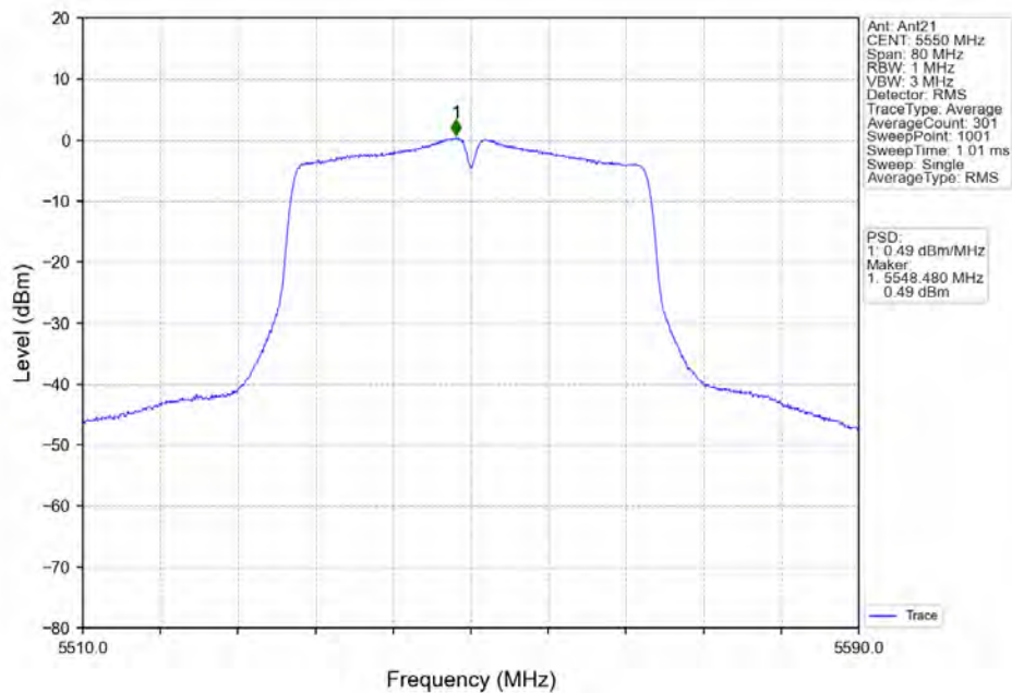
802.11n(HT40) MCH_5550MHz_Ant21_NTNV
