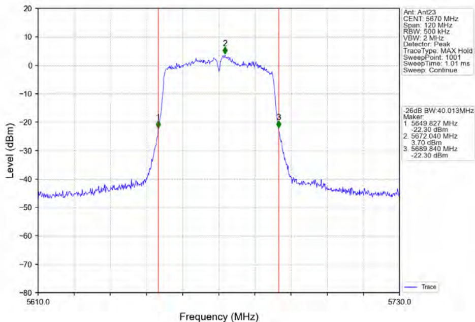
802.11n(HT40) HCH 5670MHz Ant23 NTN
