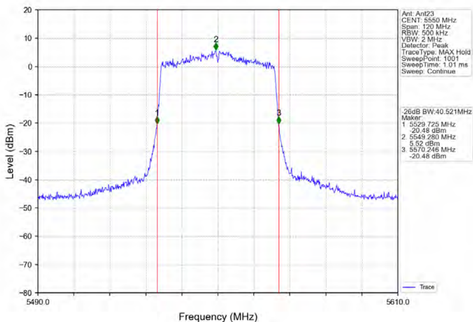
802.11ax(HE40) MCH 5550MHz RU484 Left Ant23 NTVN
