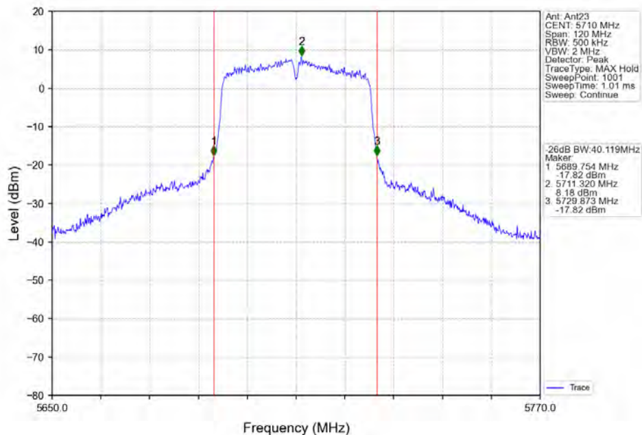
802.11ac(VHT40) HCH_5710MHz_Ant23_NTNV
