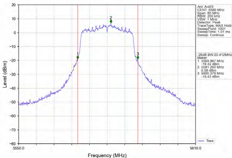
802.11ac(VHT20)_MCH_5580MHz_Ant23_NTNV
