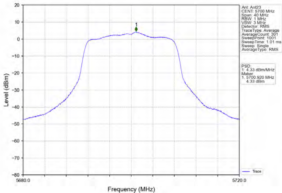
802.11a_HCH_5700MHz_Ant23_NTNV
