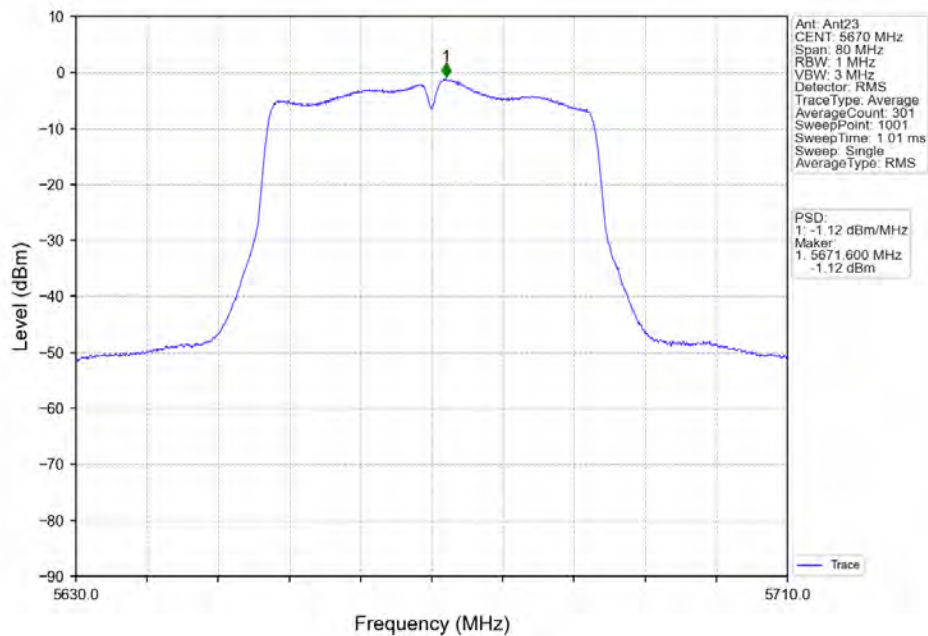
802.11n(HT40) HCH 5670MHz Ant23 NTNV
