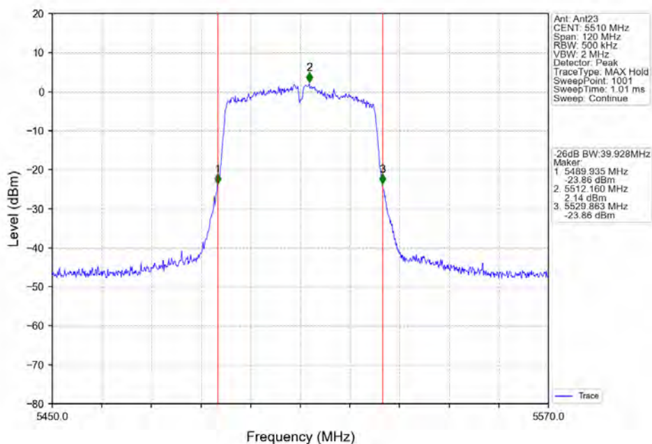
802.11n(HT40) LCH_5510MHz_Ant23_NTNV
