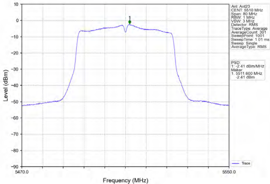
802.11n(HT40) LCH_5510MHz_Ant23_NTNV
