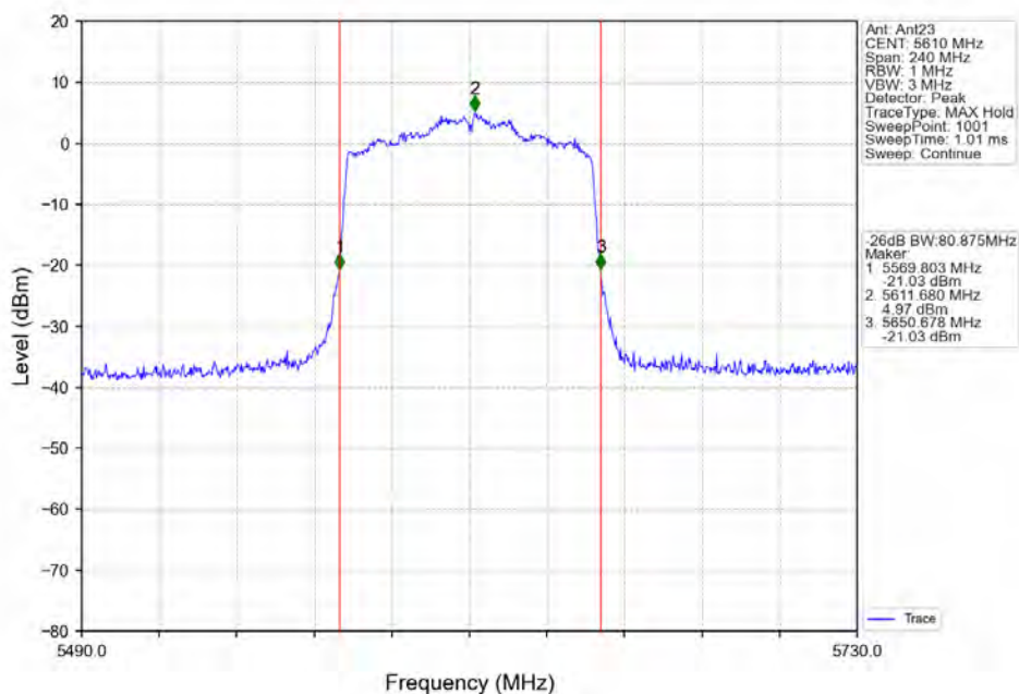
802.11ac(VHT80)_HCH_5610MHz_Ant23_NTNV
