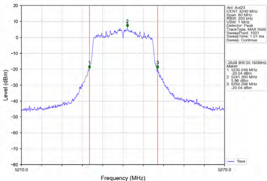
802.11ac(VHT20)_HCH_5240MHz_Ant23_NTNV
