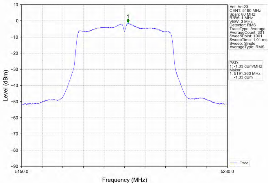
802.11n(HT40) LCH_5190MHz_Ant23_NTNV
