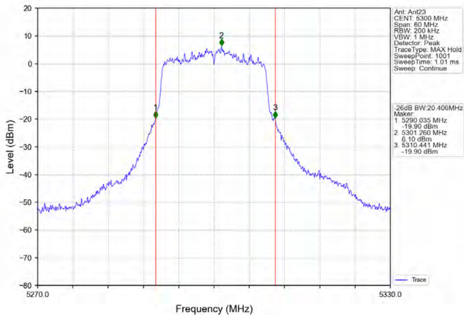
802.11ac(VHT20)_MCH_5300MHz_Ant23_NTNV
