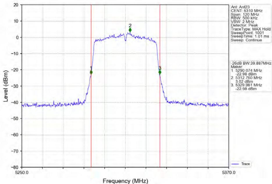
802.11ac(VHT40)_HCH_5310MHz_Ant23_NTNV
