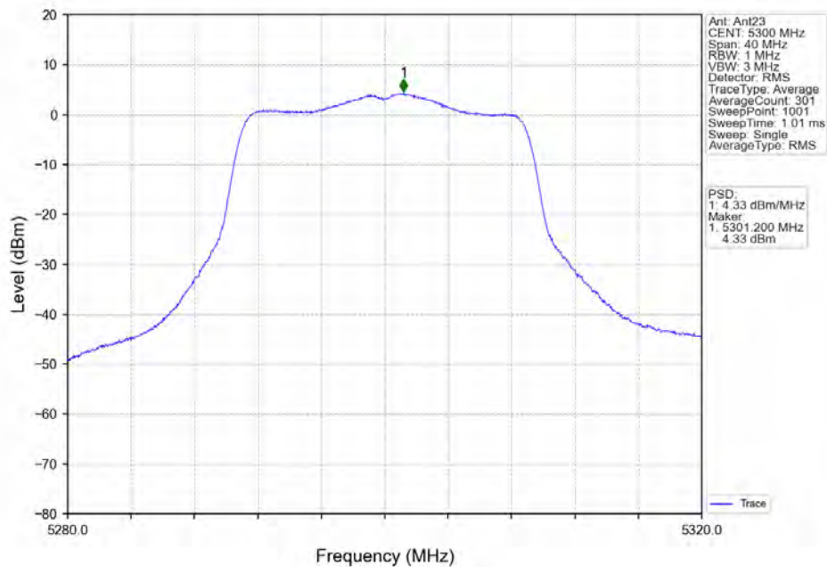
802.11ac(VHT20)_MCH_5300MHz_Ant23_NTNV
