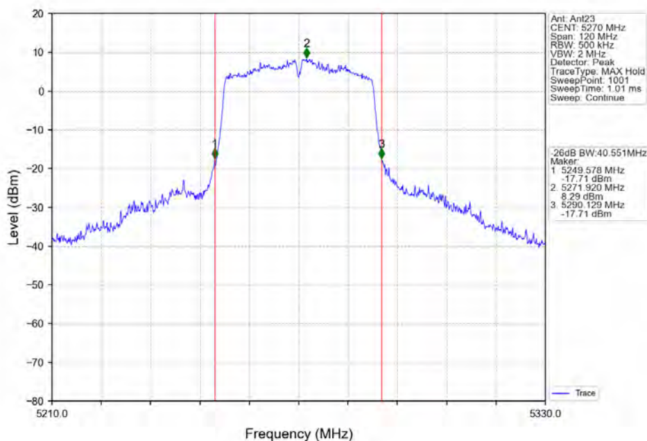
802.11ac(VHT40)_LCH_5270MHz_Ant23_NTNV
