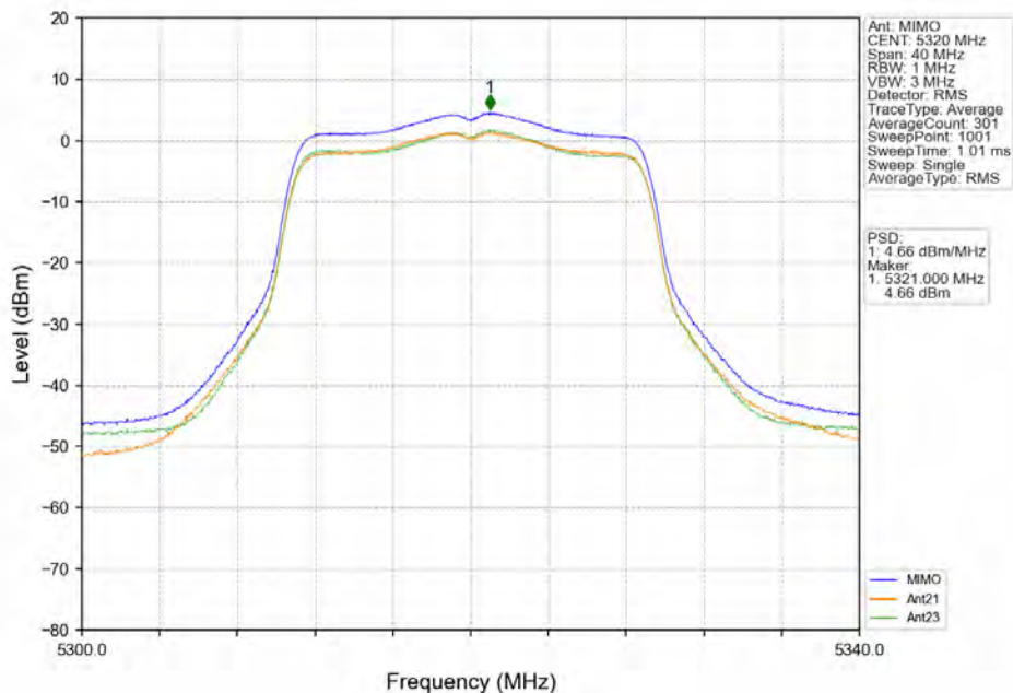
802.11ac(VHT20)_HCH_5320MHz_MIMO_NTNV
