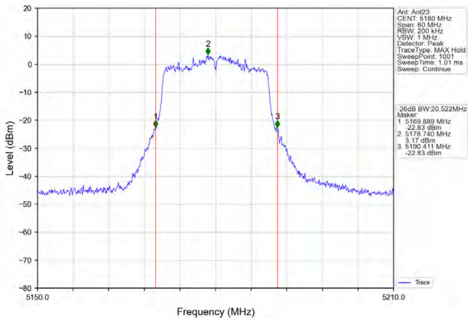
802.11ac(VHT20)_LCH_5180MHz_Ant23_NTNV
