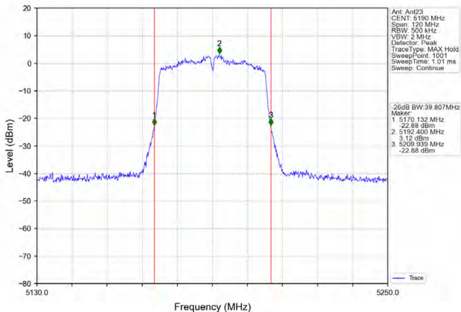
802.11ac(VHT40)_LCH_5190MHz_Ant23_NTNV
