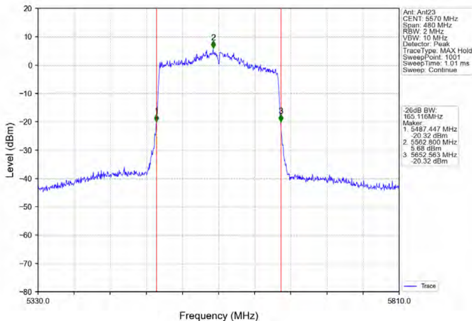
802.11ax(HE160) MCH_5570MHz 2xRU996 Left Ant23 NTN
