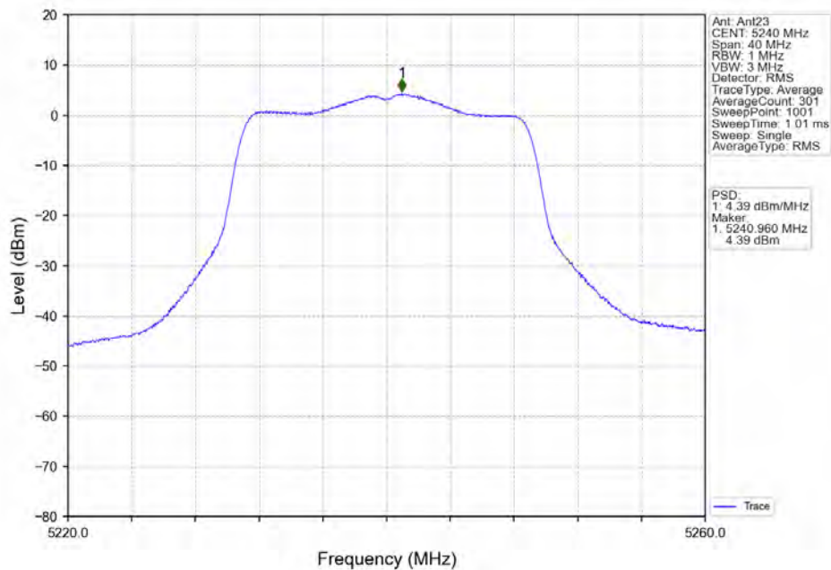
802.11ac(VHT20) HCH_5240MHz_Ant23_NTNV
