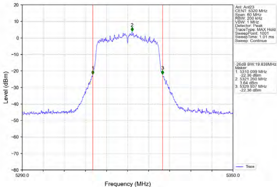
802.11ac(VHT20)_HCH_5320MHz_Ant23_NTNV
