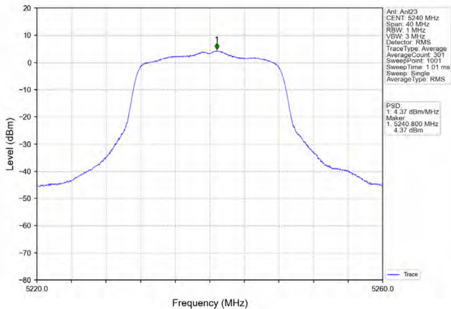
802.11a_HCH_5240MHz_Ant23_NTNV
