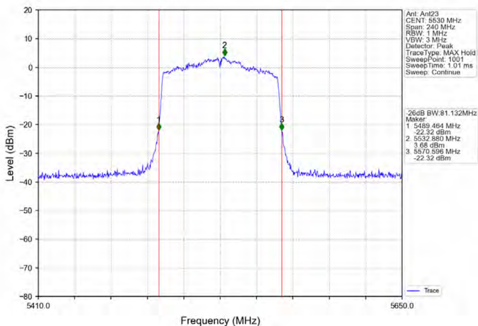
802.11ac(VHT80)_LCH_5530MHz_Ant23_NTNV
