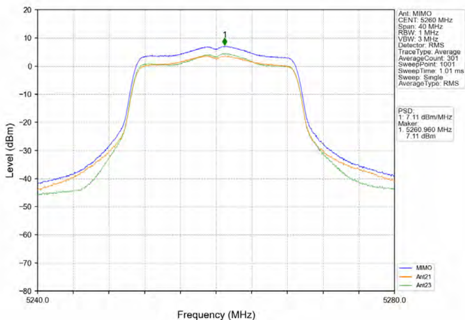
802.11ac(VHT20)_LCH_5260MHz_MIMO_NTNV
