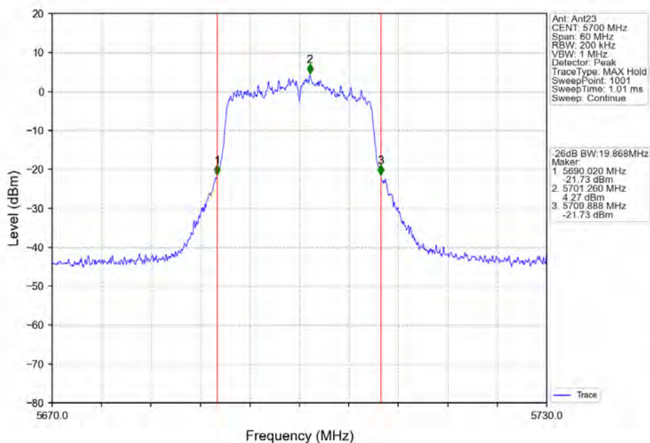
802.11ac(VHT20)_HCH_5700MHz_Ant23_NTNV
