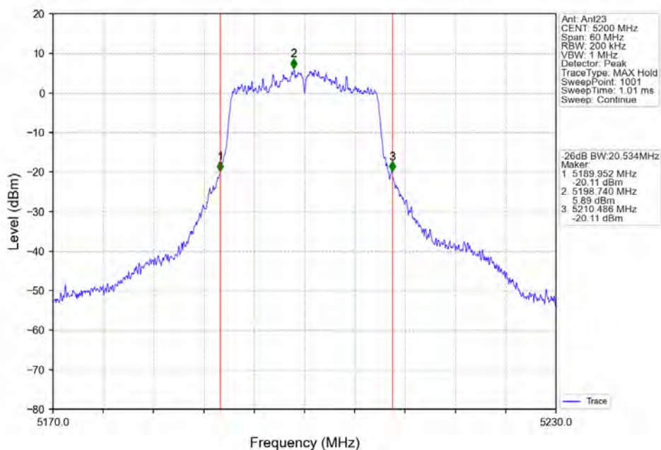
802.11ac(VHT20)_MCH_5200MHz_Ant23_NTNV
