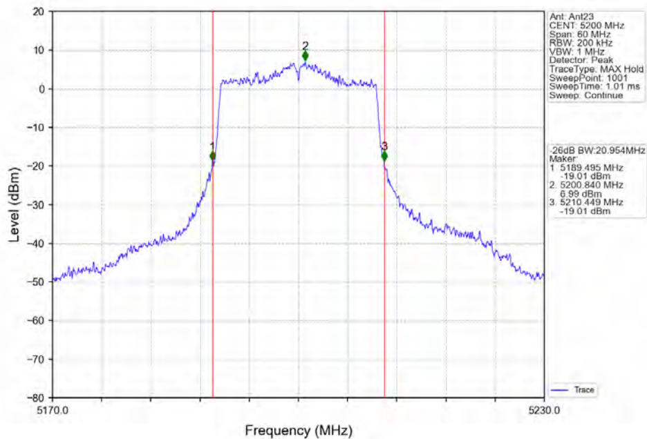
802.11ax(HE20) MCH 5200MHz RU242 Left Ant23 NTN
