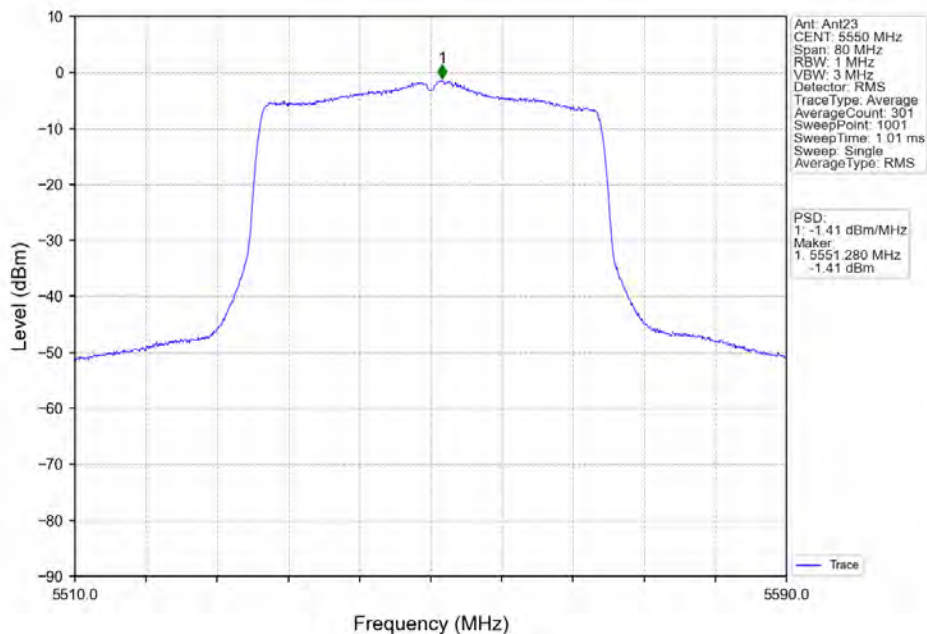
802.11ax(HE40) MCH 5550MHz RU484 Left Ant23 NTVN
