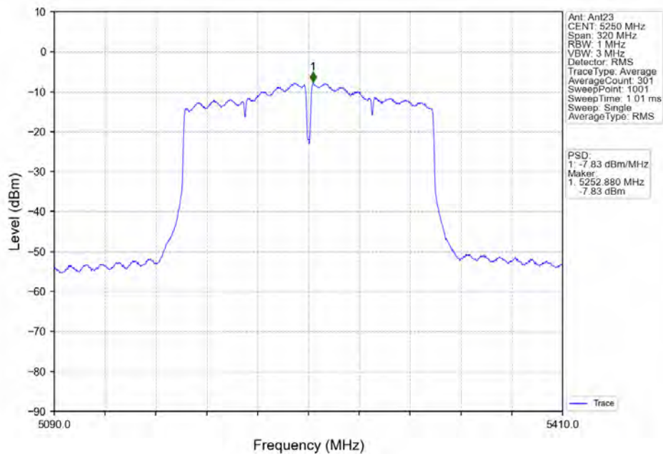
802.11ac(VHT160)_MCH_5250MHz_Ant23_NTNV
