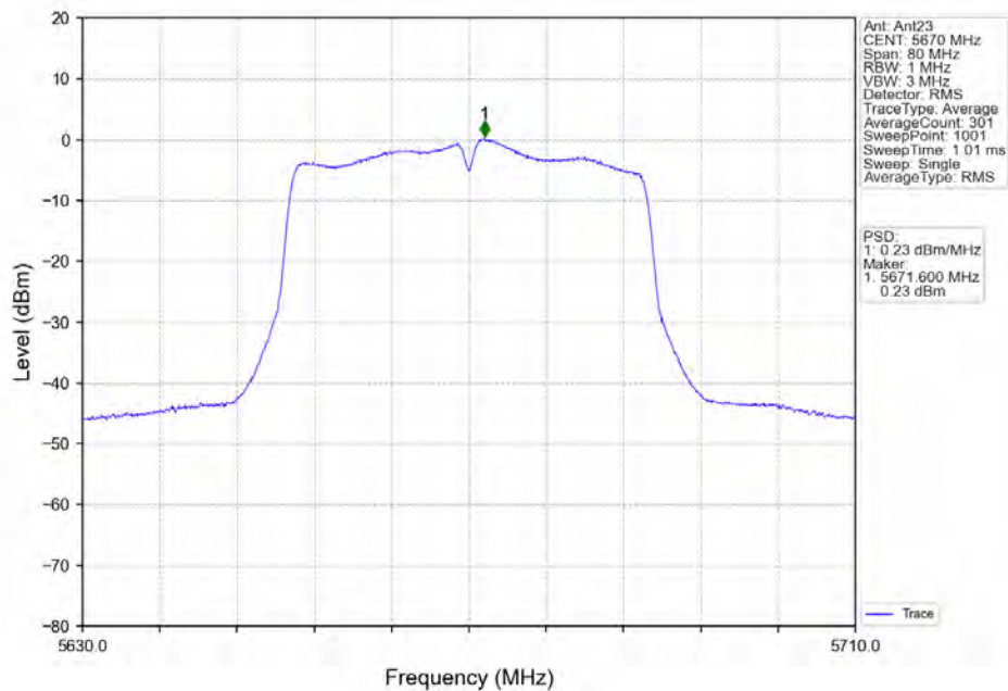
802.11ac(VHT40)_HCH_5670MHz_Ant23_NTNV
