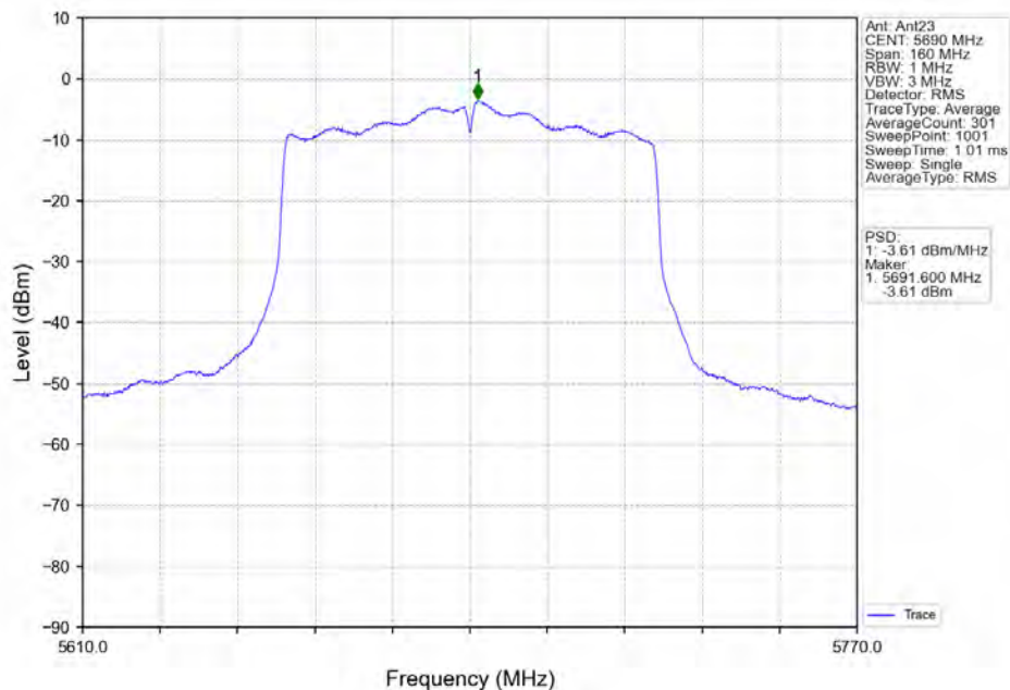
802.11ac(VHT80)_HCH_5690MHz_Ant23_NTNV
