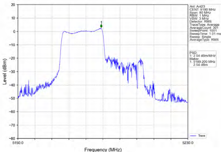
802.11ax(HE40) LCH_5190MHz_RU242_Left_MIMO_NTNV
