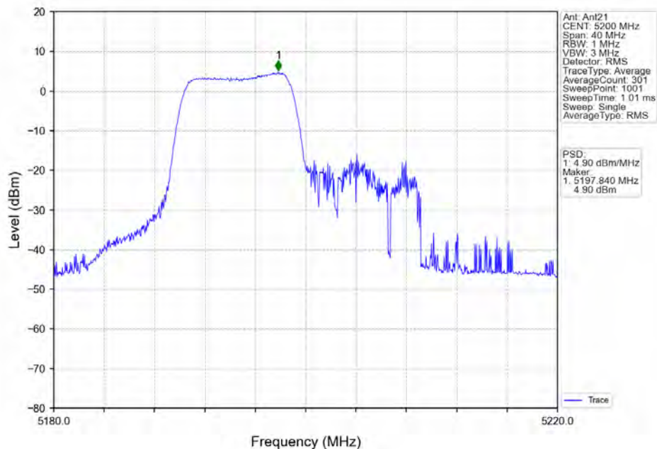
802.11ax(HE20) MCH 5200MHz RU106 Left Ant21_NTNV
