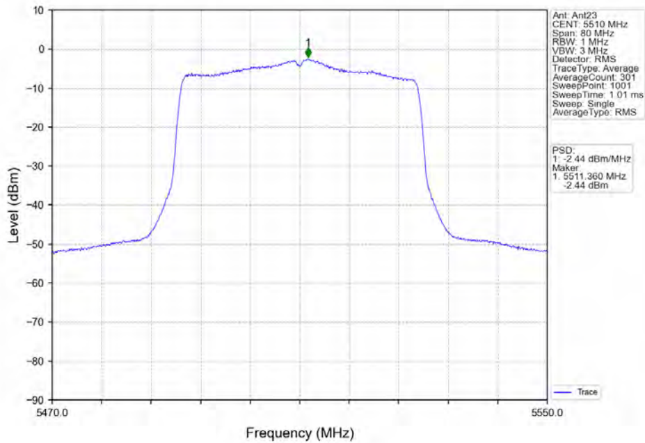
802.11ax(HE40) LCH_5510MHz RU484 Left MIMO_NTNV
