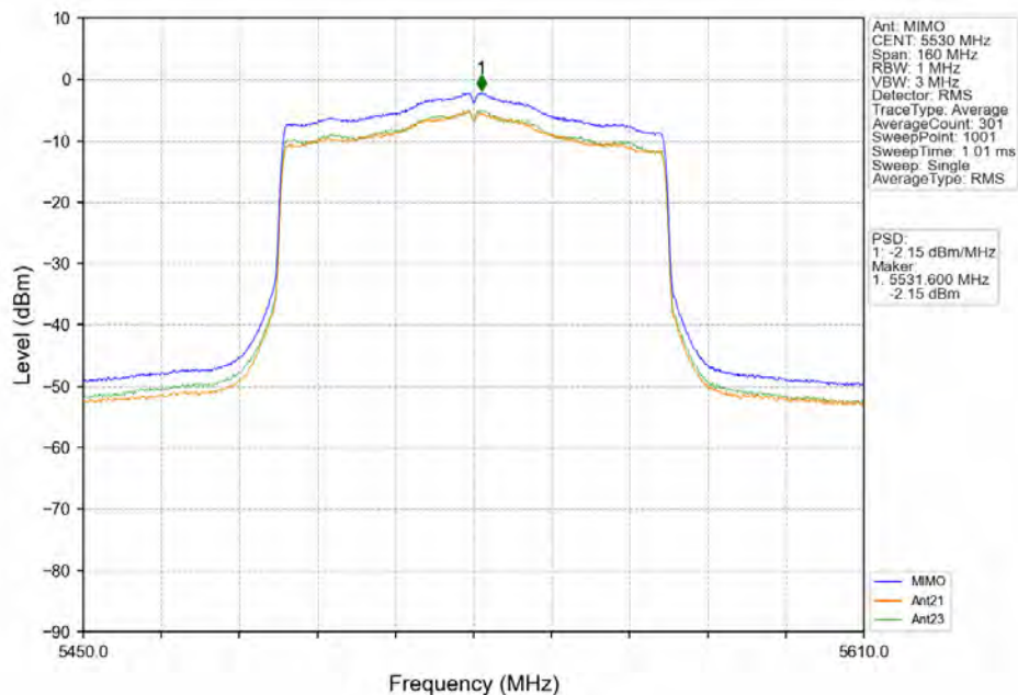
802.11ax(HE80) LCH_5530MHz RU996 Left MIMO_NTNV
