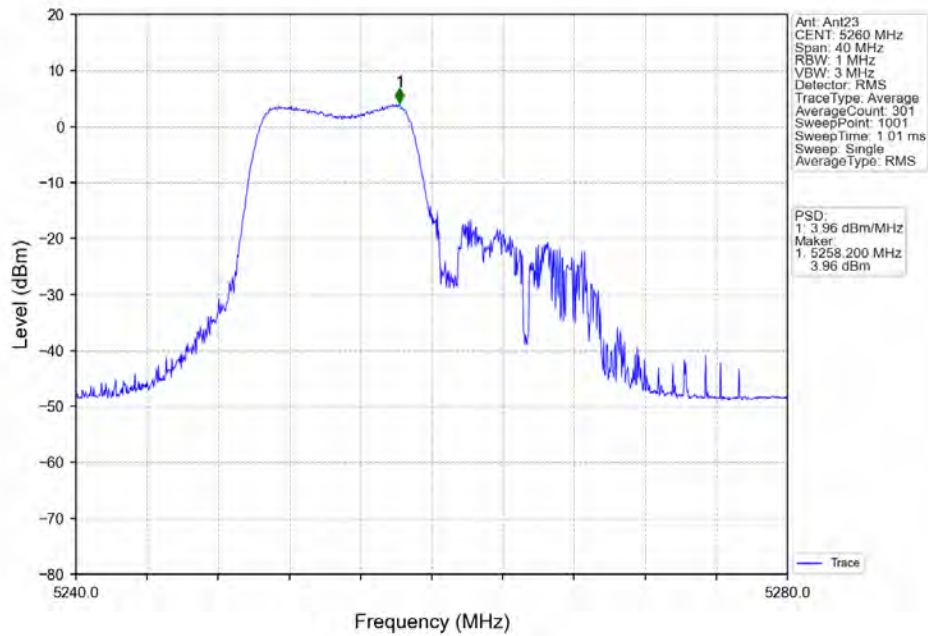
802.11ax(HE20) LCH_5260MHz_RU106_Left_MIMO_NTNV
