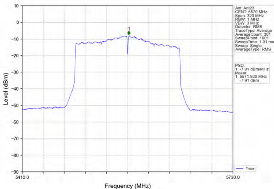
802.11ax(HE160) MCH_5570MHz 2xRU996 Left Ant23 NTN
