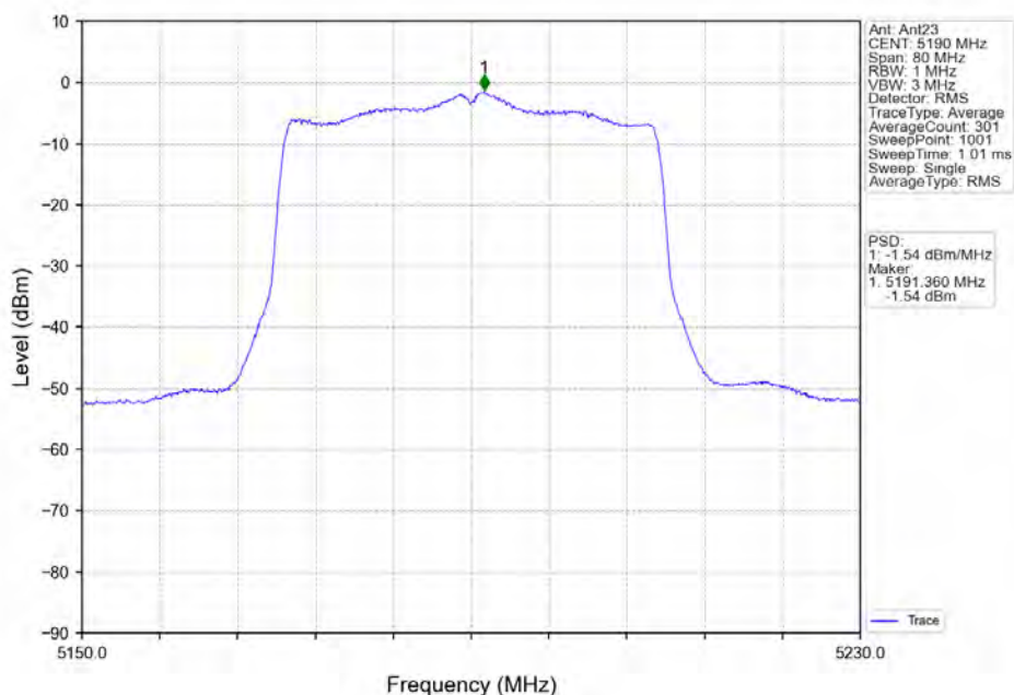
802.11ax(HE40) LCH_5190MHz RU484 Left MIMO_NTNV
