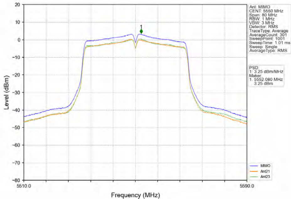
802.11ac(VHT40)_MCH_5550MHz_MIMO_NTNV
