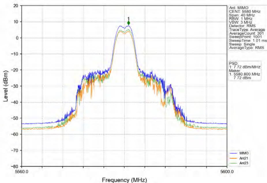
802.11ax(HE20) MCH 5580MHz RU26 Mid_MIMO_NTNV
