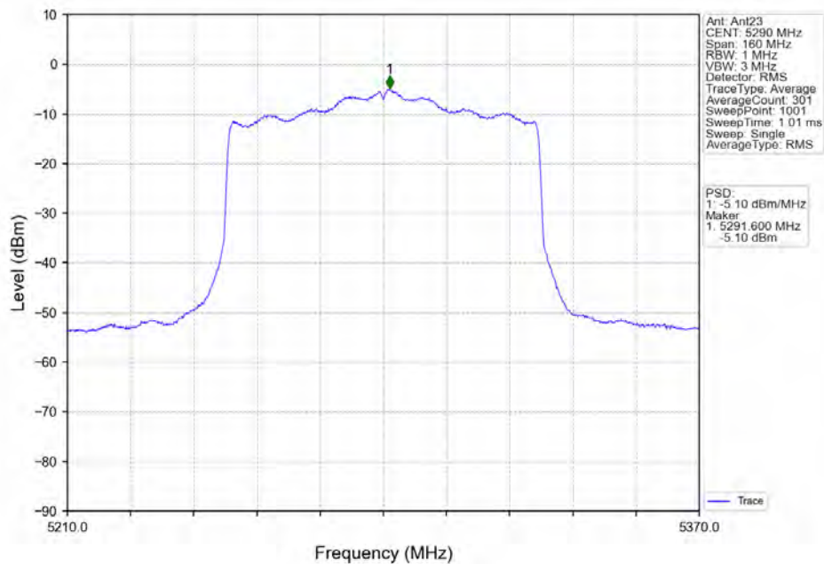
802.11ax(HE80) MCH 5290MHz RU996 Left Ant23 NTVN
