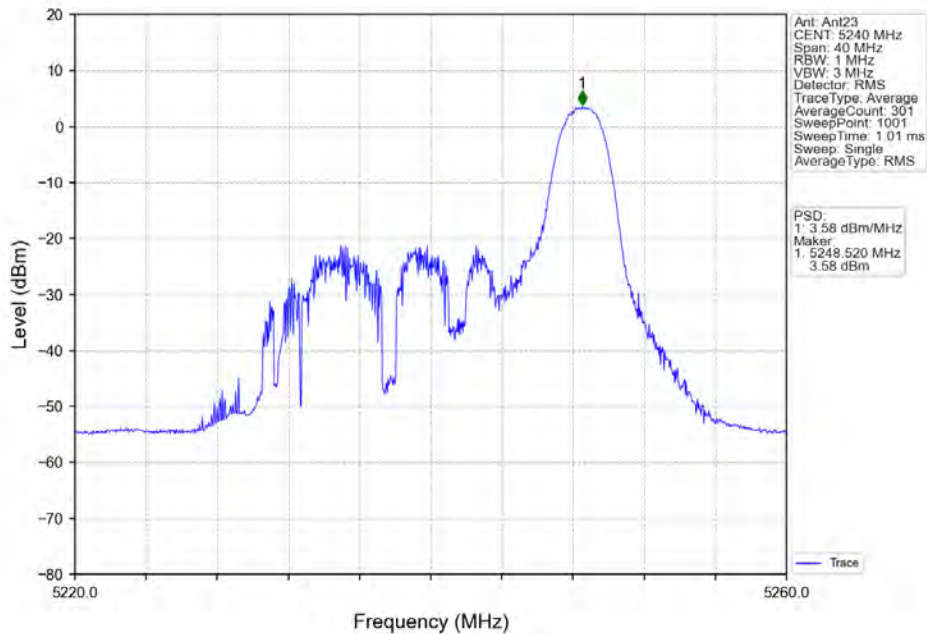
802.11ax(HE20) HCH 5240MHz RU26 Right Ant23 NTNV
