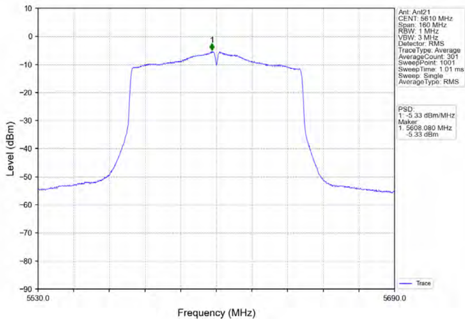
802.11ac(VHT80)_HCH_5610MHz_Ant21_NTNV
