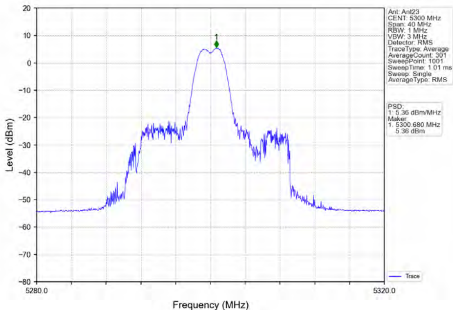
802.11ax(HE20) MCH 5300MHz RU26 Mid_Ant23_NTNV
