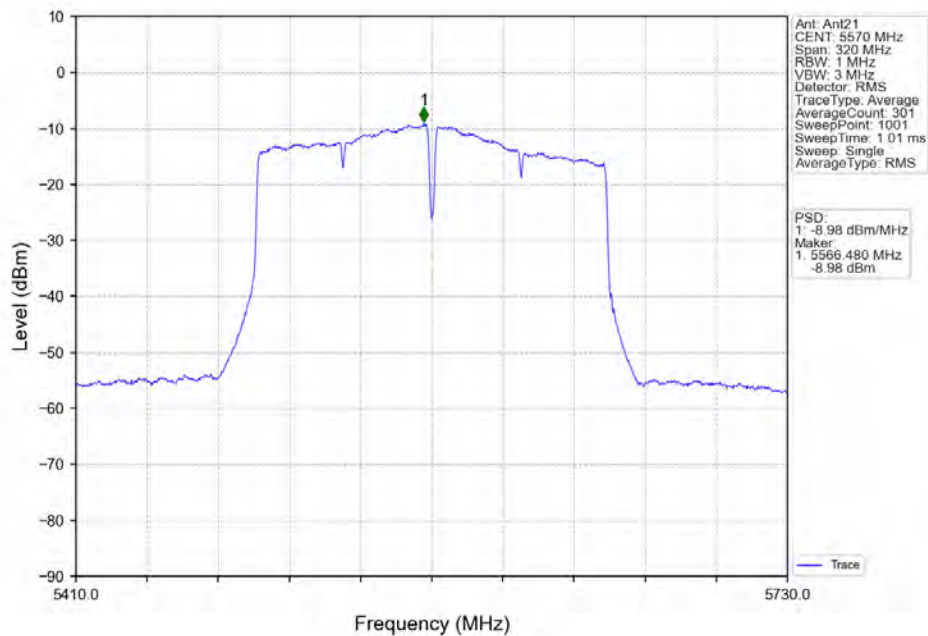
802.11ac(VHT160) MCH_5570MHz_Ant21_NTNV
