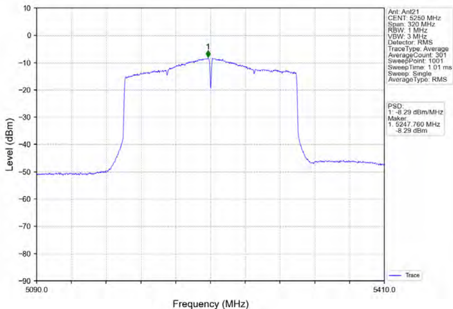
802.11ax(HE160) MCH_5250MHz_2xRU996 Left Ant21 NTN
