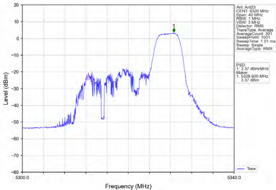
802.11ax(HE20) HCH_5320MHz RU52 Right Ant23 NTVN
