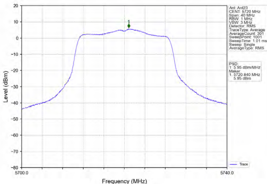
802.11ac(VHT20)_HCH_5720MHz_MIMO_NTNV
