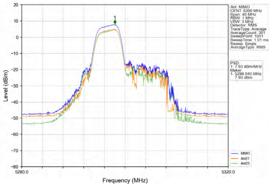
802.11ax(HE20) MCH 5300MHz RU52 Mid_MIMO_NTNV
