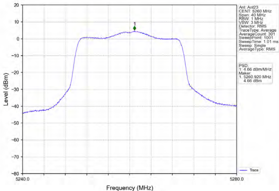
802.11ax(HE20) LCH_5260MHz RU242 Left Ant23_NTNV
