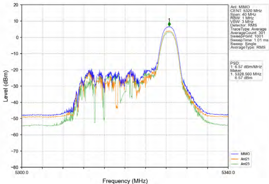
802.11ax(HE20) HCH_5320MHz_RU26_Right_MIMO_NTNV
