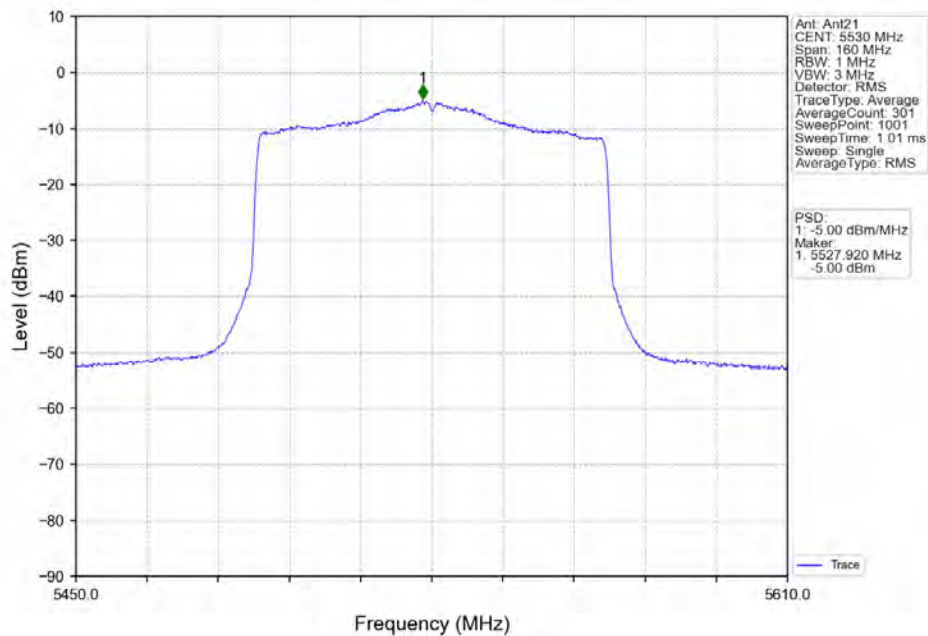
802.11ax(HE80) LCH 5530MHz RU996 Left Ant21 NTN
