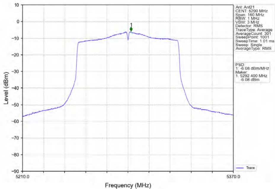
802.11ac(VHT80)_MCH_5290MHz_Ant21_NTNV
