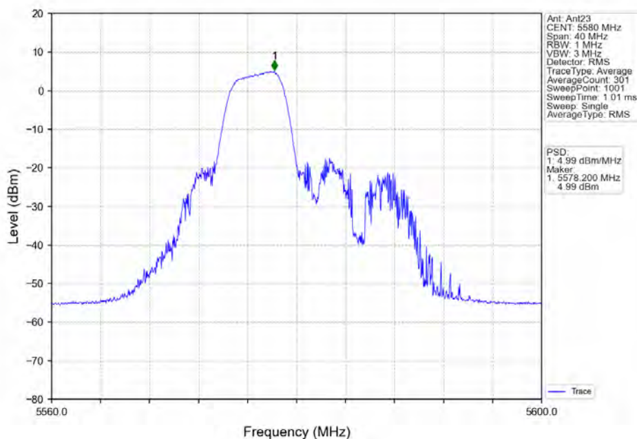
802.11ax(HE20) MCH 5580MHz RU52 Mid_Ant23_NTNV
