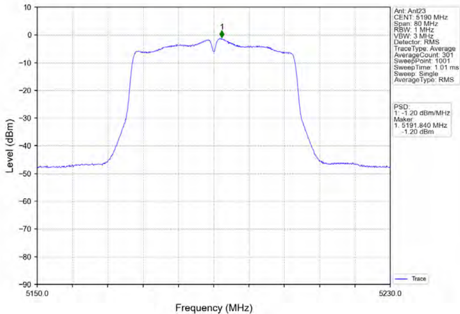
802.11ac(VHT40)_LCH_5190MHz_Ant23_NTNV
