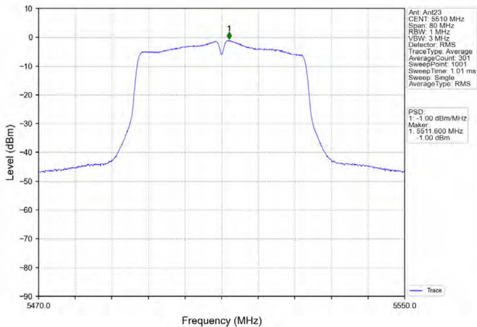
802.11ac(VHT40)_LCH_5510MHz_Ant23_NTNV
