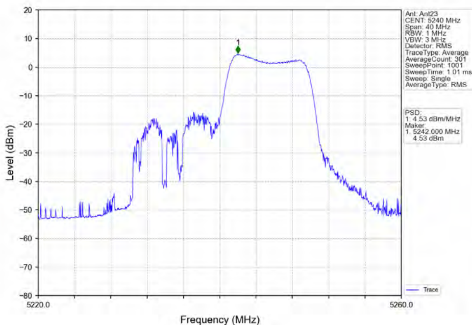
802.11ax(HE20) HCH 5240MHz RU106 Right_Ant23 NTN
