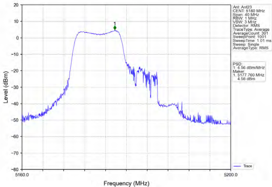
802.11ax(HE20) LCH_5180MHz_RU106_Left_Ant23_NTNV
