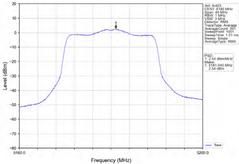
802.11ax(HE20) LCH_5180MHz_RU242_Left_MIMO_NTNV
