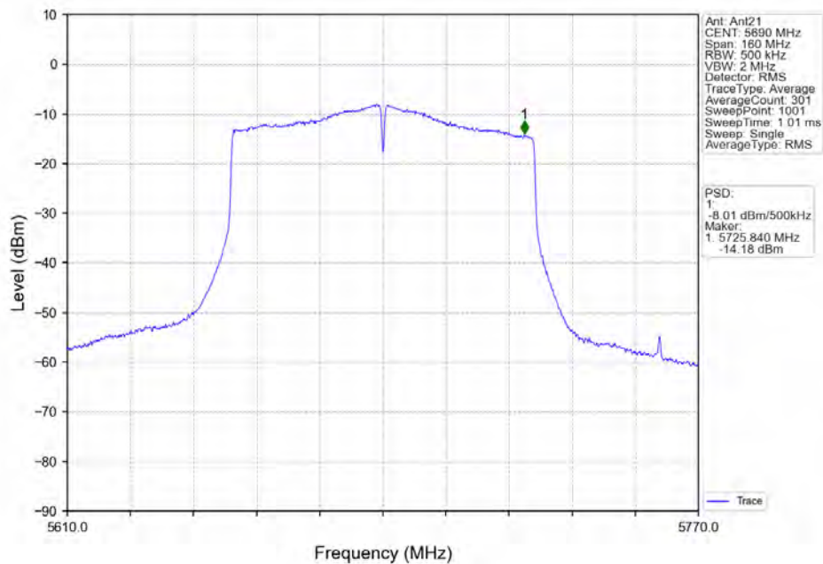
802.11ac(VHT80)_HCH_5690MHz_Ant21_NTNV
