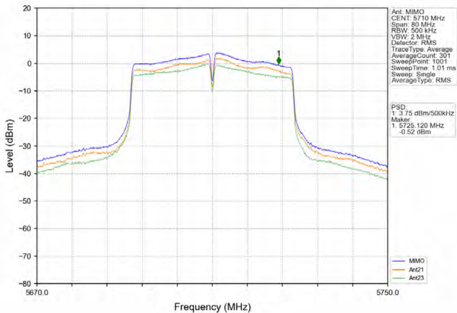
802.11ac(VHT40) HCH_5710MHz_MIMO_NTNV
