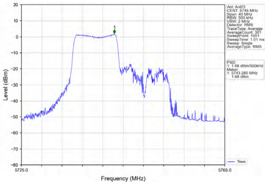
802.11ax(HE20) LCH_5745MHz_RU106_Left_Ant23_NTNV
