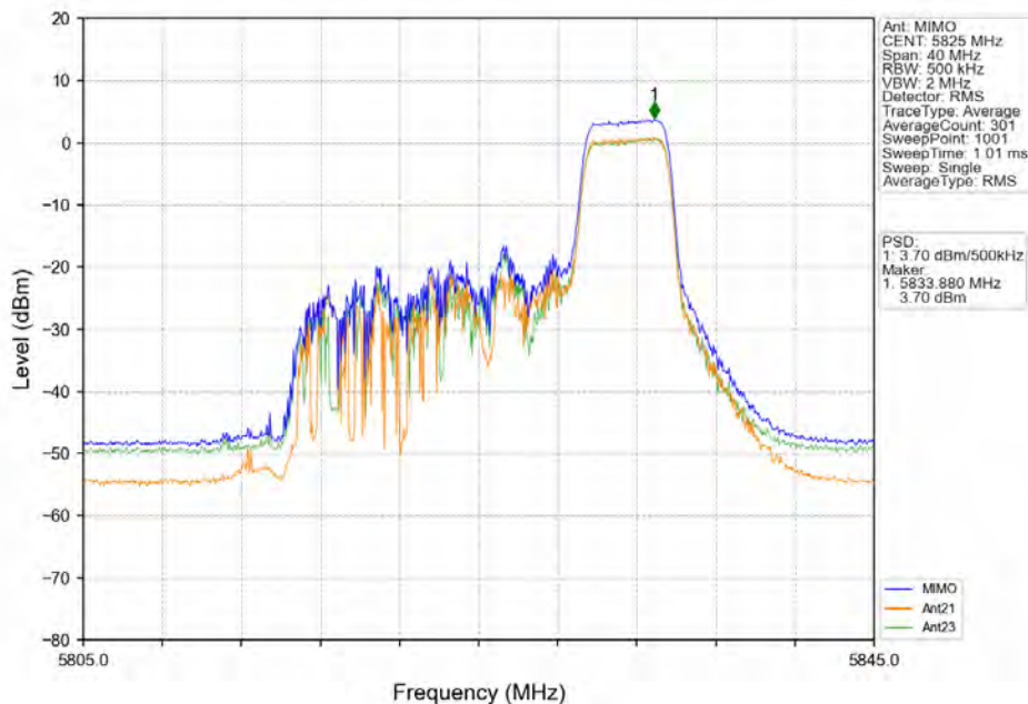
802.11ax(HE20) HCH_5825MHz_RU52_Right_MIMO_NTNV
