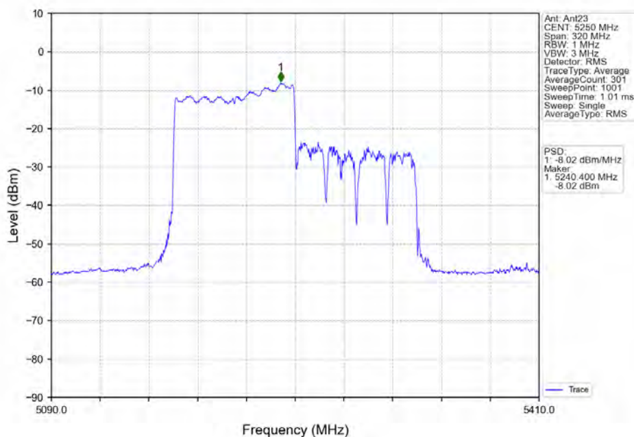
802.11ax(HE160) MCH 5250MHz RU996 Left Ant23 NTN
