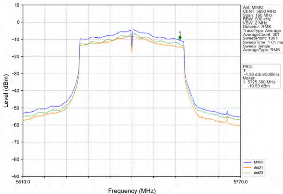
802.11ac(VHT80)_HCH_5690MHz_MIMO_NTNV
