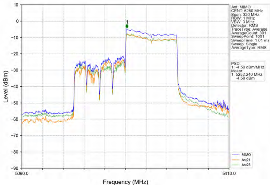
802.11ax(HE160)_MCH_5250MHz_RU996_Right_MIMO_NTNV
