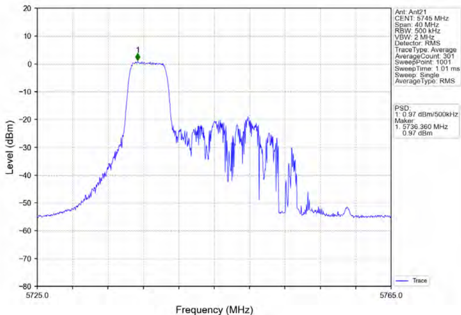
802.11ax(HE20) LCH 5745MHz RU52 Left Ant21 NTN
