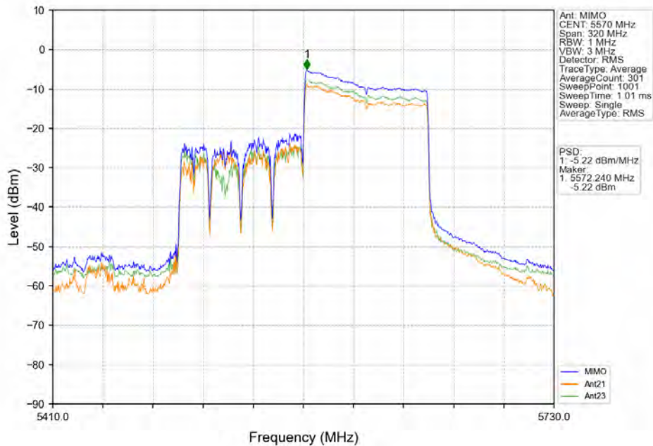
802.11ax(HE160) MCH 5570MHz RU996 Right MIMO NTN
