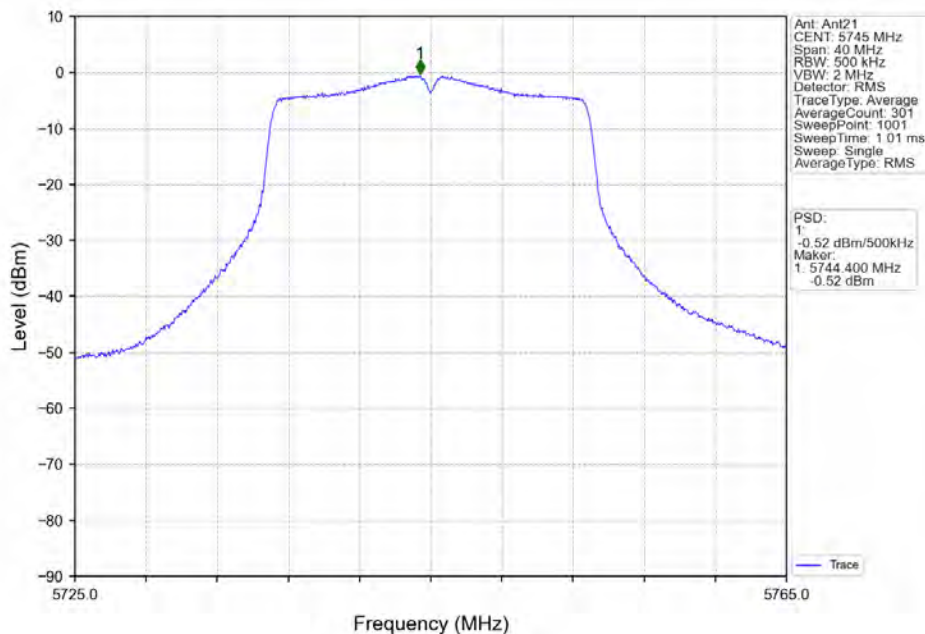
802.11ac(VHT20)_LCH_5745MHz_Ant21_NTNV
