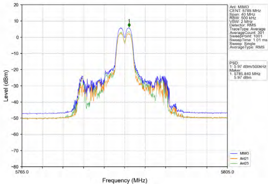
802.11ax(HE20) MCH 5785MHz RU26 Mid_MIMO_NTNV
