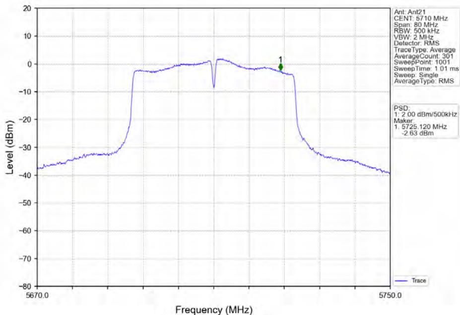
802.11ac(VHT40) HCH_5710MHz_Ant21_NTNV
