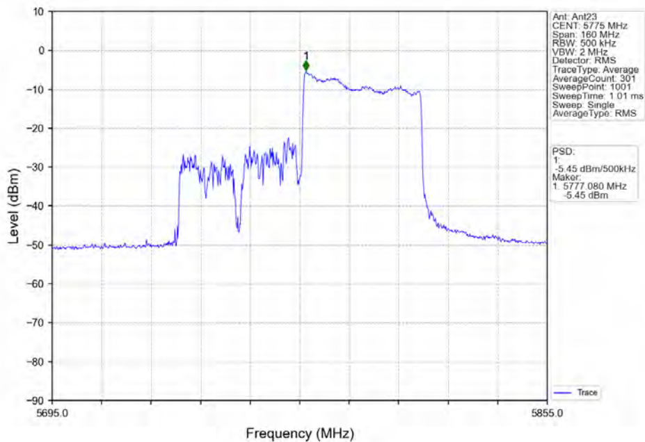
802.11ax(HE80) MCH 5775MHz RU484 Right Ant23 NTN
