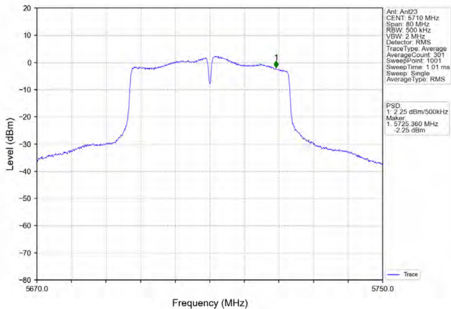
802.11n(HT40) HCH 5710MHz Ant23 NTN
