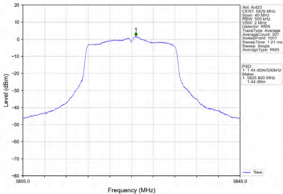
802.11a_HCH_5825MHz_Ant23_NTNV
