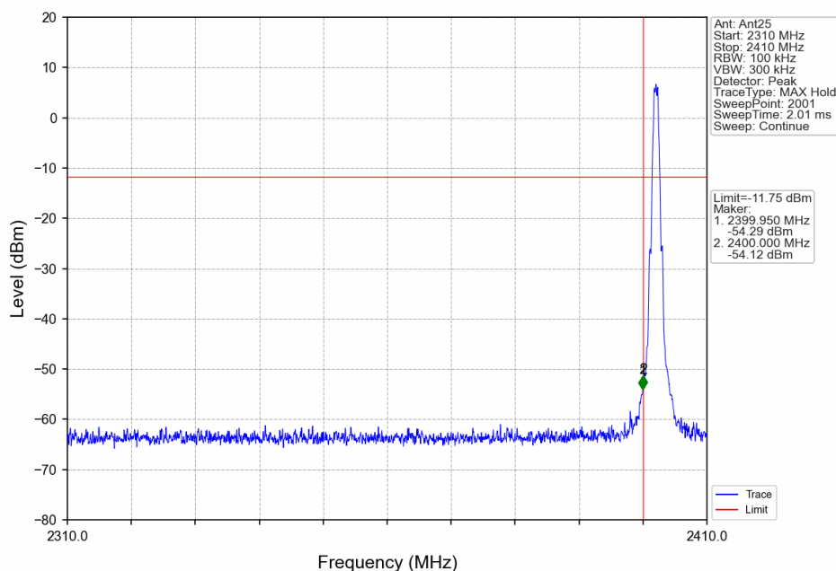
1M_LCH_2402MHz_Ant25_NTNV
