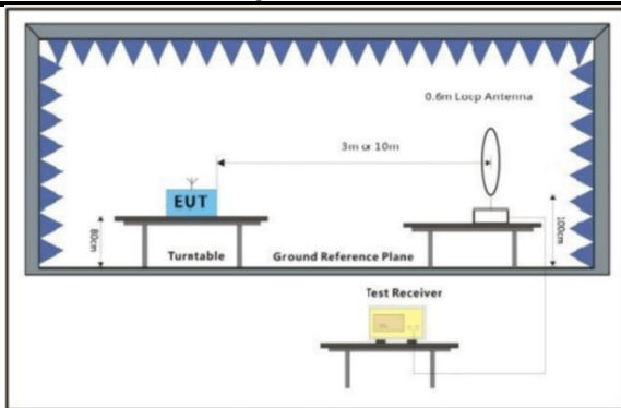
Figure 1. Below 30MHz
