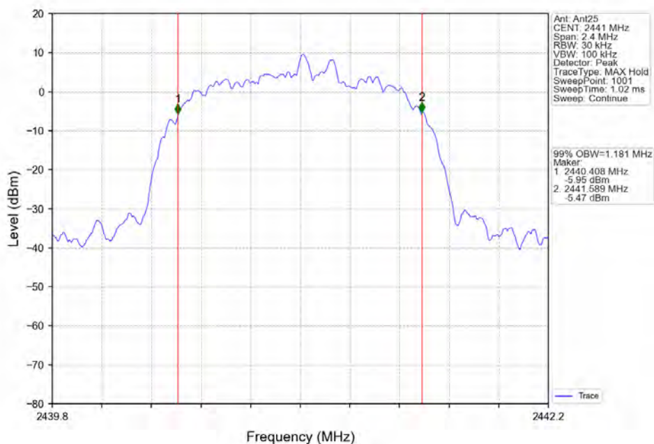
8DPSK_3DH5_MCH_2441MHz_Ant25_NTNV
