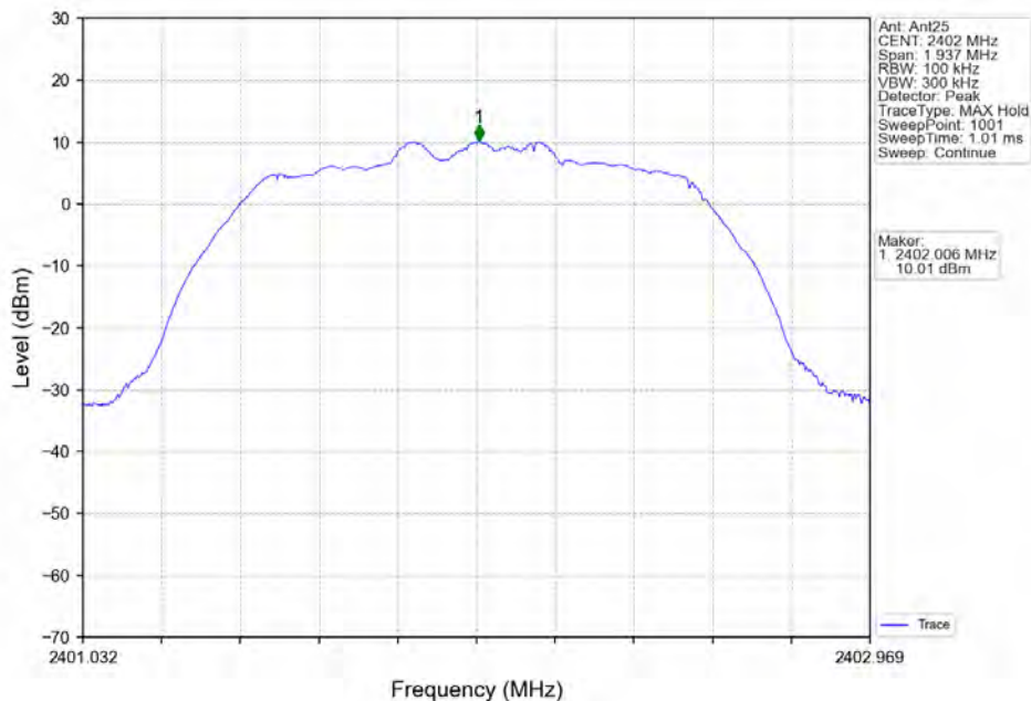
Pi/4DQPSK_2DH5_LCH_2402MHz_Ant25_NTNV
