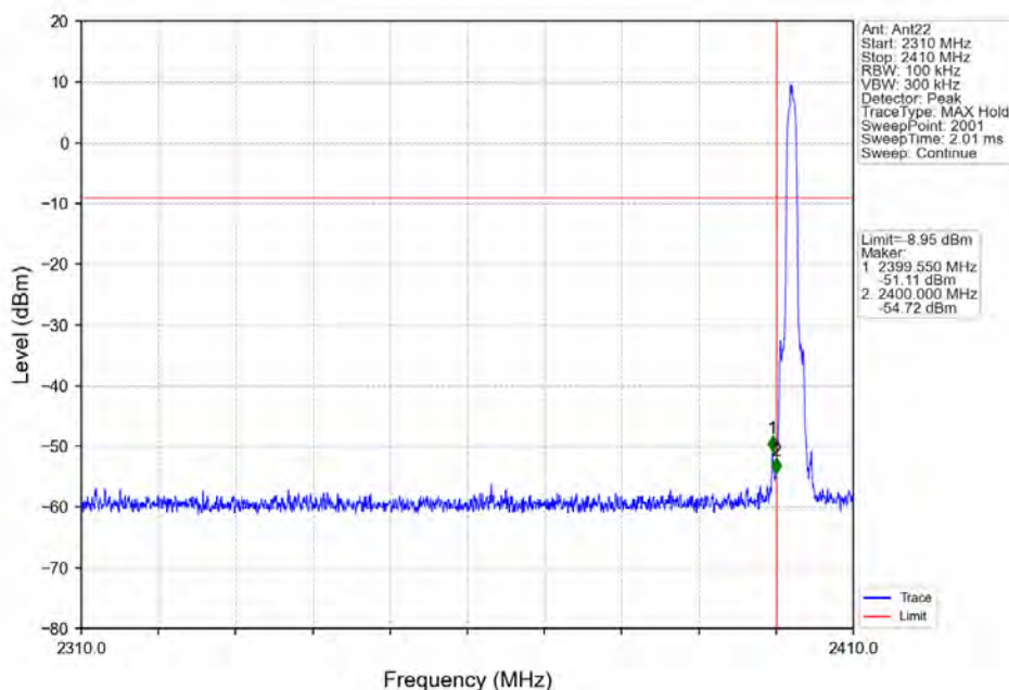
Pi/4DQPSK 2DH5 LCH 2402MHz Ant22 NTNV
