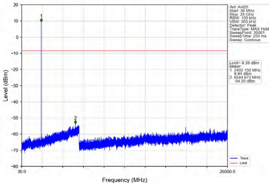
GFSK_DH5_LCH_2402MHz_Ant25_NTNV
