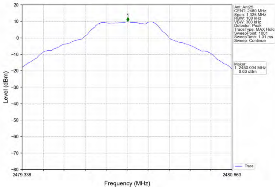
GFSK_DH5_HCH_2480MHz_Ant25_NTNV
