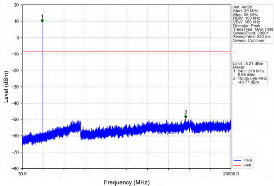
8DPSK_3DH5_LCH_2402MHz_Ant25_NTNV
