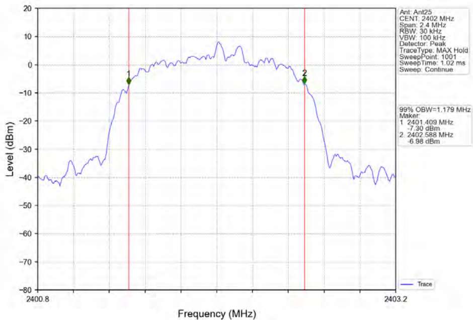
8DPSK_3DH5_LCH_2402MHz_Ant25_NTNV
