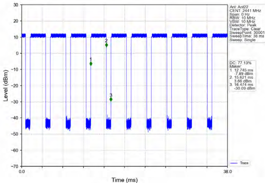
8DPSK_3DH5_MCH_2441MHz_Ant22_NTNV
