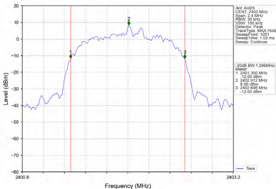
8DPSK_3DH5_LCH_2402MHz_Ant25_NTNV
