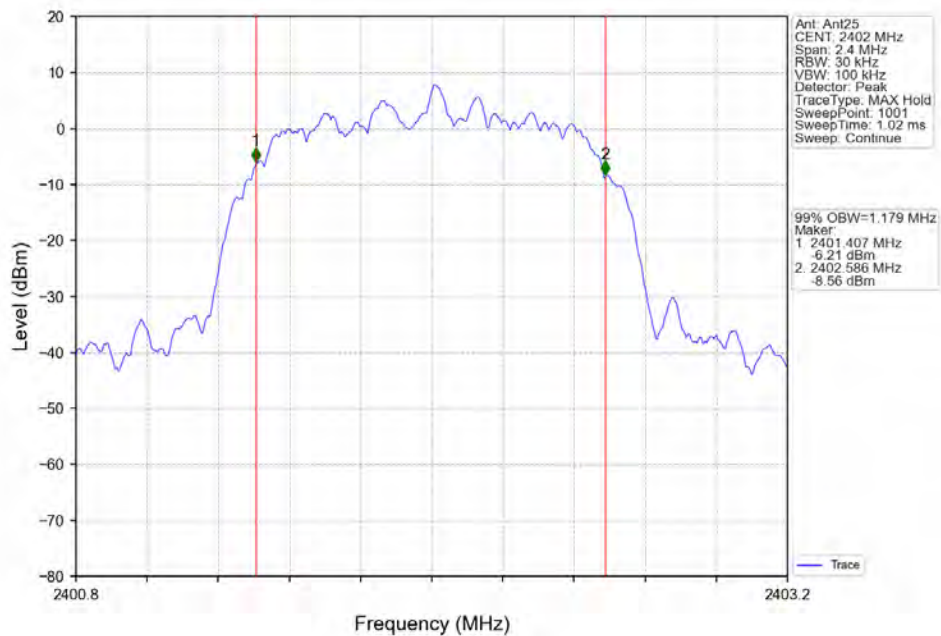
Pi/4DQPSK_2DH5_LCH_2402MHz_Ant25_NTNV
