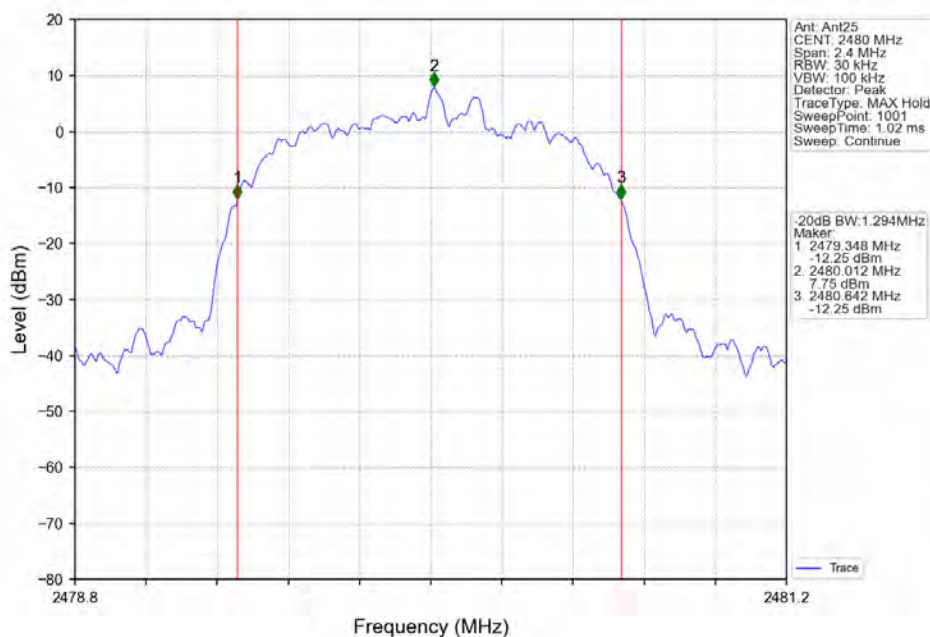
8DPSK_3DH5_HCH_2480MHz_Ant25_NTNV
