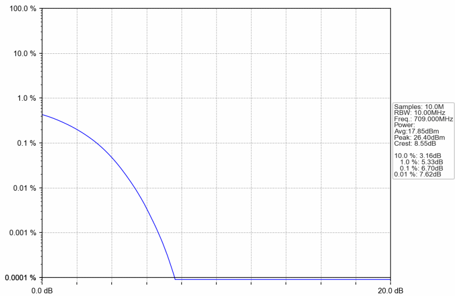
Band17_10MHz_256QAM_LCH_709MHz_RB_50_0_NTNV
