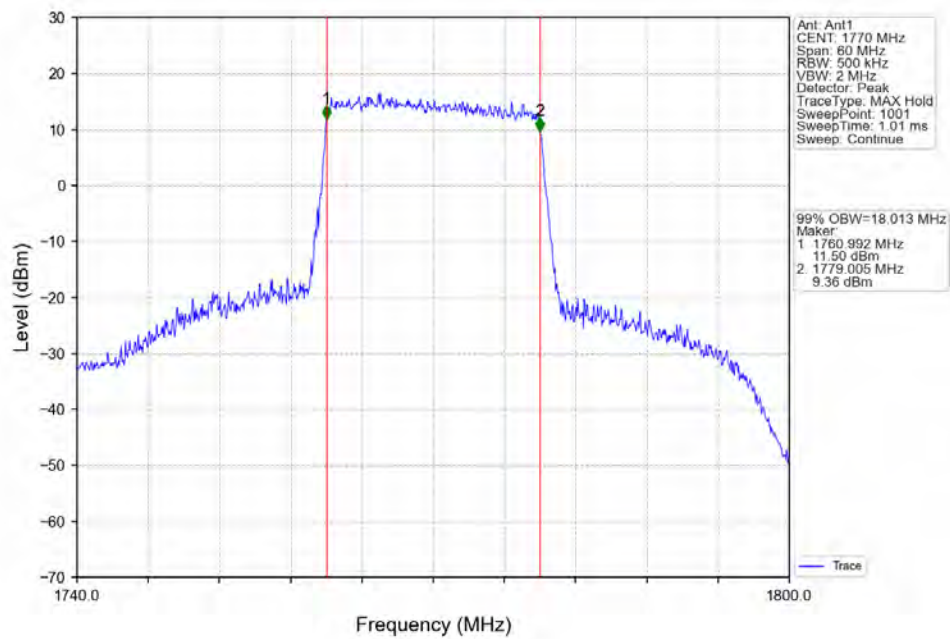
Band66_20MHz_256QAM_HCH_1770MHz_RB_100_0 NTN
