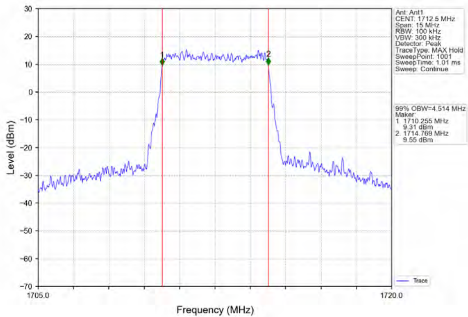
Band66_5MHz_256QAM_LCH_1712.5MHz_RB_25_0 NTN
