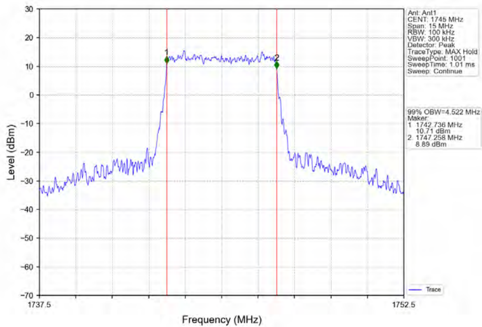
Band66_5MHz_64QAM_MCH_1745MHz_RB_25_0 NTN
