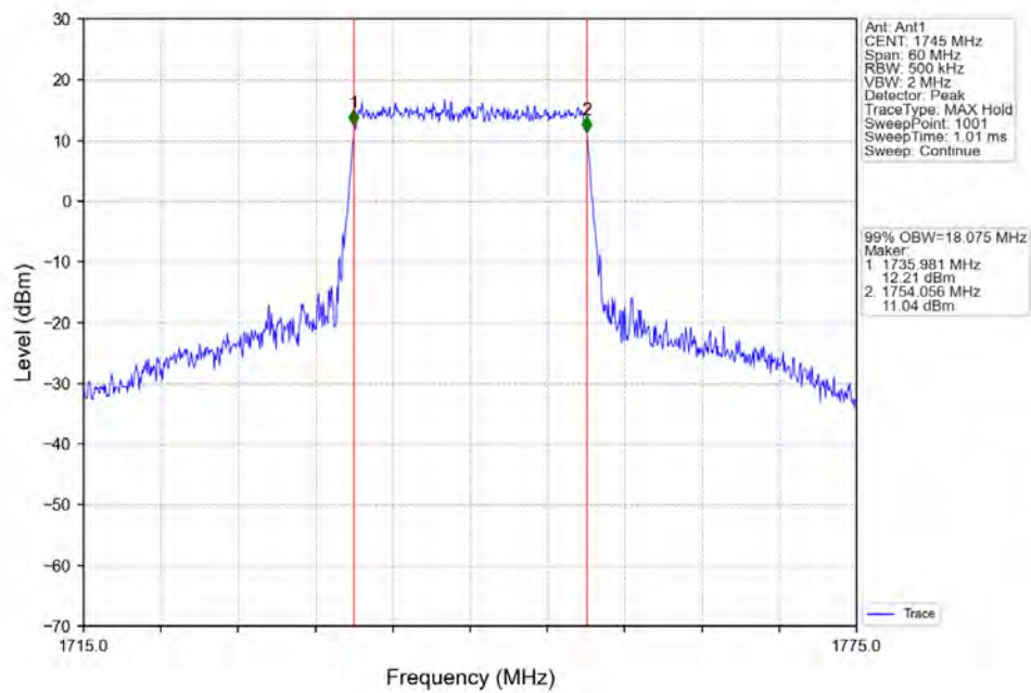
Band66_20MHz_64QAM_MCH_1745MHz_RB_100_0_NTNV
