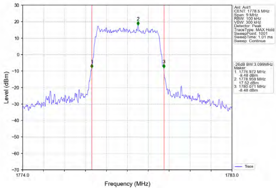
Band66_3MHz_256QAM_HCH_1778.5MHz_RB_15_0 NTN
