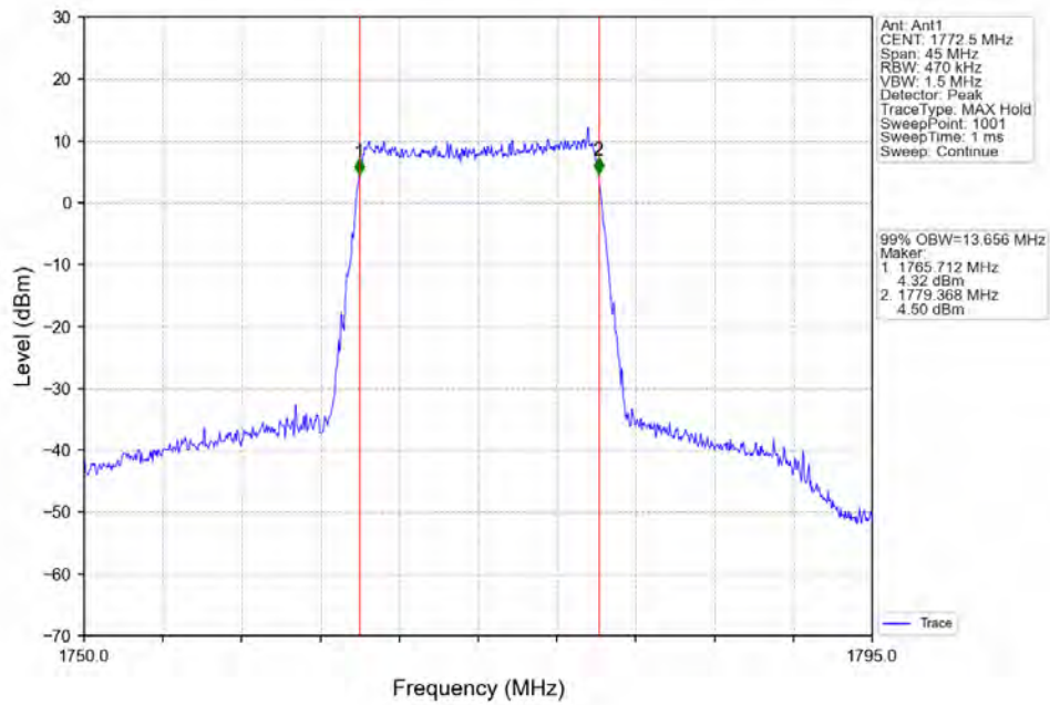
Band66 15MHz 256QAM HCH 1772.5MHz RB 75 0 NTV
