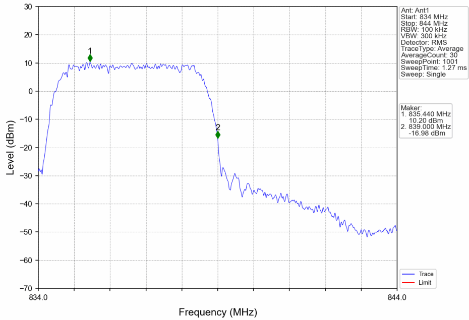
Band V_RMC_MCH_836.6MHz_12.2kbps RMC_NTNV
