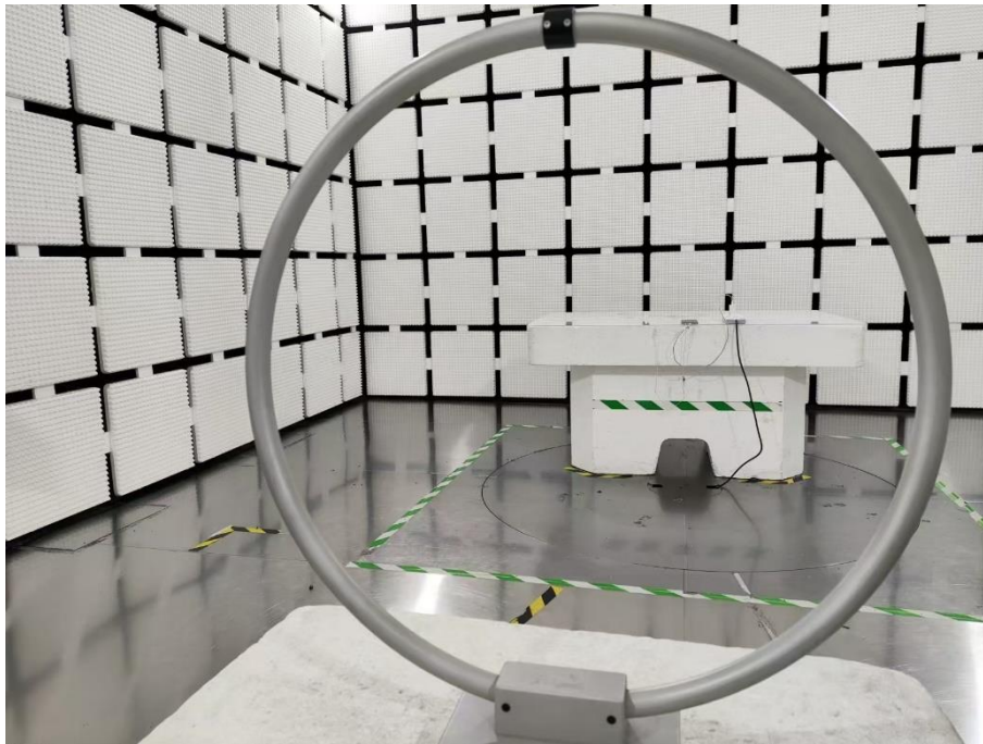
Below 30MHz-BT
