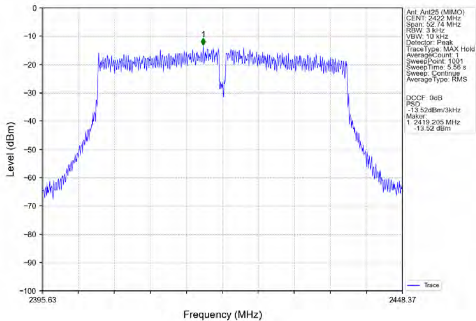
802.11ac(VHT40)_LCH_2422MHz_Ant25 (MIMO)_NTNV
