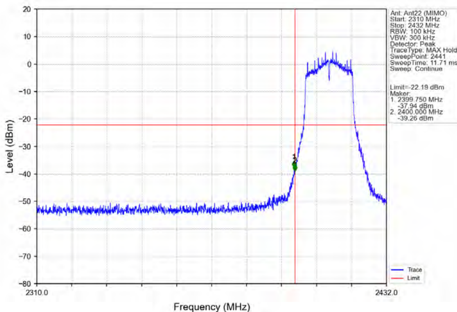
802.11g_LCH_2412MHz_Ant22 (MIMO)_NTNV
