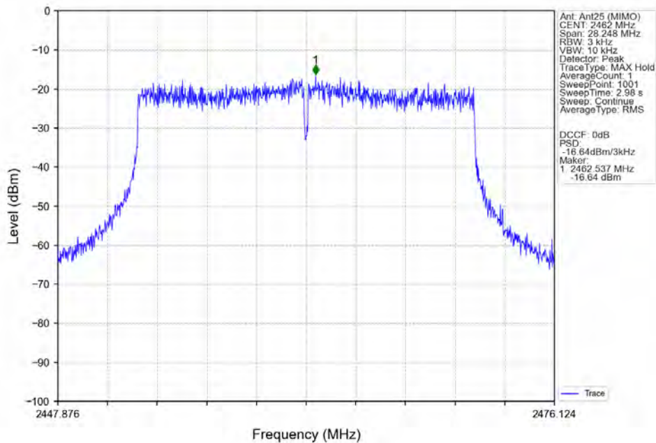
802.11ax(HEW20)_HCH_2462MHz_SU_/_Ant25 (MIMO)_NTNV
