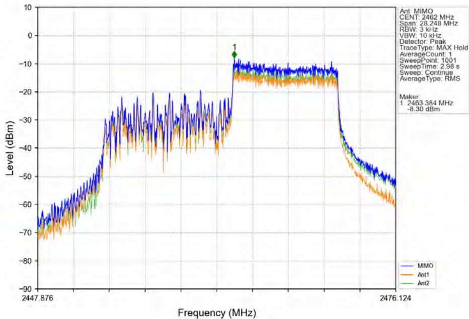
802.11ax(HEW20)_HCH_2462MHz_SU_/_Ant25 (MIMO)_NTNV
