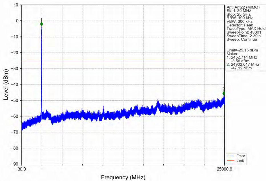
802.11ax(HEW40)_HCH_2452MHz_RU242_Right_Ant22 (MIMO)_NTNV
