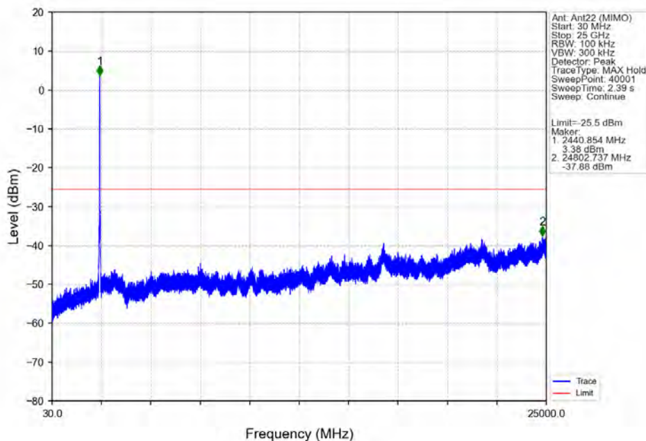
802.11ac(VHT40)_MCH_2437MHz_Ant22 (MIMO)_NTNV
