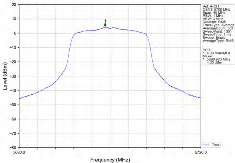
802.11a_HCH_5700MHz_Ant21_NTNV
