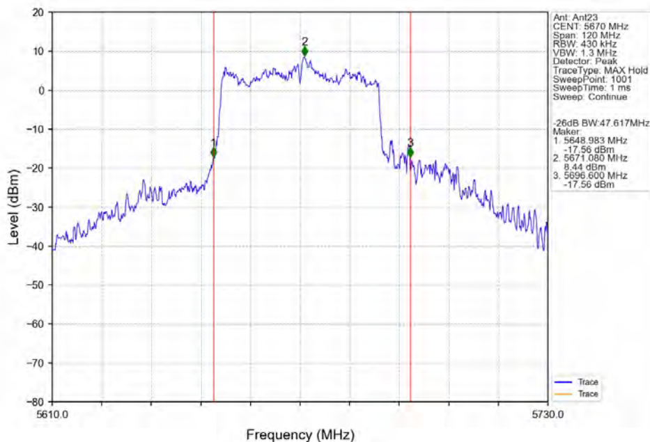
802.11ax(HEW40)_HCH_5670MHz_SU_/_Ant23_NTNV
