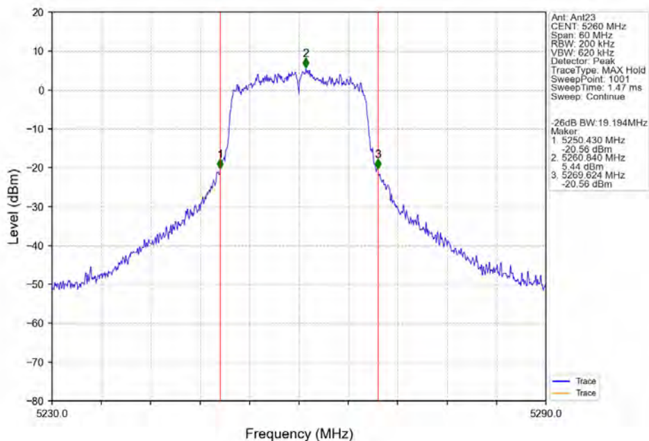
802.11a_LCH_5260MHz_Ant23_NTNV
