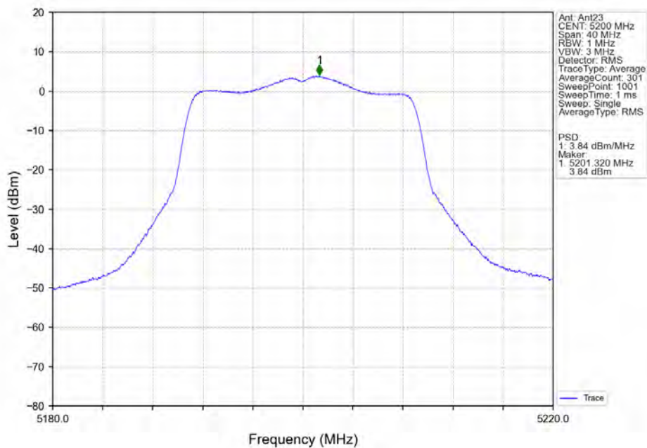
802.11n(HT20)_MCH_5200MHz_Ant23_NTNV
