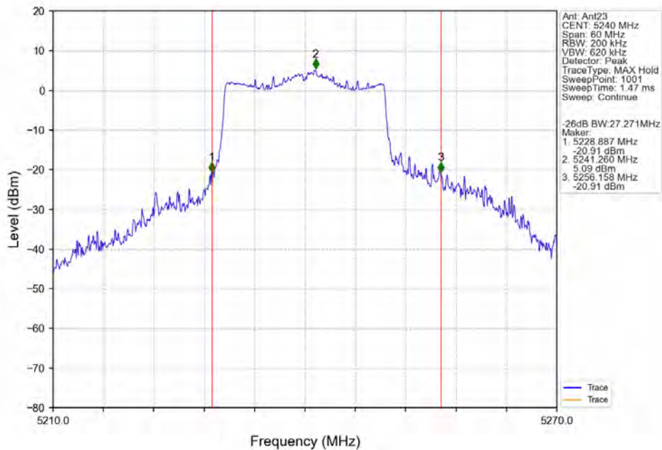
802.11ax(HEW20)_HCH_5240MHz_SU_/_Ant23_NTNV
