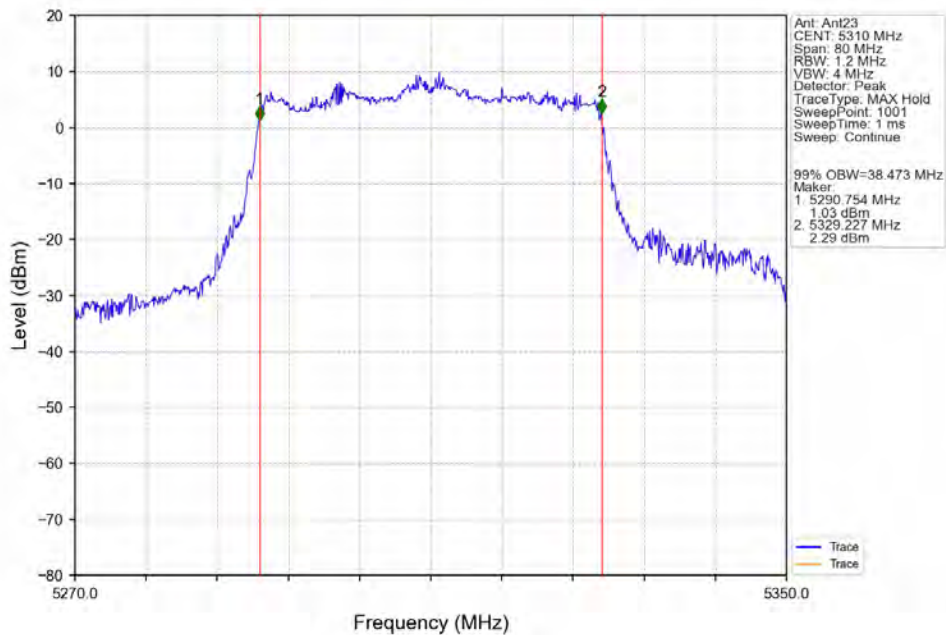
802.11ax(HEW40)_HCH_5310MHz_SU_/_Ant23_NTNV
