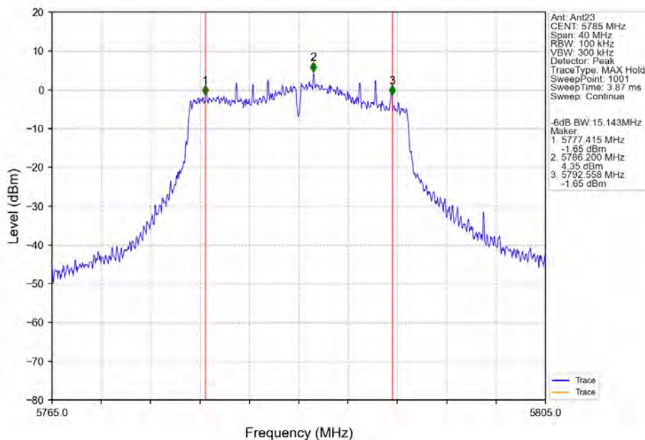
802.11ac(VHT20)_MCH_5785MHz_Ant23_NTNV
