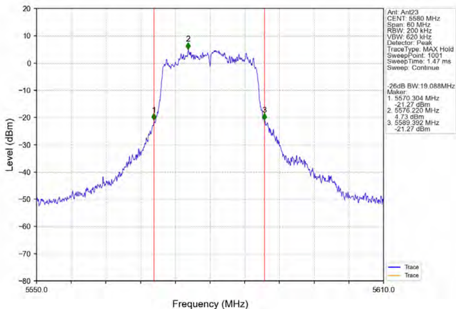
802.11a_MCH_5580MHz_Ant23_NTNV
