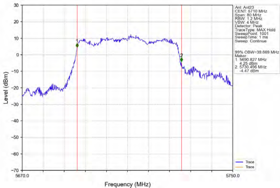
802.11ax(HEW40)_HCH_5710MHz_SU_/_Ant23_NTNV
