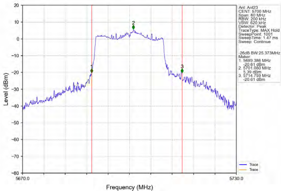
802.11ax(HEW20)_HCH_5700MHz_SU_/_Ant23_NTNV
