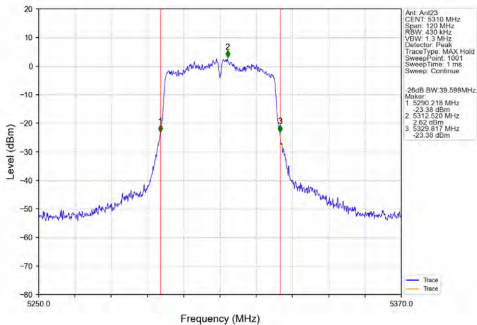
802.11n(HT40)_HCH_5310MHz_Ant23_NTNV
