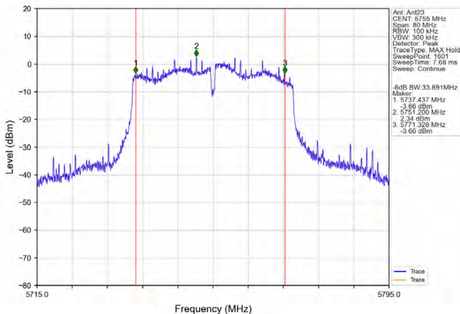
802.11ac(VHT40)_LCH_5755MHz_Ant23_NTNV
