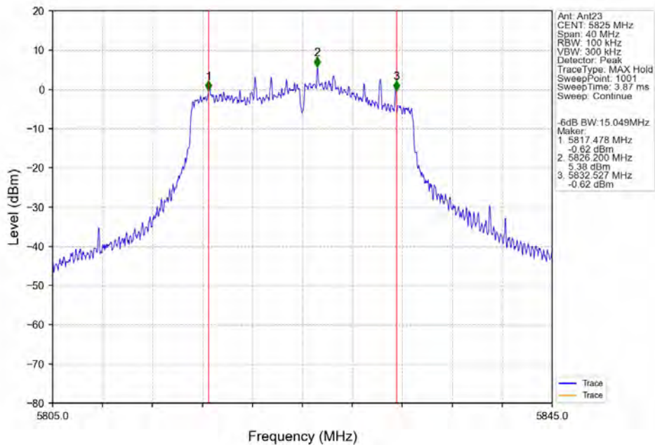
802.11n(HT20)_HCH_5825MHz_Ant23_NTNV
