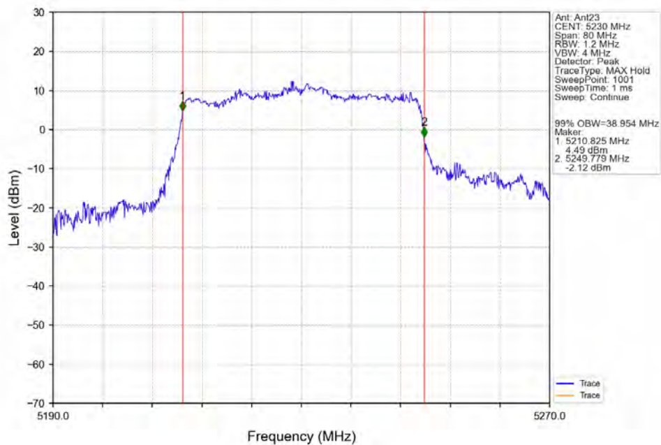
802.11ax(HEW40)_HCH_5230MHz_SU_/_Ant23_NTNV
