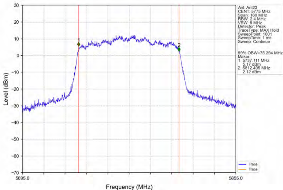
802.11ac(VHT80)_MCH_5775MHz_Ant23_NTNV
