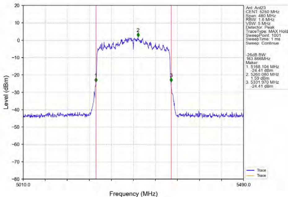
802.11ax(HEW160)_MCH_5250MHz_SU_/_Ant23_NTNV
