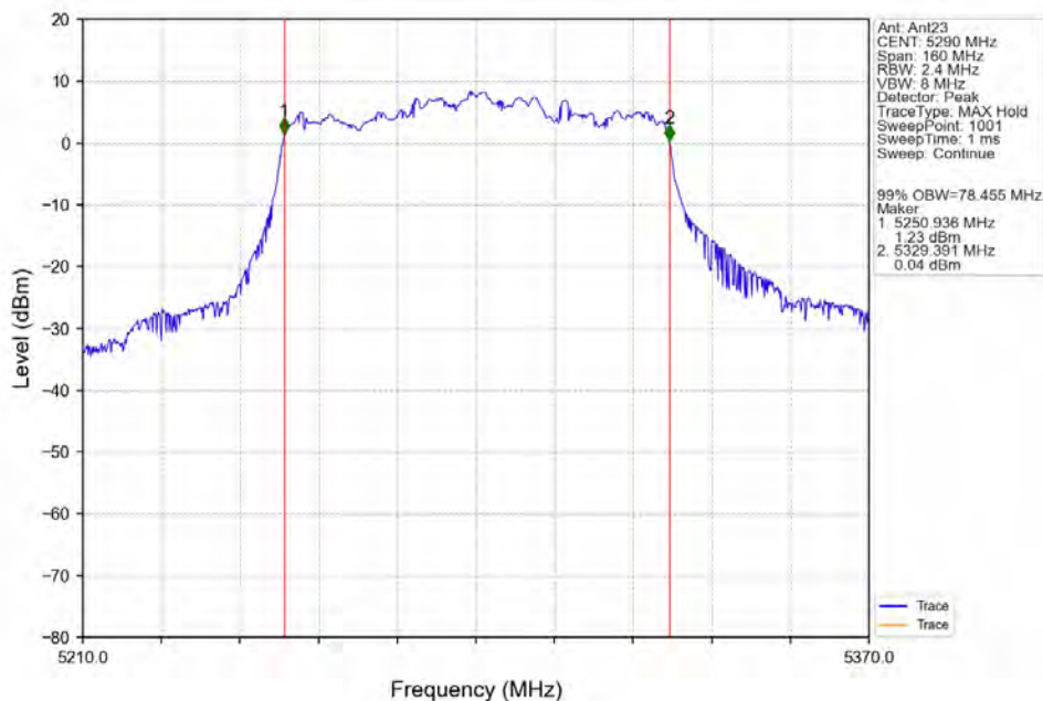
802.11ax(HEW80)_MCH_5290MHz_SU_ / _Ant23_NTNV
