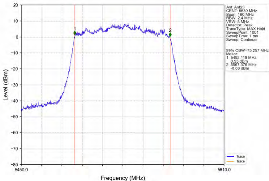
802.11ac(VHT80)_LCH_5530MHz_Ant23_NTNV
