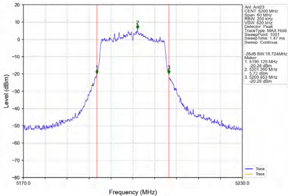
802.11n(HT20)_MCH_5200MHz_Ant23_NTNV
