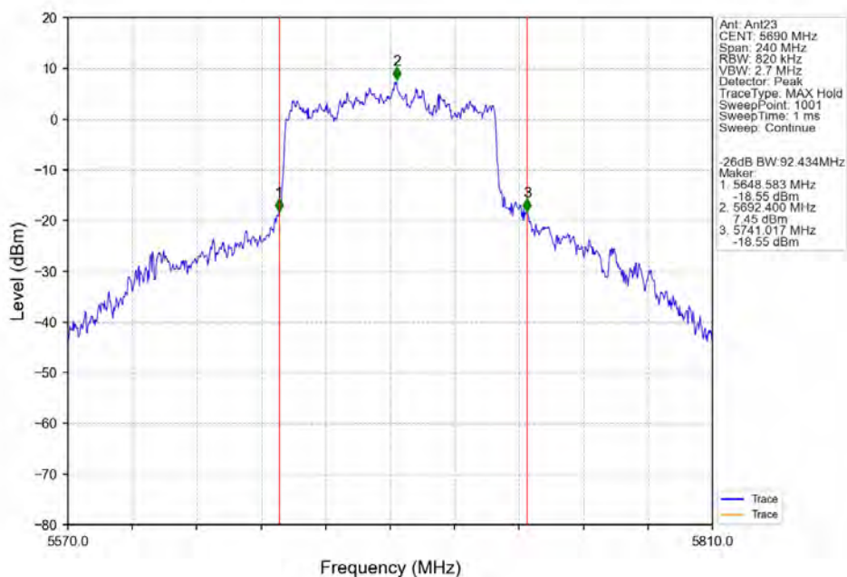
802.11ax(HEW80)_HCH_5690MHz_SU_/_Ant23_NTNV
