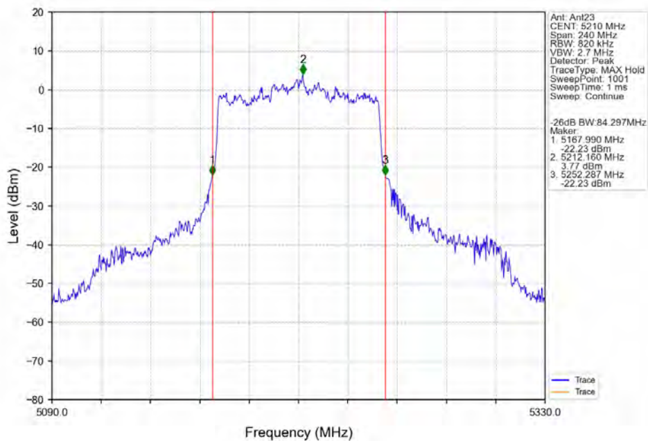
802.11ax(HEW80)_MCH_5210MHz_SU_/_Ant23_NTNV
