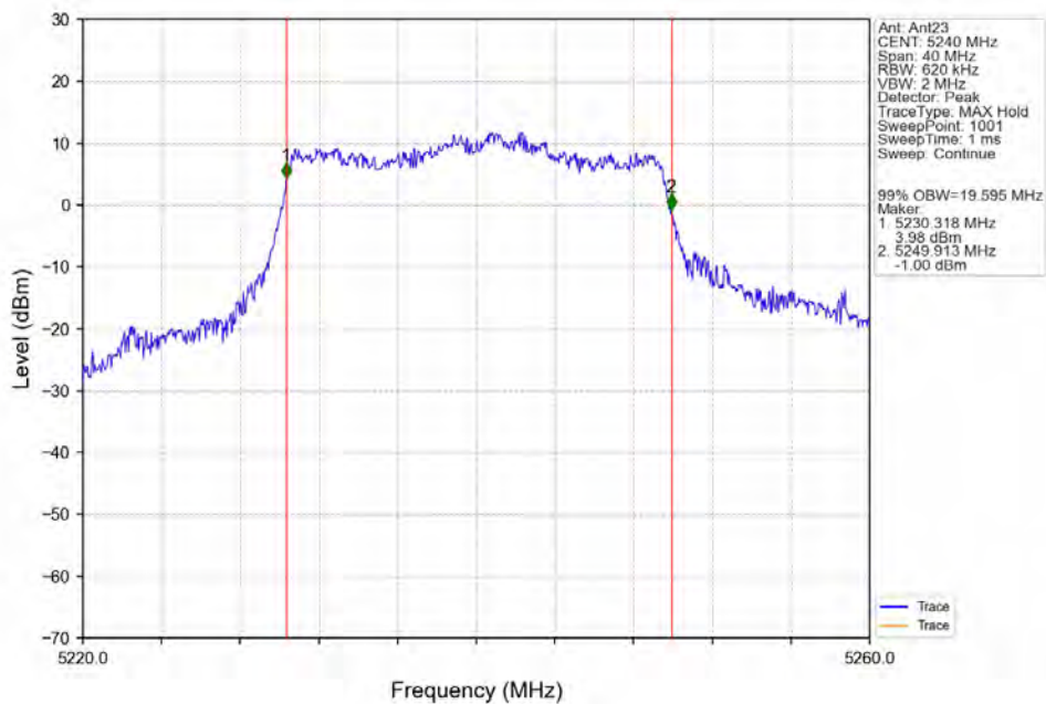
802.11ax(HEW20)_HCH_5240MHz_SU_/_Ant23_NTNV
