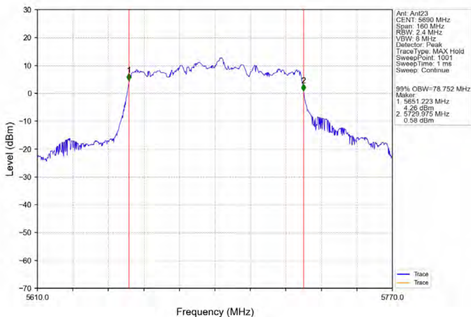
802.11ax(HEW80)_HCH_5690MHz_SU_/_Ant23_NTNV
