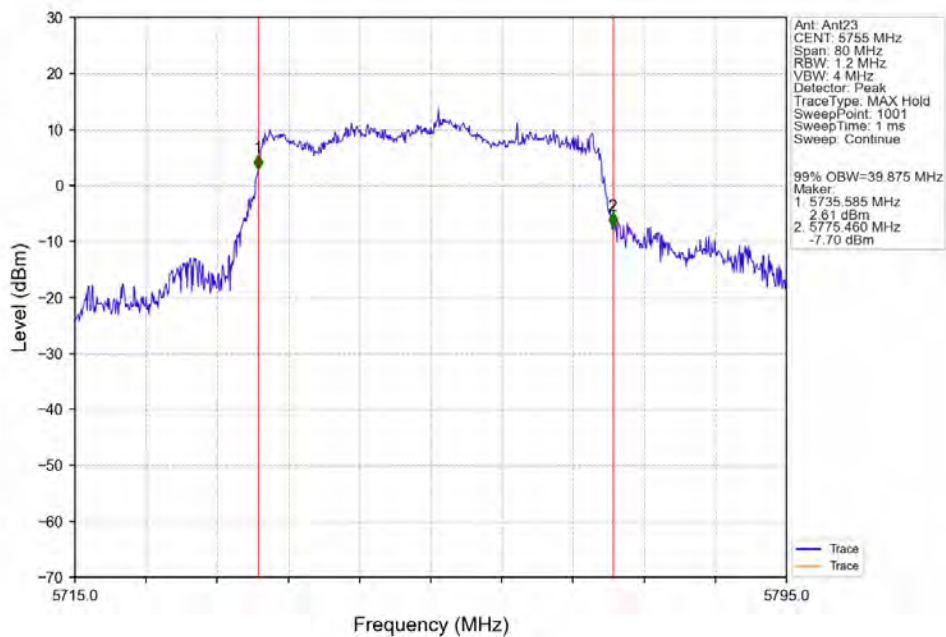
802.11ax(HEW40)_LCH_5755MHz_SU_/_Ant23_NTNV
