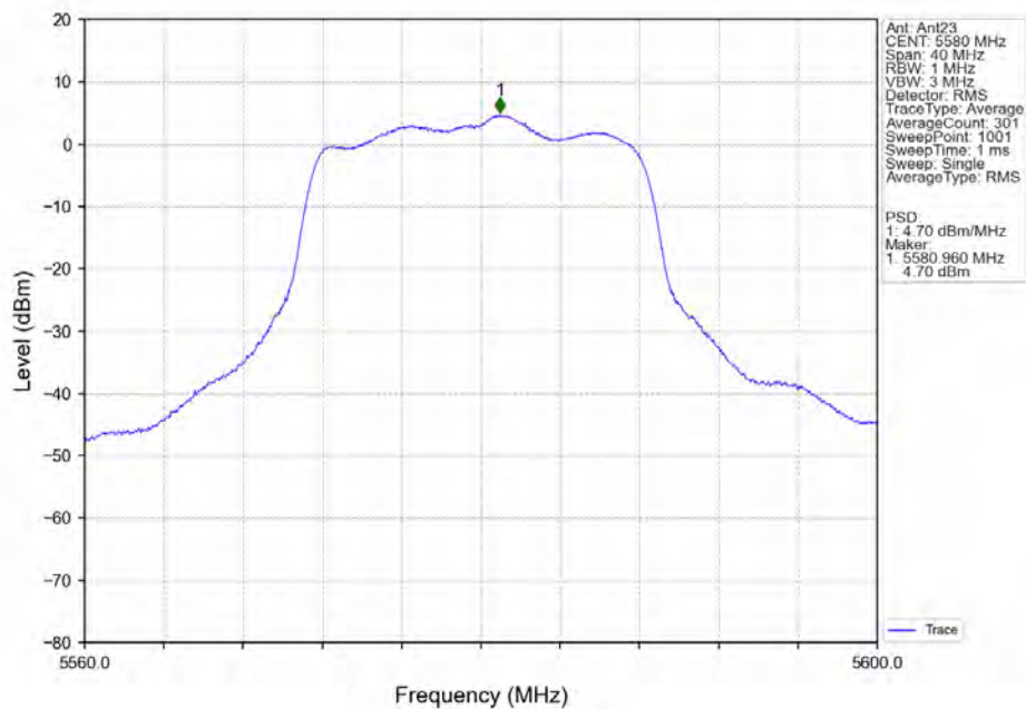
802.11a_MCH_5580MHz_Ant23_NTNV
