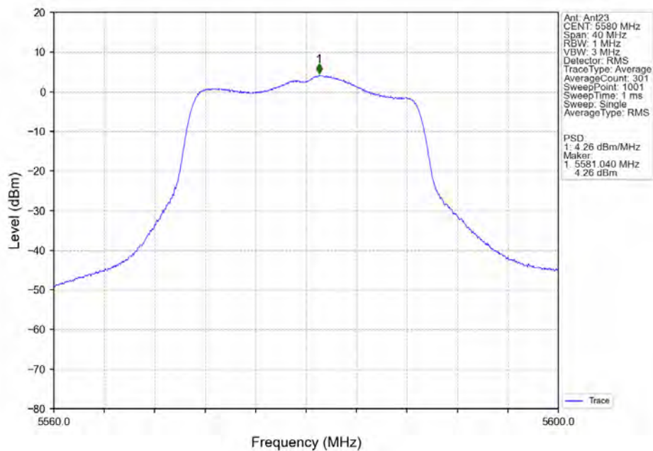
802.11n(HT20)_MCH_5580MHz_Ant23_NTNV
