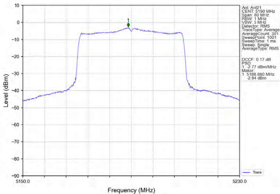
802.11ax(HEW40)_LCH_5190MHz_SU_/_Ant21_NTNV
