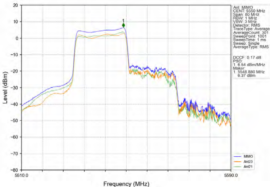
802.11ax(HEW40)_MCH_5550MHz_RU242_Left_MIMO_NTNV
