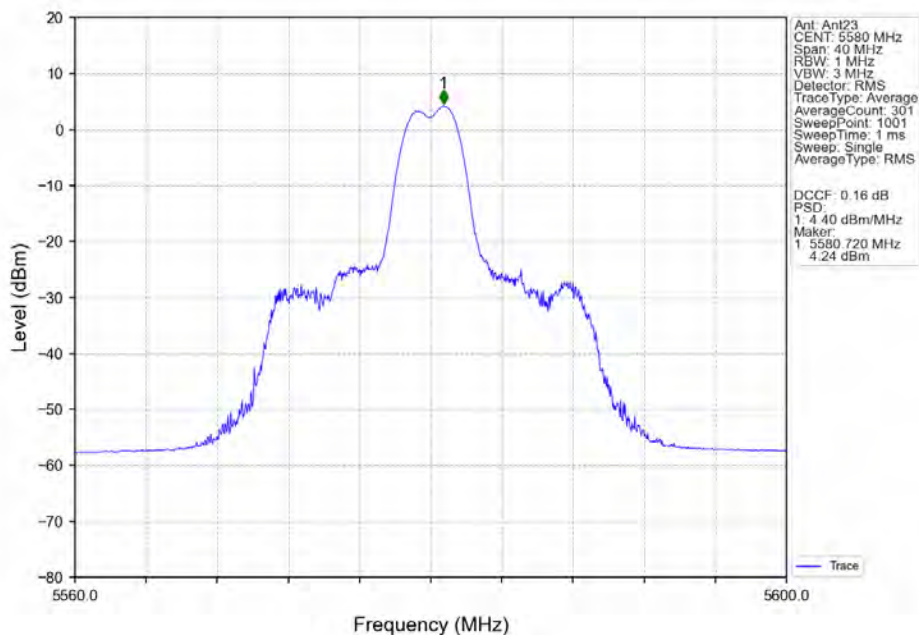
802.11ax(HEW20)_MCH_5580MHz_RU26_Mid_Ant23_NTNV
