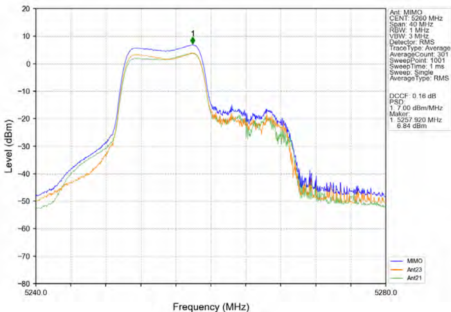
802.11ax(HEW20)_LCH_5260MHz_RU106_Left_MIMO_NTNV
