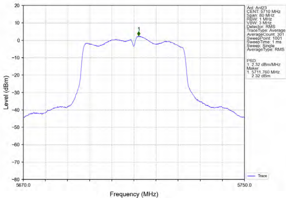
802.11ac(VHT40)_HCH_5710MHz_Ant23_NTNV
