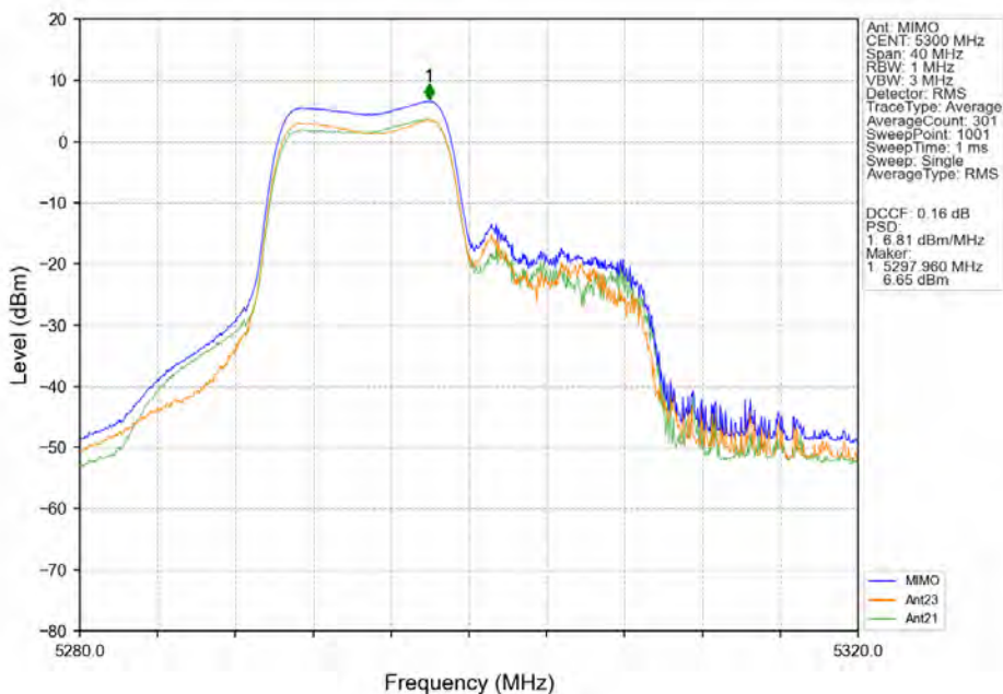
802.11ax(HEW20)_MCH_5300MHz_RU106_Left_MIMO_NTNV
