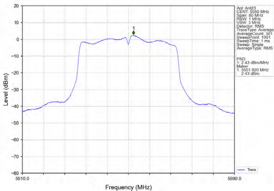
802.11ac(VHT40)_MCH_5550MHz_Ant23_NTNV
