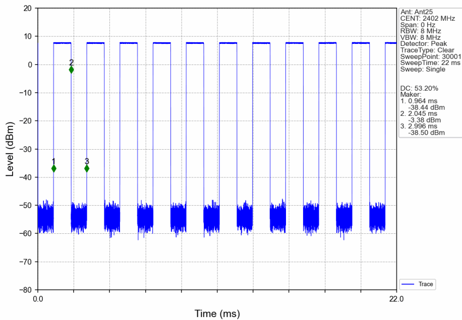
2M_LCH_2402MHz_Ant25_NTNV
