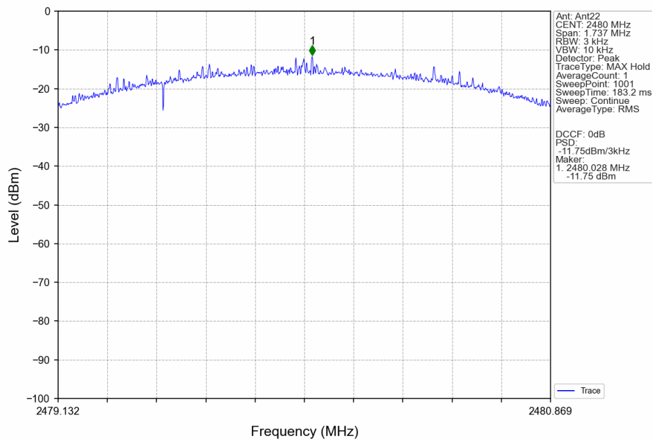
2M_HCH_2480MHz_Ant22_NTNV
