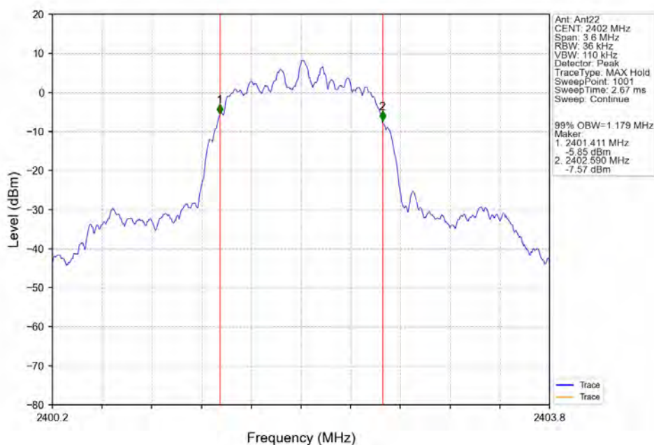
Pi/4DQPSK_2DH5_LCH_2402MHz_Ant22_NTNV
