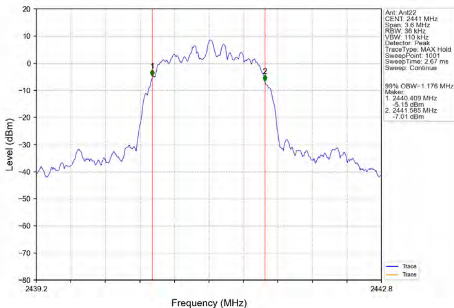
Pi/4DQPSK_2DH5_MCH_2441MHz_Ant22_NTNV
