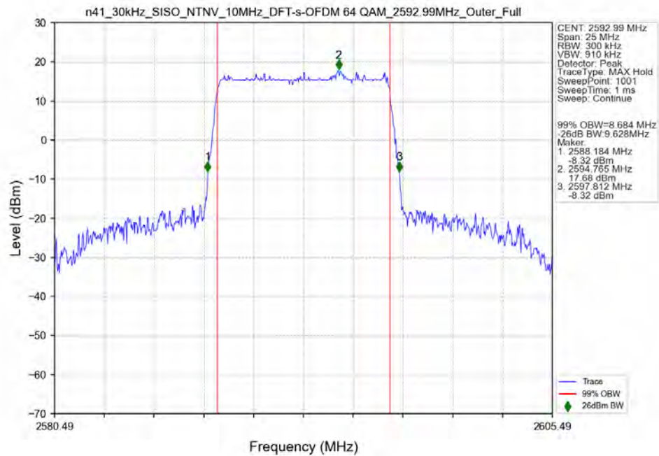
n41_30kHz_SISO_NTNV_10MHz_DFT-s-OFDM_64_QAM_2592.99MHz_Outer_Full_Ant31
