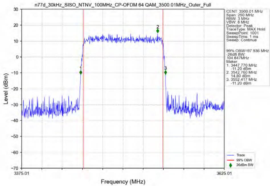
n77d_30kHz_SISO_NTNV_100MHz_CP-OFDM 64 QAM_3500.01MHz_Outer_Full_Ant11
