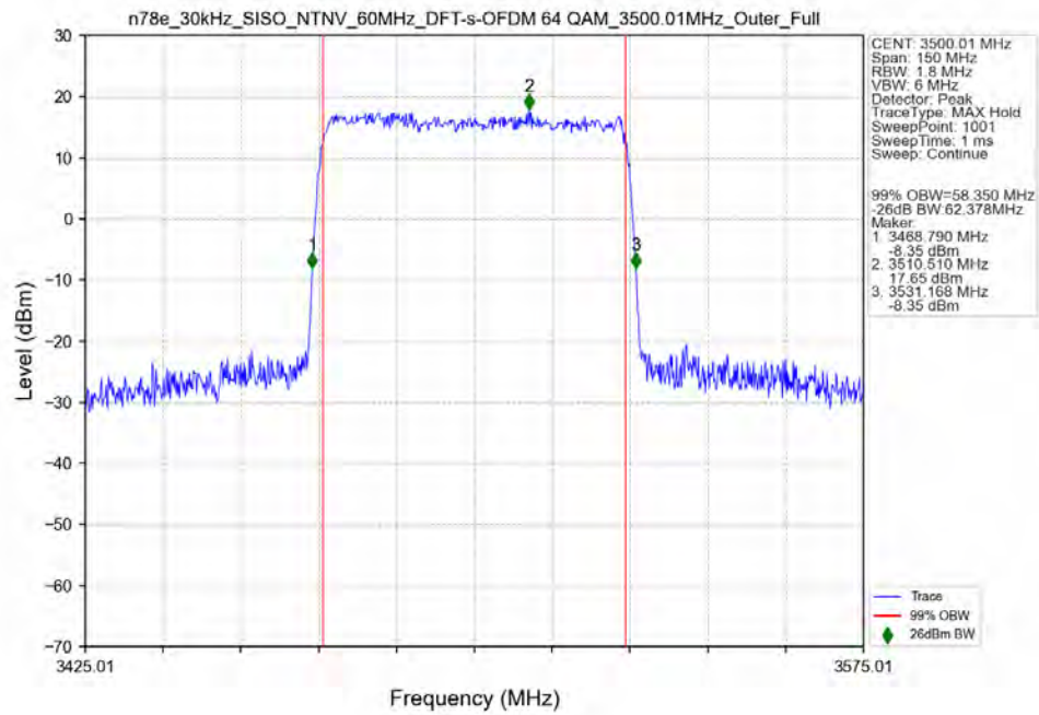
n78e_30kHz_SISO_NTNV_60MHz_DFT-s-OFDM_64_QAM_3500.01MHz_Outer_Full_Ant11
