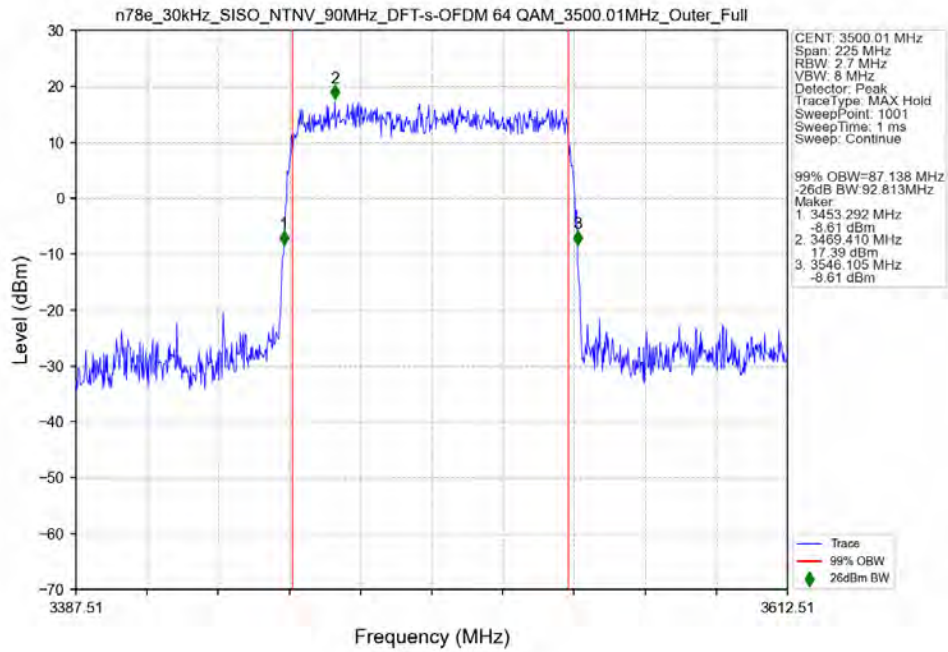
n78e_30kHz_SISO_NTNV_90MHz_DFT-s-OFDM_64_QAM_3500.01MHz_Outer_Full_Ant11
