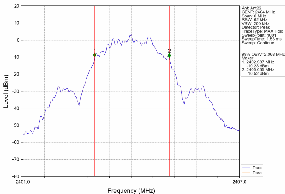
2M_LCH_2404MHz_Ant22_NTNV
