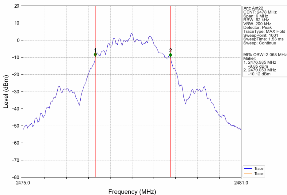
2M_HCH_2478MHz_Ant22_NTNV
