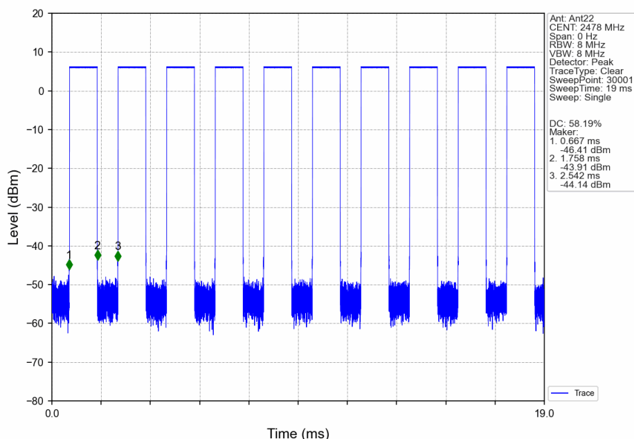
2M_HCH_2478MHz_Ant22_NTNV
