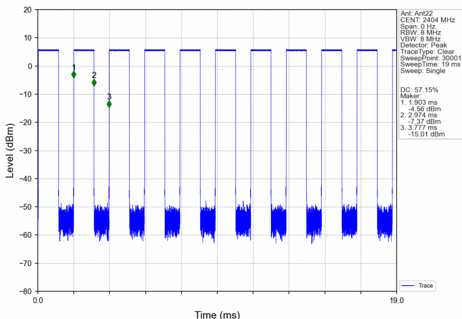
2M_LCH_2404MHz_Ant22_NTNV
