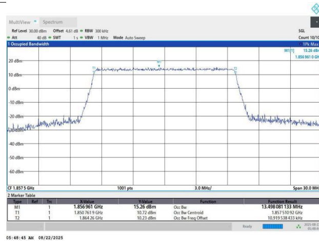
Band2-15MHz-64QAM-18675-75RB#0-13.5-15.02
