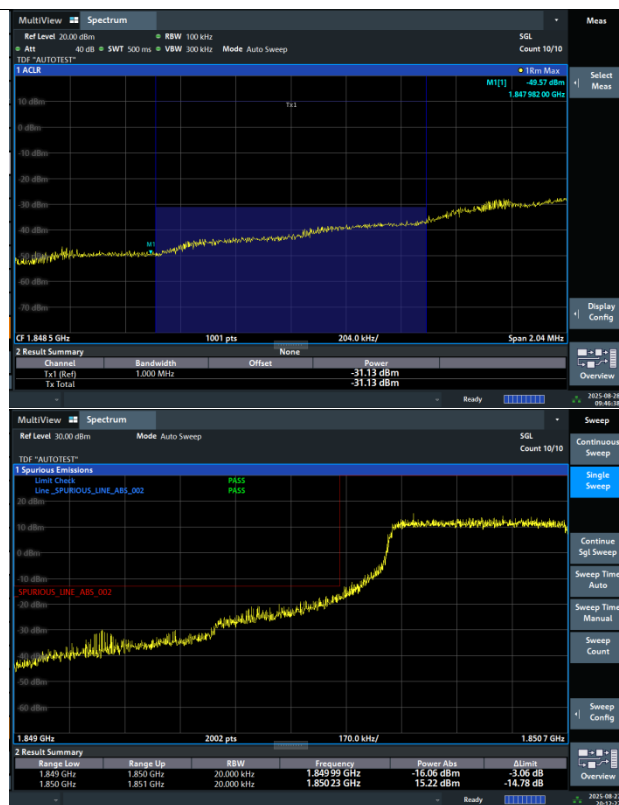
Band2-1.4MHz-QPSK-18607-3RB#0-PASS
