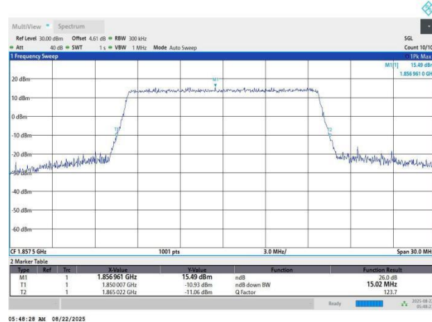
Band2-15MHz-64QAM-18675-75RB#0-13.5-15.02
