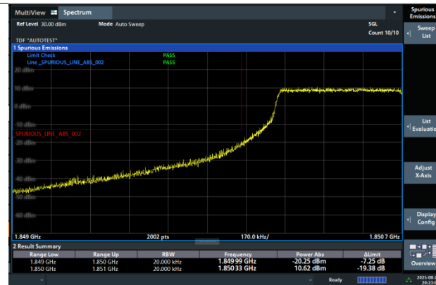
Band2-1.4MHz-64QAM-18607-6RB#0-PASS
