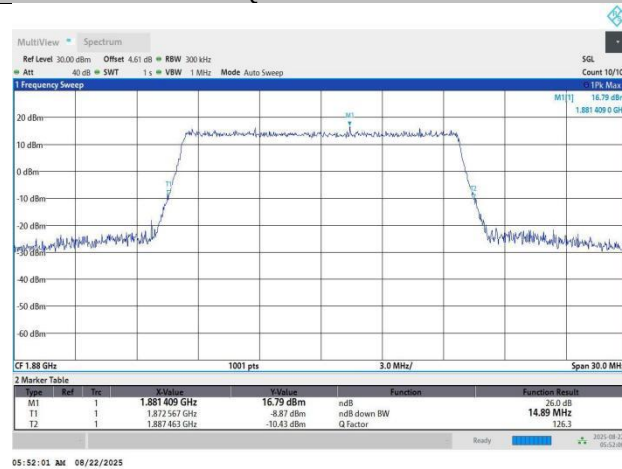
Band2-15MHz-64QAM-18900-75RB#0-13.51-14.89
