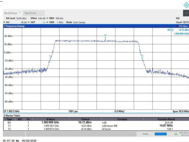
Band2-15MHz-64QAM-19125-75RB#0-13.48-14.87
