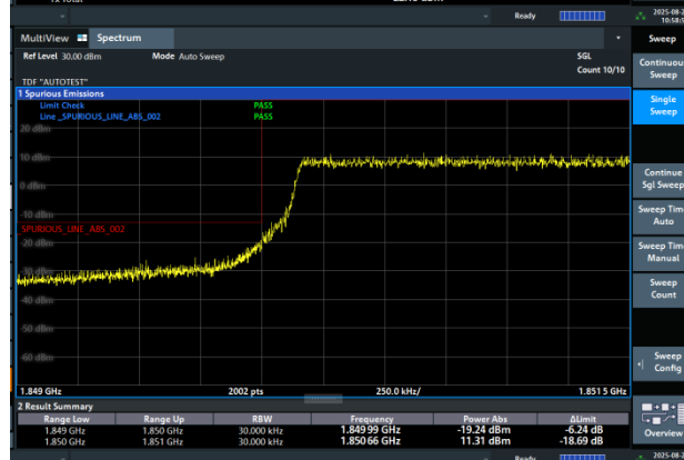
Band2-3MHz-QPSK-18615-8RB#0-PASS
