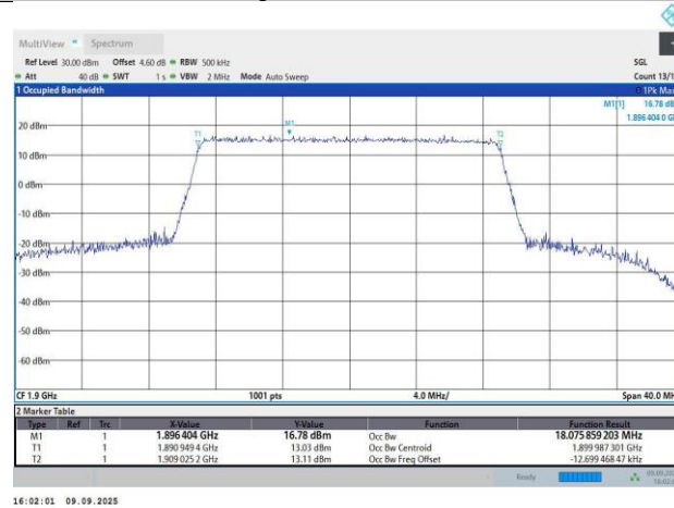
Band2-20MHz-64QAM-19100-100RB#0-18.08-19.98
