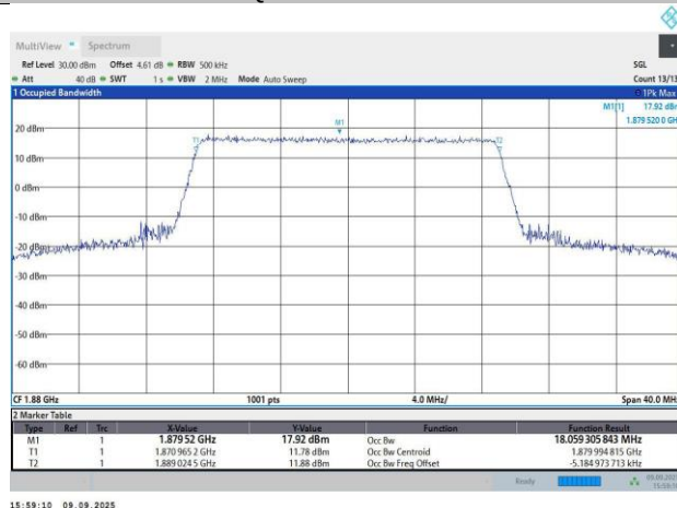
Band2-20MHz-16QAM-18900-100RB#0-18.06-20.14
