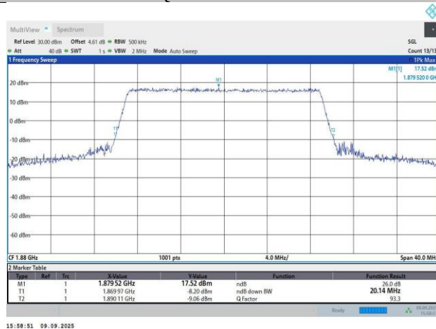
Band2-20MHz-16QAM-18900-100RB#0-18.06-20.14
