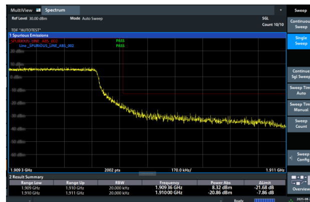
Band2-1.4MHz-QPSK-19193-3RB#3-PASS
