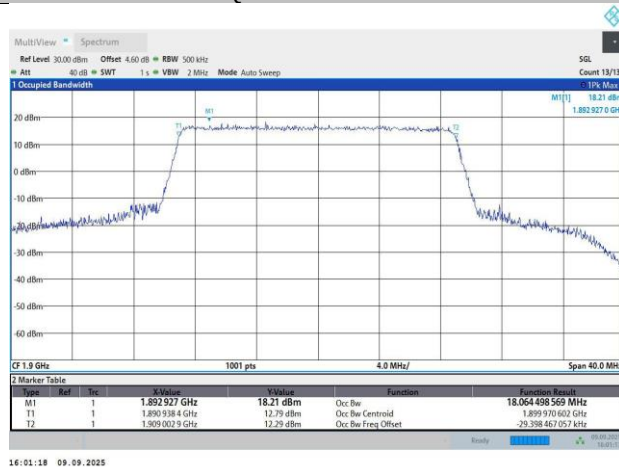
Band2-20MHz-16QAM-19100-100RB#0-18.06-20.14
