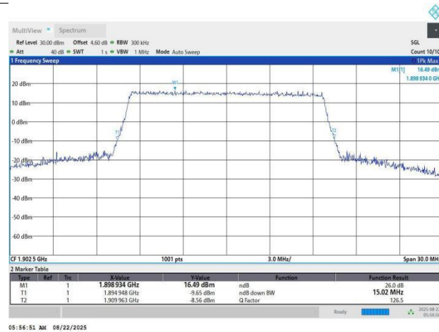
Band2-15MHz-16QAM-19125-75RB#0-13.48-15.02
