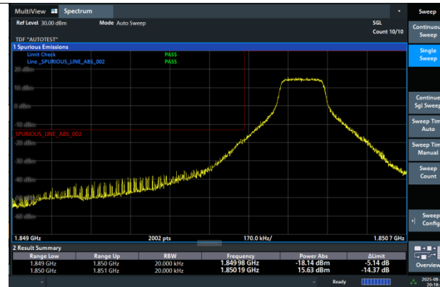
Band2-1.4MHz-16QAM-18607-1RB#0-PASS
