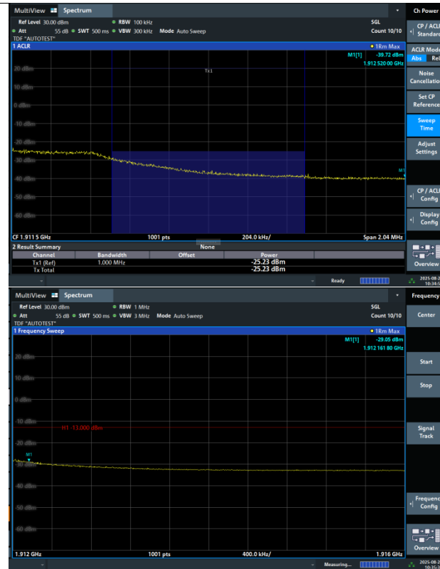
Band2-1.4MHz-QPSK-19193-6RB#0-PASS
