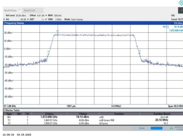
Band2-20MHz-QPSK-18900-100RB#0-18.08-20.1
