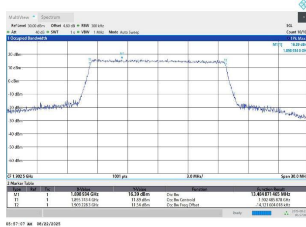
Band2-15MHz-16QAM-19125-75RB#0-13.48-15.02
