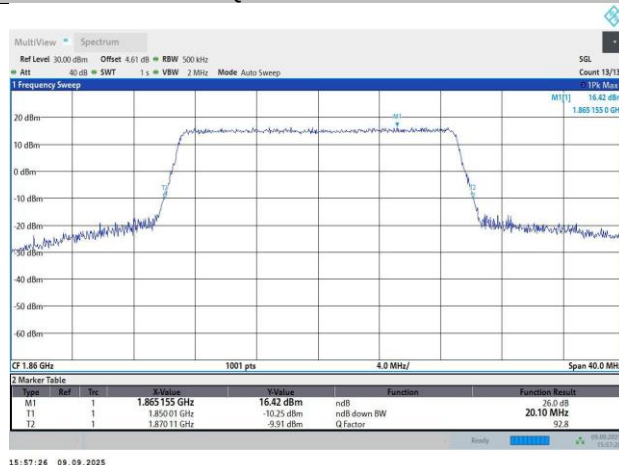
Band2-20MHz-64QAM-18700-100RB#0-18.05-20.1
