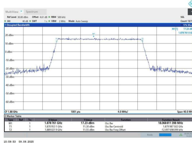
Band2-20MHz-64QAM-18900-100RB#0-18.07-20.1
