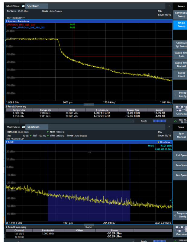
Band2-1.4MHz-16QAM-19193-1RB#5-PASS
