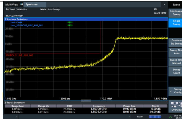
Band2-1.4MHz-QPSK-18607-6RB#0-PASS
