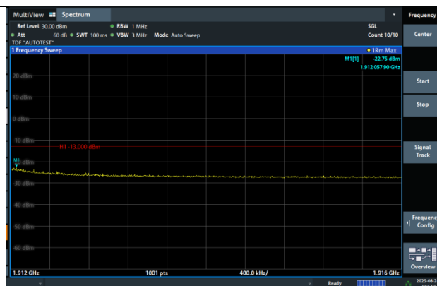
Band2-3MHz-QPSK-19185-8RB#7-PASS
