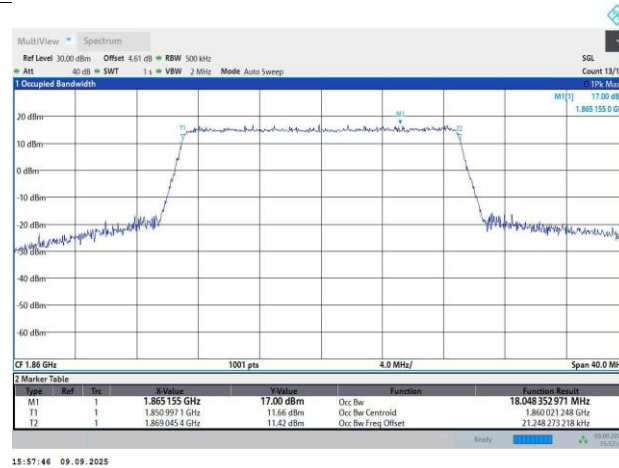
Band2-20MHz-64QAM-18700-100RB#0-18.05-20.1
