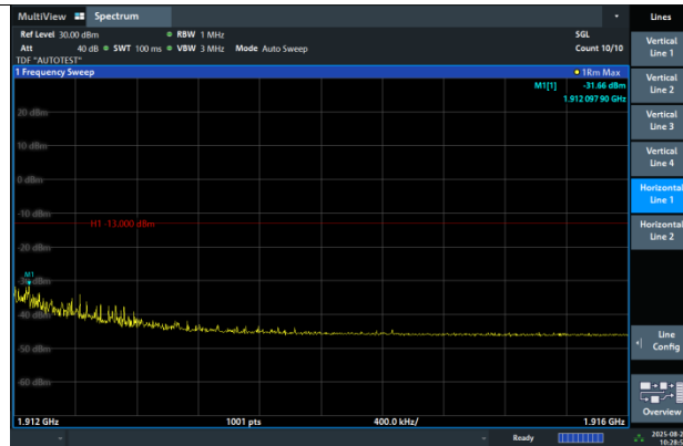
Band2-1.4MHz-16QAM-19193-3RB#3-PASS
