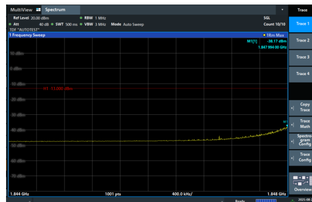
Band2-1.4MHz-64QAM-18607-1RB#0-PASS
