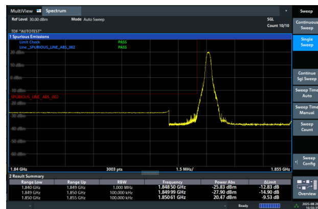
Band2-10MHz-64QAM-18650-1RB#0-PASS
