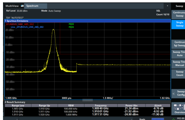
Band2-10MHz-16QAM-19150-1RB#49-PASS
