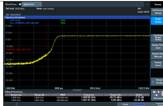
Band2-5MHz-64QAM-18625-25RB#0-PASS
