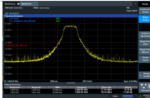
Band2-3MHz-64QAM-18615-1RB#0-PASS
