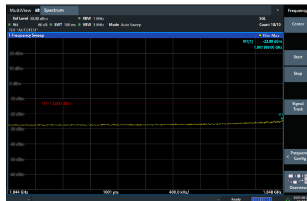
Band2-5MHz-64QAM-18625-1RB#0-PASS
