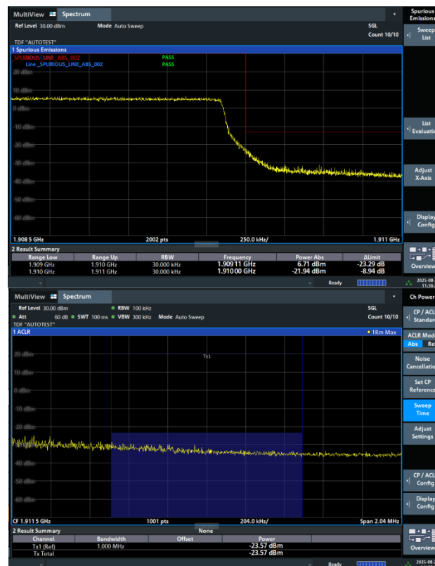
Band2-3MHz-64QAM-19185-1RB#14-PASS
