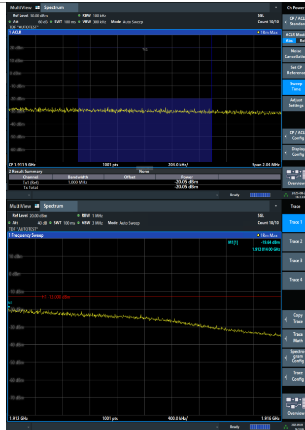
Band2-5MHz-QPSK-19175-25RB#0-PASS
