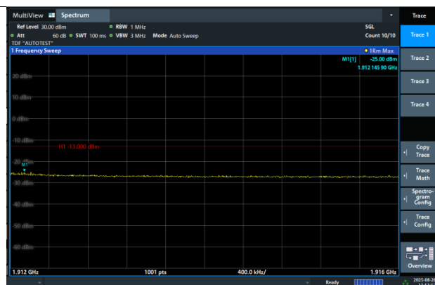
Band2-3MHz-64QAM-19185-8RB#7-PASS
