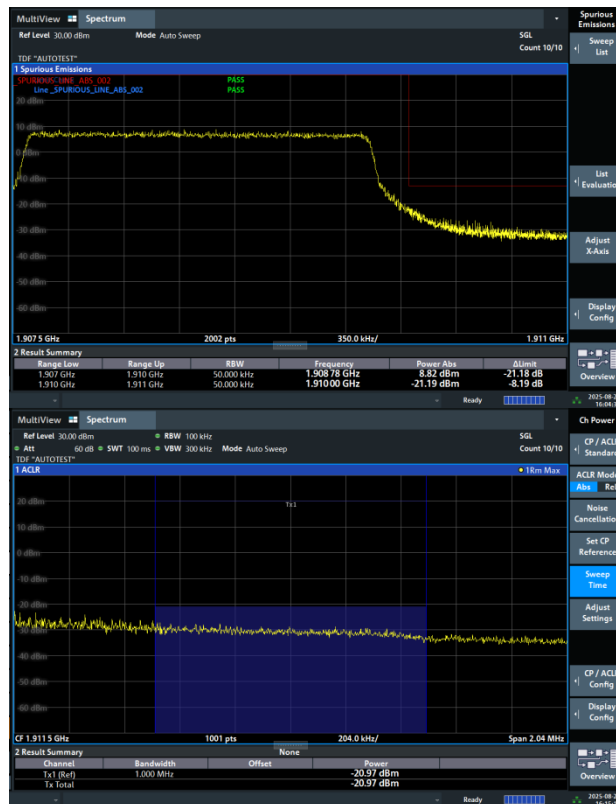
Band2-5MHz-16QAM-19175-1RB#24-PASS
