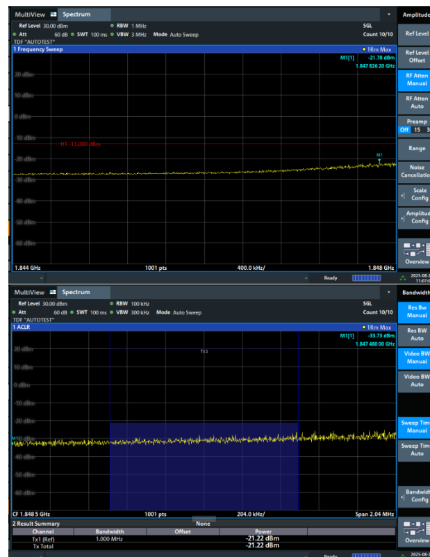
Band2-3MHz-16QAM-18615-8RB#0-PASS
