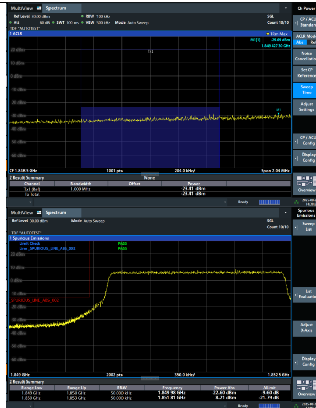
Band2-5MHz-64QAM-18625-12RB#0-PASS
