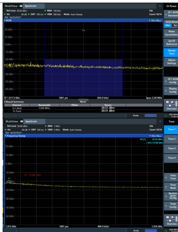
Band2-3MHz-16QAM-19185-15RB#0-PASS
