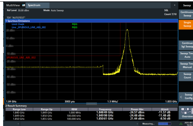
Band2-10MHz-16QAM-18650-1RB#0-PASS
