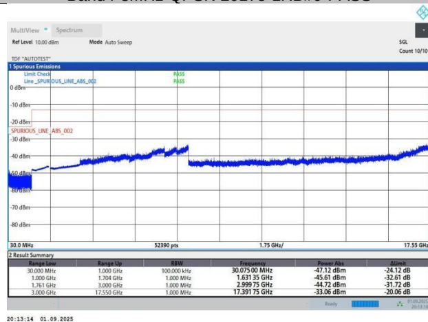
Band4-3MHz-QPSK-20175-1RB#0-PASS
