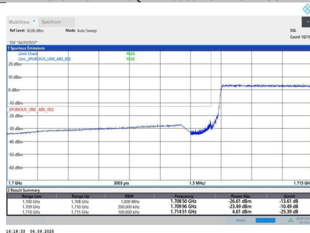
Band4-10MHz-16QAM-20000-50RB#0-PASS
