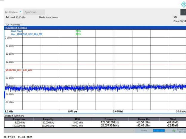
Band4-1.4MHz-QPSK-20175-1RB#0-PASS
