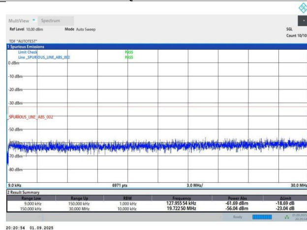
Band4-20MHz-QPSK-20300-1RB#0-PASS
