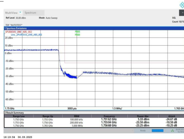
Band4-10MHz-QPSK-20350-50RB#0-PASS
