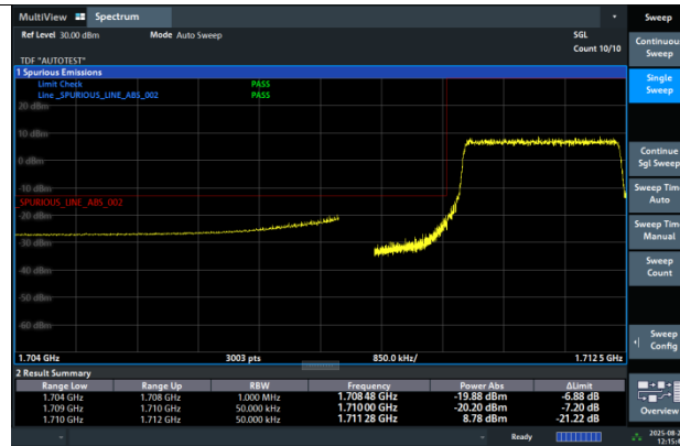
Band4-5MHz-16QAM-19975-12RB#0-PASS
