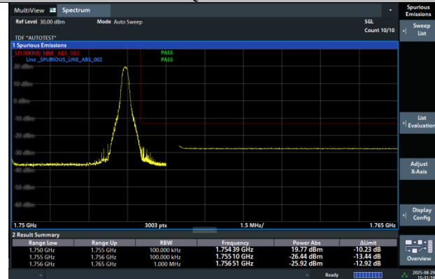
Band4-10MHz-64QAM-20350-1RB#49-PASS
