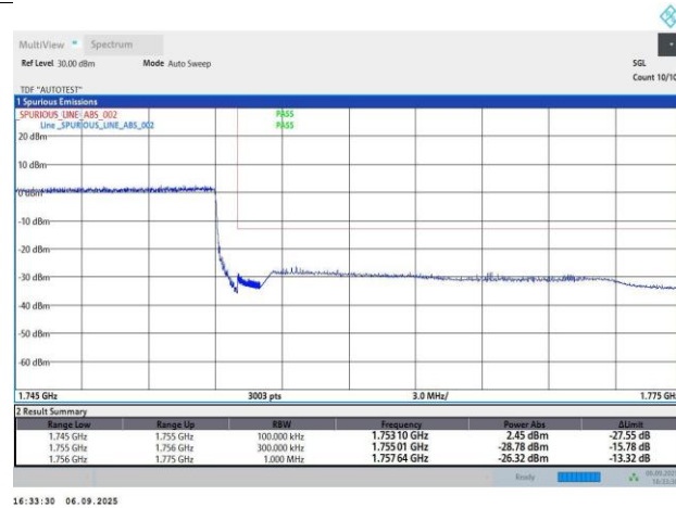
Band4-20MHz-QPSK-20300-100RB#0-PASS
