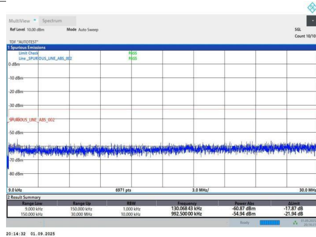
Band4-5MHz-QPSK-20175-1RB#0-PASS
