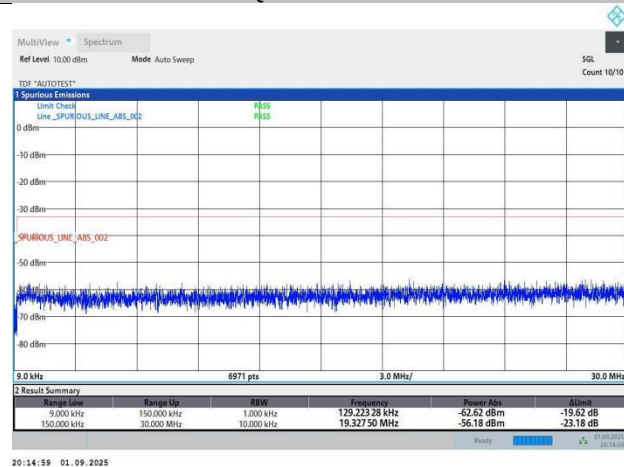
Band4-5MHz-QPSK-20375-1RB#0-PASS
