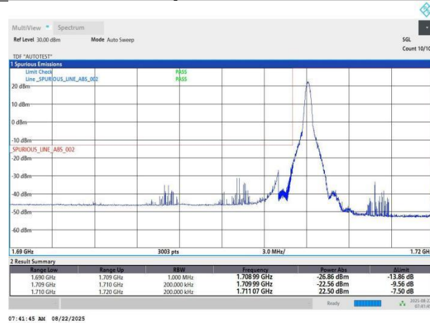
Band4-20MHz-16QAM-20050-1RB#0-PASS
