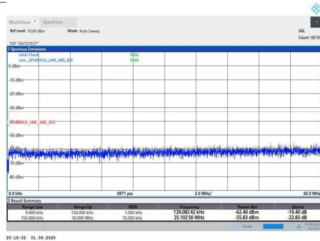
Band4-10MHz-QPSK-20175-1RB#0-PASS
