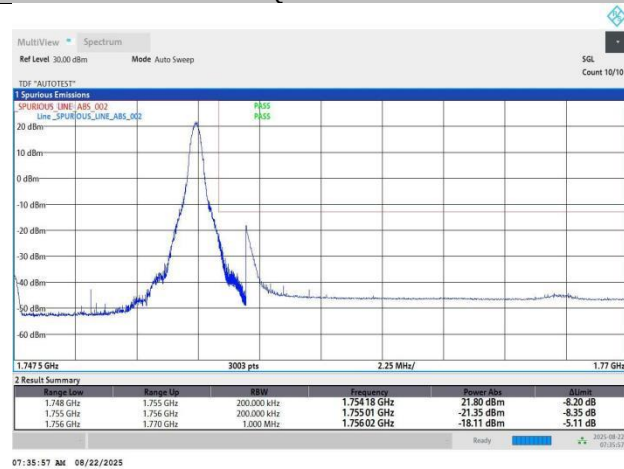
Band4-15MHz-64QAM-20325-1RB#74-PASS
