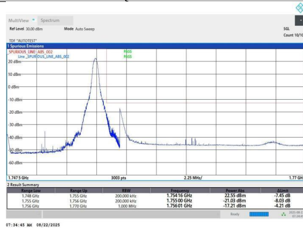
Band4-15MHz-QPSK-20325-1RB#74-PASS
