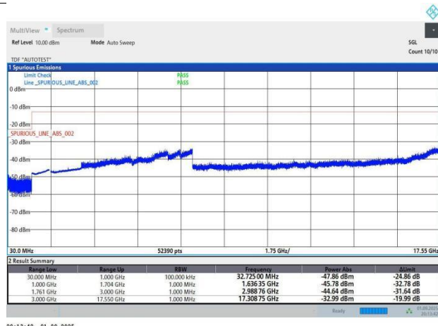
Band4-3MHz-QPSK-20385-1RB#0-PASS
