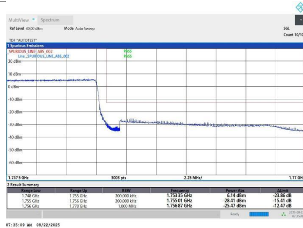
Band4-15MHz-QPSK-20325-75RB#0-PASS
