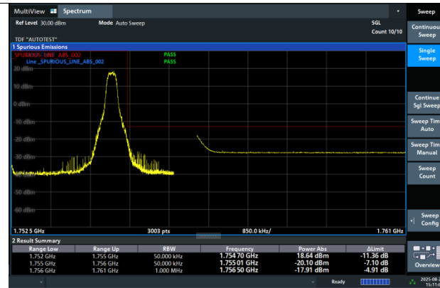
Band4-5MHz-64QAM-20375-1RB#24-PASS
