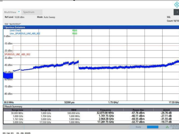
Band4-5MHz-QPSK-19975-1RB#0-PASS
