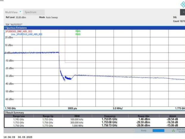
Band4-20MHz-16QAM-20300-100RB#0-PASS
