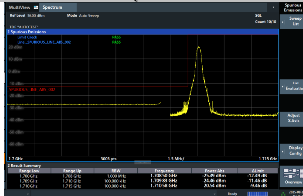
Band4-10MHz-64QAM-20000-1RB#0-PASS
