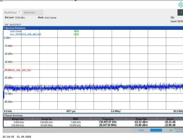
Band4-5MHz-QPSK-19975-1RB#0-PASS
