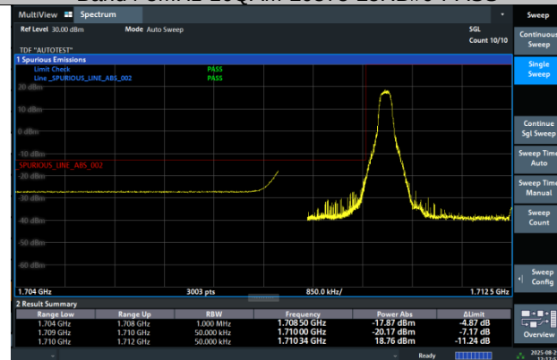
Band4-5MHz-64QAM-19975-1RB#0-PASS
