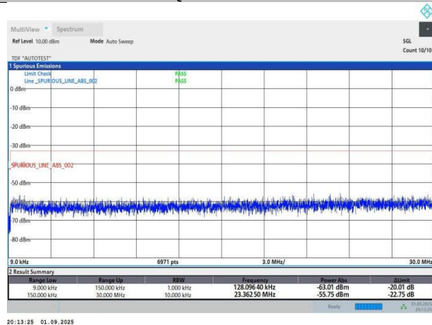
Band4-3MHz-QPSK-20385-1RB#0-PASS
