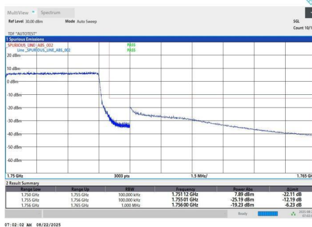
Band4-10MHz-16QAM-20350-25RB#25-PASS
