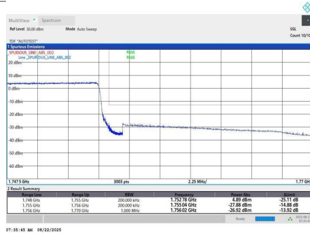
Band4-15MHz-16QAM-20325-75RB#0-PASS
