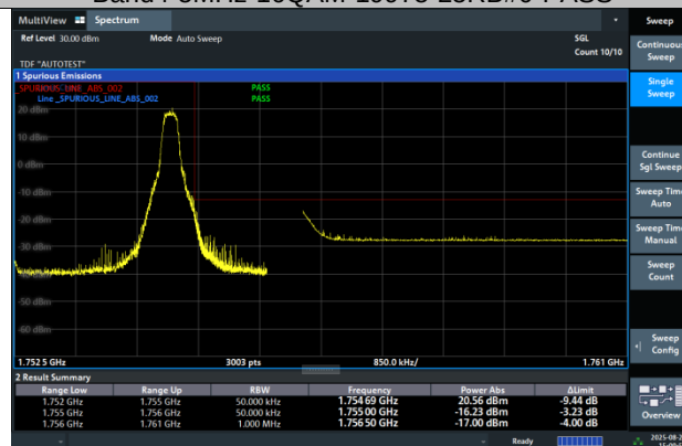
Band4-5MHz-16QAM-20375-1RB#24-PASS
