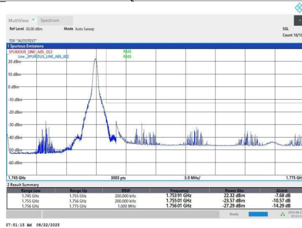
Band4-20MHz-16QAM-20300-1RB#99-PASS
