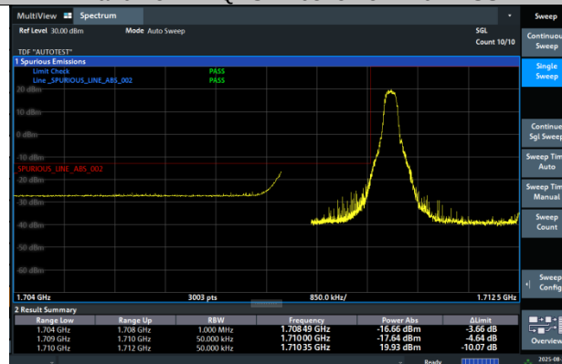
Band4-5MHz-16QAM-19975-1RB#0-PASS
