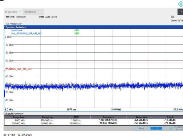
Band4-1.4MHz-QPSK-20393-1RB#0-PASS
