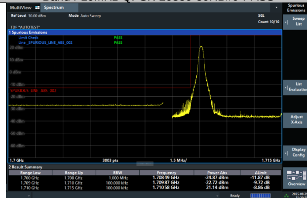
Band4-10MHz-16QAM-20000-1RB#0-PASS
