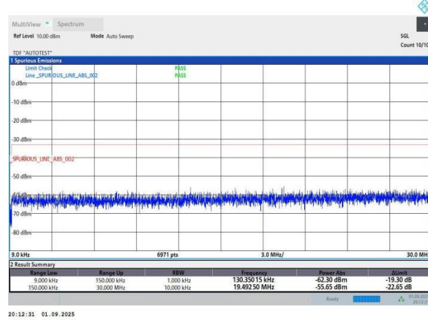
Band4-3MHz-QPSK-19965-1RB#0-PASS
