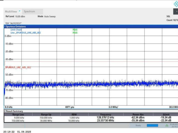
Band4-15MHz-QPSK-20325-1RB#0-PASS
