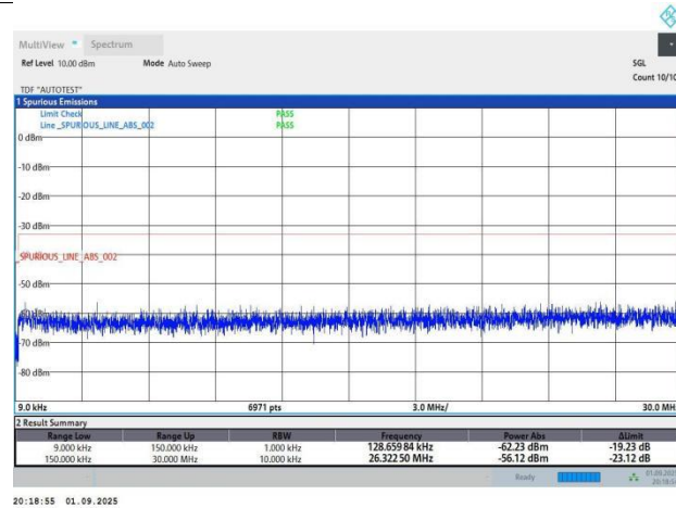
Band4-15MHz-QPSK-20175-1RB#0-PASS
