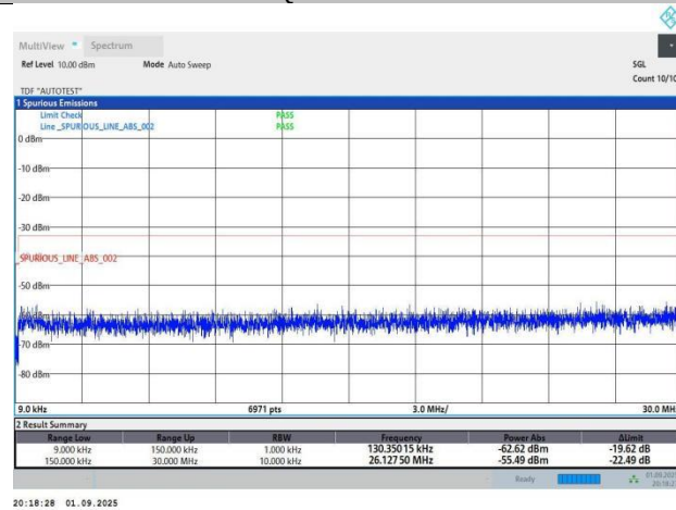
Band4-15MHz-QPSK-20025-1RB#0-PASS
