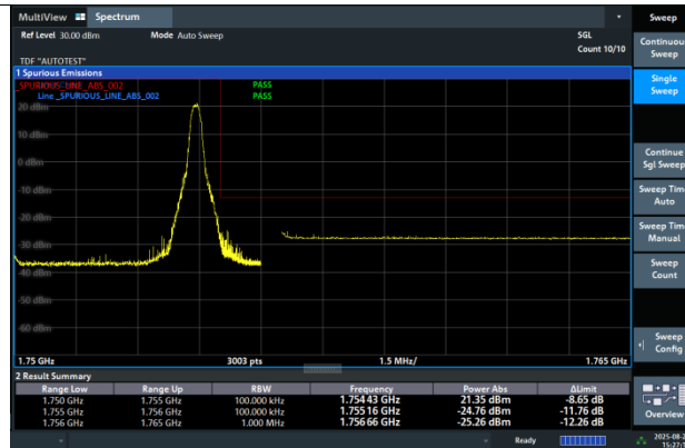
Band4-10MHz-16QAM-20350-1RB#49-PASS
