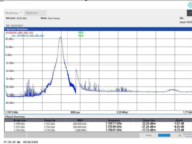
Band4-15MHz-16QAM-20325-1RB#74-PASS
