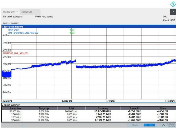
Band4-20MHz-QPSK-20300-1RB#0-PASS
