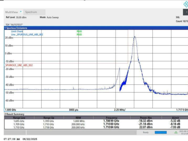
Band4-15MHz-64QAM-20025-1RB#0-PASS
