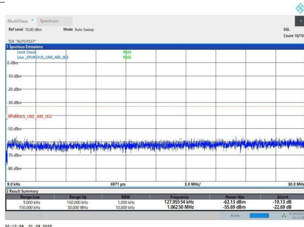
Band4-3MHz-QPSK-20175-1RB#0-PASS
