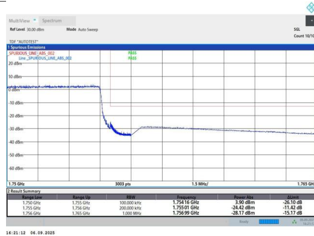
Band4-10MHz-64QAM-20350-50RB#0-PASS
