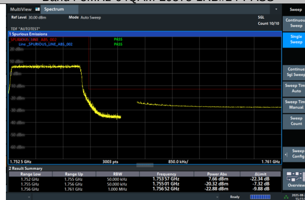
Band4-5MHz-64QAM-20375-12RB#13-PASS
