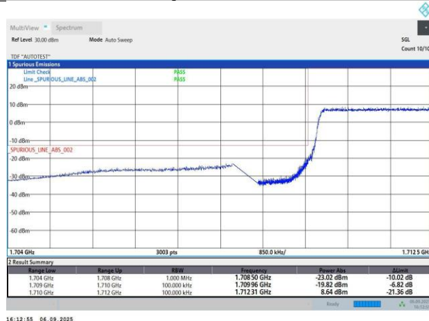
Band4-5MHz-QPSK-19975-25RB#0-PASS
