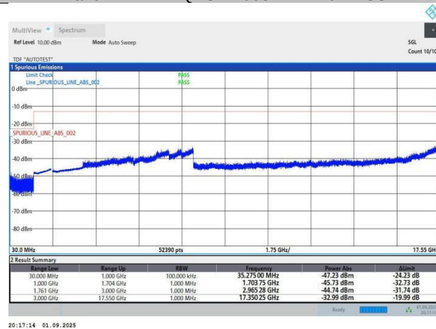
Band4-1.4MHz-QPSK-19957-1RB#0-PASS
