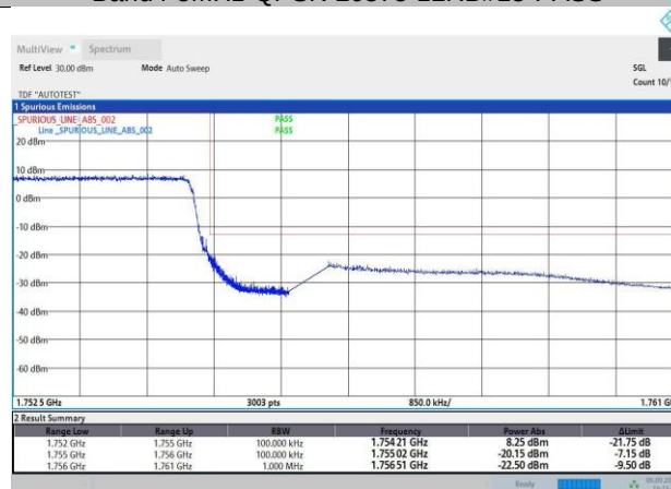
Band4-5MHz-QPSK-20375-25RB#0-PASS
