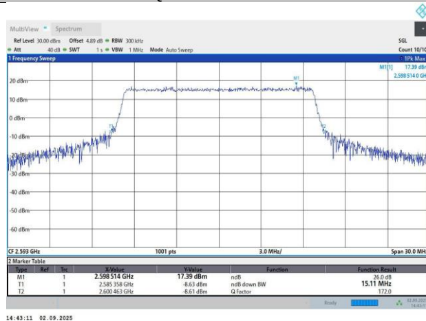
Band41-15MHz-QPSK-40620-75RB#0-13.51-15.11
