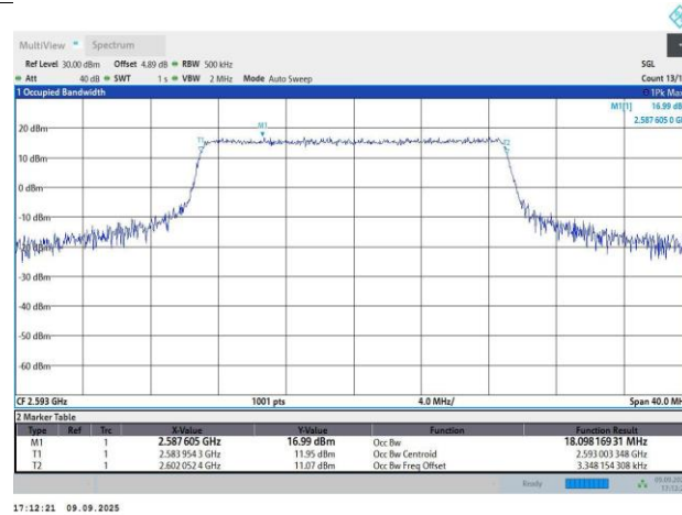
Band41-20MHz-16QAM-40620-100RB#0-18.1-20.62
