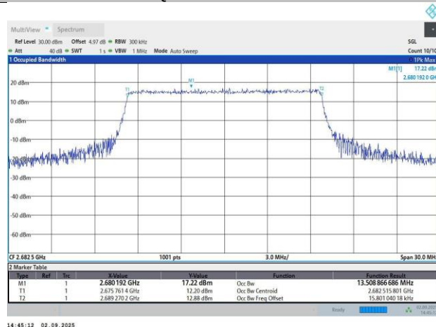
Band41-15MHz-QPSK-41515-75RB#0-13.51-15.04
