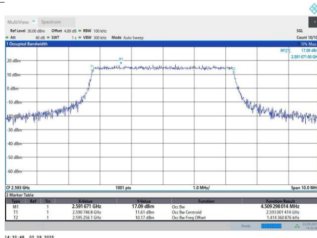
Band41-5MHz-QPSK-40620-25RB#0-4.51-5.12
