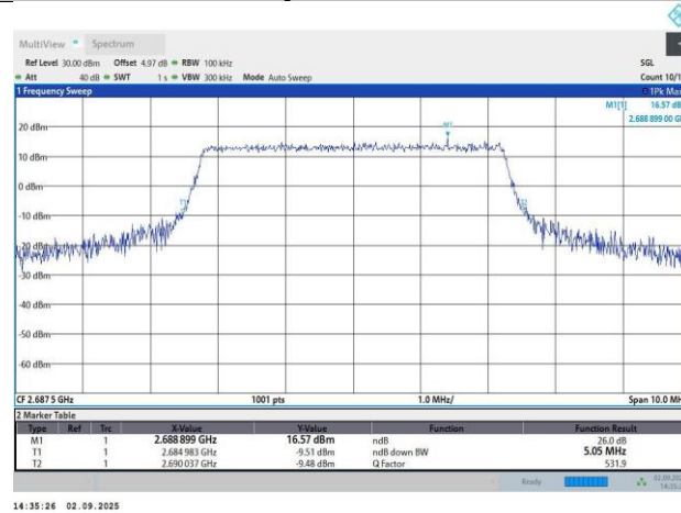
Band41-5MHz-64QAM-41565-25RB#0-4.51-5.05
