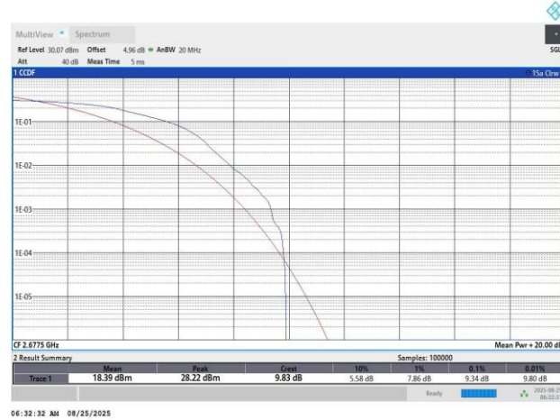
Band41-20MHz-16QAM-41490-1RB#0-9.34-13-PASS
