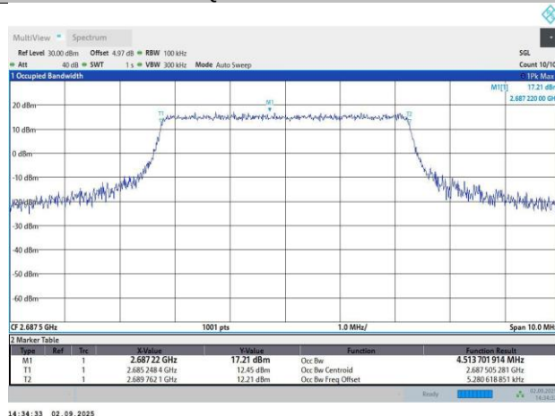
Band41-5MHz-QPSK-41565-25RB#0-4.51-5.17
