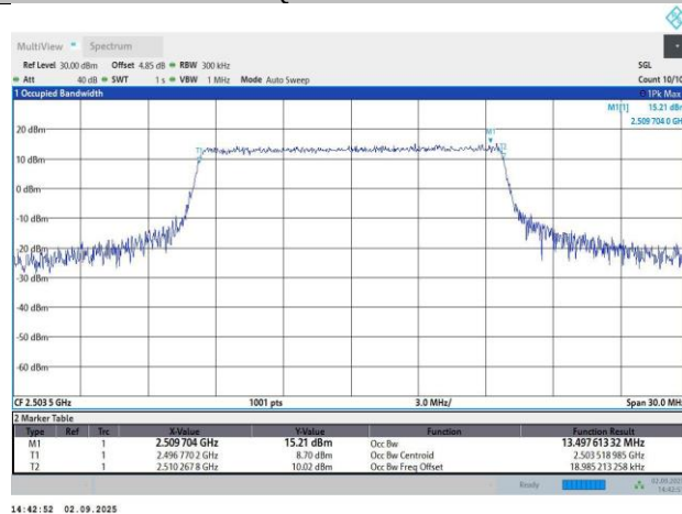
Band41-15MHz-64QAM-39725-75RB#0-13.5-14.84
