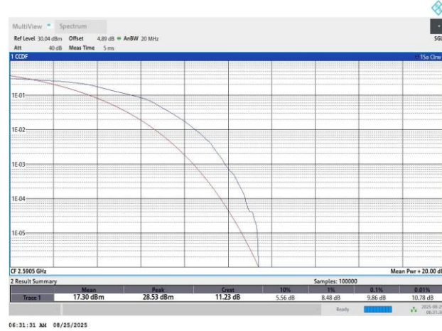
Band41-20MHz-16QAM-40620-100RB#0-9.86-13-PASS
