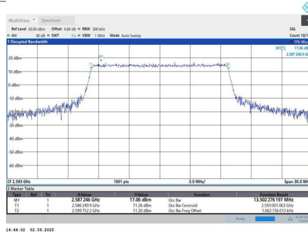
Band41-15MHz-16QAM-40620-75RB#0-13.5-14.96
