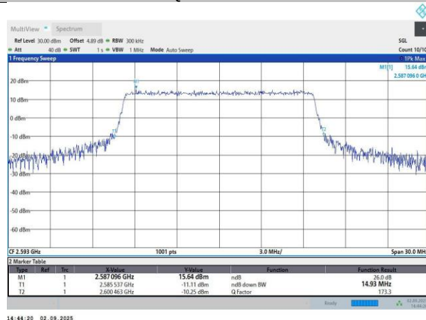
Band41-15MHz-64QAM-40620-75RB#0-13.53-14.93
