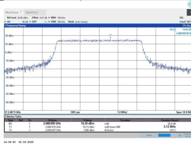
Band41-5MHz-16QAM-41565-25RB#0-4.51-5.12
