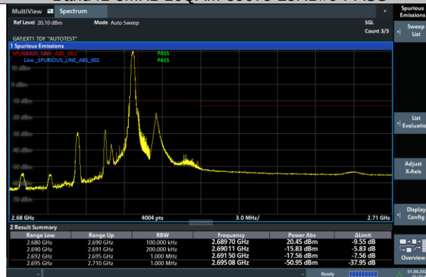
Band41-5MHz-16QAM-41565-1RB#24-PASS
