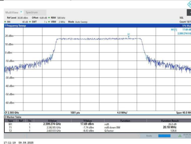
Band41-20MHz-QPSK-40620-100RB#0-18.13-20.18
