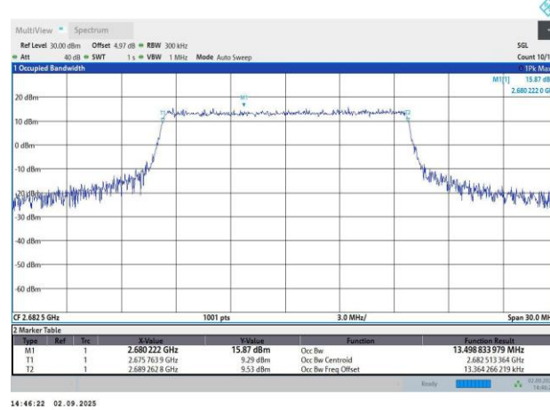
Band41-15MHz-64QAM-41515-75RB#0-13.5-14.84
