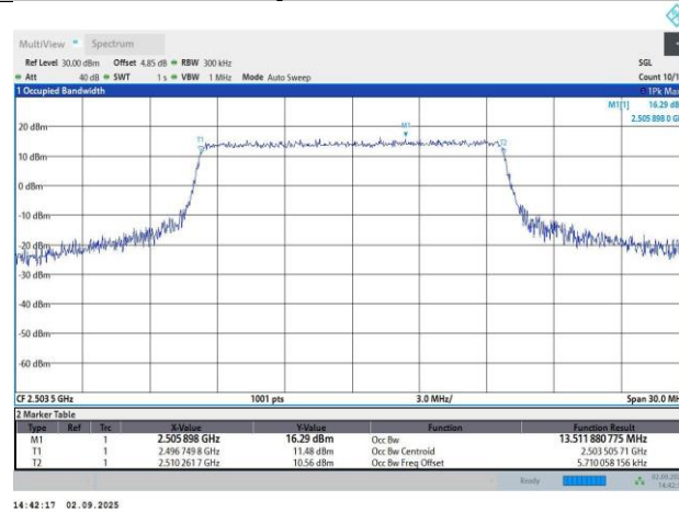
Band41-15MHz-16QAM-39725-75RB#0-13.51-14.98
