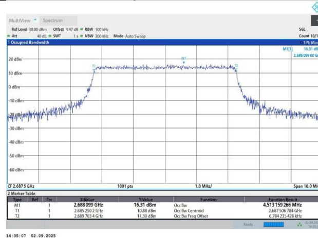
Band41-5MHz-16QAM-41565-25RB#0-4.51-5.12
