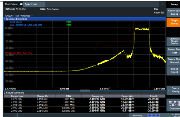
Band41-5MHz-16QAM-39675-12RB#0-PASS
