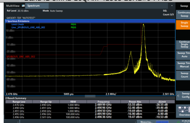
Band41-5MHz-64QAM-39675-1RB#0-PASS
