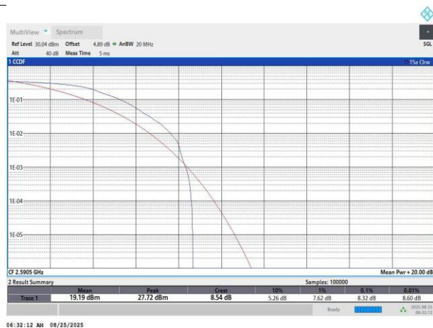
Band41-20MHz-QPSK-40620-1RB#0-8.32-13-PASS
