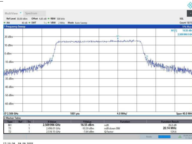
Band41-20MHz-64QAM-39750-100RB#0-18.1-20.14
