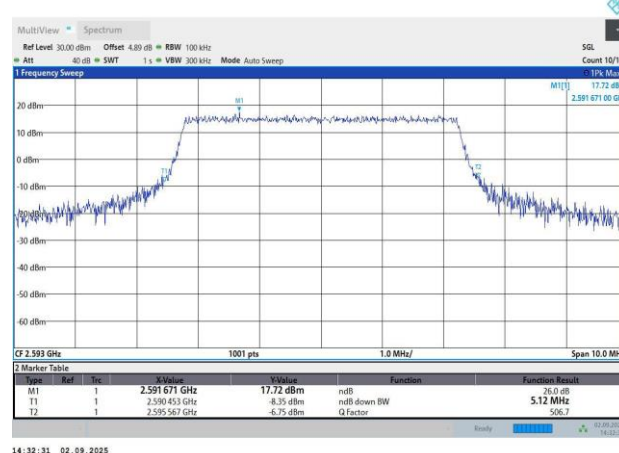
Band41-5MHz-QPSK-40620-25RB#0-4.51-5.12
