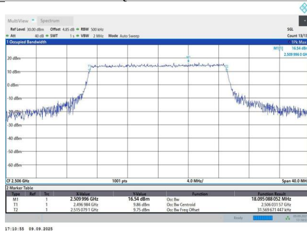
Band41-20MHz-64QAM-39750-100RB#0-18.1-20.14
