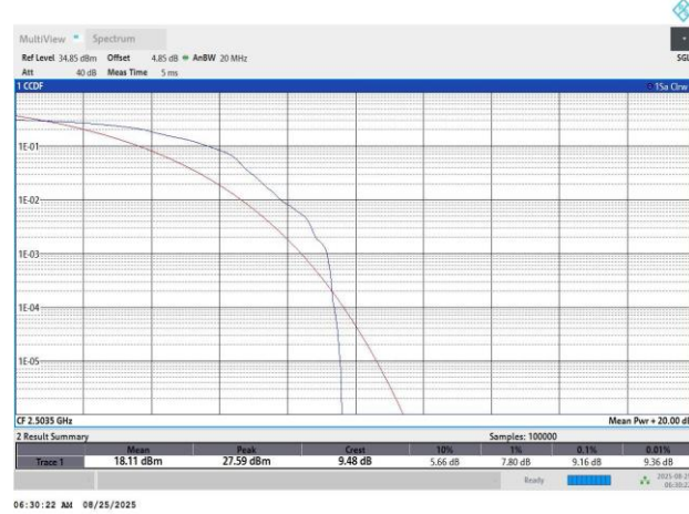
Band41-20MHz-16QAM-39750-1RB#0-9.16-13-PASS
