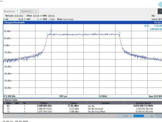
Band41-10MHz-QPSK-40620-50RB#0-9.02-10.15
