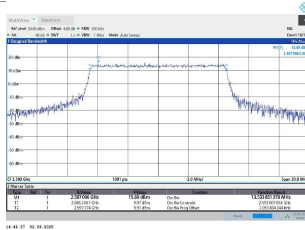
Band41-15MHz-64QAM-40620-75RB#0-13.53-14.93
