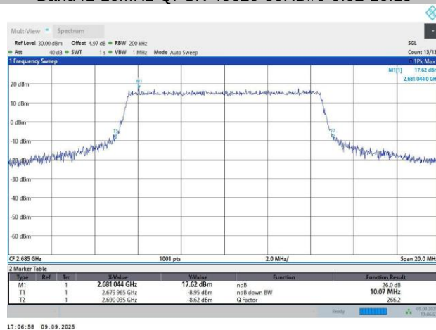
Band41-10MHz-QPSK-41540-50RB#0-9.02-10.07
