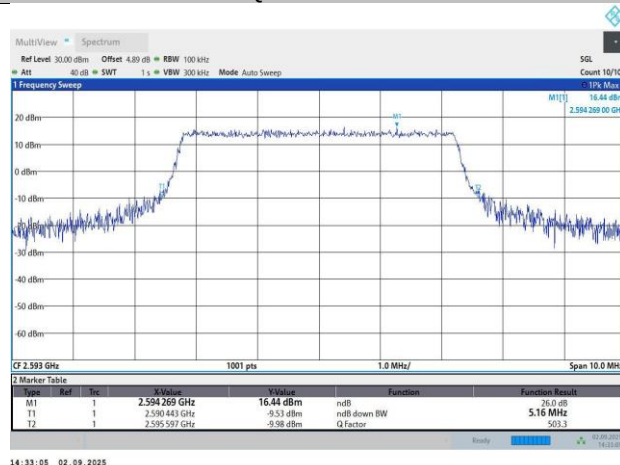
Band41-5MHz-16QAM-40620-25RB#0-4.51-5.16
