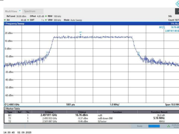
Band41-5MHz-QPSK-39675-25RB#0-4.51-5.16
