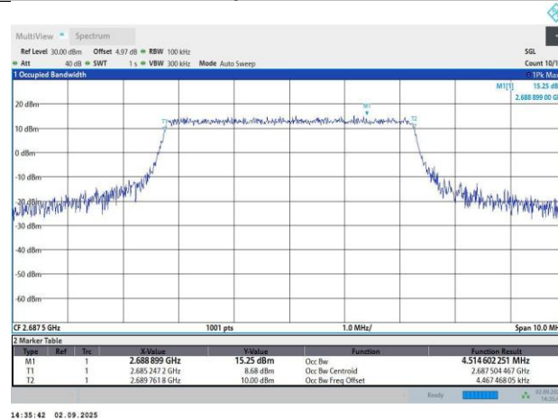
Band41-5MHz-64QAM-41565-25RB#0-4.51-5.05
