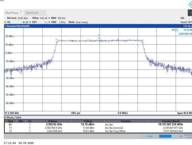
Band41-20MHz-64QAM-40620-100RB#0-18.1-20.5
