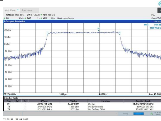
Band41-20MHz-QPSK-39750-100RB#0-18.11-20.38
