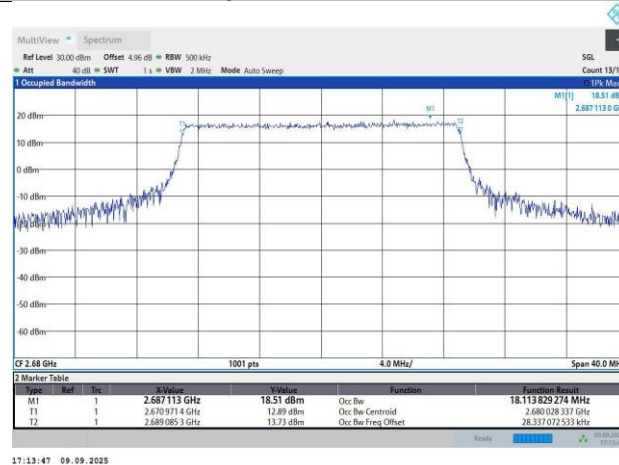
Band41-20MHz-QPSK-41490-100RB#0-18.11-20.42
