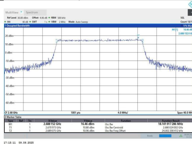
Band41-20MHz-64QAM-41490-100RB#0-18.1-20.22
