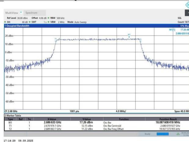
Band41-20MHz-16QAM-41490-100RB#0-18.09-20.18
