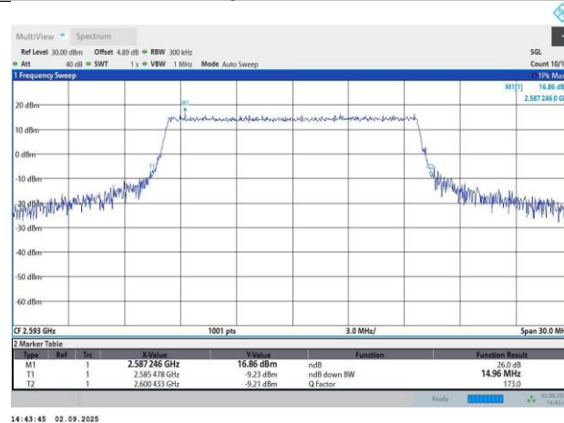
Band41-15MHz-16QAM-40620-75RB#0-13.5-14.96
