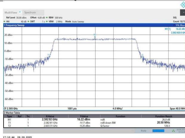
Band41-20MHz-64QAM-40620-100RB#0-18.1-20.5
