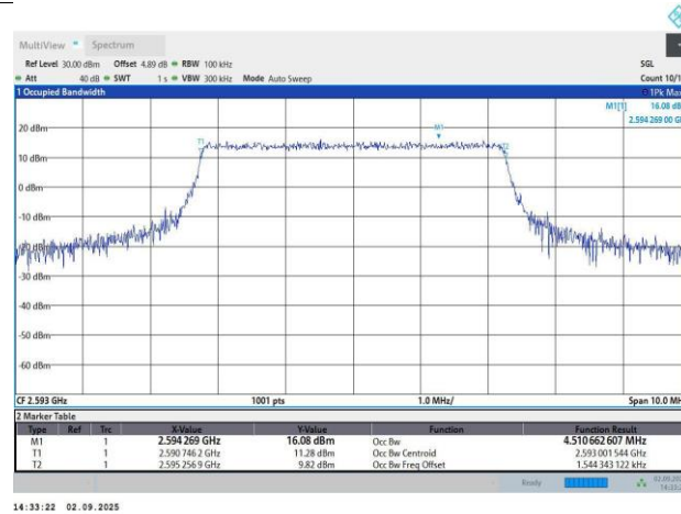
Band41-5MHz-16QAM-40620-25RB#0-4.51-5.16
