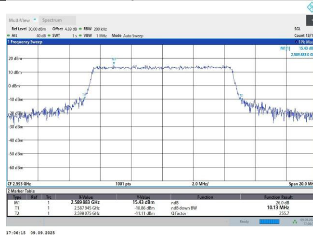
Band41-10MHz-64QAM-40620-50RB#0-9.03-10.13
