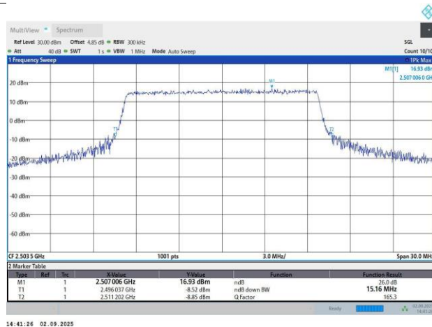
Band41-15MHz-QPSK-39725-75RB#0-13.52-15.16
