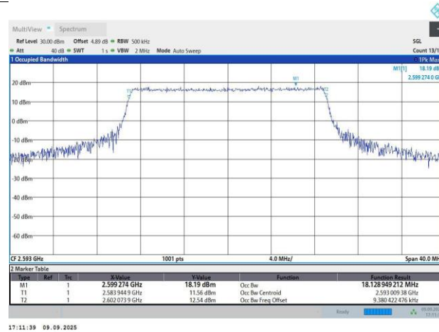
Band41-20MHz-QPSK-40620-100RB#0-18.13-20.18
