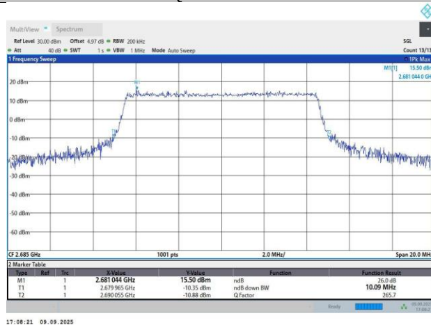
Band41-10MHz-64QAM-41540-50RB#0-9.01-10.09
