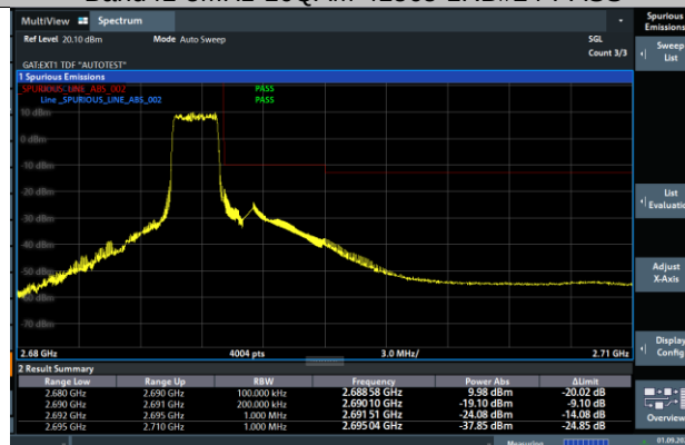
Band41-5MHz-16QAM-41565-12RB#13-PASS
