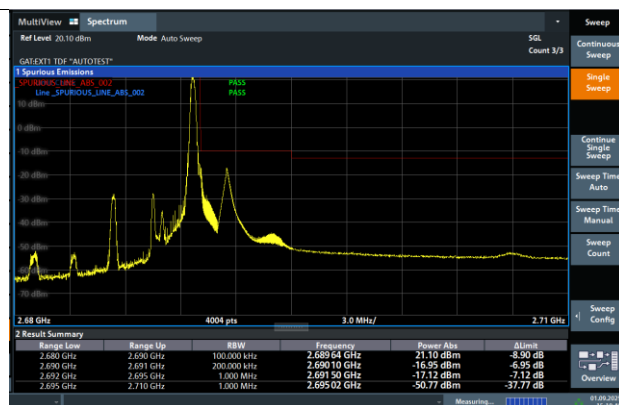
Band41-5MHz-QPSK-41565-1RB#24-PASS
