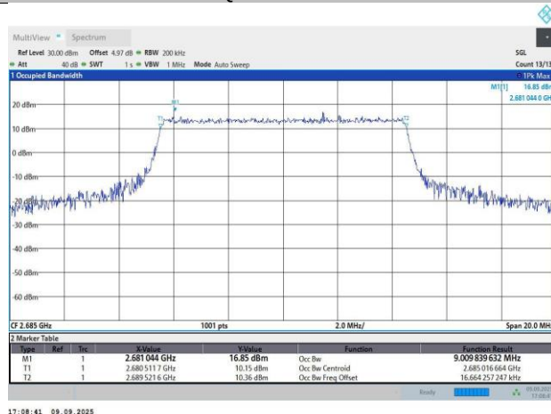
Band41-10MHz-64QAM-41540-50RB#0-9.01-10.09
