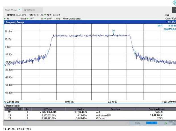
Band41-15MHz-16QAM-41515-75RB#0-13.53-14.98
