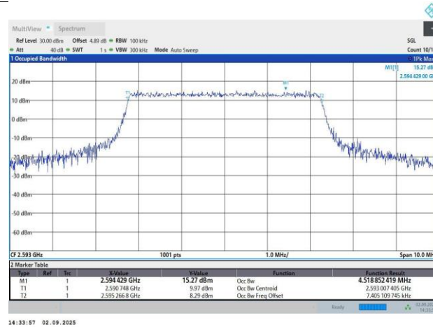
Band41-5MHz-64QAM-40620-25RB#0-4.52-5.08
