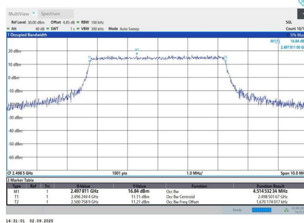
Band41-5MHz-QPSK-39675-25RB#0-4.51-5.16
