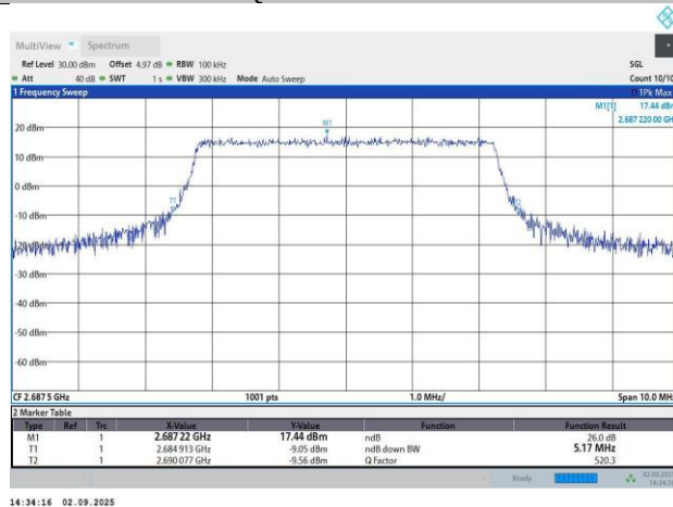
Band41-5MHz-QPSK-41565-25RB#0-4.51-5.17
