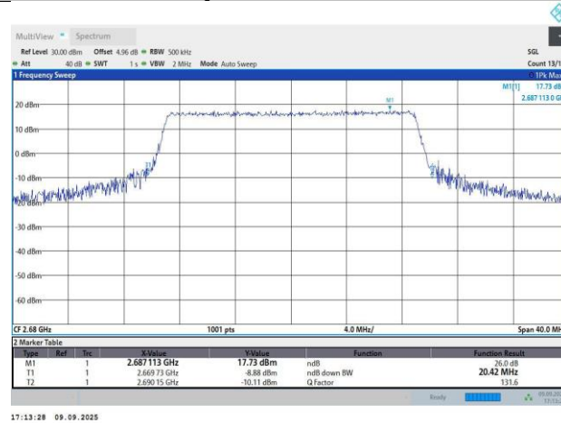
Band41-20MHz-QPSK-41490-100RB#0-18.11-20.42
