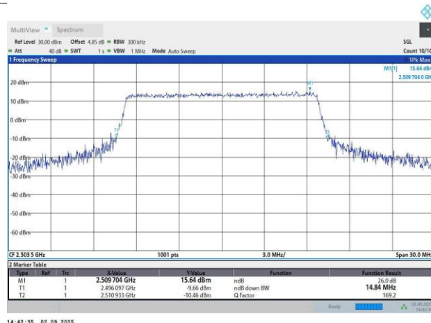
Band41-15MHz-64QAM-39725-75RB#0-13.5-14.84
