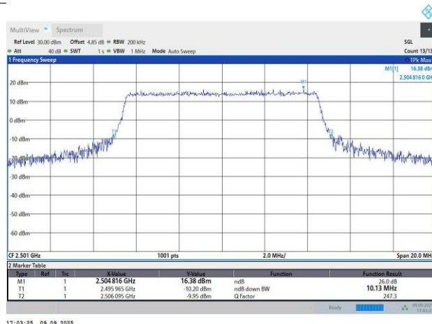
Band41-10MHz-16QAM-39700-50RB#0-9.03-10.13
