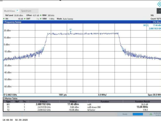
Band41-15MHz-QPSK-41515-75RB#0-13.51-15.04
