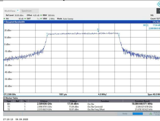
Band41-20MHz-16QAM-39750-100RB#0-18.08-19.98
