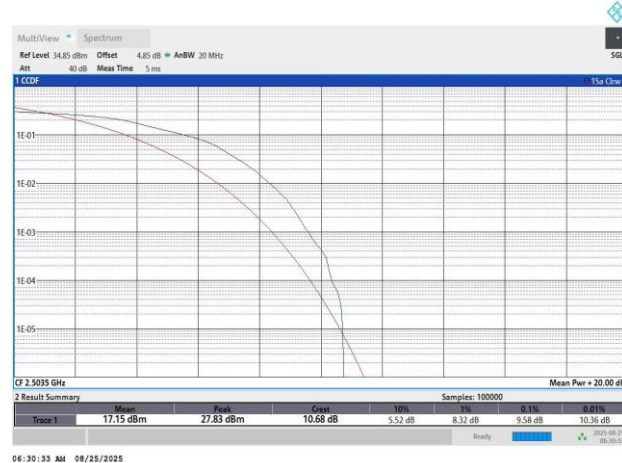
Band41-20MHz-16QAM-39750-100RB#0-9.58-13-PASS
