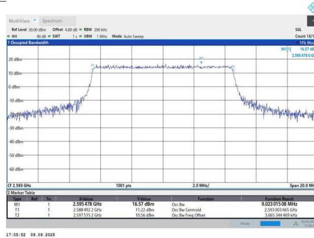
Band41-10MHz-16QAM-40620-50RB#0-9.02-10.15
