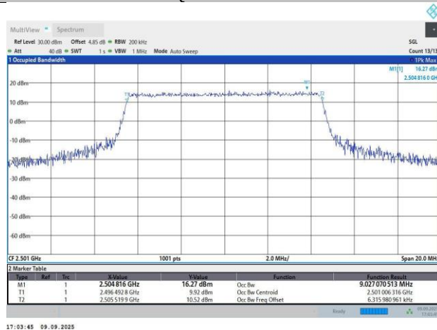
Band41-10MHz-16QAM-39700-50RB#0-9.03-10.13
