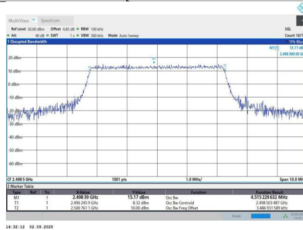
Band41-5MHz-64QAM-39675-25RB#0-4.52-5.08
