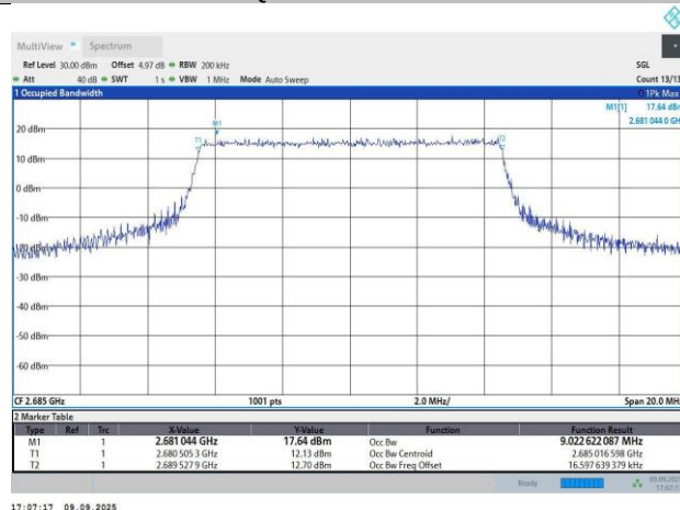
Band41-10MHz-QPSK-41540-50RB#0-9.02-10.07
