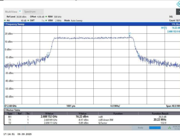
Band41-20MHz-64QAM-41490-100RB#0-18.1-20.22
