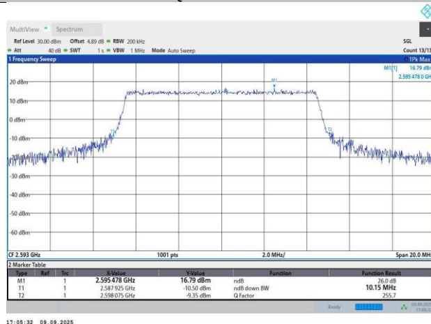
Band41-10MHz-16QAM-40620-50RB#0-9.02-10.15
