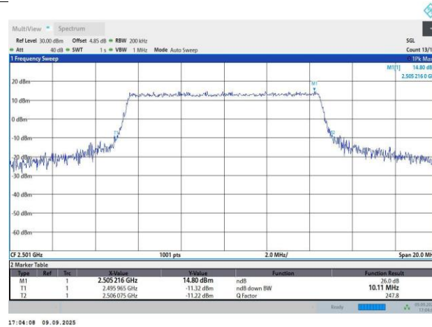
Band41-10MHz-64QAM-39700-50RB#0-9.02-10.11
