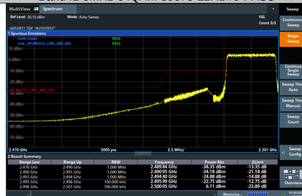
Band41-5MHz-64QAM-39675-25RB#0-PASS
