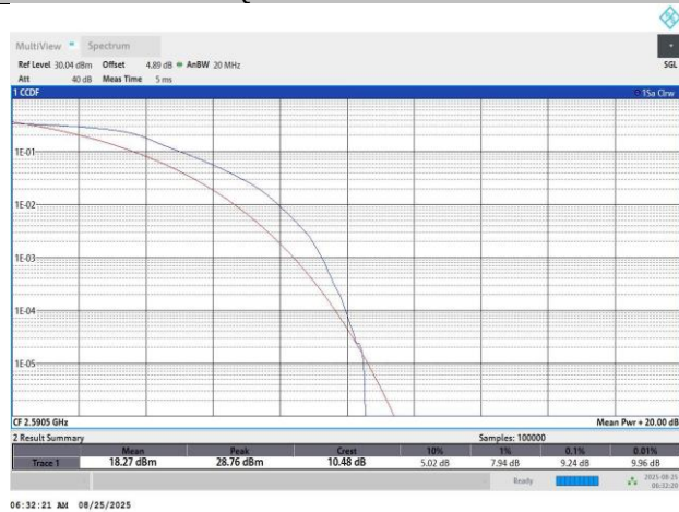
Band41-20MHz-QPSK-40620-100RB#0-9.24-13-PASS
