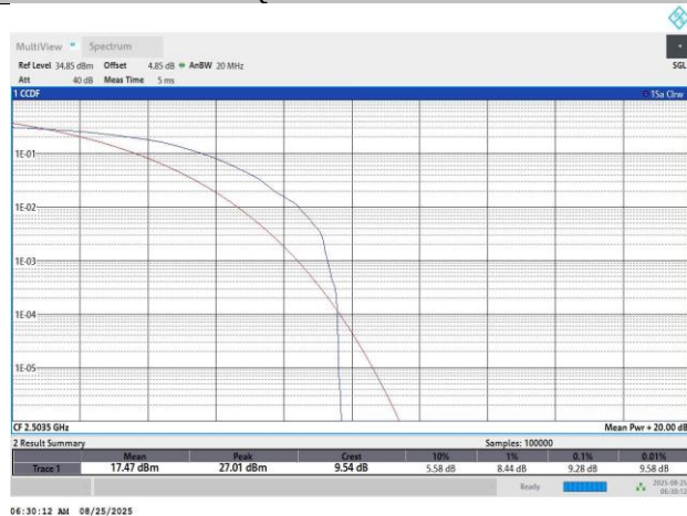
Band41-20MHz-64QAM-39750-1RB#0-9.28-13-PASS
