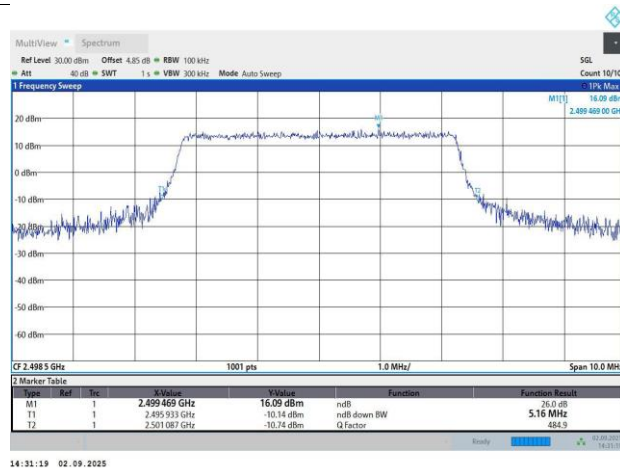
Band41-5MHz-16QAM-39675-25RB#0-4.51-5.16
