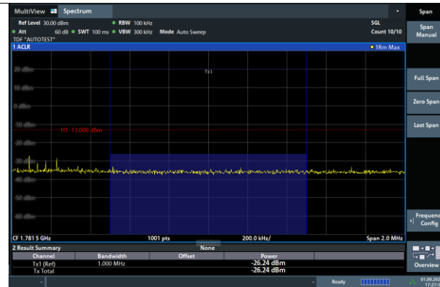
Band66-1.4MHz-64QAM-132665-1RB#5-PASS
