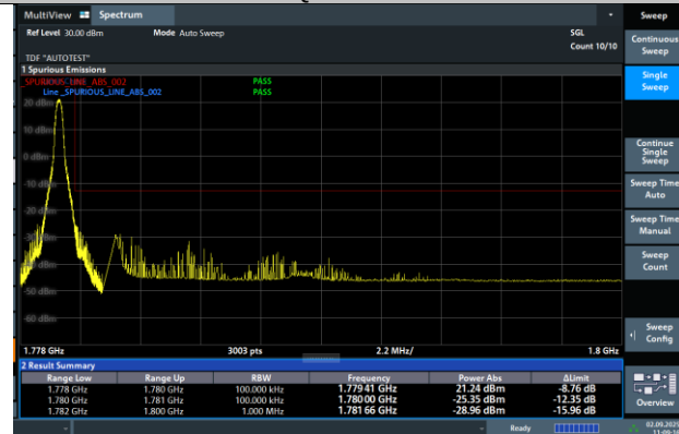
Band66-10MHz-16QAM-132622-1RB#49-PASS
