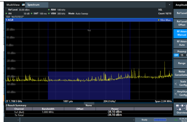
Band66-3MHz-16QAM-131987-1RB#0-PASS
