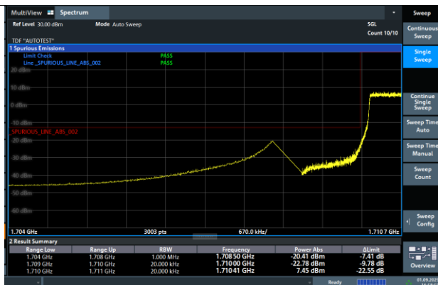
Band66-1.4MHz-16QAM-131979-3RB#0-PASS
