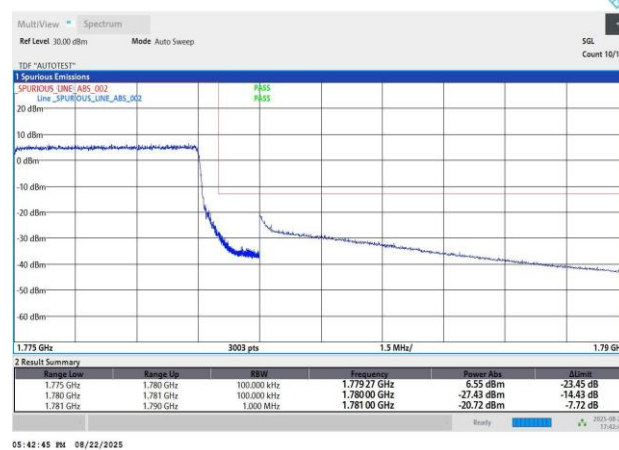
Band66-10MHz-64QAM-132622-25RB#25-PASS
