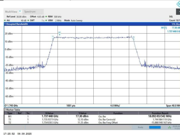
Band66-20MHz-64QAM-132322-100RB#0-18.09-20.14
