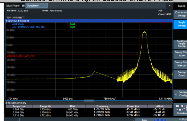
Band66-1.4MHz-64QAM-132665-6RB#0-PASS
