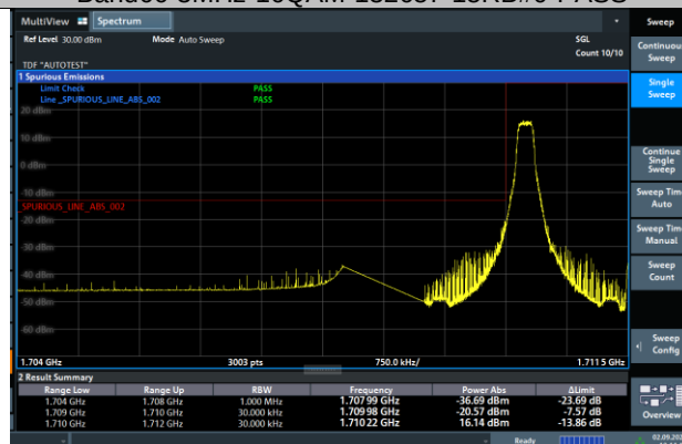
Band66-3MHz-16QAM-132657-15RB#0-PASS
