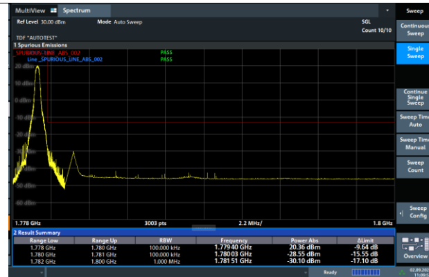
Band66-10MHz-64QAM-132622-1RB#49-PASS
