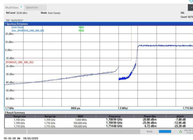
Band66-10MHz-64QAM-132022-25RB#0-PASS
