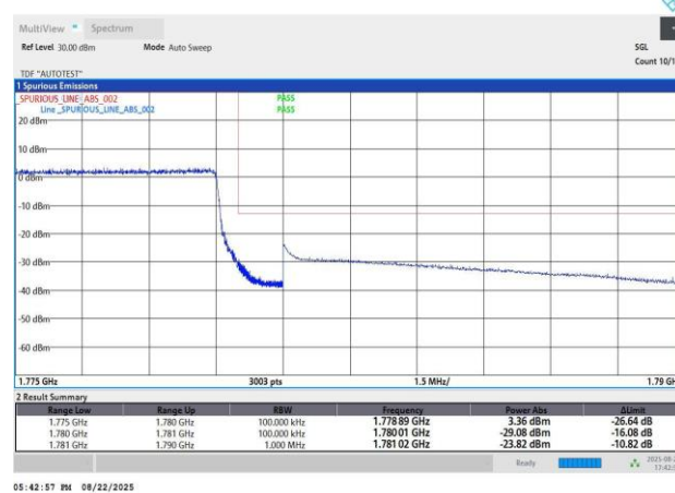
Band66-10MHz-64QAM-132622-50RB#0-PASS
