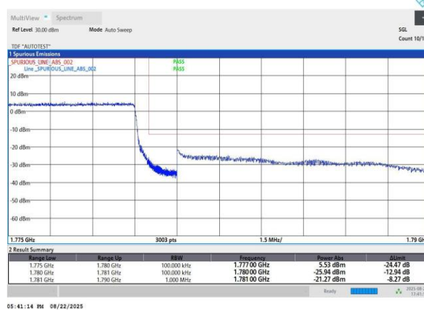
Band66-10MHz-QPSK-132622-50RB#0-PASS
