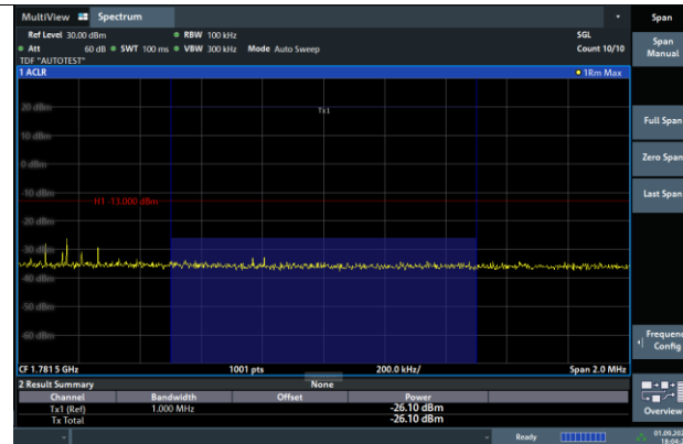
Band66-3MHz-64QAM-132657-1RB#14-PASS
