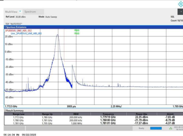
Band66-15MHz-QPSK-132597-1RB#74-PASS
