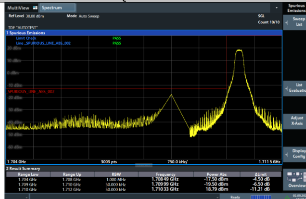
Band66-5MHz-16QAM-131997-1RB#0-PASS
