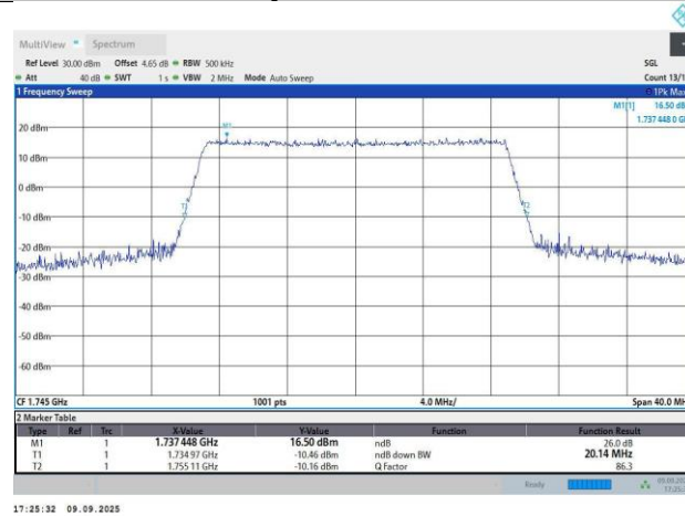
Band66-20MHz-64QAM-132322-100RB#0-18.09-20.14
