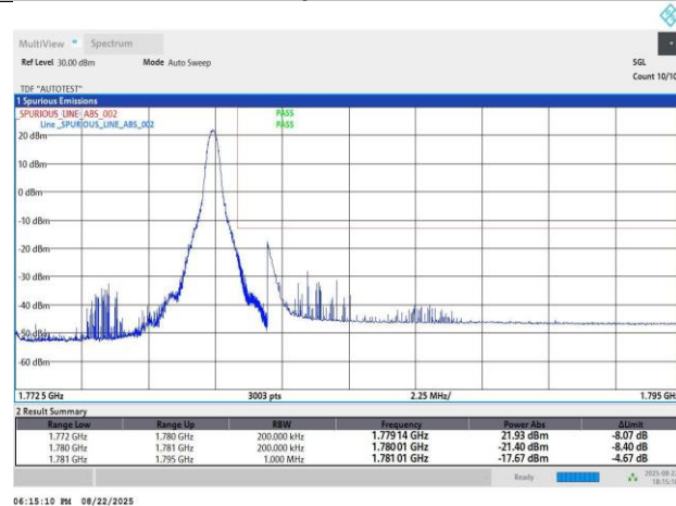
Band66-15MHz-16QAM-132597-1RB#74-PASS
