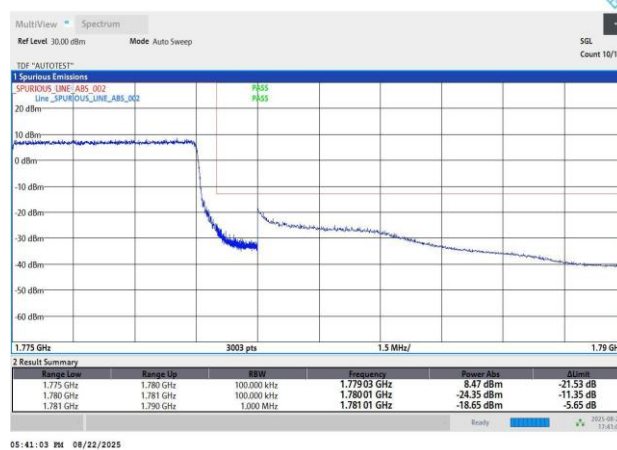
Band66-10MHz-QPSK-132622-25RB#25-PASS
