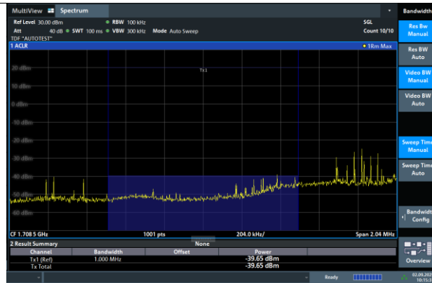
Band66-3MHz-64QAM-131987-1RB#0-PASS
