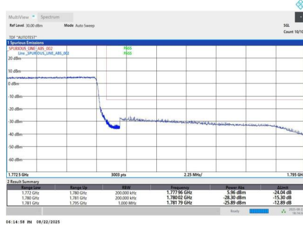
Band66-15MHz-QPSK-132597-75RB#0-PASS
