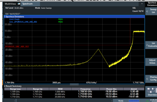
Band66-1.4MHz-64QAM-131979-3RB#0-PASS
