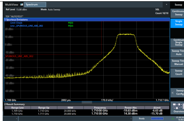
Band66-1.4MHz-64QAM-131979-1RB#0-PASS
