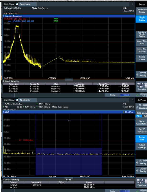
Band66-1.4MHz-16QAM-132665-1RB#5-PASS
