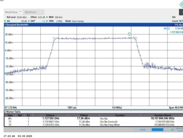
Band66-20MHz-64QAM-132072-100RB#0-18.1-20.06
