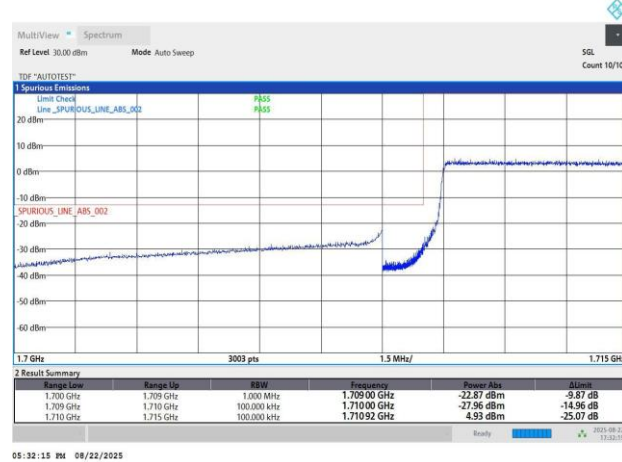
Band66-10MHz-16QAM-132022-50RB#0-PASS
