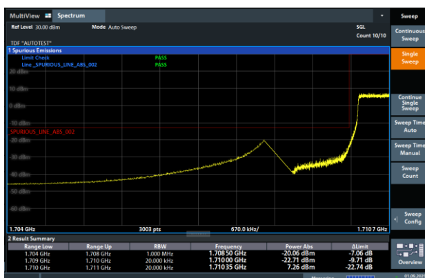
Band66-1.4MHz-16QAM-131979-6RB#0-PASS
