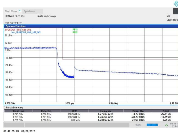
Band66-10MHz-16QAM-132622-50RB#0-PASS
