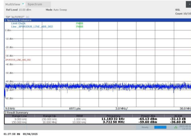
N26-15KHz-10MHz-DFT-s-OFDM QPSK-167300-1RB#0-PASS
