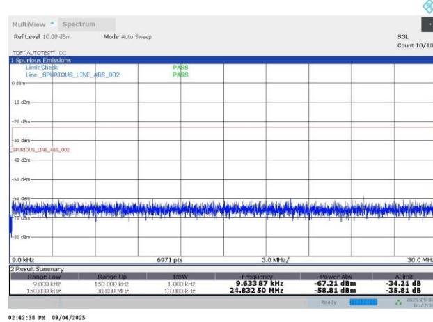
N26-15KHz-20MHz-DFT-s-OFDM PI/2 BPSK-167300-1RB#105-PASS
