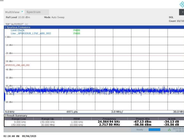
N26-15KHz-20MHz-DFT-s-OFDM QPSK-166800-100RB#0-PASS
