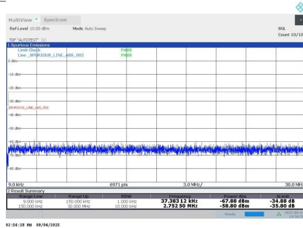
N26-15KHz-20MHz-DFT-s-OFDM QPSK-167800-1RB#0-PASS
