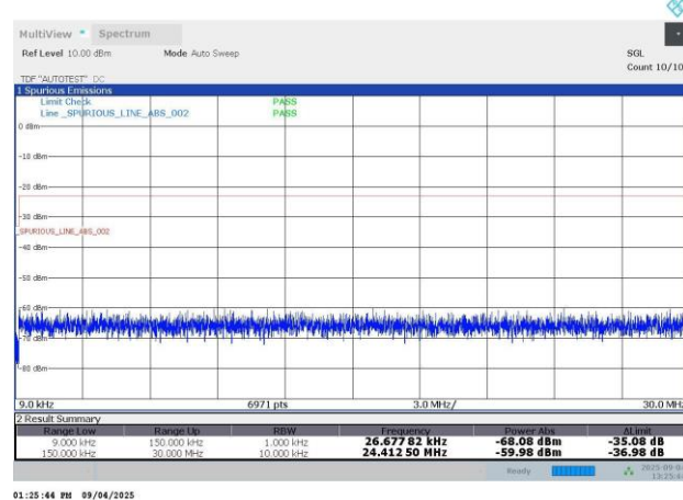
N26-15KHz-10MHz-CP-OFDM QPSK-165800-1RB#0-PASS
