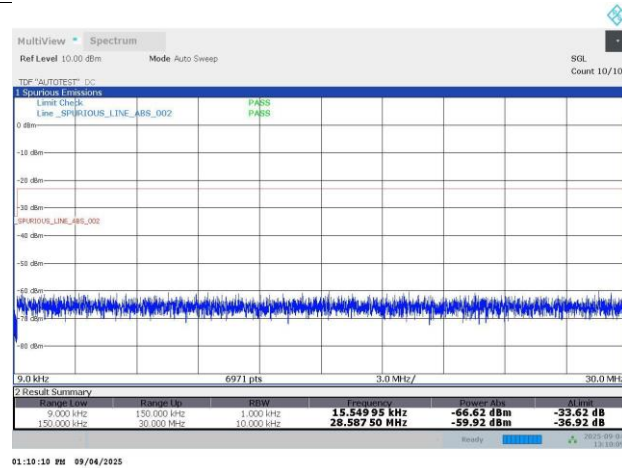
N26-15KHz-5MHz-DFT-s-OFDM QPSK-169300-1RB#0-PASS
