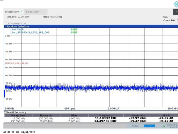
N26-15KHz-20MHz-DFT-s-OFDM QPSK-167300-100RB#0-PASS
