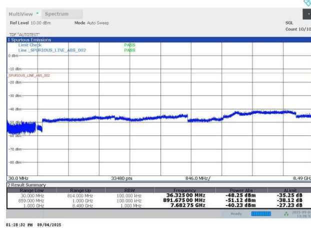
N26-15KHz-10MHz-DFT-s-OFDM QPSK-165800-1RB#51-PASS
