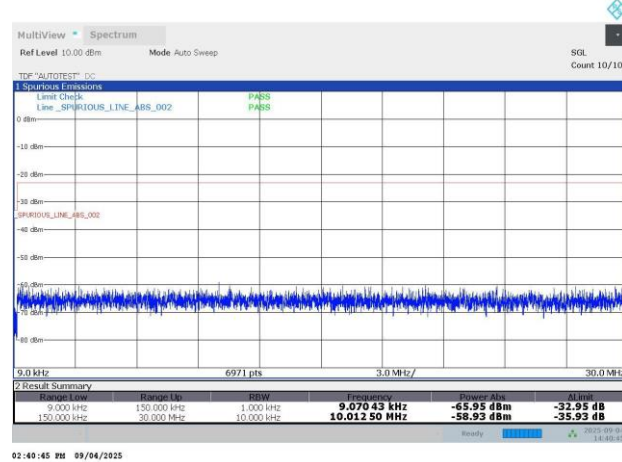
N26-15KHz-20MHz-DFT-s-OFDM PI/2 BPSK-167300-1RB#0-PASS
