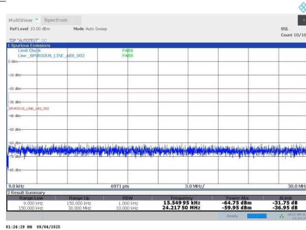
N26-15KHz-10MHz-DFT-s-OFDM QPSK-165800-50RB#0-PASS
