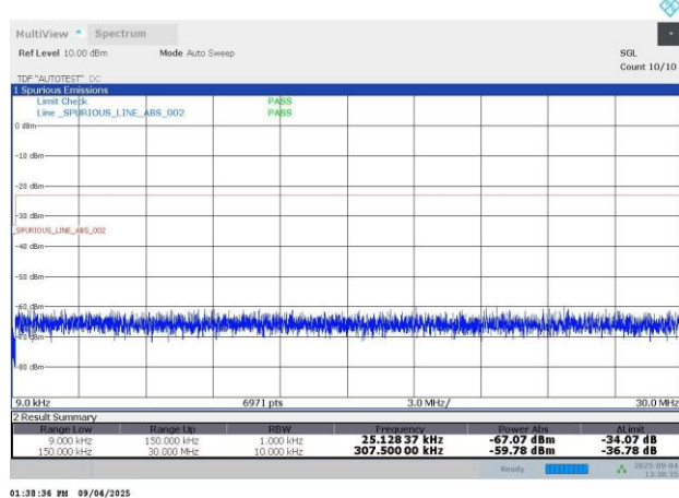
N26-15KHz-10MHz-DFT-s-OFDM PI/2 BPSK-167300-1RB#0-PASS
