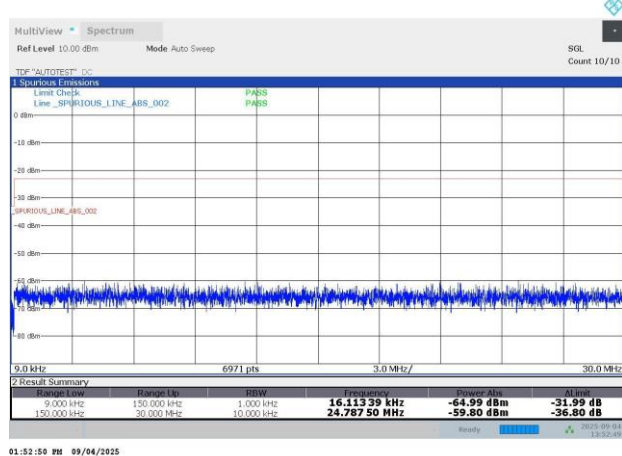
N26-15KHz-10MHz-DFT-s-OFDM PI/2 BPSK-168800-50RB#0-PASS
