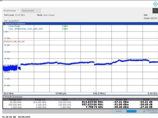
N26-15KHz-10MHz-DFT-s-OFDM PI/2 BPSK-167300-50RB#0-PASS
