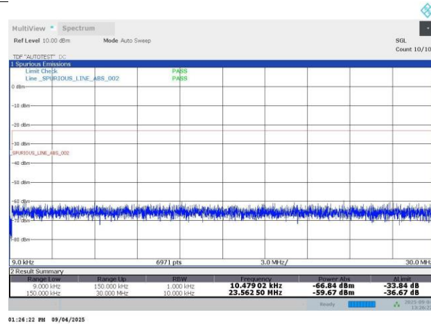
N26-15KHz-10MHz-DFT-s-OFDM QPSK-165800-1RB#0-PASS
