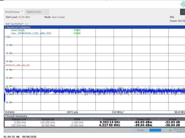
N26-15KHz-5MHz-CP-OFDM QPSK-169300-1RB#0-PASS
