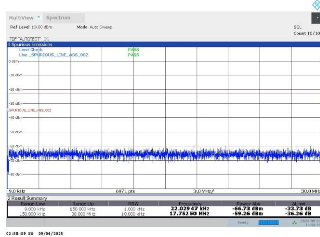
N26-15KHz-20MHz-DFT-s-OFDM PI/2 BPSK-167800-1RB#105-PASS
