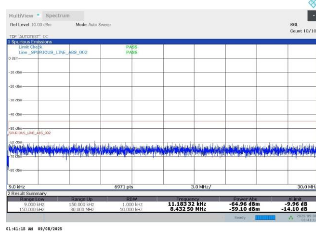
N38-30KHz-10MHz-DFT-s-OFDM PI/2 BPSK-519000-1RB#0-PASS
