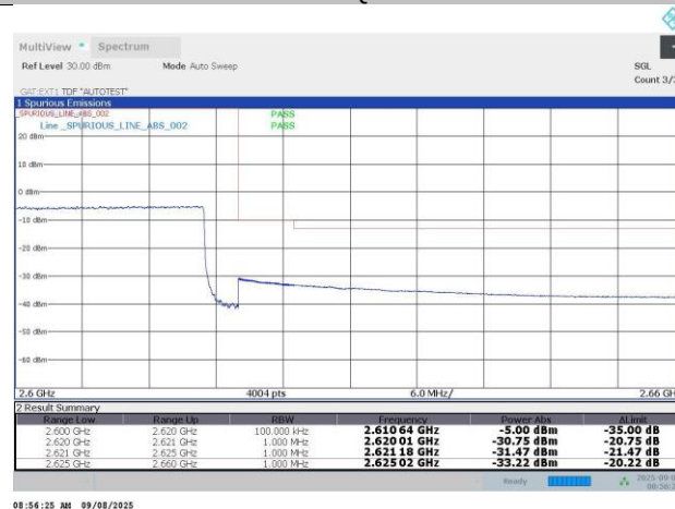
N38-30KHz-40MHz-DFT-s-OFDM PI/2 BPSK-520000-100RB#0-PASS
