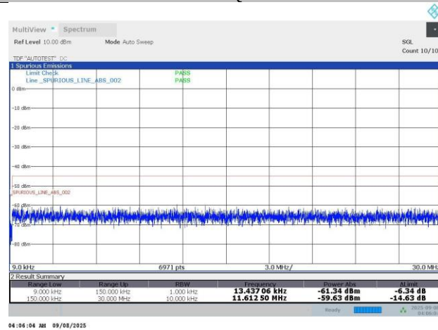
N38-30KHz-20MHz-DFT-s-OFDM PI/2 BPSK-519000-50RB#0-PASS
