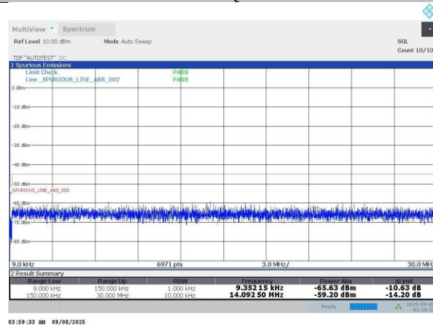
N38-30KHz-20MHz-DFT-s-OFDM PI/2 BPSK-516000-50RB#0-PASS
