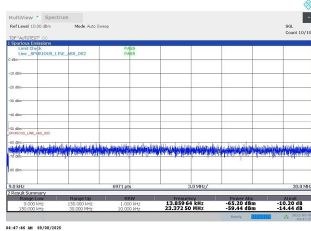
N38-30KHz-20MHz-DFT-s-OFDM PI/2 BPSK-522000-1RB#50-PASS
