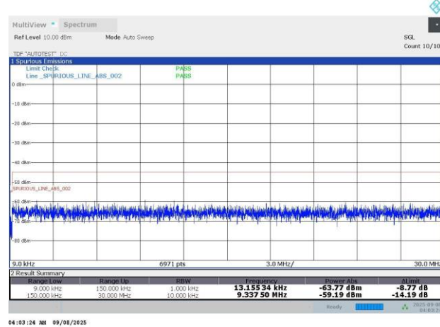
N38-30KHz-20MHz-DFT-s-OFDM PI/2 BPSK-516000-1RB#50-PASS
