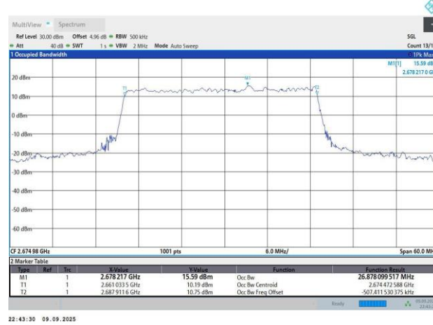
N41-30KHz-30MHz-DFT-s-OFDM QPSK-534996-75RB#0-26.88-29.13
