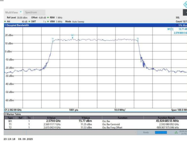
N41-30KHz-50MHz-DFT-s-OFDM QPSK-518598-128RB#0-45.92-50.35
