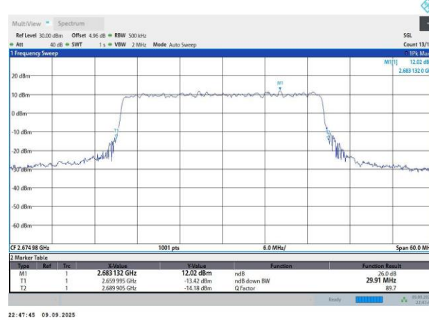
N41-30KHz-30MHz-CP-OFDM 256QAM-534996-78RB#0-27.93-29.91
