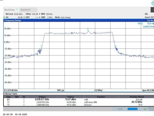
N41-30KHz-30MHz-DFT-s-OFDM QPSK-534996-75RB#0-26.88-29.13
