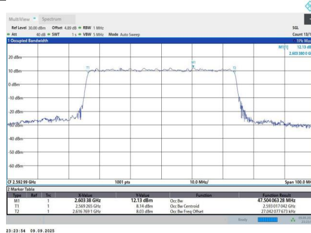
N41-30KHz-50MHz-CP-OFDM 256QAM-518598-133RB#0-47.5-50.65
