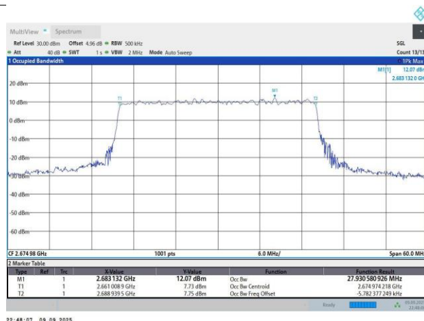
N41-30KHz-30MHz-CP-OFDM 256QAM-534996-78RB#0-27.93-29.91
