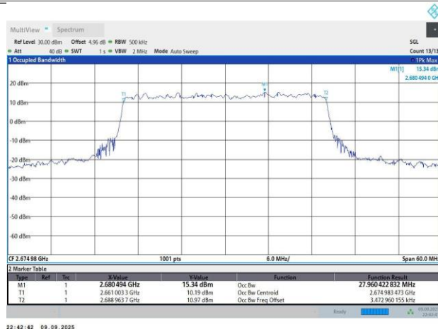
N41-30KHz-30MHz-CP-OFDM QPSK-534996-78RB#0-27.96-30.33
