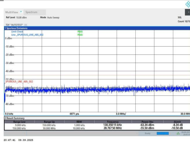
N41-30KHz-60MHz-DFT-s-OFDM PI/2 BPSK-505200-1RB#0-PASS
