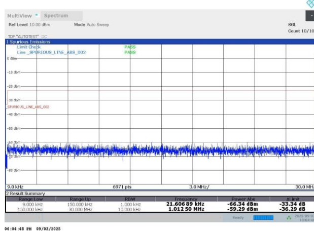
N5-15KHz-20MHz-DFT-s-OFDM PI/2 BPSK-167300-100RB#0-PASS
