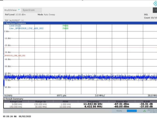
N5-15KHz-20MHz-DFT-s-OFDM PI/2 BPSK-166800-100RB#0-PASS
