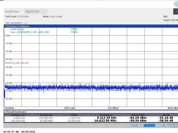
N5-15KHz-15MHz-CP-OFDM QPSK-168300-79RB#0-PASS
