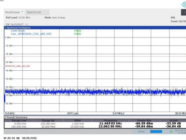
N5-15KHz-15MHz-DFT-s-OFDM QPSK-168300-1RB#78-PASS
