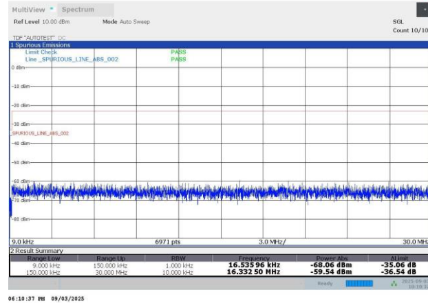
N5-15KHz-20MHz-DFT-s-OFDM QPSK-167800-100RB#0-PASS
