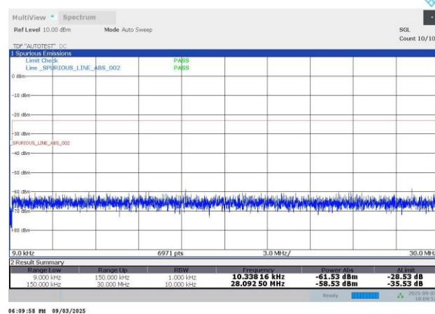
N5-15KHz-20MHz-CP-OFDM QPSK-167800-106RB#0-PASS
