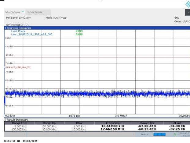
N5-15KHz-20MHz-DFT-s-OFDM PI/2 BPSK-167800-100RB#0-PASS
